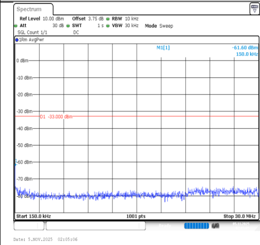
Band4-3MHz-QPSK-20175-1RB#0-0.15~30- PASS
