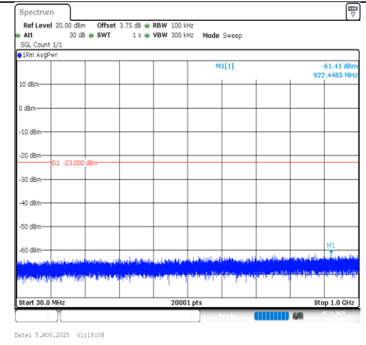
Band4-1.4MHz-64QAM-20393-1RB#0-30~1000- PASS
