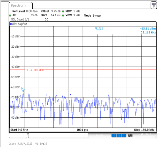
Band4-1.4MHz-64QAM-20393-1RB#5- 0.009~0.15-PASS
