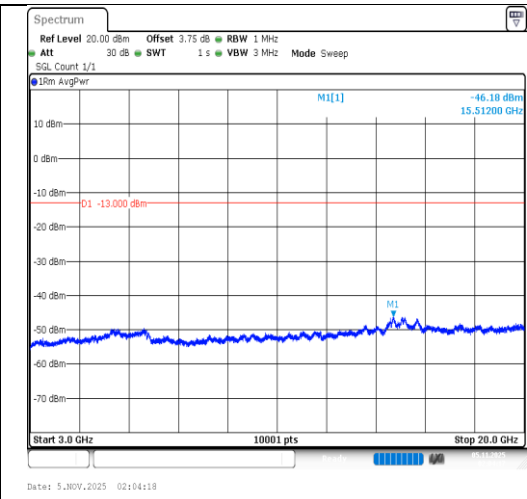
Band4-3MHz-16QAM-19965-15RB#0- 3000~20000-PASS
