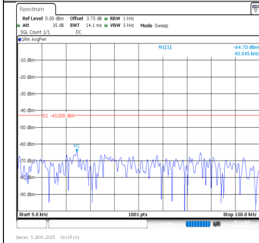
Band4-3MHz-QPSK-20175-1RB#0-0.009~0.15- PASS
