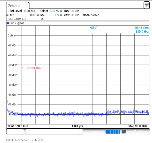
Band4-1.4MHz-64QAM-20393-1RB#5-0.15~30- PASS
