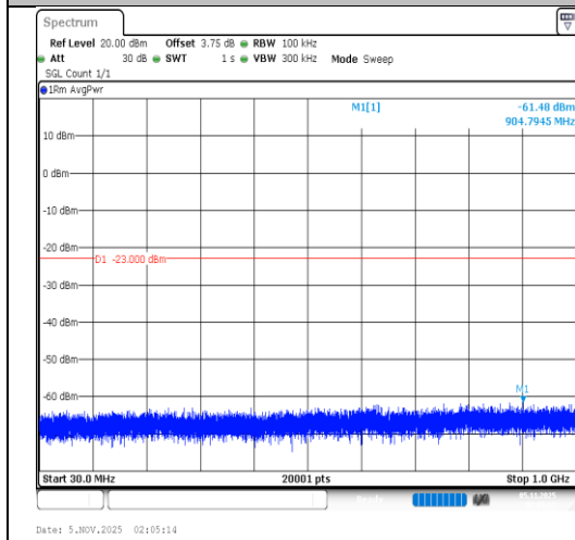
Band4-3MHz-QPSK-20175-1RB#0-30~1000- PASS
