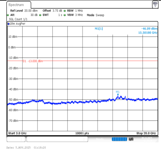
Band4-1.4MHz-64QAM-20393-1RB#0- 3000~20000-PASS
