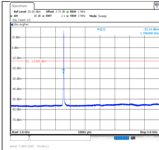
Band4-3MHz-16QAM-19965-15RB#0- 1000~3000-PASS
