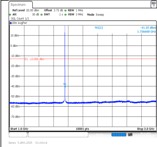
Band4-1.4MHz-64QAM-20393-1RB#0- 1000~3000-PASS
