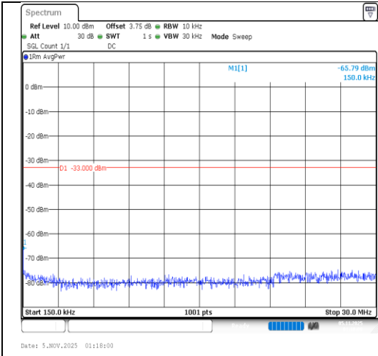
Band4-1.4MHz-64QAM-20393-1RB#0-0.15~30- PASS
