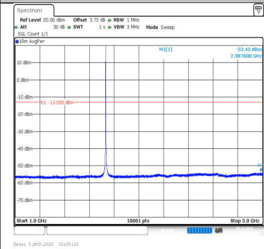
Band4-3MHz-QPSK-20175-1RB#0-1000~3000- PASS
