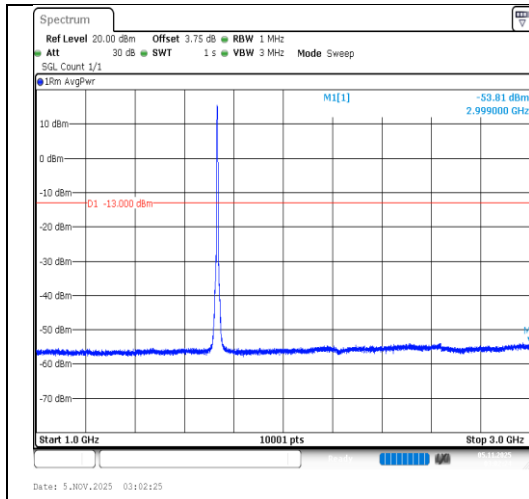
Band4-5MHz-QPSK-20175-25RB#0-1000~3000-PASS
