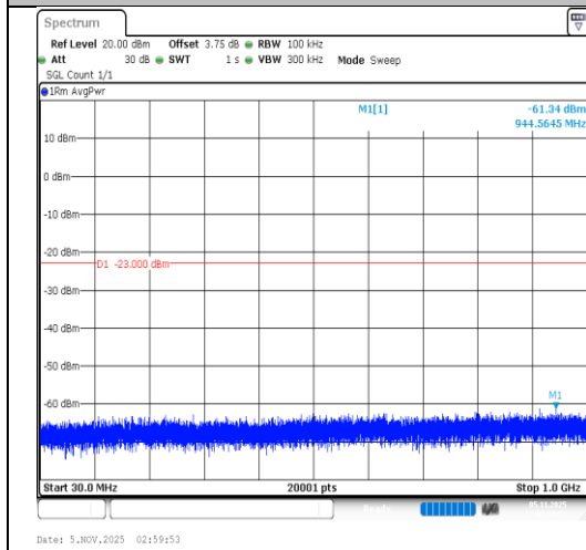
Band4-5MHz-64QAM-20175-1RB#0-30~1000-PASS
