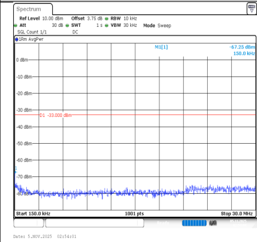
Band4-5MHz-16QAM-19975-1RB#0-0.15~30- PASS
