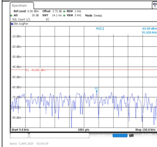
Band4-5MHz-64QAM-20175-1RB#0-0.009~0.15-PASS
