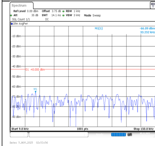
Band4-5MHz-16QAM-19975-1RB#0-0.009~0.15- PASS
