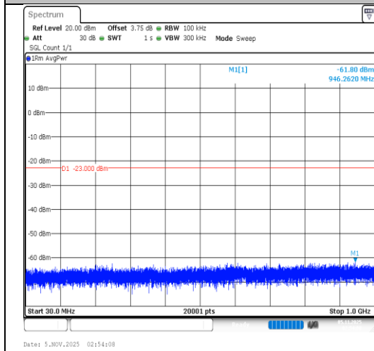
Band4-5MHz-16QAM-19975-1RB#0-30~1000- PASS
