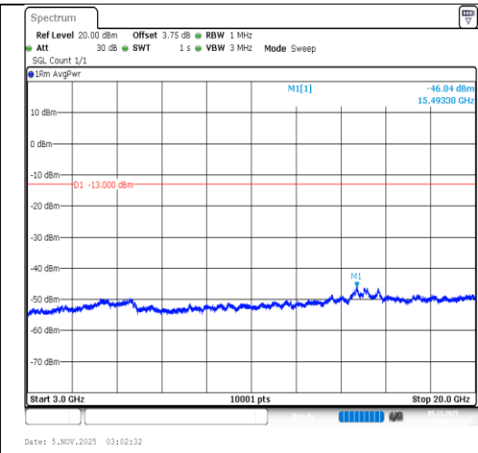
Band4-5MHz-QPSK-20175-25RB#0-3000~20000-PASS
