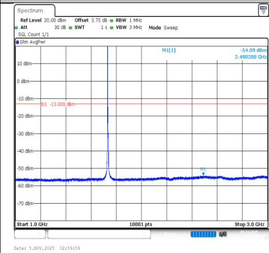
Band4-5MHz-64QAM-20175-1RB#0-1000~3000-PASS
