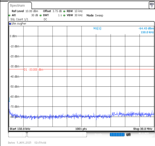
Band4-5MHz-64QAM-20175-1RB#0-0.15~30-PASS
