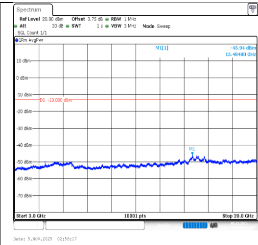
Band4-5MHz-64QAM-19975-25RB#0- 3000~20000-PASS
