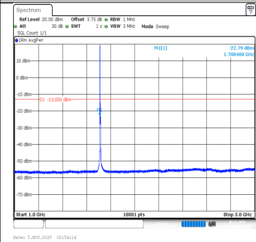
Band4-5MHz-16QAM-19975-1RB#0-1000~3000- PASS
