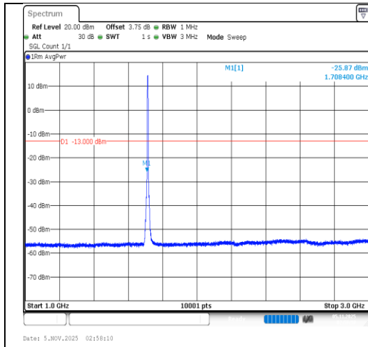
Band4-5MHz-64QAM-19975-25RB#0- 1000~3000-PASS
