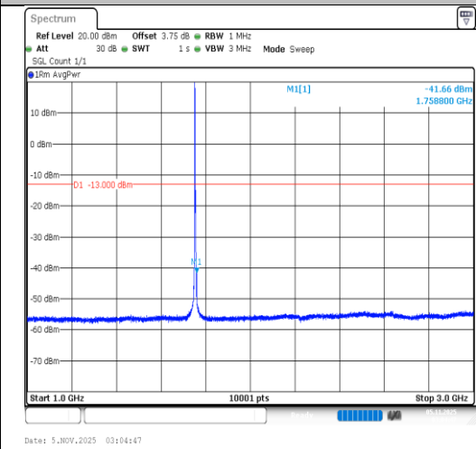
Band4-5MHz-16QAM-20375-1RB#0-1000~3000- PASS
