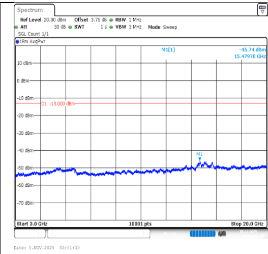
Band4-10MHz-16QAM-20000-50RB#0- 3000~20000-PASS
