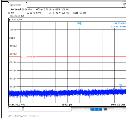
Band4-5MHz-16QAM-20375-1RB#0-30~1000- PASS
