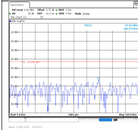
Band4-10MHz-QPSK-20175-1RB#0-0.009~0.15- PASS
