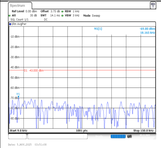
Band4-10MHz-16QAM-20000-50RB#0-0.009~0.15-PASS
