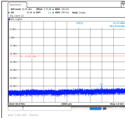
Band4-10MHz-16QAM-20000-1RB#49-30~1000-PASS
