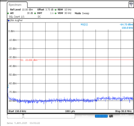
Band4-10MHz-QPSK-20175-1RB#0-0.15~30- PASS
