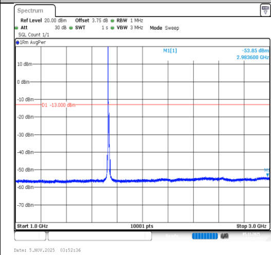
Band4-10MHz-QPSK-20175-1RB#0-1000~3000- PASS
