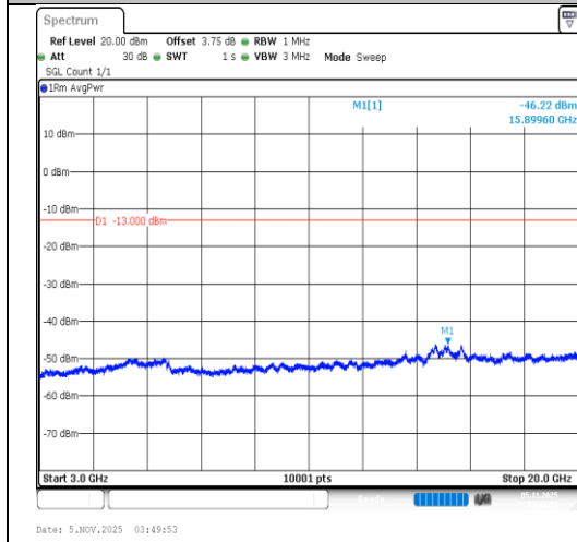
Band4-10MHz-16QAM-20000-1RB#49-3000~20000-PASS
