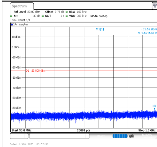
Band4-10MHz-QPSK-20175-1RB#0-30~1000- PASS
