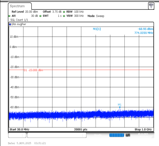
Band4-10MHz-16QAM-20000-50RB#0-30~1000-PASS
