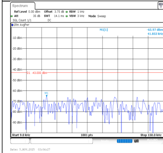
Band4-5MHz-16QAM-20375-1RB#0-0.009~0.15- PASS
