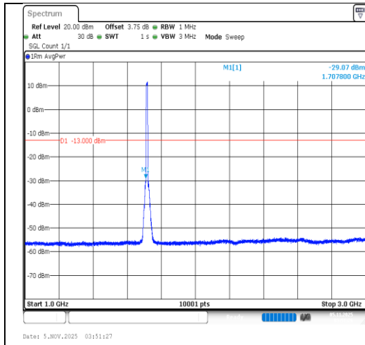
Band4-10MHz-16QAM-20000-50RB#0- 1000~3000-PASS
