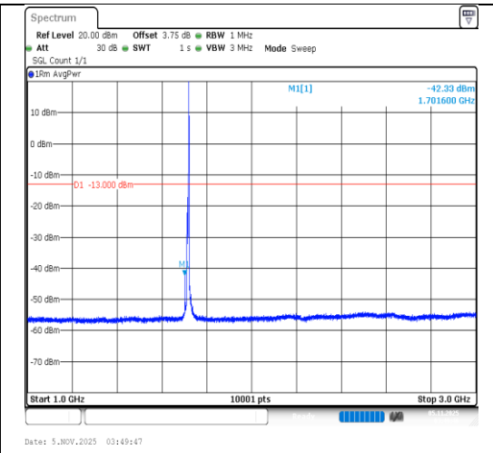
Band4-10MHz-16QAM-20000-1RB#49-1000~3000-PASS
