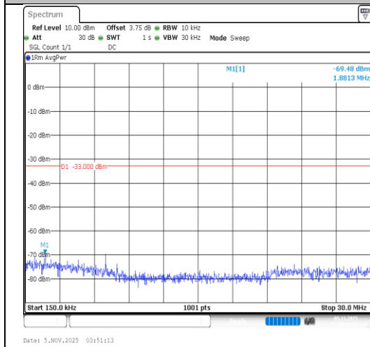
Band4-10MHz-16QAM-20000-50RB#0-0.15~30-PASS
