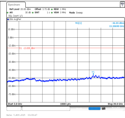
Band4-5MHz-64QAM-20375-25RB#0- 3000~20000-PASS
