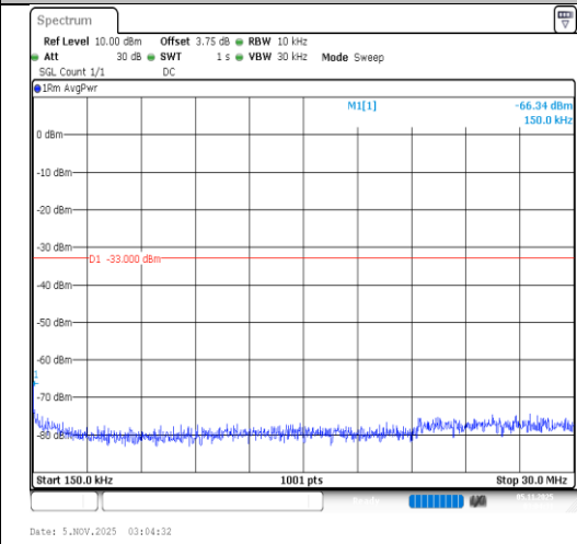
Band4-5MHz-16QAM-20375-1RB#0-0.15~30- PASS
