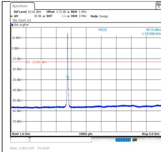
Band4-5MHz-64QAM-20375-25RB#0- 1000~3000-PASS
