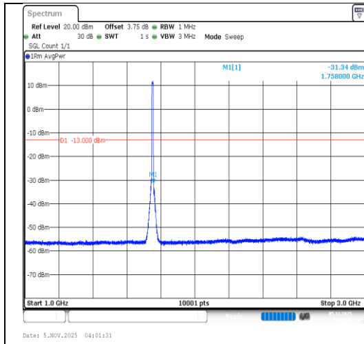
Band4-10MHz-16QAM-20350-50RB#0- 1000~3000-PASS
