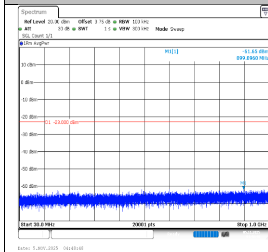
Band4-15MHz-64QAM-20175-1RB#0-30~1000- PASS
