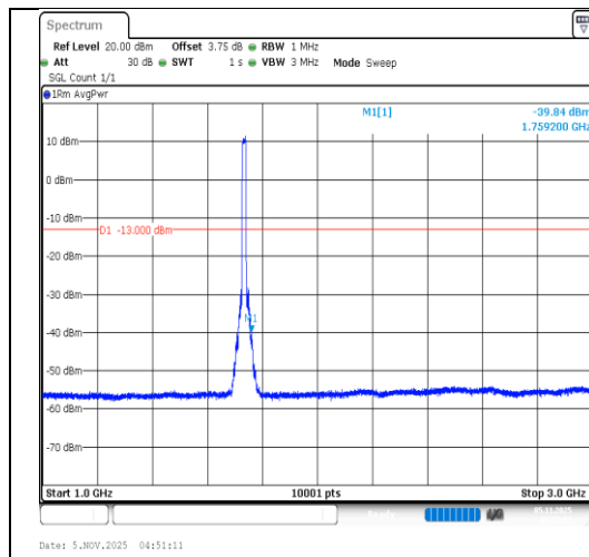
Band4-15MHz-QPSK-20175-75RB#0- 1000~3000-PASS
