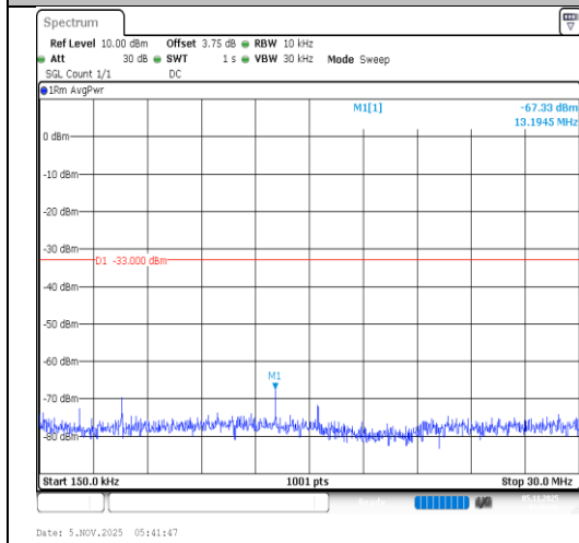
Band4-20MHz-QPSK-20050-100RB#0-0.15~30-PASS
