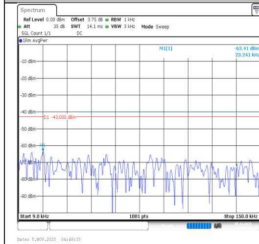
Band4-15MHz-64QAM-20175-1RB#0- 0.009~0.15-PASS
