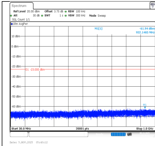
Band4-20MHz-QPSK-20050-1RB#99-30~1000-PASS
