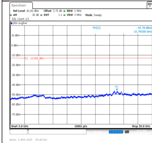
Band4-20MHz-QPSK-20050-1RB#99-3000~20000-PASS
