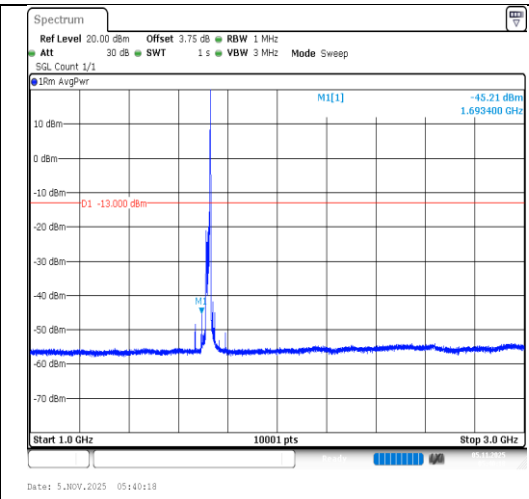
Band4-20MHz-QPSK-20050-1RB#99-1000~3000-PASS
