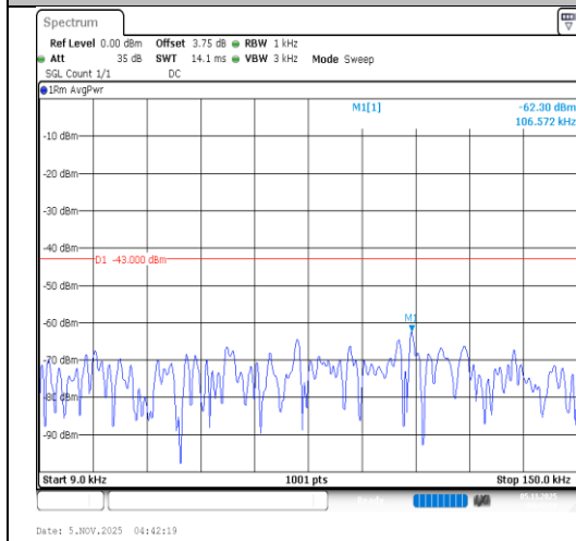
Band4-15MHz-QPSK-20025-1RB#0-0.009~0.15- PASS
