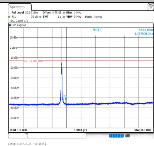
Band4-15MHz-64QAM-20175-1RB#0- 1000~3000-PASS
