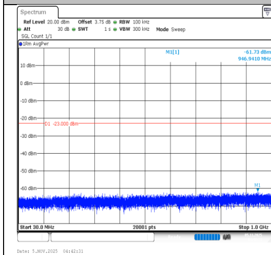
Band4-15MHz-QPSK-20025-1RB#0-30~1000- PASS
