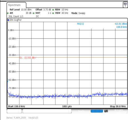
Band4-15MHz-QPSK-20025-1RB#0-0.15~30- PASS
