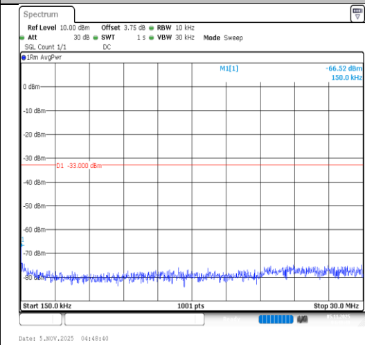
Band4-15MHz-64QAM-20175-1RB#0-0.15~30- PASS
