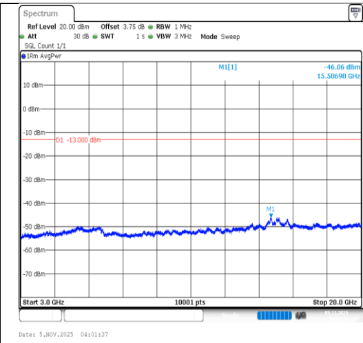
Band4-10MHz-16QAM-20350-50RB#0- 3000~20000-PASS
