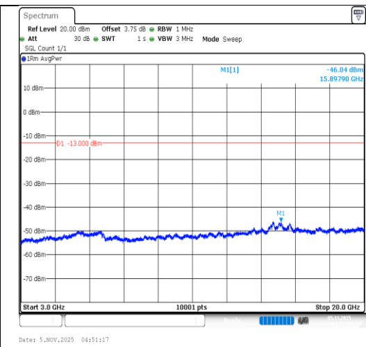
Band4-15MHz-QPSK-20175-75RB#0- 3000~20000-PASS
