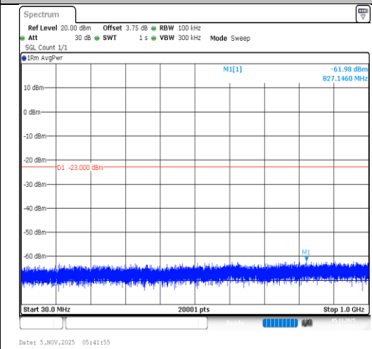
Band4-20MHz-QPSK-20050-100RB#0-30~1000-PASS
