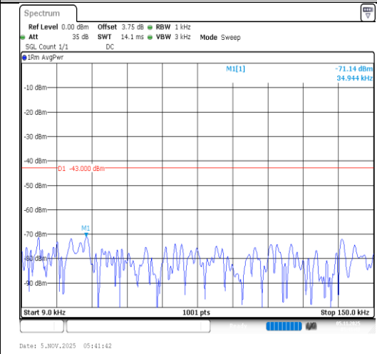
Band4-20MHz-QPSK-20050-100RB#0-0.009~0.15-PASS
