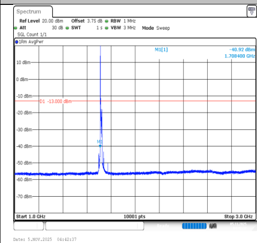
Band4-15MHz-QPSK-20025-1RB#0-1000~3000- PASS
