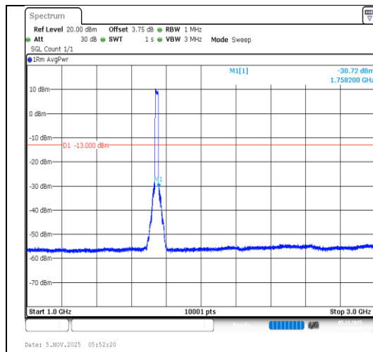
Band4-20MHz-QPSK-20300-100RB#0- 1000~3000-PASS
