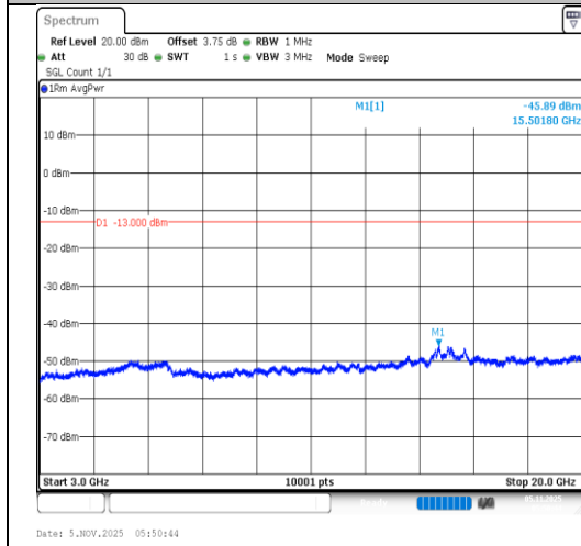
Band4-20MHz-QPSK-20300-1RB#99-3000~20000-PASS
