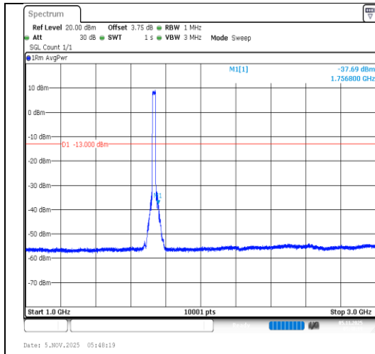
Band4-20MHz-64QAM-20175-100RB#0- 1000~3000-PASS
