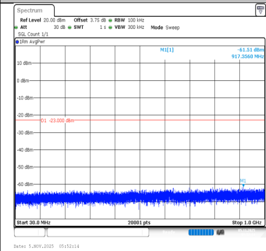
Band4-20MHz-QPSK-20300-100RB#0-30~1000-PASS
