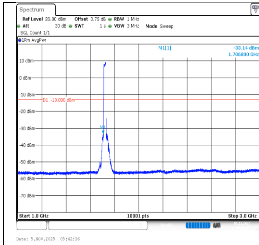
Band4-20MHz-16QAM-20050-100RB#0- 1000~3000-PASS
