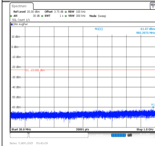
Band4-20MHz-QPSK-20175-1RB#0-30~1000- PASS
