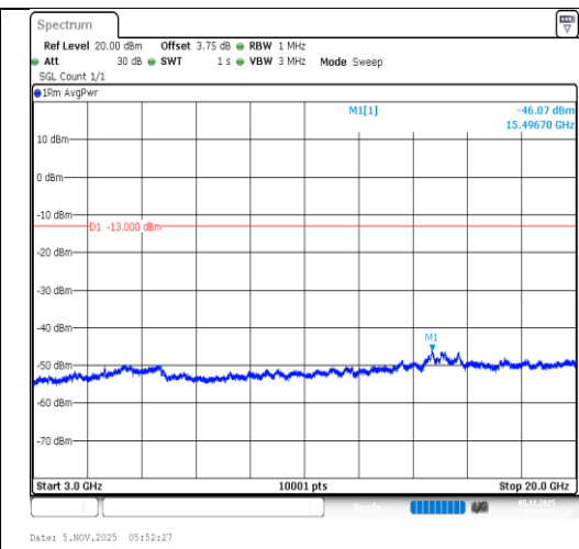
Band4-20MHz-QPSK-20300-100RB#0- 3000~20000-PASS
