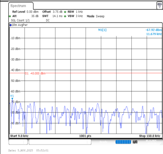
Band4-20MHz-QPSK-20300-100RB#0-0.009~0.15-PASS
