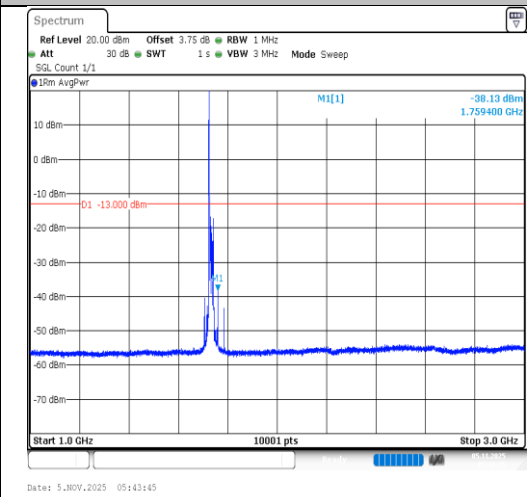
Band4-20MHz-QPSK-20175-1RB#0-1000~3000- PASS
