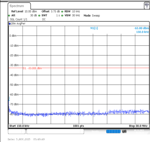
Band4-20MHz-64QAM-20300-1RB#0-0.15~30- PASS
