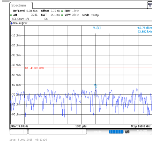
Band4-20MHz-QPSK-20175-1RB#0-0.009~0.15- PASS
