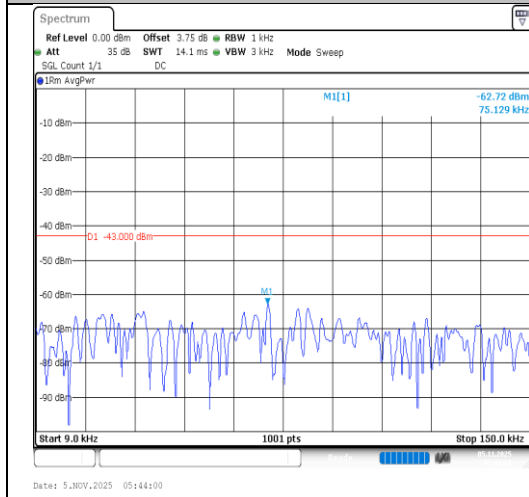
Band4-20MHz-16QAM-20175-1RB#0- 0.009~0.15-PASS
