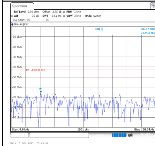
Band4-20MHz-64QAM-20300-1RB#0- 0.009~0.15-PASS
