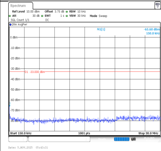
Band4-20MHz-QPSK-20175-1RB#0-0.15~30- PASS
