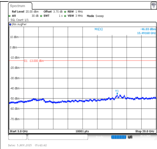
Band4-20MHz-16QAM-20050-100RB#0- 3000~20000-PASS
