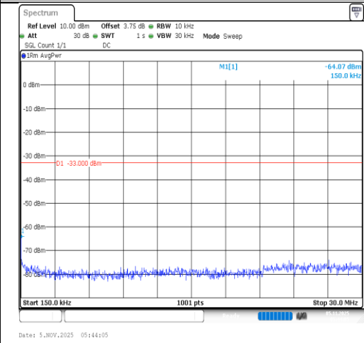
Band4-20MHz-16QAM-20175-1RB#0-0.15~30- PASS
