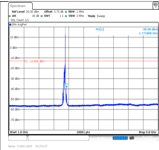
Band4-20MHz-QPSK-20300-1RB#99-1000~3000-PASS
