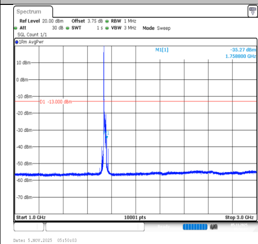
Band4-20MHz-64QAM-20300-1RB#0- 1000~3000-PASS
