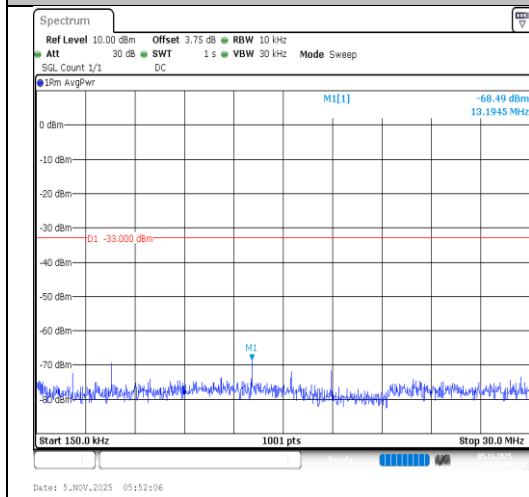
Band4-20MHz-QPSK-20300-100RB#0-0.15~30-PASS
