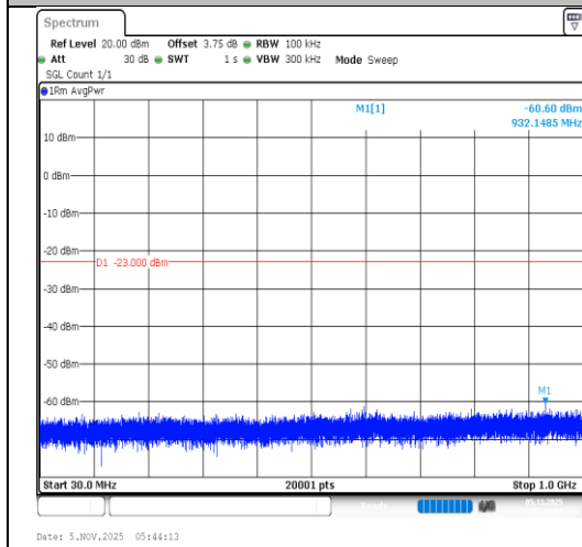
Band4-20MHz-16QAM-20175-1RB#0-30~1000- PASS
