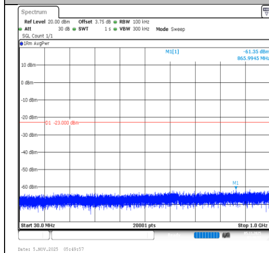
Band4-20MHz-64QAM-20300-1RB#0-30~1000- PASS
