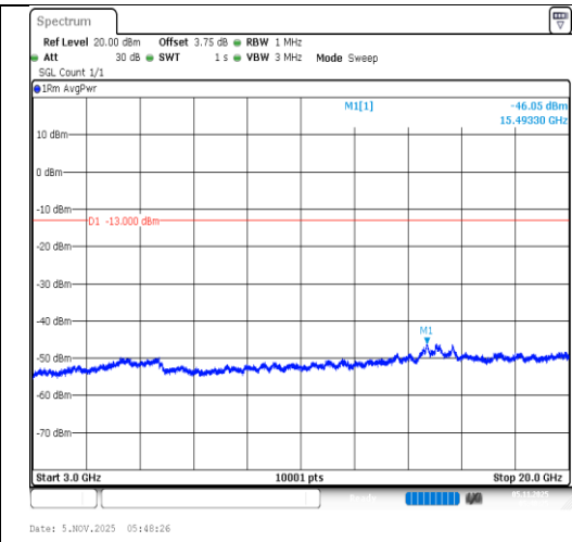
Band4-20MHz-64QAM-20175-100RB#0- 3000~20000-PASS
