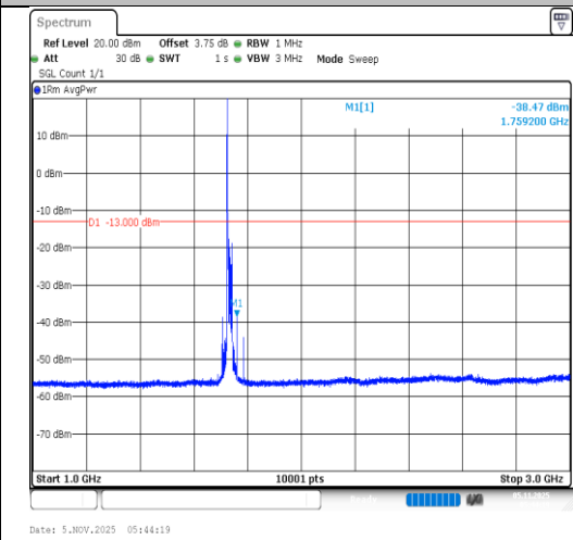
Band4-20MHz-16QAM-20175-1RB#0- 1000~3000-PASS
