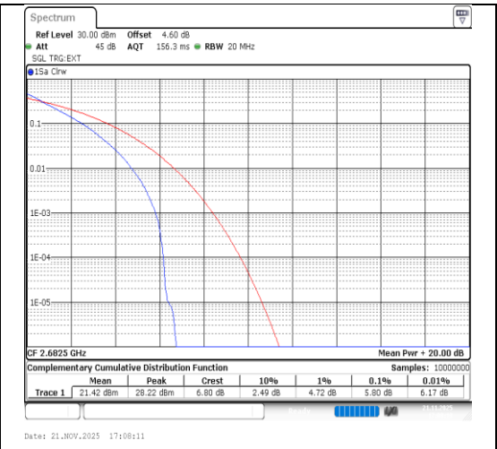
Band41-15MHz-QPSK-41515-75RB#0-PASS
