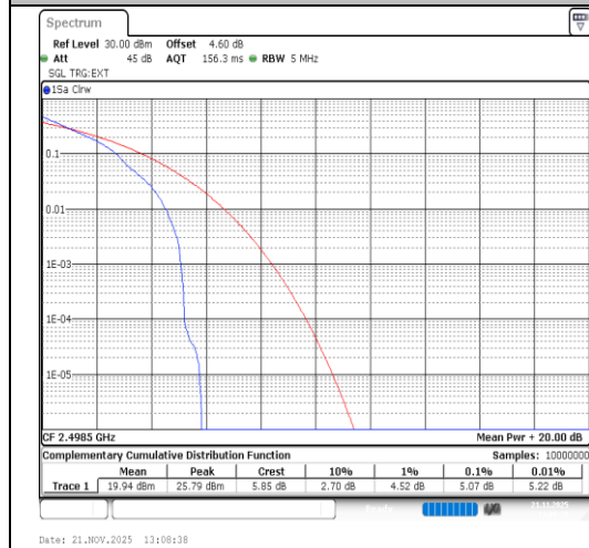
Band41-5MHz-64QAM-39675-1RB#0-PASS
