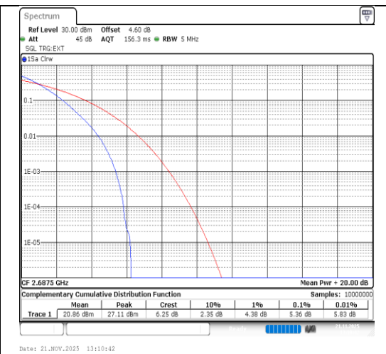
Band41-5MHz-QPSK-41565-25RB#0-PASS
