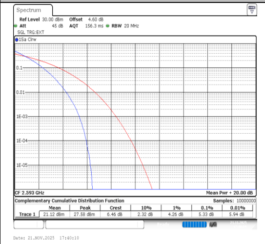
Band41-20MHz-64QAM-40620-100RB#0-PASS
