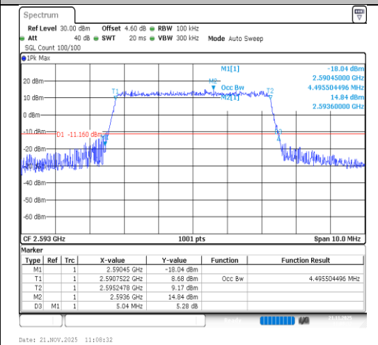
Band41-5MHz-16QAM-40620-25RB#0-PASS
