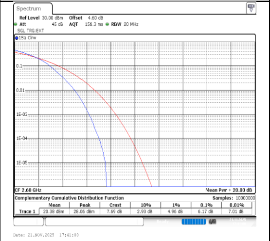
Band41-20MHz-16QAM-41490-100RB#0-PASS
