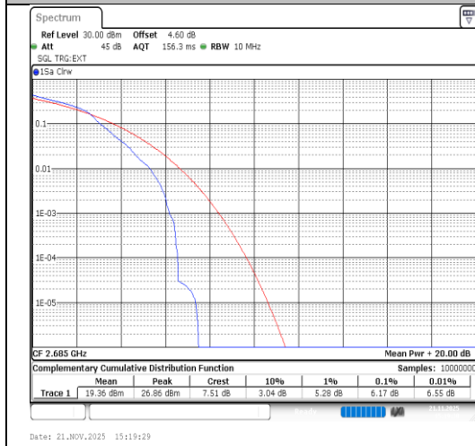
Band41-10MHz-16QAM-41540-1RB#0-PASS
