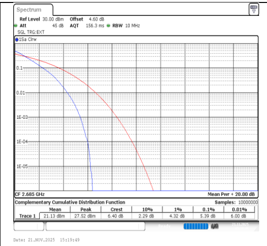
Band41-10MHz-QPSK-41540-50RB#0-PASS
