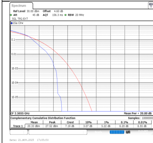
Band41-15MHz-16QAM-39725-1RB#0-PASS
