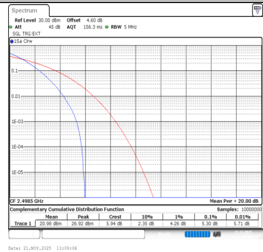
Band41-5MHz-64QAM-39675-25RB#0-PASS
