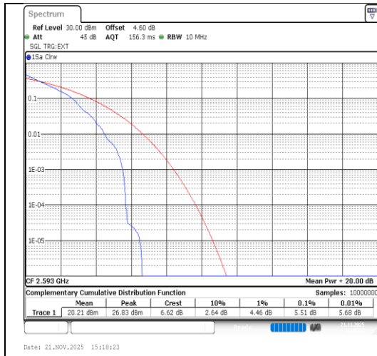
Band41-10MHz-QPSK-40620-1RB#0-PASS
