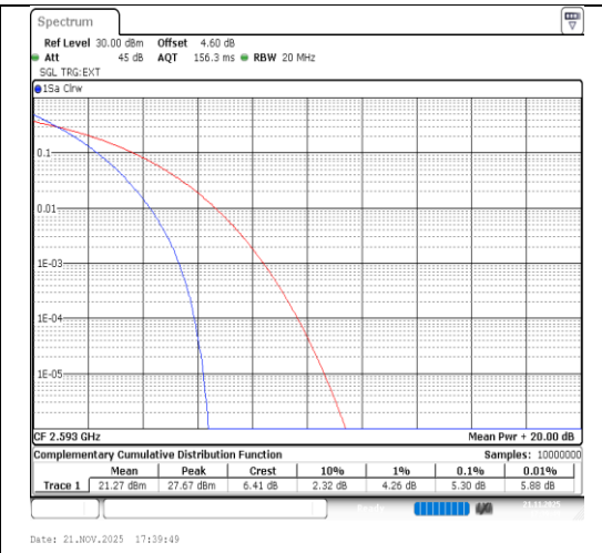
Band41-20MHz-QPSK-40620-100RB#0-PASS
