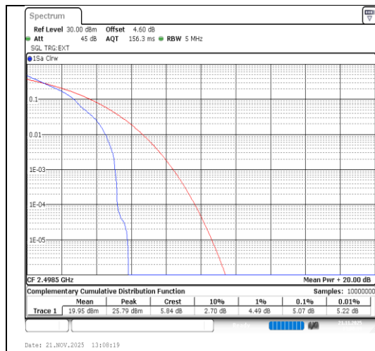
Band41-5MHz-QPSK-39675-1RB#0-PASS
