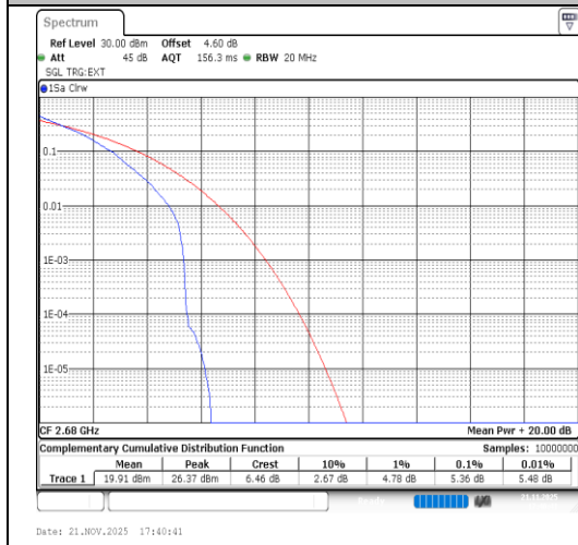
Band41-20MHz-64QAM-41490-1RB#0-PASS
