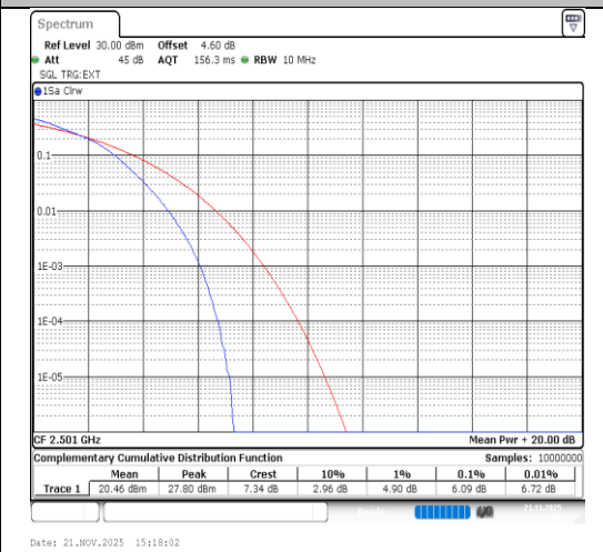
Band41-10MHz-16QAM-39700-50RB#0-PASS
