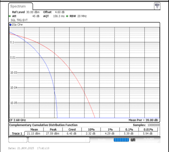
Band41-20MHz-64QAM-41490-100RB#0-PASS
