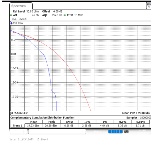
Band41-10MHz-64QAM-41540-1RB#0-PASS
