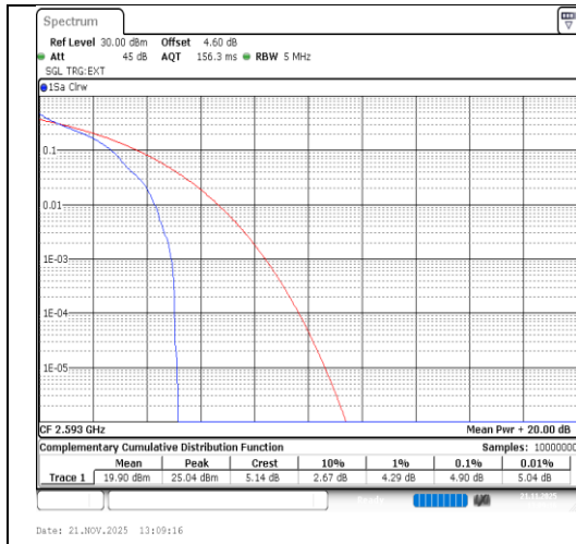
Band41-5MHz-QPSK-40620-1RB#0-PASS
