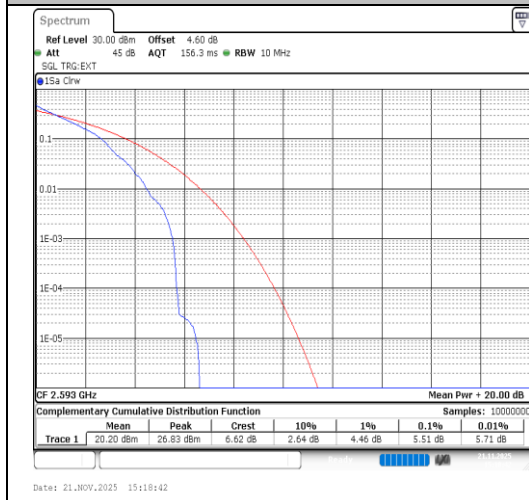
Band41-10MHz-64QAM-40620-1RB#0-PASS
