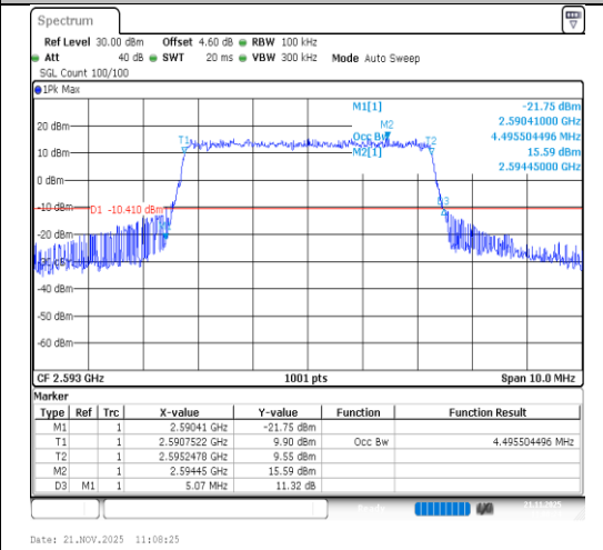
Band41-5MHz-QPSK-40620-25RB#0-PASS
