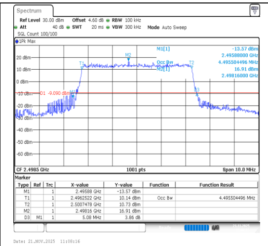
Band41-5MHz-64QAM-39675-25RB#0-PASS
