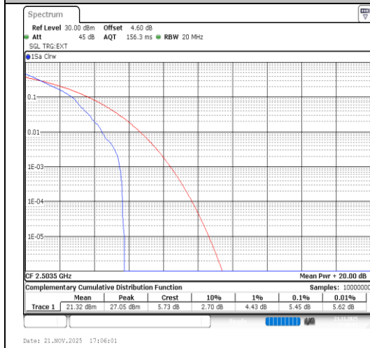
Band41-15MHz-64QAM-39725-1RB#0-PASS
