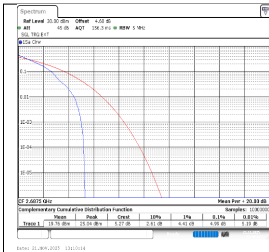
Band41-5MHz-QPSK-41565-1RB#0-PASS
