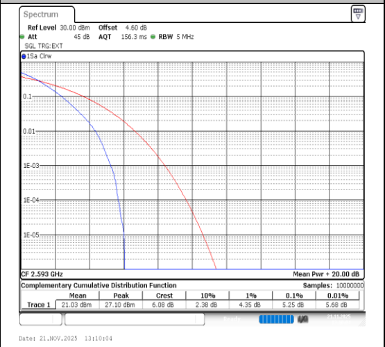
Band41-5MHz-64QAM-40620-25RB#0-PASS
