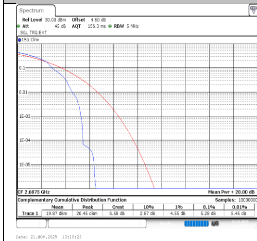
Band41-5MHz-16QAM-41565-1RB#0-PASS
