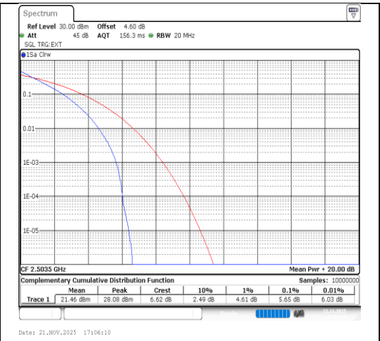
Band41-15MHz-QPSK-39725-75RB#0-PASS
