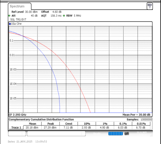
Band41-5MHz-16QAM-40620-25RB#0-PASS
