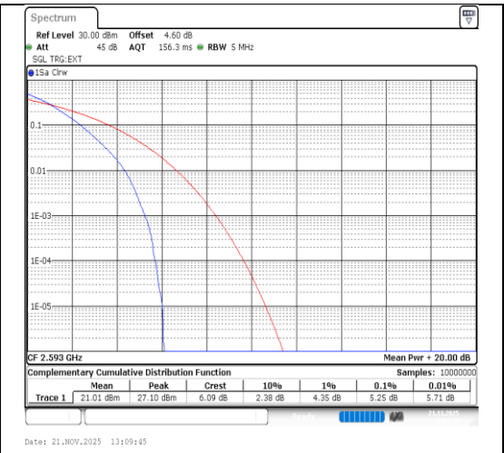
Band41-5MHz-QPSK-40620-25RB#0-PASS
