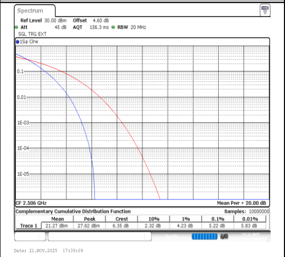
Band41-20MHz-64QAM-39750-100RB#0-PASS
