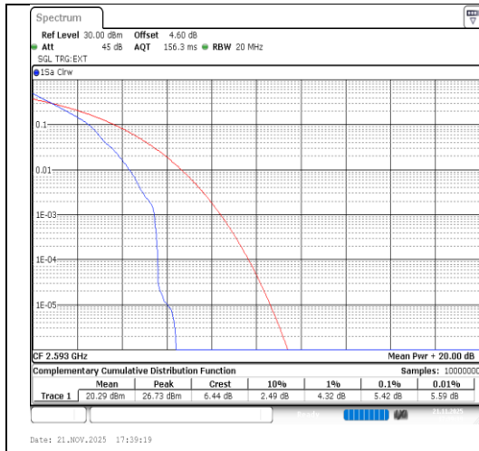
Band41-20MHz-QPSK-40620-1RB#0-PASS
