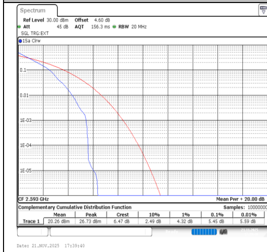
Band41-20MHz-64QAM-40620-1RB#0-PASS
