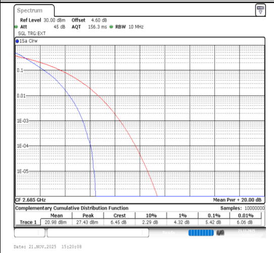
Band41-10MHz-64QAM-41540-50RB#0-PASS
