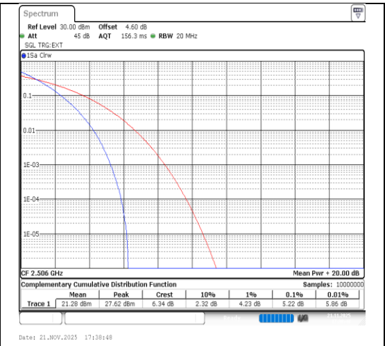
Band41-20MHz-QPSK-39750-100RB#0-PASS
