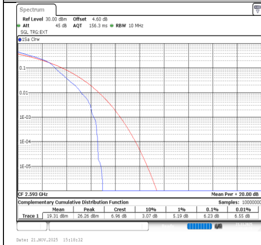
Band41-10MHz-16QAM-40620-1RB#0-PASS
