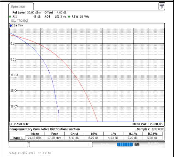
Band41-10MHz-64QAM-40620-50RB#0-PASS
