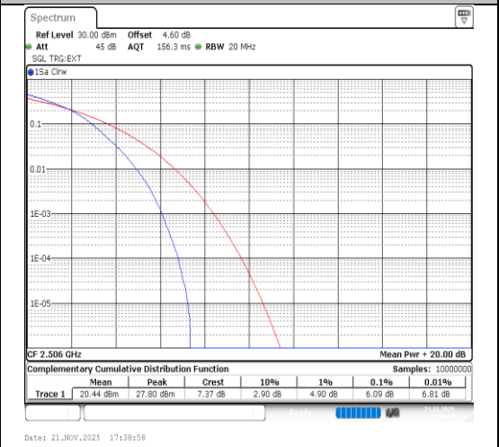
Band41-20MHz-16QAM-39750-100RB#0-PASS
