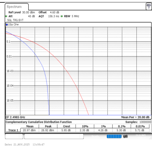
Band41-5MHz-QPSK-39675-25RB#0-PASS
