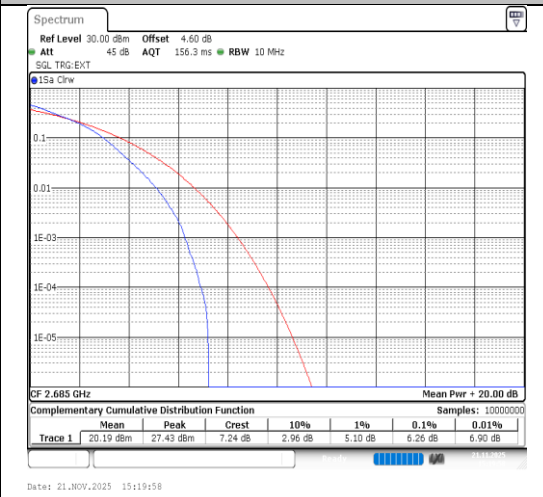
Band41-10MHz-16QAM-41540-50RB#0-PASS
