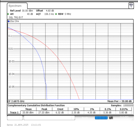
Band41-5MHz-64QAM-41565-25RB#0-PASS
