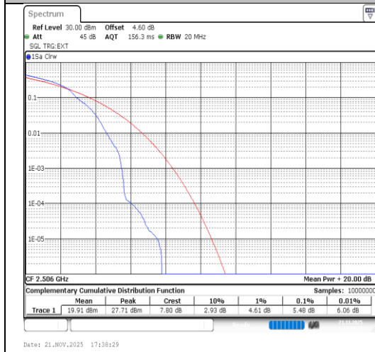
Band41-20MHz-16QAM-39750-1RB#0-PASS
