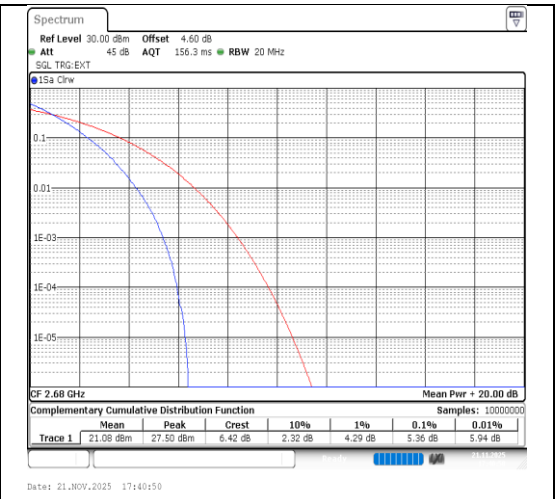
Band41-20MHz-QPSK-41490-100RB#0-PASS
