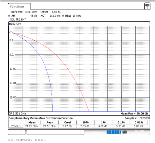
Band41-10MHz-64QAM-39700-50RB#0-PASS
