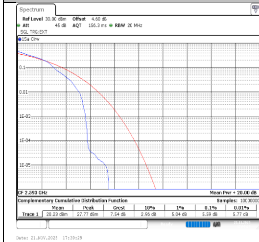
Band41-20MHz-16QAM-40620-1RB#0-PASS
