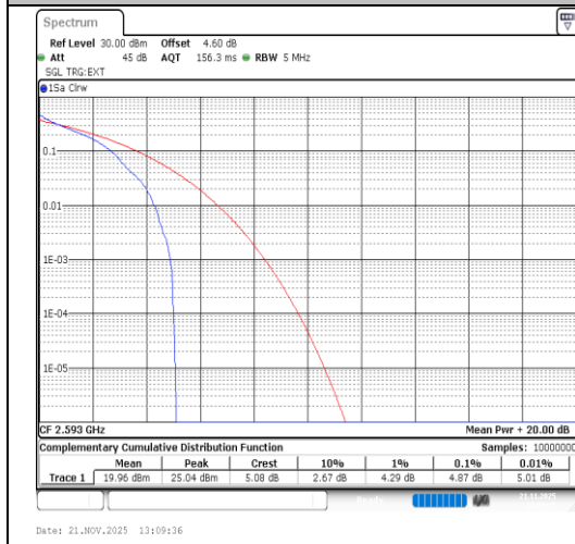
Band41-5MHz-64QAM-40620-1RB#0-PASS
