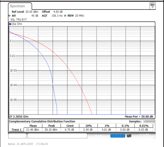
Band41-15MHz-64QAM-39725-75RB#0-PASS
