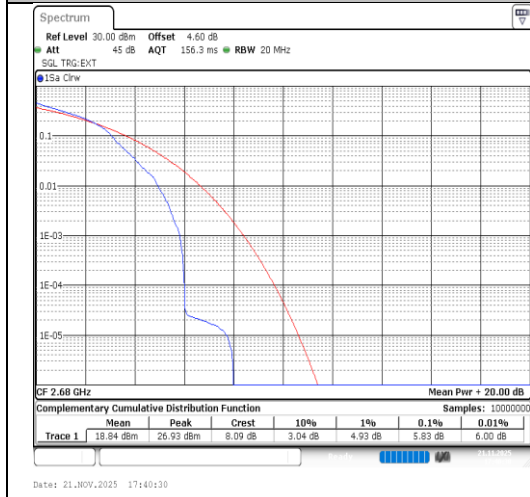
Band41-20MHz-16QAM-41490-1RB#0-PASS
