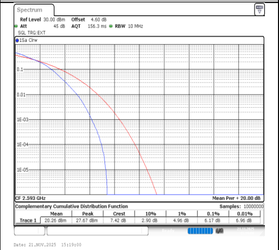
Band41-10MHz-16QAM-40620-50RB#0-PASS
