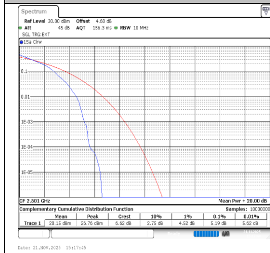
Band41-10MHz-64QAM-39700-1RB#0-PASS
