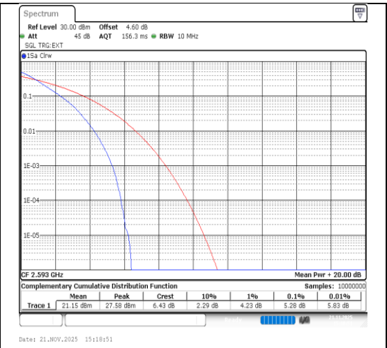
Band41-10MHz-QPSK-40620-50RB#0-PASS
