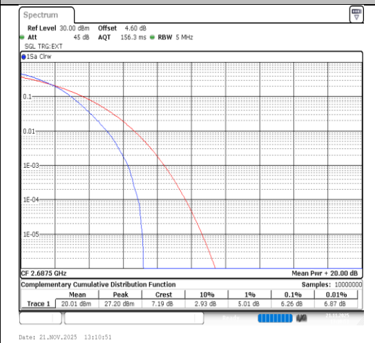
Band41-5MHz-16QAM-41565-25RB#0-PASS
