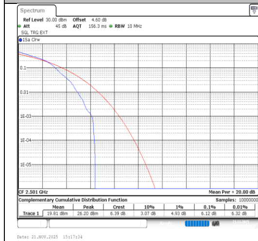
Band41-10MHz-16QAM-39700-1RB#0-PASS
