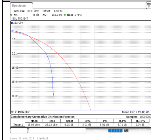
Band41-5MHz-16QAM-39675-1RB#0-PASS
