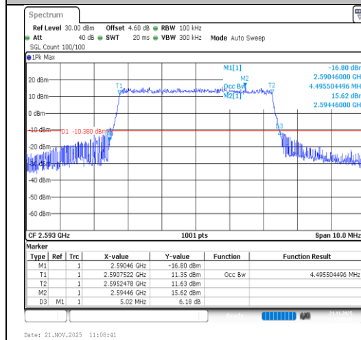
Band41-5MHz-64QAM-40620-25RB#0-PASS
