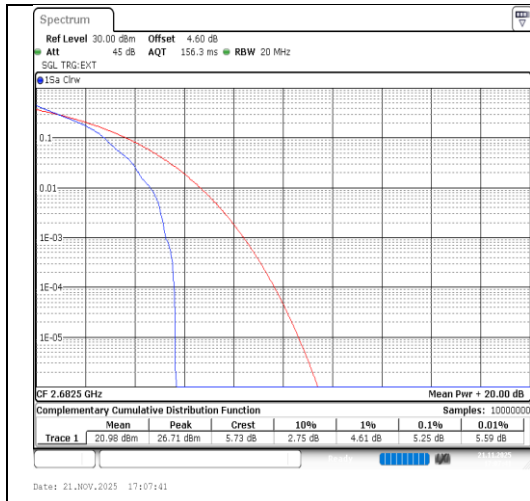
Band41-15MHz-QPSK-41515-1RB#0-PASS
