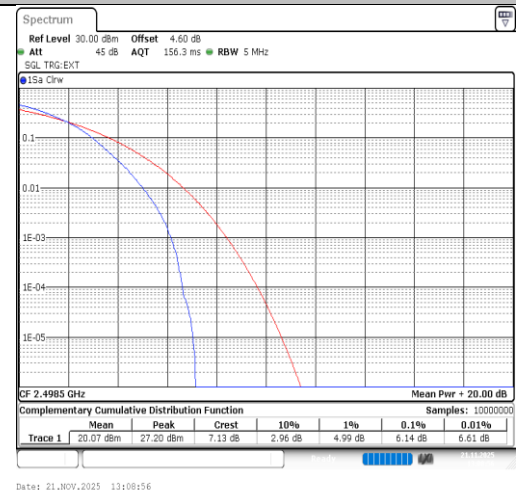
Band41-5MHz-16QAM-39675-25RB#0-PASS
