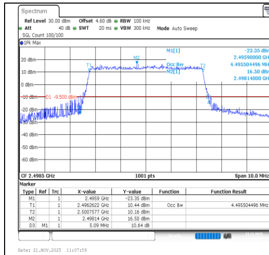
Band41-5MHz-QPSK-39675-25RB#0-PASS
