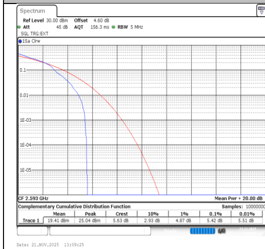
Band41-5MHz-16QAM-40620-1RB#0-PASS
