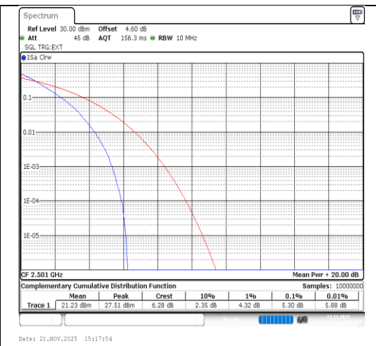
Band41-10MHz-QPSK-39700-50RB#0-PASS
