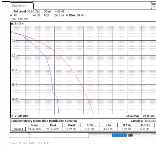
Band41-10MHz-QPSK-41540-1RB#0-PASS
