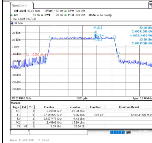
Band41-5MHz-16QAM-39675-25RB#0-PASS
