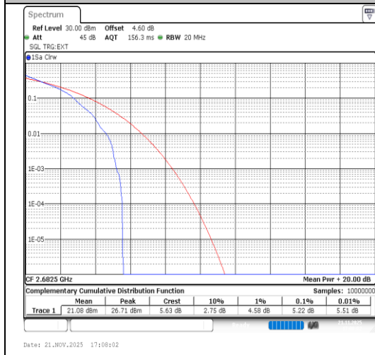
Band41-15MHz-64QAM-41515-1RB#0-PASS
