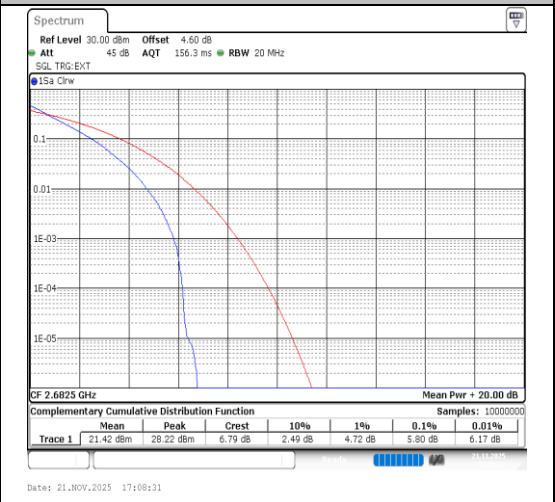
Band41-15MHz-64QAM-41515-75RB#0-PASS
