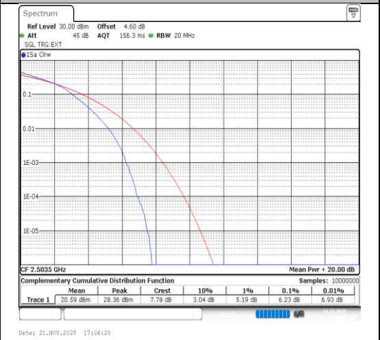
Band41-15MHz-16QAM-39725-75RB#0-PASS
