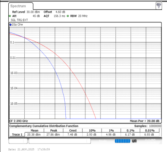
Band41-20MHz-16QAM-40620-100RB#0-PASS
