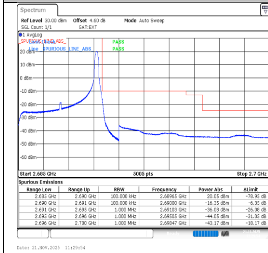
Band41-5MHz-16QAM-41565-1RB#24-PASS
