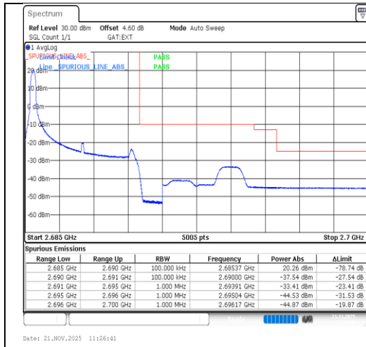
Band41-5MHz-64QAM-41565-1RB#0-PASS
