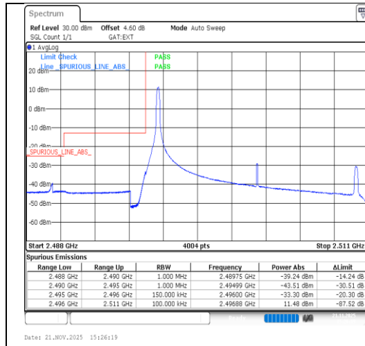
Band41-15MHz-QPSK-39725-1RB#0-PASS
