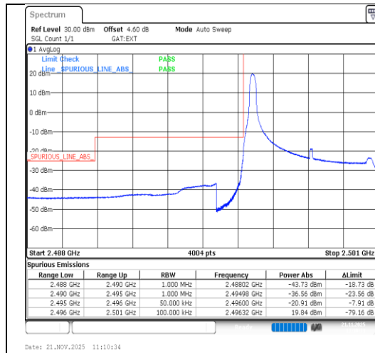
Band41-5MHz-QPSK-39675-1RB#0-PASS
