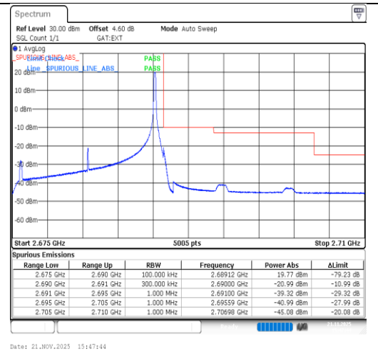
Band41-15MHz-64QAM-41515-1RB#74-PASS
