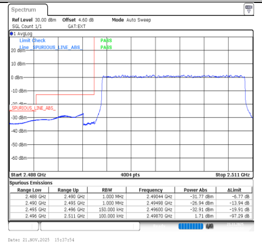
Band41-15MHz-64QAM-39725-75RB#0-PASS
