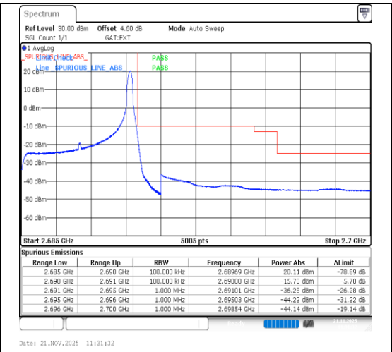
Band41-5MHz-64QAM-41565-1RB#24-PASS
