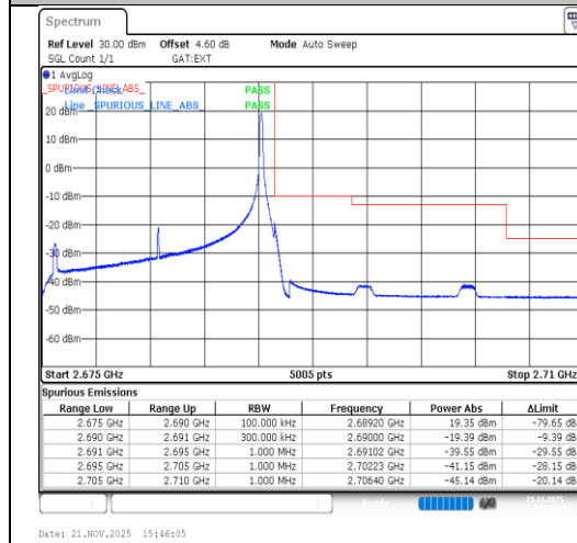
Band41-15MHz-16QAM-41515-1RB#74-PASS
