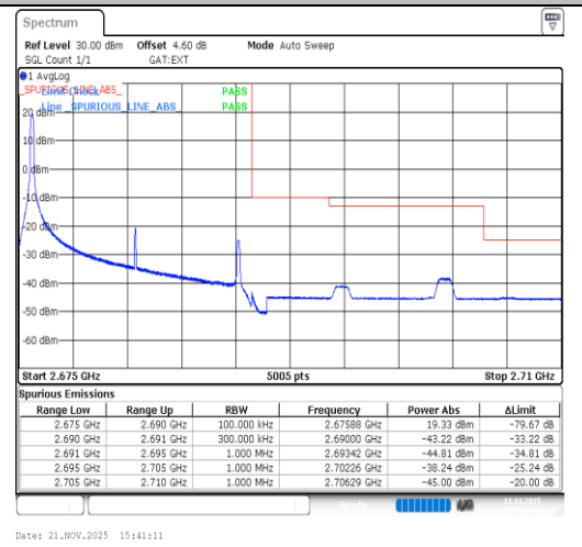
Band41-15MHz-16QAM-41515-1RB#0-PASS
