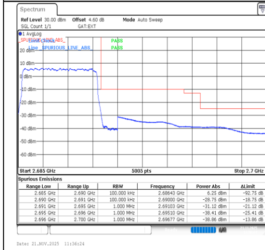
Band41-5MHz-64QAM-41565-25RB#0-PASS
