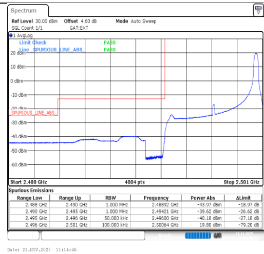
Band41-5MHz-QPSK-39675-1RB#24-PASS
