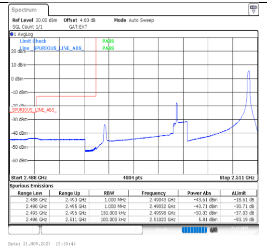
Band41-15MHz-QPSK-39725-1RB#74-PASS
