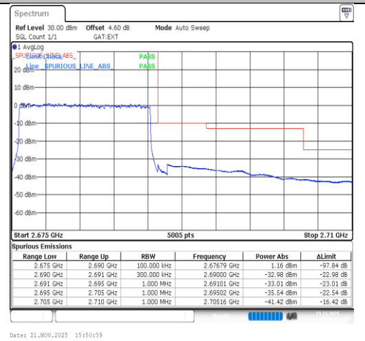
Band41-15MHz-16QAM-41515-75RB#0-PASS
