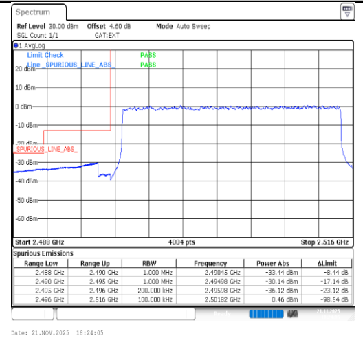
Band41-20MHz-64QAM-39750-100RB#0-PASS
