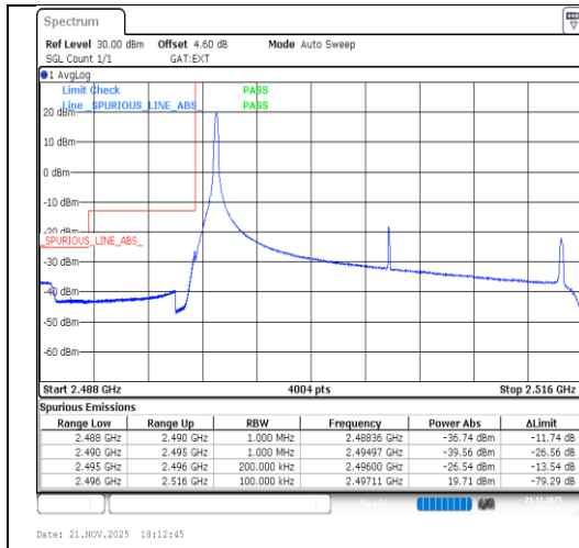
Band41-20MHz-QPSK-39750-1RB#0-PASS
