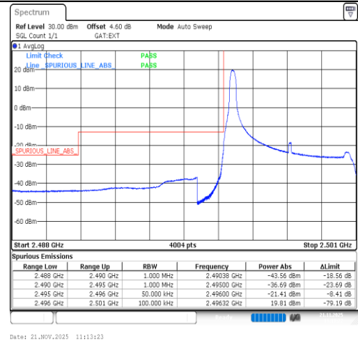
Band41-5MHz-64QAM-39675-1RB#0-PASS
