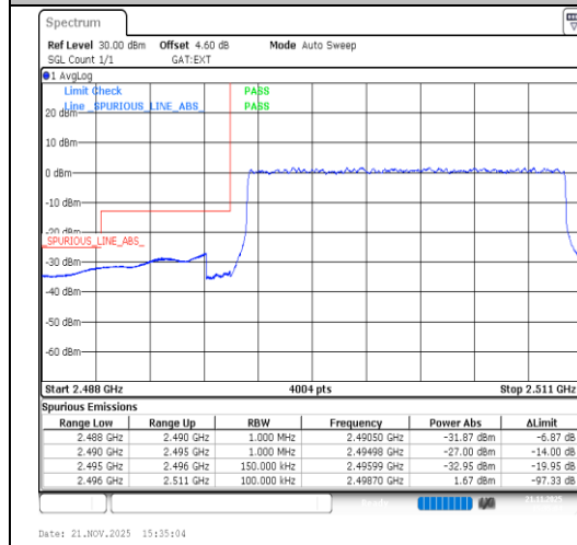
Band41-15MHz-QPSK-39725-75RB#0-PASS
