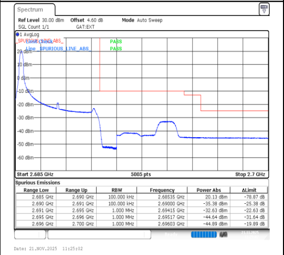
Band41-5MHz-16QAM-41565-1RB#0-PASS
