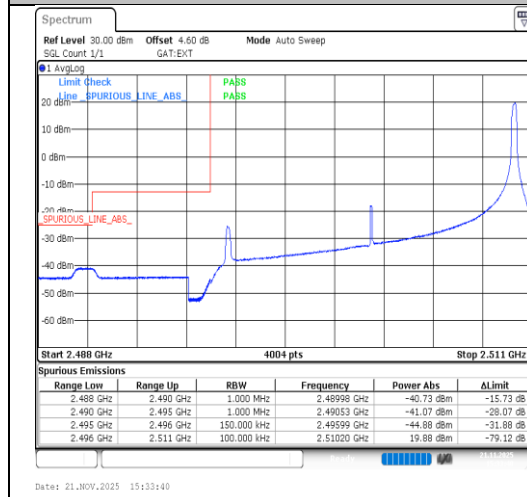
Band41-15MHz-64QAM-39725-1RB#74-PASS
