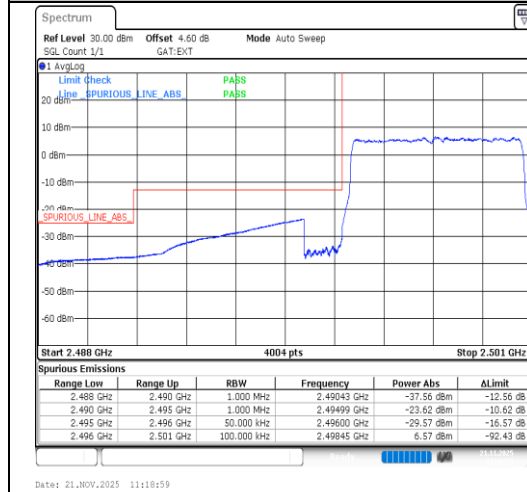
Band41-5MHz-QPSK-39675-25RB#0-PASS
