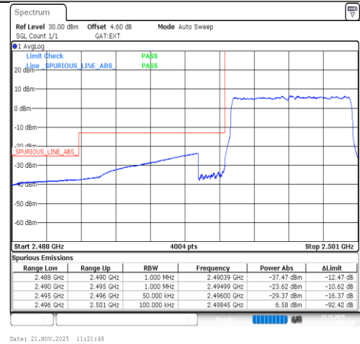
Band41-5MHz-64QAM-39675-25RB#0-PASS
