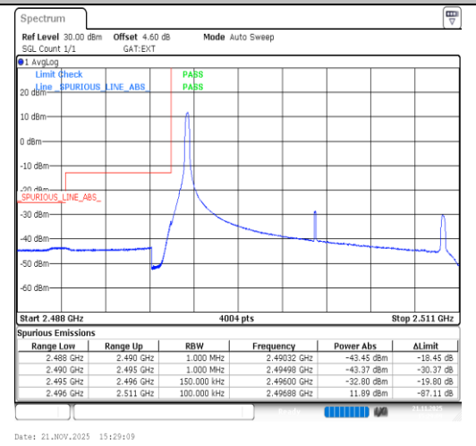
Band41-15MHz-64QAM-39725-1RB#0-PASS
