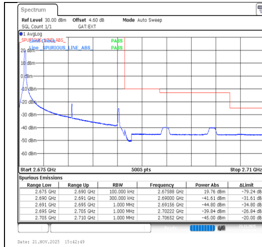
Band41-15MHz-64QAM-41515-1RB#0-PASS
