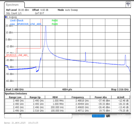
Band41-20MHz-64QAM-39750-1RB#0-PASS
