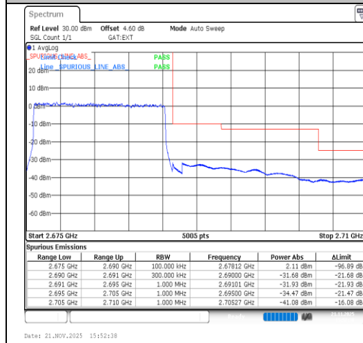
Band41-15MHz-64QAM-41515-75RB#0-PASS
