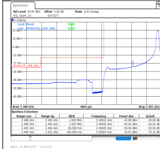
Band41-5MHz-64QAM-39675-1RB#24-PASS
