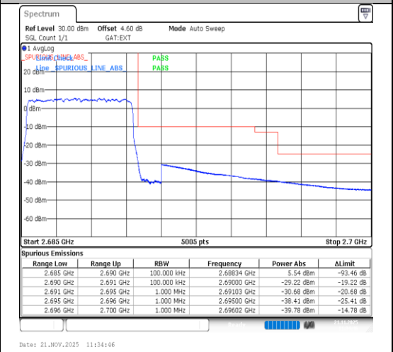
Band41-5MHz-16QAM-41565-25RB#0-PASS
