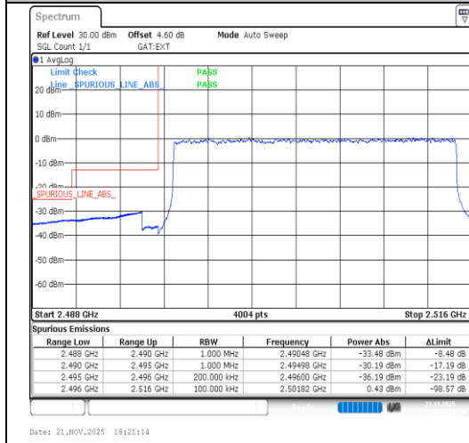
Band41-20MHz-QPSK-39750-100RB#0-PASS
