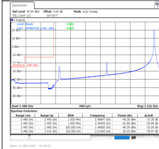
Band41-20MHz-64QAM-39750-1RB#99-PASS
