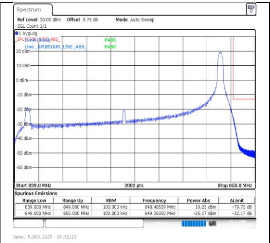
Band5-10MHz-64QAM-20600-1RB#49-PASS
