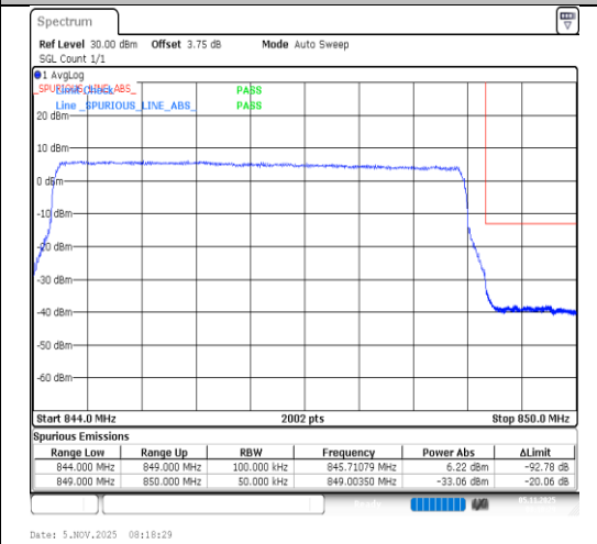
Band5-5MHz-QPSK-20625-25RB#0-PASS
