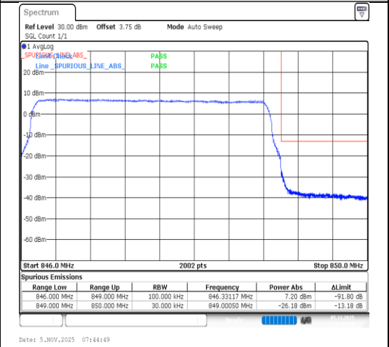
Band5-3MHz-16QAM-20635-15RB#0-PASS
