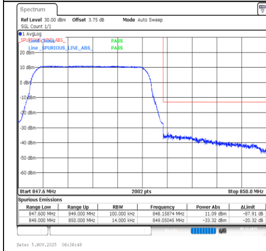
Band5-1.4MHz-64QAM-20643-6RB#0-PASS
