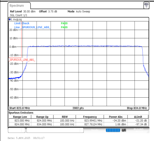
Band5-10MHz-64QAM-20450-50RB#0-PASS
