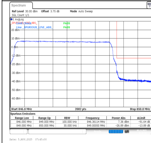
Band5-3MHz-64QAM-20635-15RB#0-PASS
