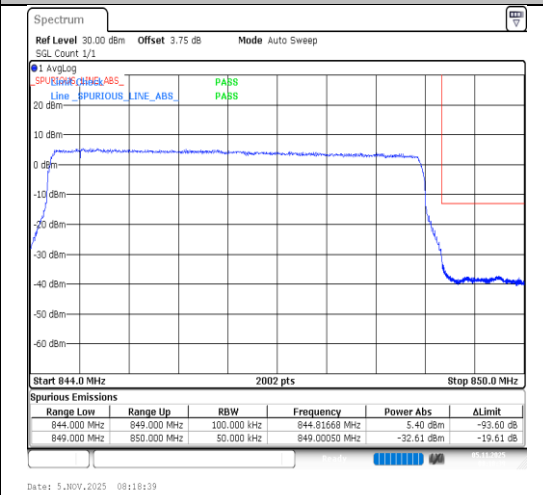
Band5-5MHz-16QAM-20625-25RB#0-PASS
