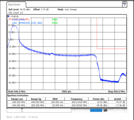
Band5-3MHz-16QAM-20635-1RB#0-PASS
