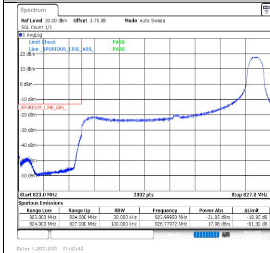
Band5-3MHz-64QAM-20415-1RB#14-PASS
