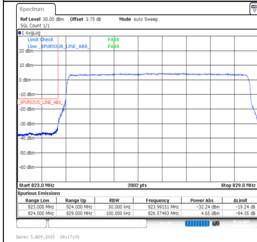
Band5-5MHz-16QAM-20425-25RB#0-PASS
