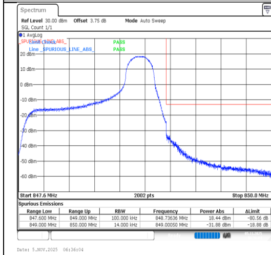
Band5-1.4MHz-16QAM-20643-1RB#5-PASS
