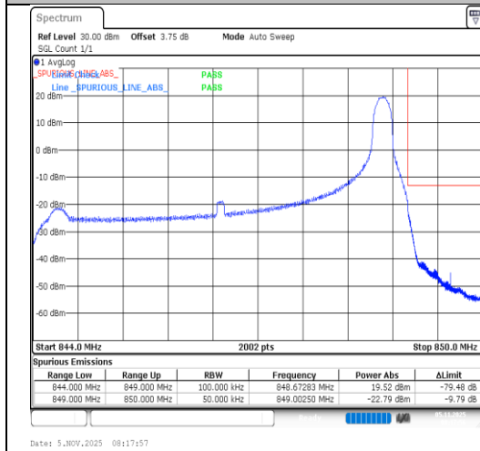
Band5-5MHz-QPSK-20625-1RB#24-PASS
