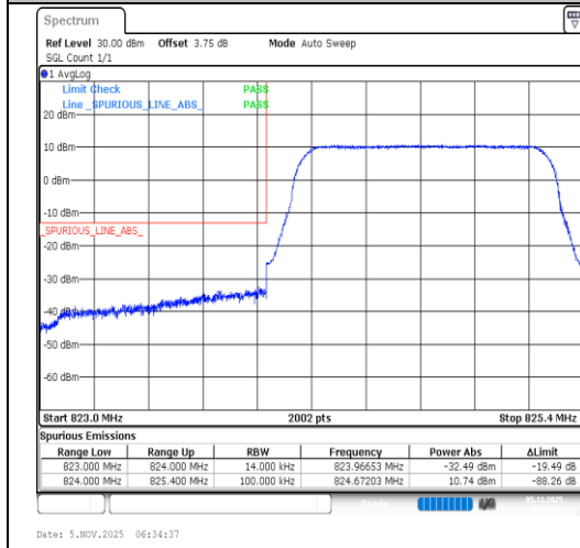
Band5-1.4MHz-16QAM-20407-6RB#0-PASS
