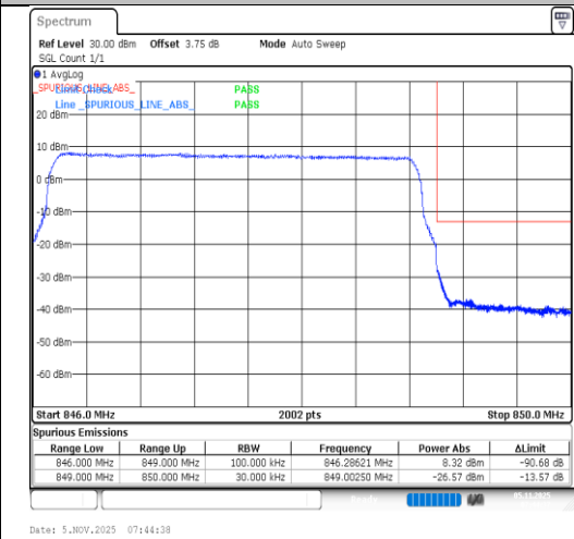
Band5-3MHz-QPSK-20635-15RB#0-PASS
