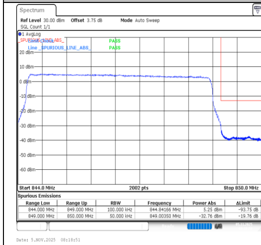
Band5-5MHz-64QAM-20625-25RB#0-PASS
