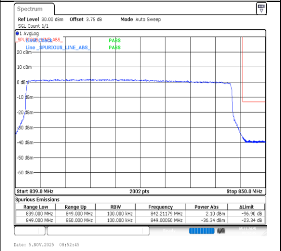
Band5-10MHz-16QAM-20600-50RB#0-PASS
