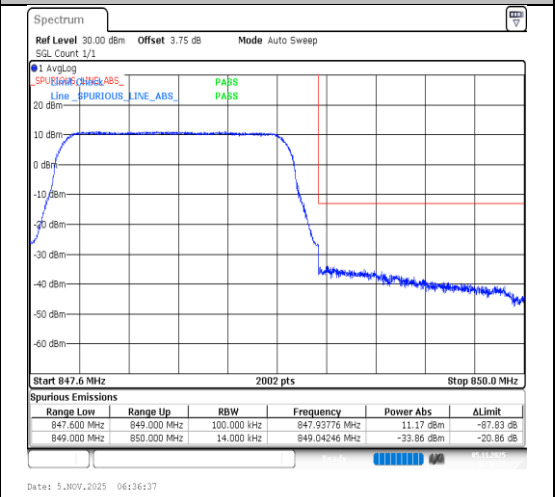
Band5-1.4MHz-16QAM-20643-6RB#0-PASS
