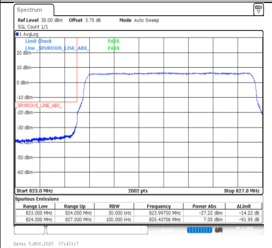
Band5-3MHz-64QAM-20415-15RB#0-PASS
