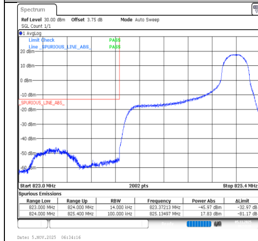
Band5-1.4MHz-64QAM-20407-1RB#5-PASS
