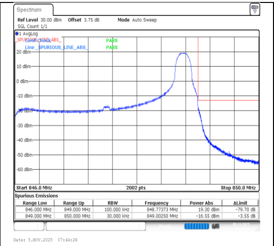
Band5-3MHz-64QAM-20635-1RB#14-PASS
