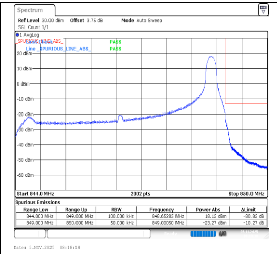
Band5-5MHz-64QAM-20625-1RB#24-PASS
