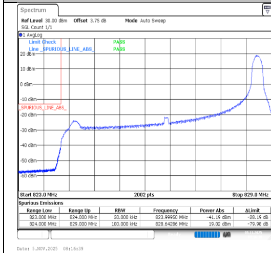
Band5-5MHz-64QAM-20425-1RB#24-PASS
