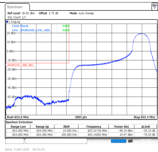
Band5-1.4MHz-QPSK-20407-1RB#5-PASS
