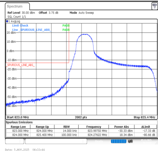
Band5-1.4MHz-64QAM-20407-1RB#0-PASS
