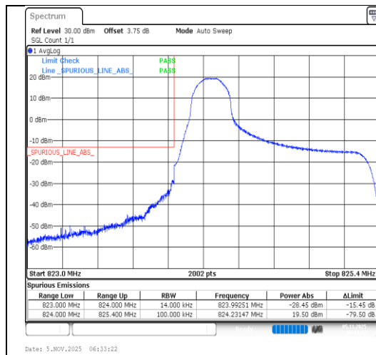
Band5-1.4MHz-QPSK-20407-1RB#0-PASS
