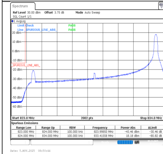
Band5-10MHz-64QAM-20450-1RB#49-PASS
