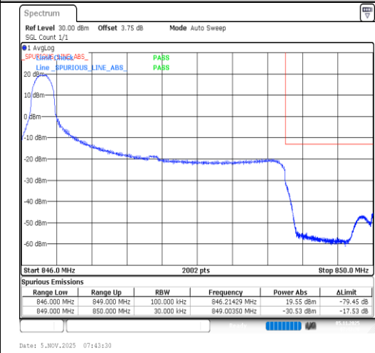
Band5-3MHz-QPSK-20635-1RB#0-PASS
