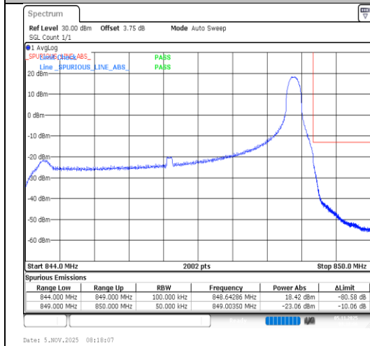
Band5-5MHz-16QAM-20625-1RB#24-PASS
