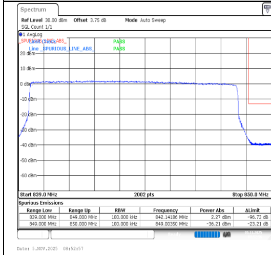
Band5-10MHz-64QAM-20600-50RB#0-PASS
