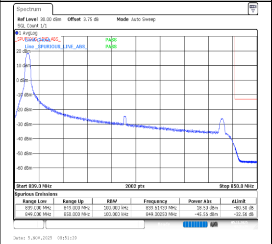
Band5-10MHz-16QAM-20600-1RB#0-PASS
