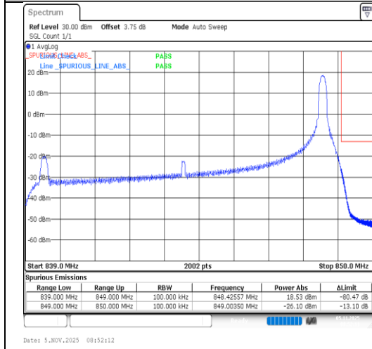
Band5-10MHz-16QAM-20600-1RB#49-PASS
