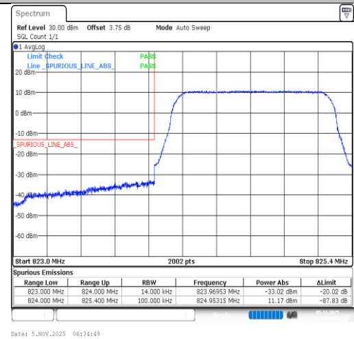
Band5-1.4MHz-64QAM-20407-6RB#0-PASS
