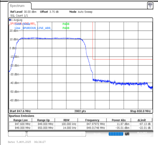
Band5-1.4MHz-QPSK-20643-6RB#0-PASS
