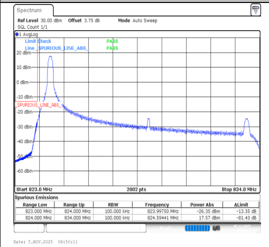
Band5-10MHz-64QAM-20450-1RB#0-PASS
