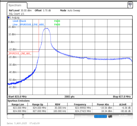
Band5-3MHz-64QAM-20415-1RB#0-PASS
