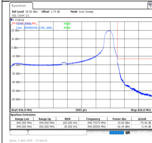
Band5-3MHz-QPSK-20635-1RB#14-PASS
