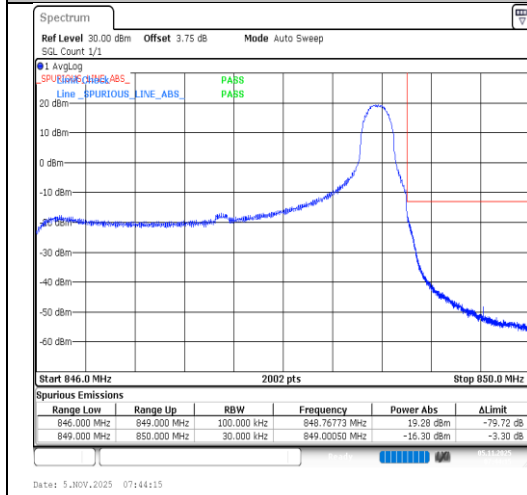
Band5-3MHz-16QAM-20635-1RB#14-PASS
