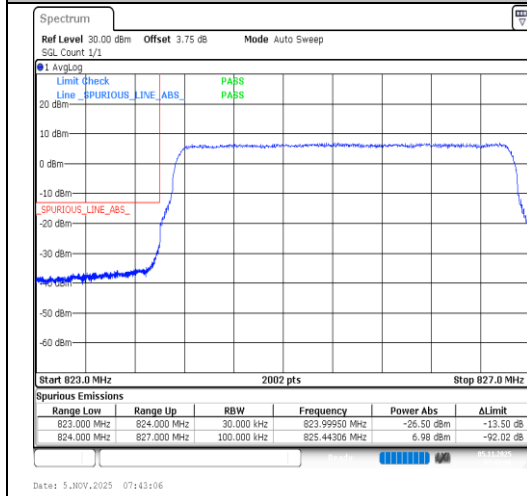
Band5-3MHz-16QAM-20415-15RB#0-PASS
