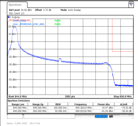
Band5-5MHz-QPSK-20625-1RB#0-PASS
