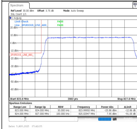
Band5-3MHz-QPSK-20415-15RB#0-PASS
