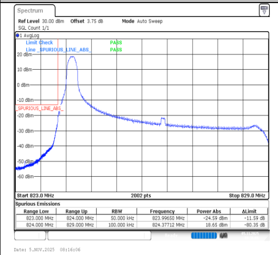
Band5-5MHz-64QAM-20425-1RB#0-PASS
