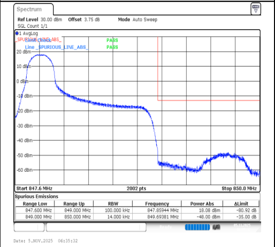
Band5-1.4MHz-16QAM-20643-1RB#0-PASS
