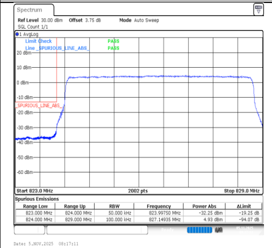
Band5-5MHz-64QAM-20425-25RB#0-PASS
