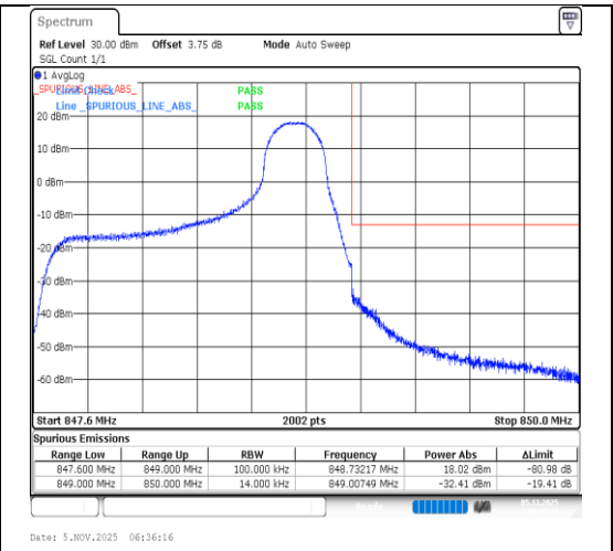
Band5-1.4MHz-64QAM-20643-1RB#5-PASS
