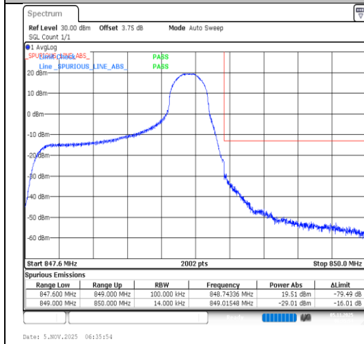
Band5-1.4MHz-QPSK-20643-1RB#5-PASS
