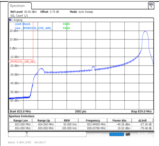
Band5-5MHz-QPSK-20425-1RB#24-PASS
