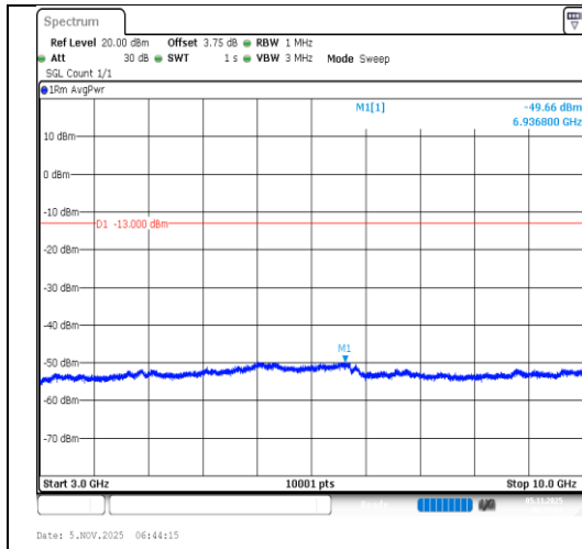
Band5-1.4MHz-64QAM-20525-1RB#0- 3000~10000-PASS
