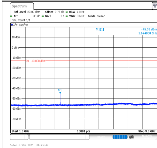
Band5-1.4MHz-64QAM-20525-1RB#5- 1000~3000-PASS
