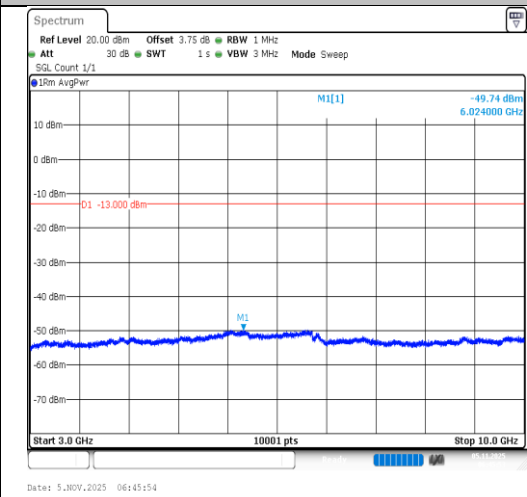
Band5-1.4MHz-64QAM-20525-1RB#5- 3000~10000-PASS
