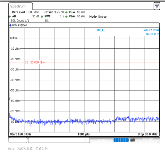
Band5-3MHz-QPSK-20525-1RB#0-0.15~30- PASS
