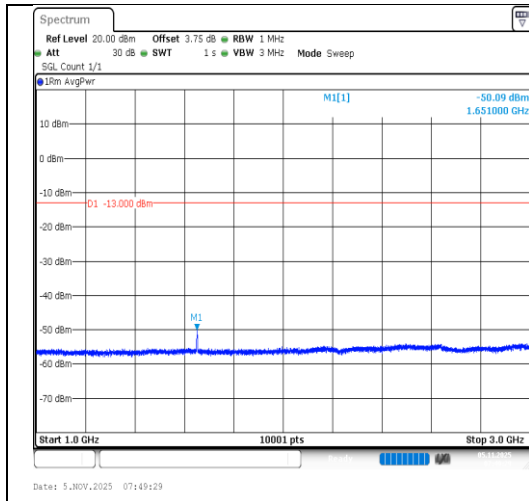
Band5-3MHz-16QAM-20415-15RB#0- 1000~3000-PASS
