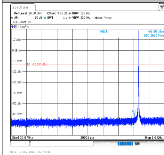
Band5-3MHz-QPSK-20525-1RB#0-30~1000- PASS
