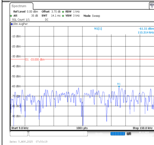
Band5-3MHz-QPSK-20525-1RB#0-0.009~0.15- PASS
