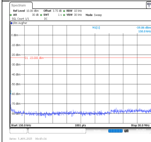
Band5-1.4MHz-64QAM-20525-1RB#5-0.15~30- PASS
