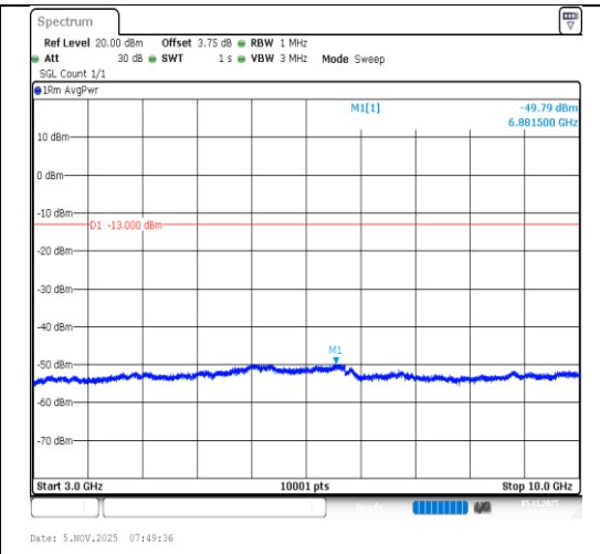
Band5-3MHz-16QAM-20415-15RB#0- 3000~10000-PASS
