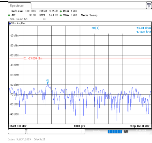
Band5-1.4MHz-64QAM-20525-1RB#5- 0.009~0.15-PASS
