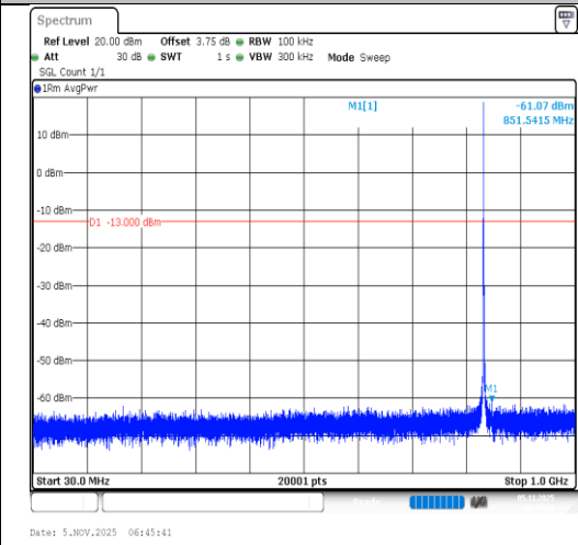
Band5-1.4MHz-64QAM-20525-1RB#5-30~1000- PASS
