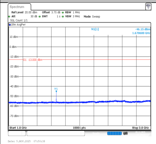
Band5-3MHz-QPSK-20525-1RB#0-1000~3000- PASS
