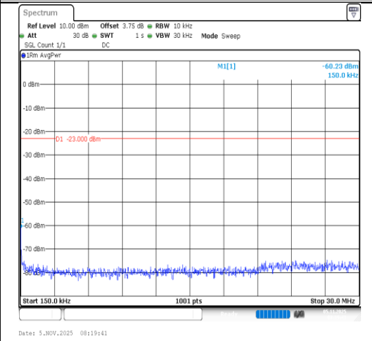
Band5-5MHz-16QAM-20425-1RB#0-0.15~30- PASS
