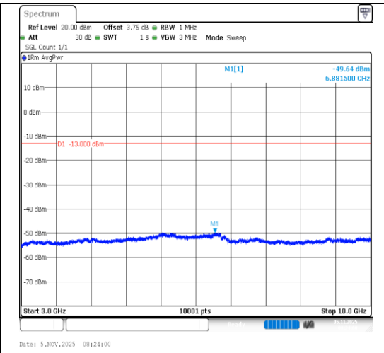
Band5-5MHz-64QAM-20425-25RB#0- 3000~10000-PASS
