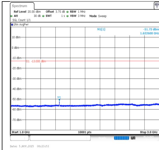
Band5-5MHz-64QAM-20425-25RB#0- 1000~3000-PASS
