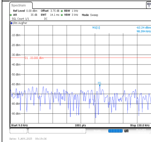
Band5-5MHz-16QAM-20425-1RB#0-0.009~0.15- PASS
