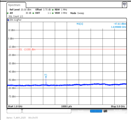
Band5-5MHz-16QAM-20425-1RB#0-1000~3000- PASS
