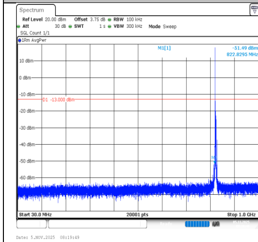
Band5-5MHz-16QAM-20425-1RB#0-30~1000- PASS
