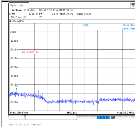
Band5-10MHz-64QAM-20525-50RB#0-0.15~30-PASS
