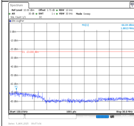
Band5-10MHz-16QAM-20450-50RB#0-0.15~30-PASS
