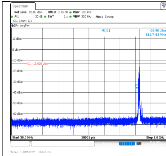
Band5-10MHz-16QAM-20450-1RB#49-30~1000-PASS
