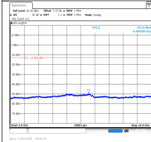
Band5-10MHz-64QAM-20525-1RB#49-3000~10000-PASS
