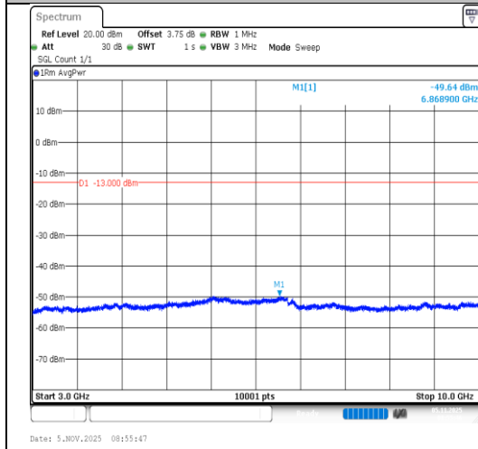
Band5-10MHz-16QAM-20450-1RB#49-3000~10000-PASS
