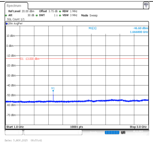
Band5-10MHz-16QAM-20450-1RB#49-1000~3000-PASS
