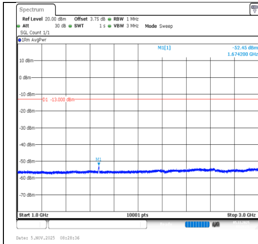
Band5-5MHz-16QAM-20525-25RB#0- 1000~3000-PASS
