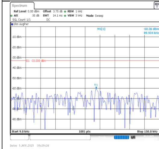
Band5-5MHz-QPSK-20625-1RB#0-0.009~0.15- PASS
