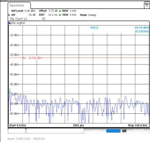
Band5-10MHz-64QAM-20525-50RB#0-0.009~0.15-PASS
