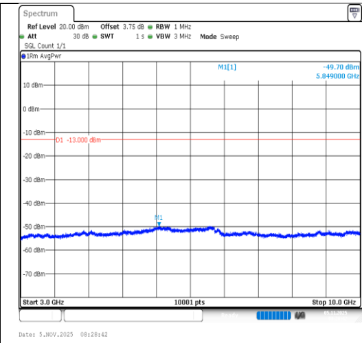
Band5-5MHz-16QAM-20525-25RB#0- 3000~10000-PASS
