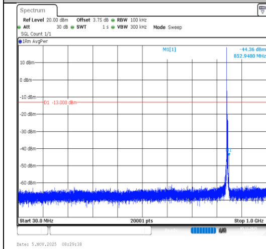
Band5-5MHz-QPSK-20625-1RB#0-30~1000- PASS
