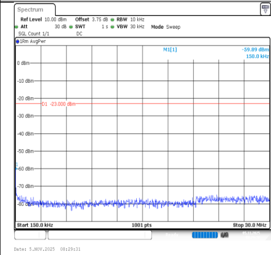
Band5-5MHz-QPSK-20625-1RB#0-0.15~30- PASS
