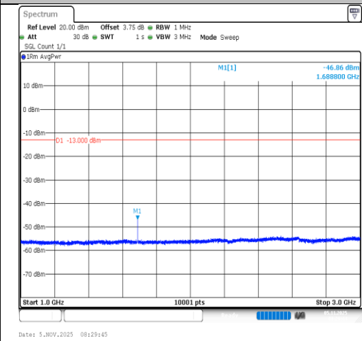
Band5-5MHz-QPSK-20625-1RB#0-1000~3000- PASS
