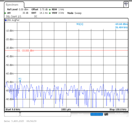
Band5-10MHz-16QAM-20450-50RB#0-0.009~0.15-PASS
