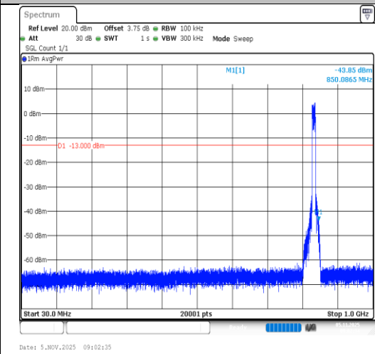
Band5-10MHz-64QAM-20525-50RB#0-30~1000-PASS
