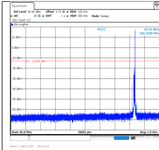
Band5-10MHz-64QAM-20525-1RB#49-30~1000-PASS
