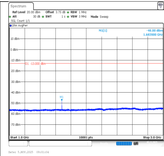
Band5-10MHz-64QAM-20525-1RB#49-1000~3000-PASS
