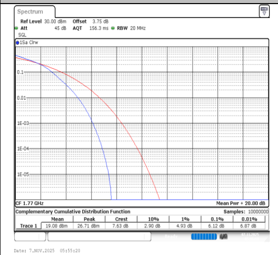
Band66-20MHz-64QAM-132572-100RB#0-PASS
