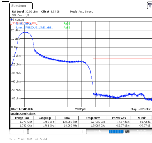
Band66-1.4MHz-64QAM-132665-1RB#0-PASS
