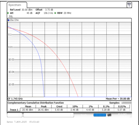
Band66-15MHz-QPSK-132322-75RB#0-PASS
