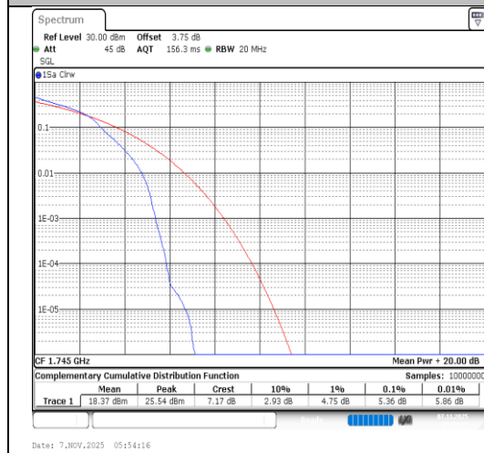
Band66-20MHz-16QAM-132322-1RB#0-PASS
