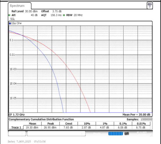
Band66-20MHz-16QAM-132072-100RB#0-PASS
