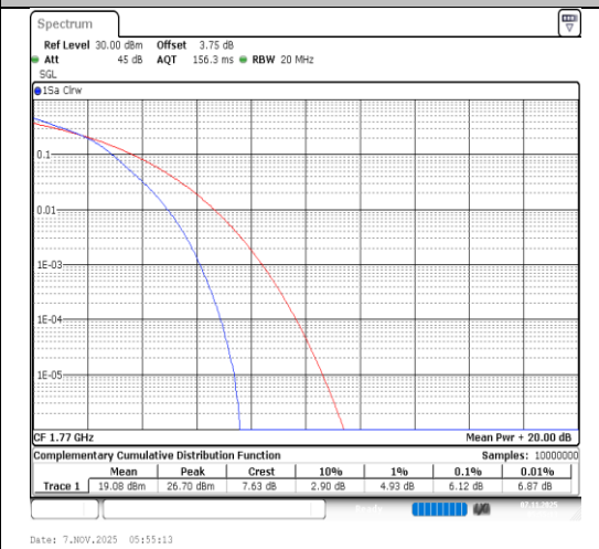
Band66-20MHz-16QAM-132572-100RB#0-PASS
