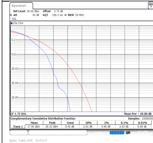
Band66-20MHz-16QAM-132072-1RB#0-PASS
