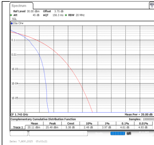
Band66-15MHz-QPSK-132322-1RB#0-PASS
