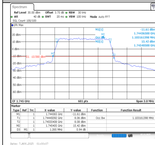
Band66-1.4MHz-64QAM-132322-6RB#0-PASS
