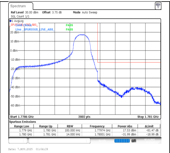
Band66-1.4MHz-64QAM-132665-1RB#5-PASS
