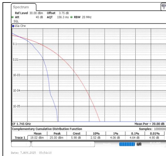
Band66-20MHz-QPSK-132322-1RB#0-PASS
