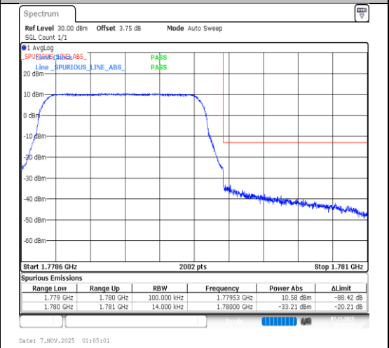
Band66-1.4MHz-16QAM-132665-6RB#0-PASS
