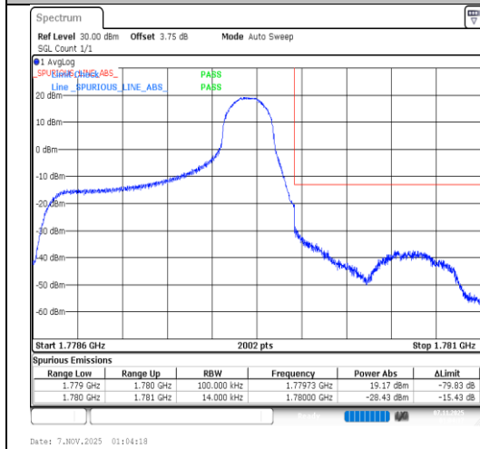
Band66-1.4MHz-QPSK-132665-1RB#5-PASS
