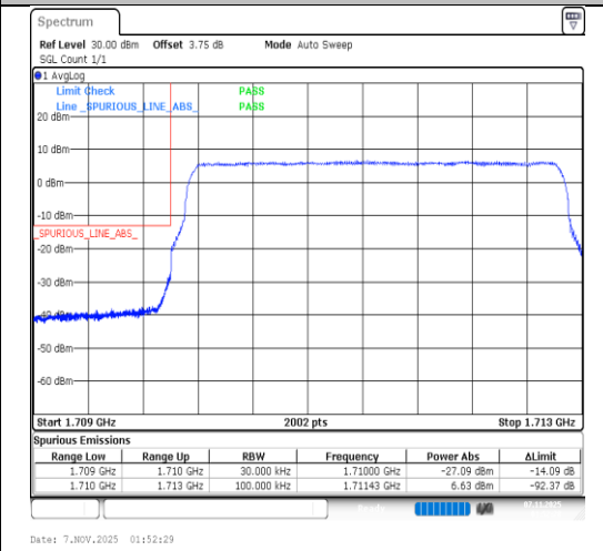
Band66-3MHz-64QAM-131987-15RB#0-PASS
