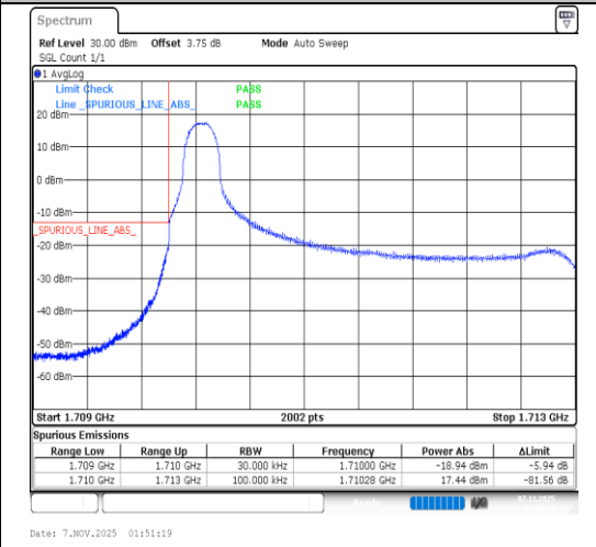
Band66-3MHz-64QAM-131987-1RB#0-PASS
