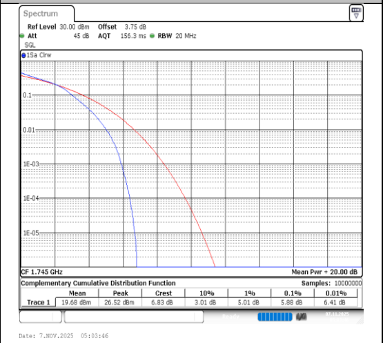
Band66-15MHz-16QAM-132322-75RB#0-PASS
