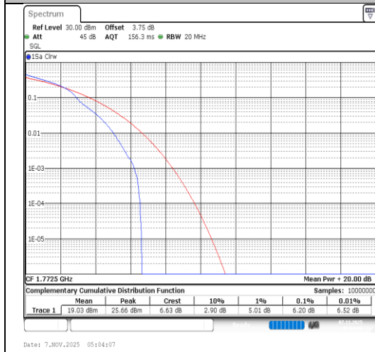
Band66-15MHz-16QAM-132597-1RB#0-PASS
