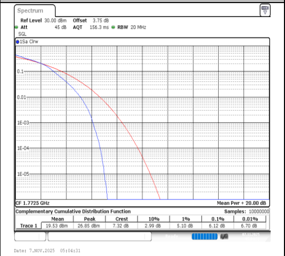
Band66-15MHz-64QAM-132597-75RB#0-PASS
