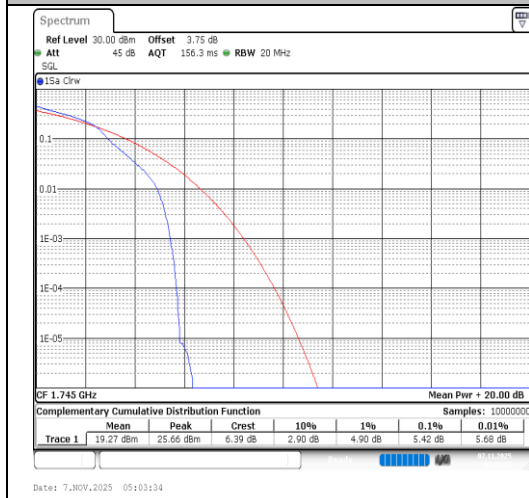
Band66-15MHz-64QAM-132322-1RB#0-PASS
