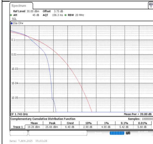
Band66-15MHz-16QAM-132322-1RB#0-PASS
