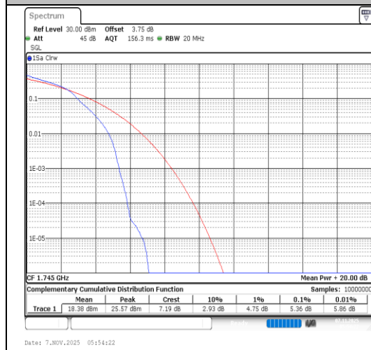
Band66-20MHz-64QAM-132322-1RB#0-PASS
