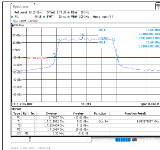
Band66-1.4MHz-QPSK-131979-6RB#0-PASS
