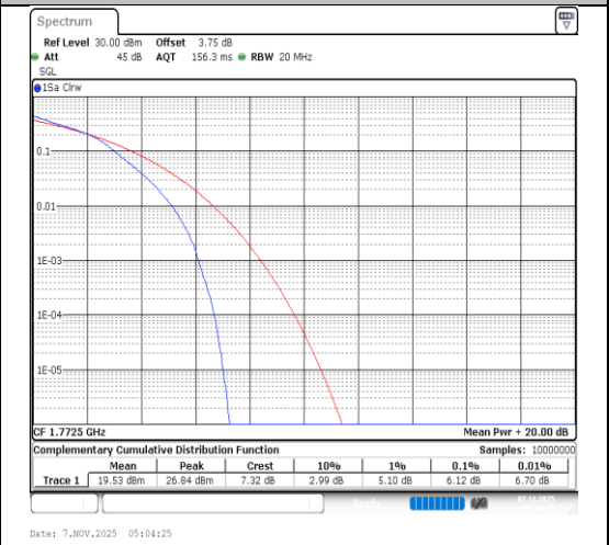
Band66-15MHz-16QAM-132597-75RB#0-PASS
