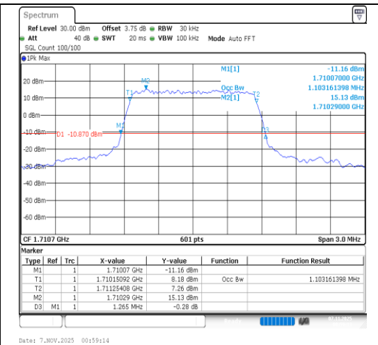
Band66-1.4MHz-64QAM-131979-6RB#0-PASS
