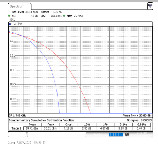
Band66-20MHz-16QAM-132322-100RB#0-PASS
