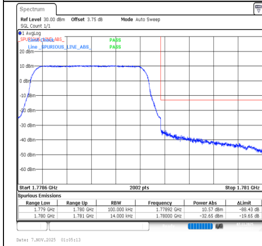
Band66-1.4MHz-64QAM-132665-6RB#0-PASS
