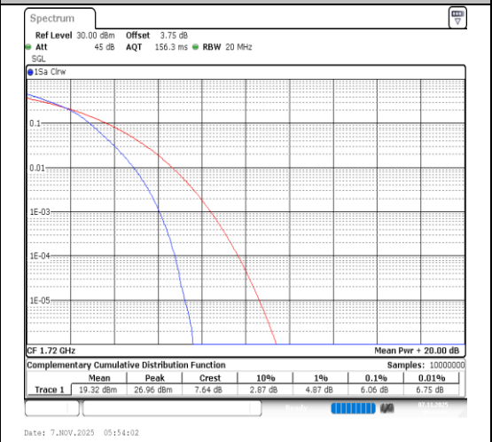
Band66-20MHz-64QAM-132072-100RB#0-PASS
