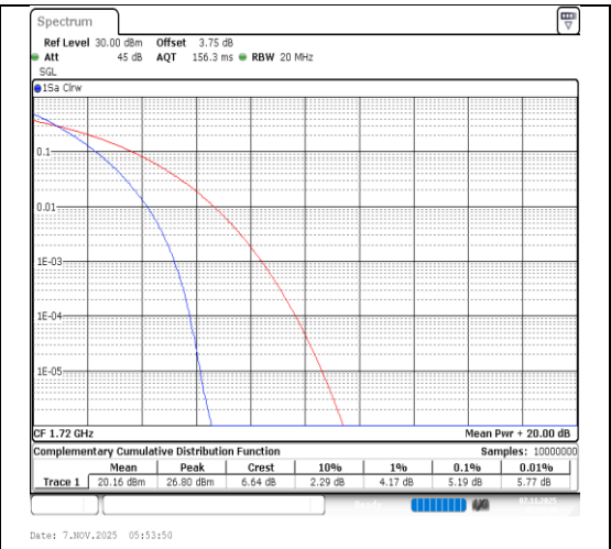
Band66-20MHz-QPSK-132072-100RB#0-PASS
