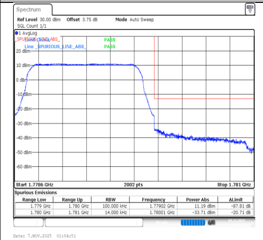
Band66-1.4MHz-QPSK-132665-6RB#0-PASS
