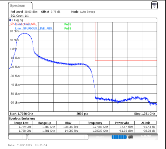
Band66-1.4MHz-16QAM-132665-1RB#0-PASS
