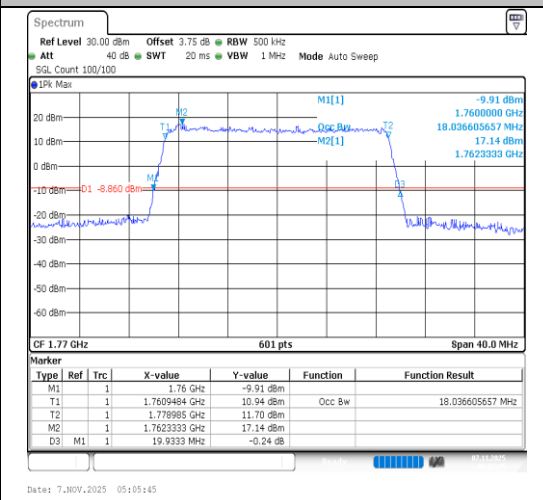
Band66-20MHz-QPSK-132572-100RB#0-PASS
