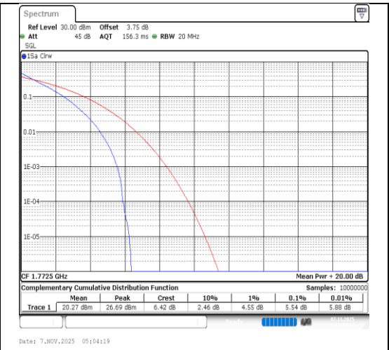
Band66-15MHz-QPSK-132597-75RB#0-PASS
