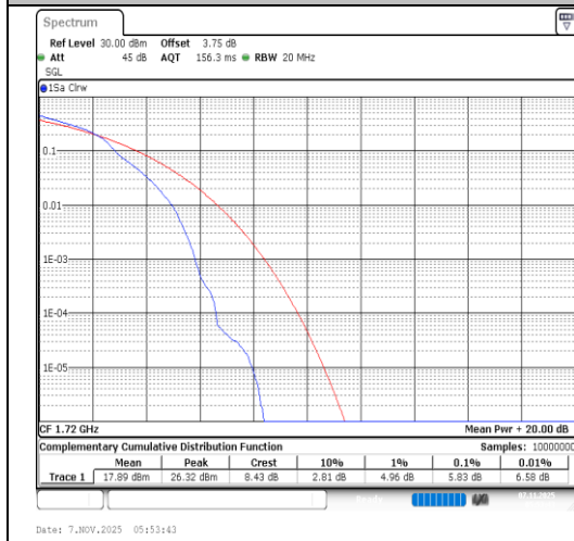
Band66-20MHz-64QAM-132072-1RB#0-PASS
