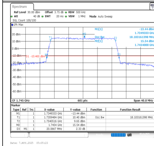
Band66-20MHz-16QAM-132322-100RB#0-PASS
