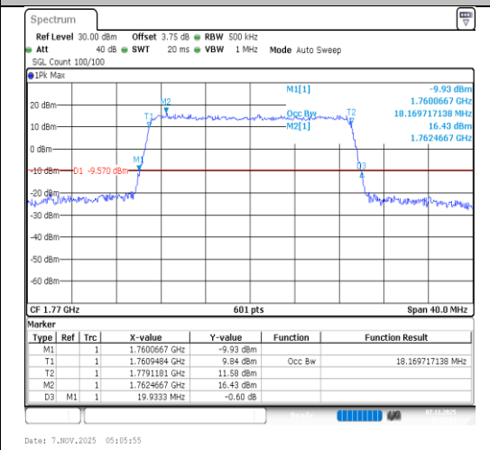
Band66-20MHz-16QAM-132572-100RB#0-PASS
