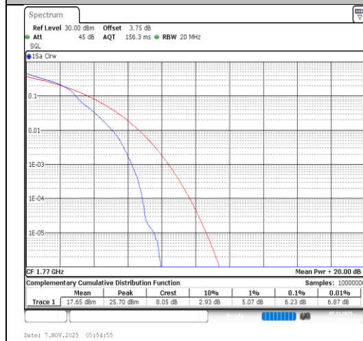
Band66-20MHz-16QAM-132572-1RB#0-PASS
