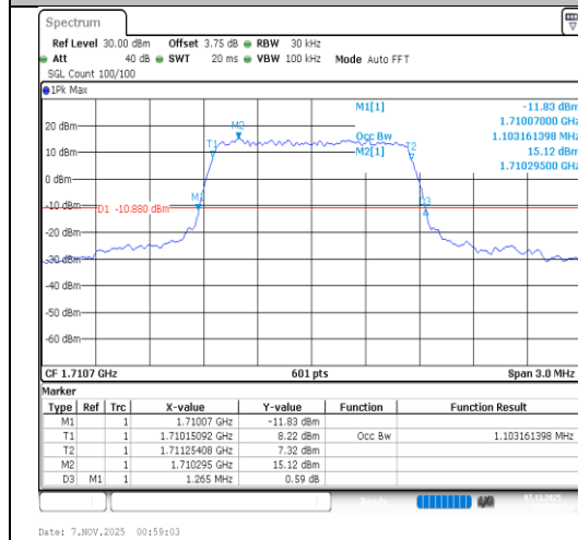
Band66-1.4MHz-16QAM-131979-6RB#0-PASS
