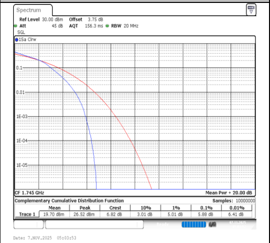
Band66-15MHz-64QAM-132322-75RB#0-PASS
