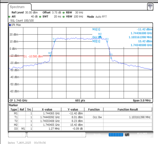
Band66-1.4MHz-16QAM-132322-6RB#0-PASS
