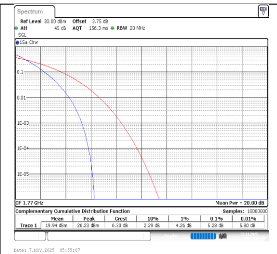
Band66-20MHz-QPSK-132572-100RB#0-PASS
