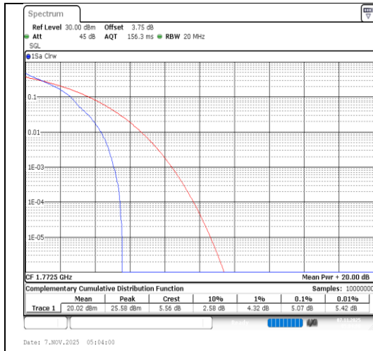
Band66-15MHz-QPSK-132597-1RB#0-PASS
