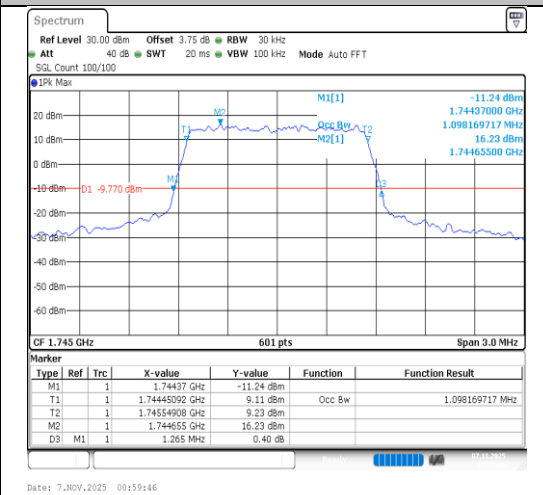
Band66-1.4MHz-QPSK-132322-6RB#0-PASS
