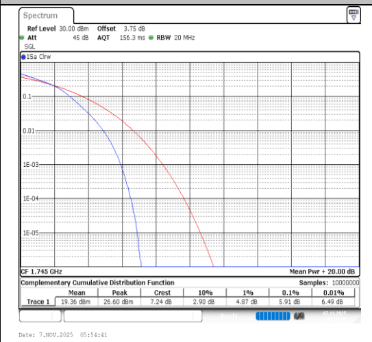
Band66-20MHz-64QAM-132322-100RB#0-PASS
