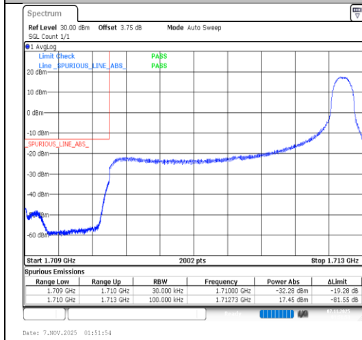
Band66-3MHz-64QAM-131987-1RB#14-PASS
