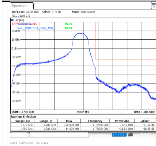
Band66-1.4MHz-16QAM-132665-1RB#5-PASS
