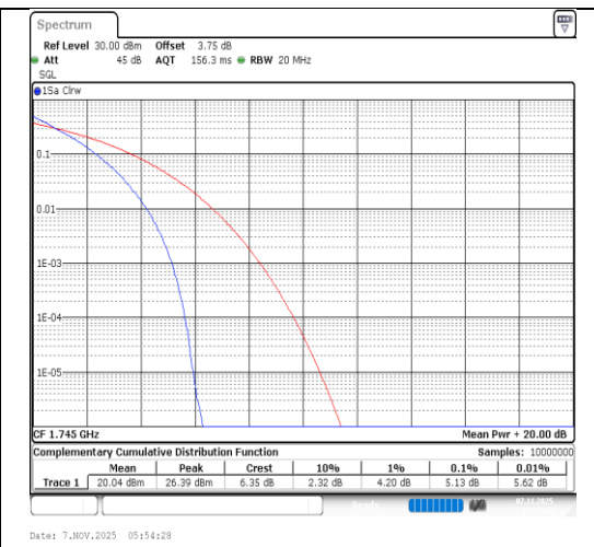
Band66-20MHz-QPSK-132322-100RB#0-PASS
