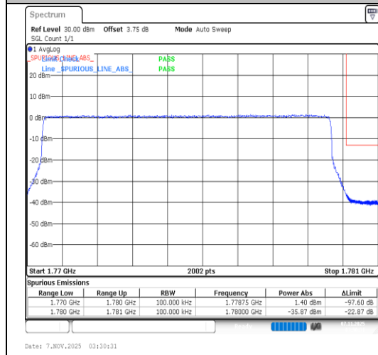
Band66-10MHz-64QAM-132622-50RB#0-PASS
