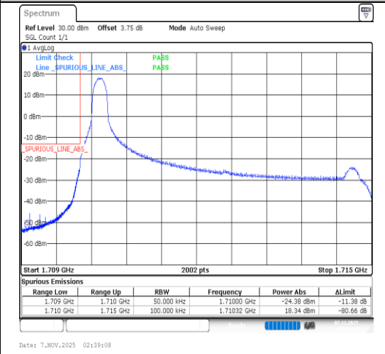
Band66-5MHz-64QAM-131997-1RB#0-PASS
