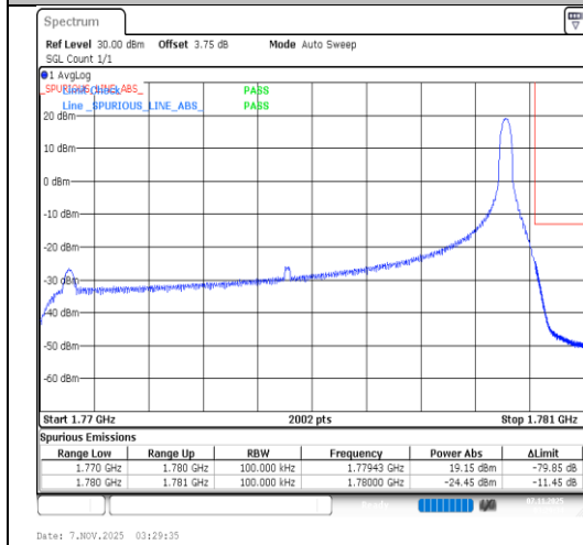
Band66-10MHz-QPSK-132622-1RB#49-PASS
