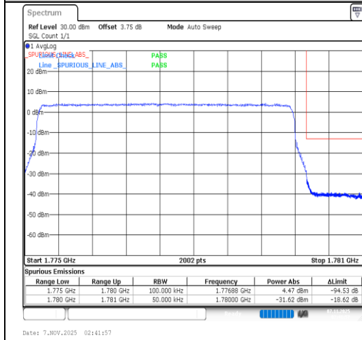
Band66-5MHz-64QAM-132647-25RB#0-PASS
