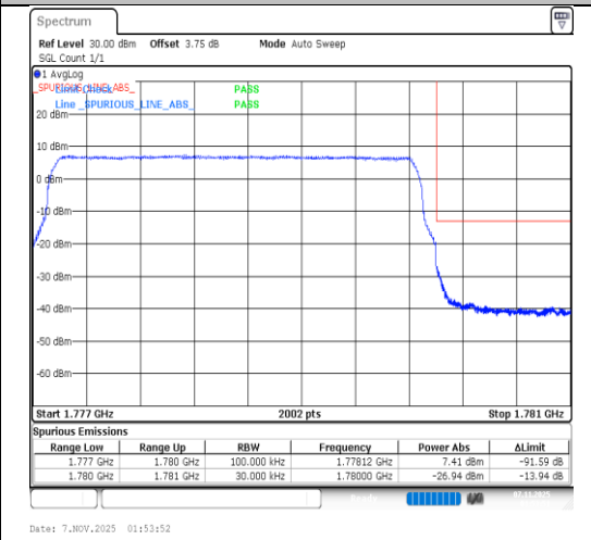
Band66-3MHz-QPSK-132657-15RB#0-PASS
