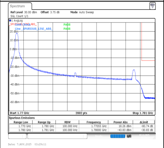
Band66-10MHz-16QAM-132622-1RB#0-PASS
