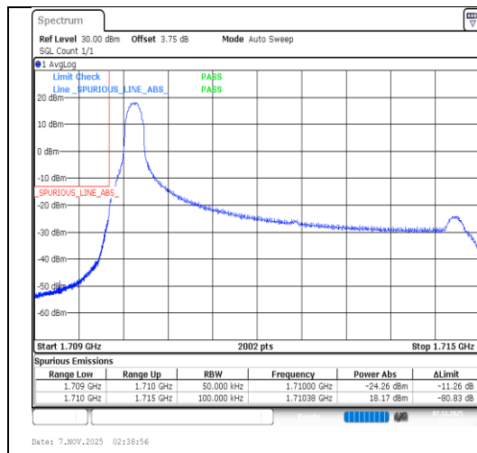
Band66-5MHz-16QAM-131997-1RB#0-PASS
