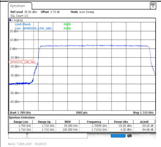
Band66-5MHz-64QAM-131997-25RB#0-PASS
