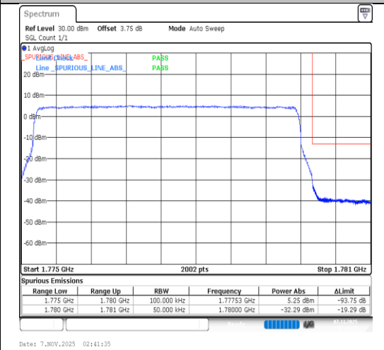
Band66-5MHz-QPSK-132647-25RB#0-PASS
