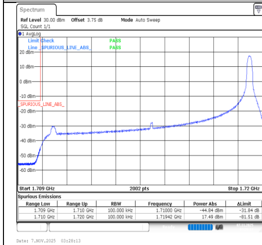
Band66-10MHz-64QAM-132022-1RB#49-PASS
