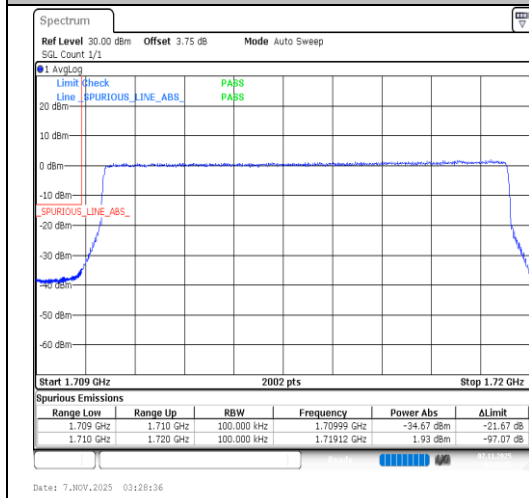
Band66-10MHz-16QAM-132022-50RB#0-PASS
