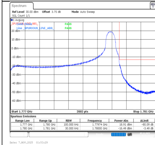
Band66-3MHz-16QAM-132657-1RB#14-PASS
