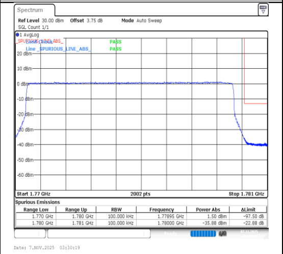
Band66-10MHz-16QAM-132622-50RB#0-PASS
