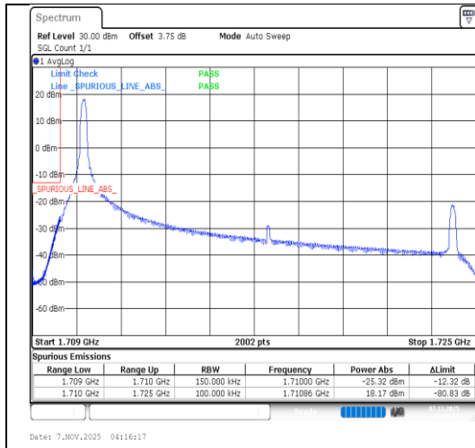
Band66-15MHz-16QAM-132047-1RB#0-PASS
