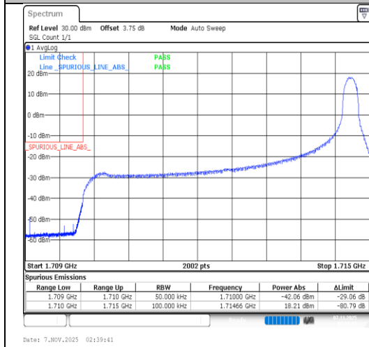
Band66-5MHz-64QAM-131997-1RB#24-PASS
