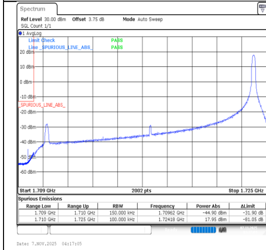
Band66-15MHz-64QAM-132047-1RB#74-PASS
