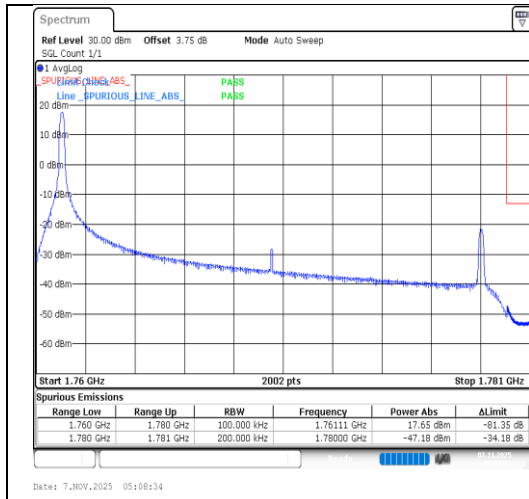
Band66-20MHz-64QAM-132572-1RB#0-PASS
