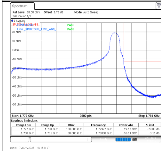
Band66-3MHz-QPSK-132657-1RB#14-PASS
