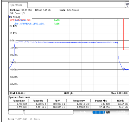
Band66-20MHz-64QAM-132572-100RB#0-PASS
