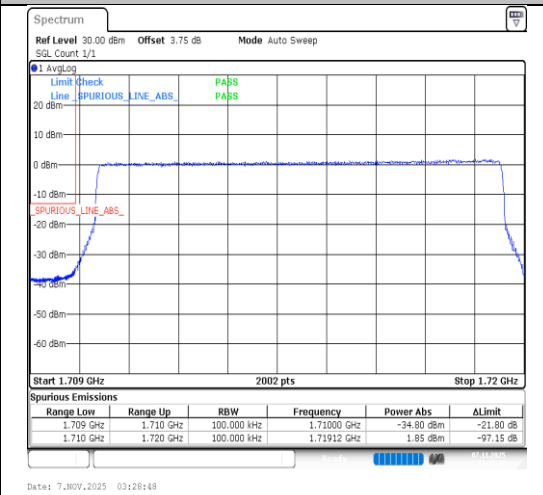
Band66-10MHz-64QAM-132022-50RB#0-PASS
