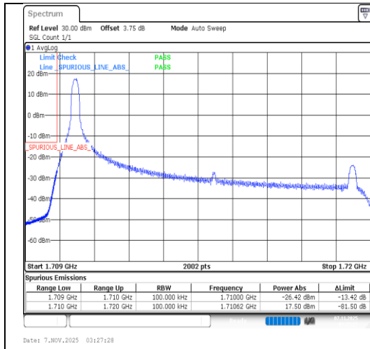
Band66-10MHz-16QAM-132022-1RB#0-PASS
