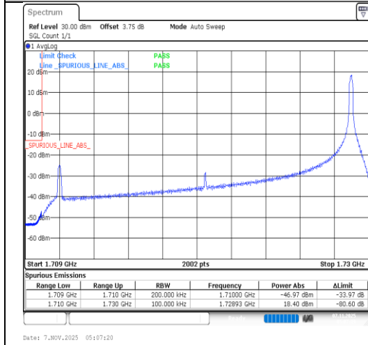
Band66-20MHz-64QAM-132072-1RB#99-PASS
