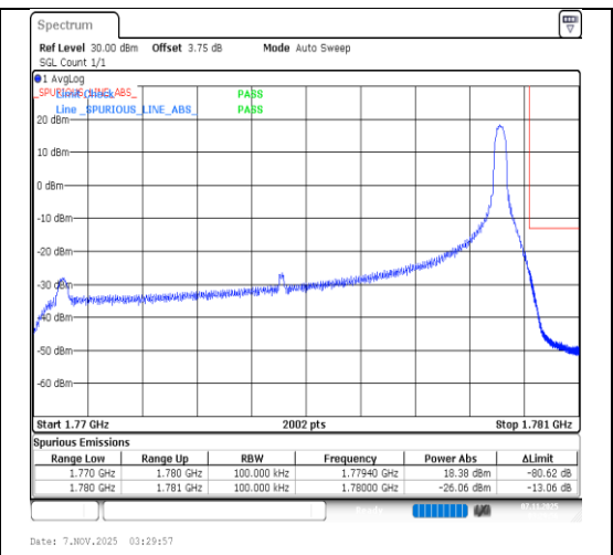
Band66-10MHz-64QAM-132622-1RB#49-PASS
