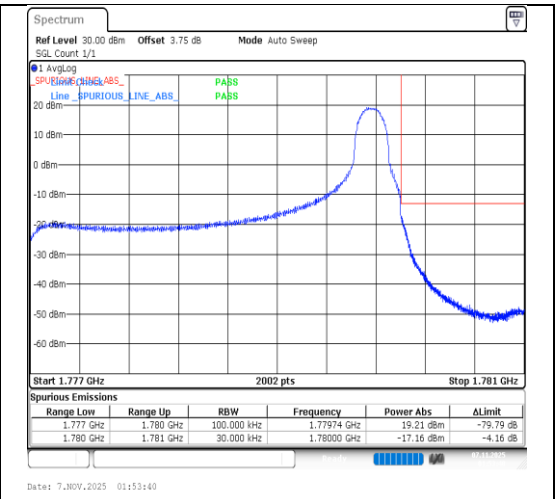
Band66-3MHz-64QAM-132657-1RB#14-PASS
