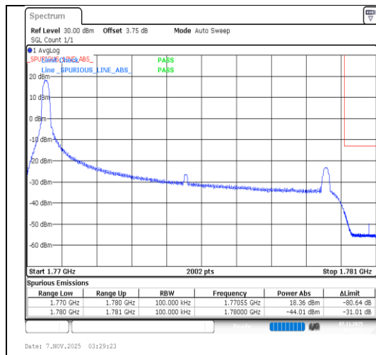
Band66-10MHz-64QAM-132622-1RB#0-PASS
