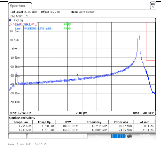
Band66-15MHz-64QAM-132597-1RB#74-PASS
