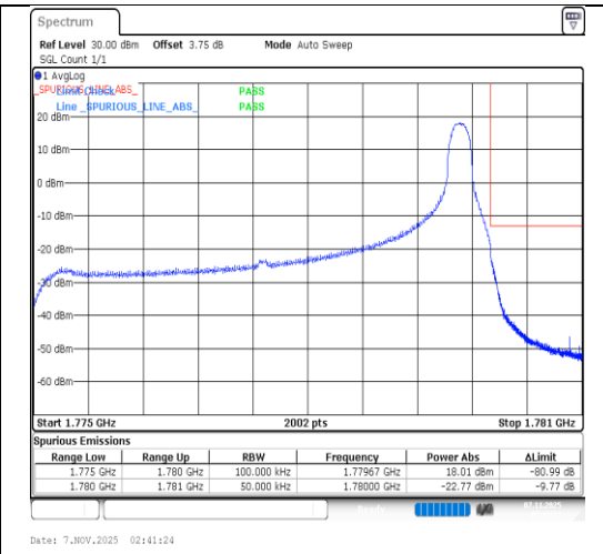
Band66-5MHz-64QAM-132647-1RB#24-PASS
