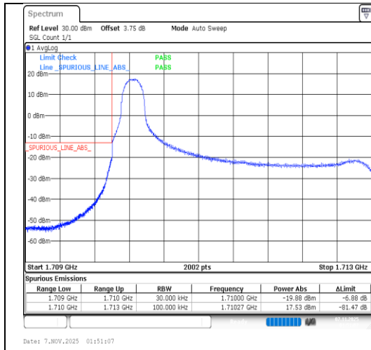
Band66-3MHz-16QAM-131987-1RB#0-PASS
