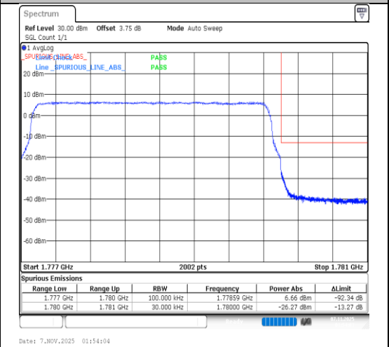
Band66-3MHz-16QAM-132657-15RB#0-PASS
