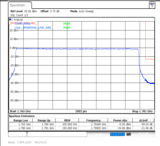
Band66-15MHz-16QAM-132597-75RB#0-PASS
