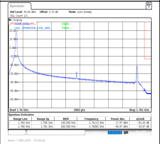
Band66-20MHz-16QAM-132572-1RB#0-PASS
