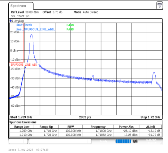
Band66-10MHz-64QAM-132022-1RB#0-PASS
