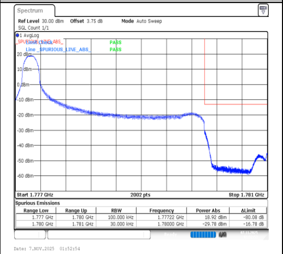
Band66-3MHz-16QAM-132657-1RB#0-PASS
