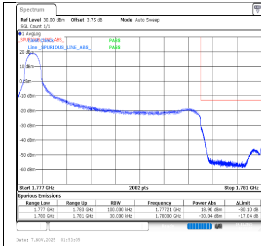
Band66-3MHz-64QAM-132657-1RB#0-PASS
