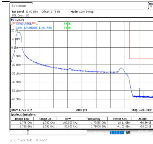
Band66-5MHz-64QAM-132647-1RB#0-PASS
