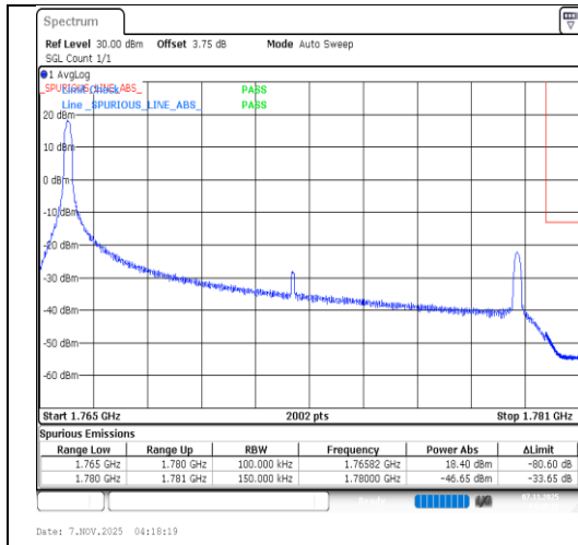
Band66-15MHz-64QAM-132597-1RB#0-PASS
