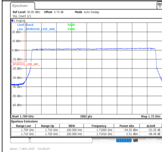
Band66-10MHz-QPSK-132022-50RB#0-PASS
