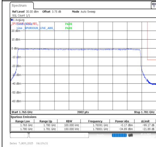
Band66-15MHz-64QAM-132597-75RB#0-PASS
