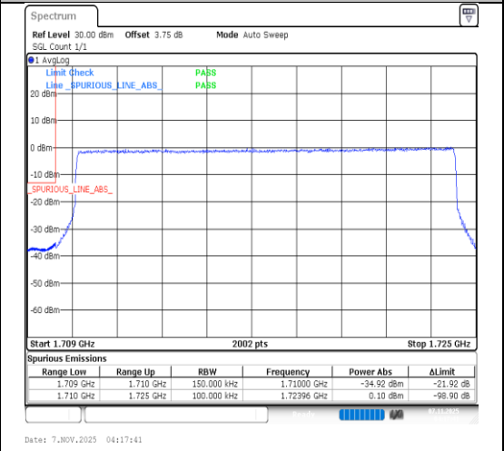
Band66-15MHz-64QAM-132047-75RB#0-PASS
