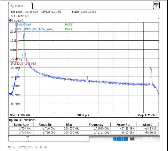
Band66-20MHz-64QAM-132072-1RB#0-PASS
