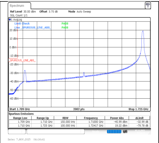
Band66-15MHz-QPSK-132047-1RB#74-PASS
