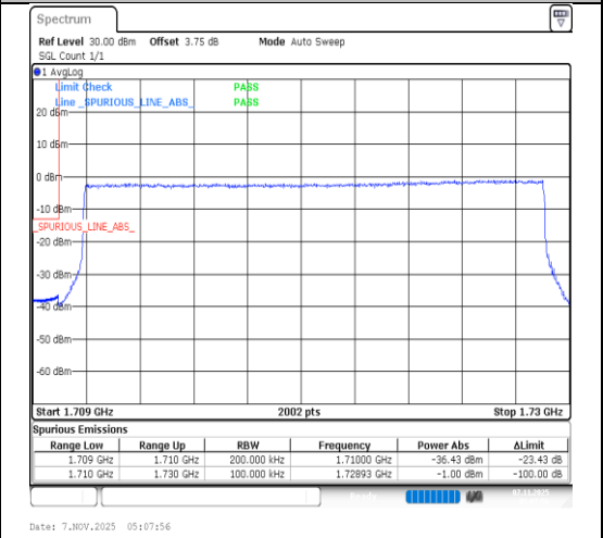
Band66-20MHz-64QAM-132072-100RB#0-PASS
