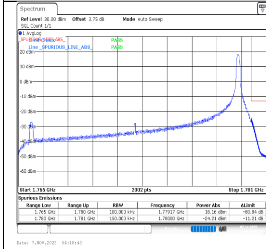
Band66-15MHz-16QAM-132597-1RB#74-PASS
