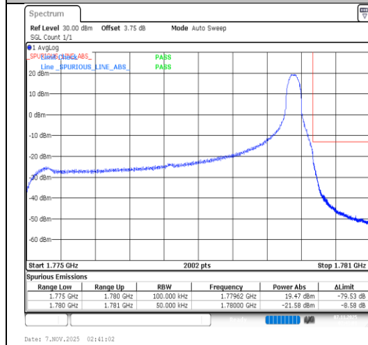
Band66-5MHz-QPSK-132647-1RB#24-PASS
