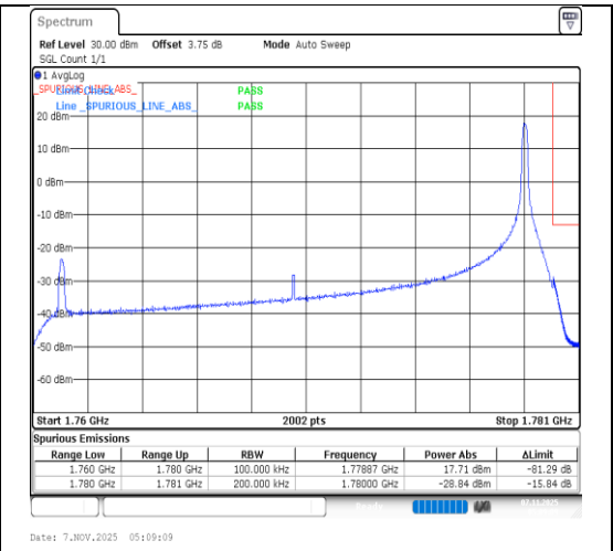
Band66-20MHz-64QAM-132572-1RB#99-PASS
