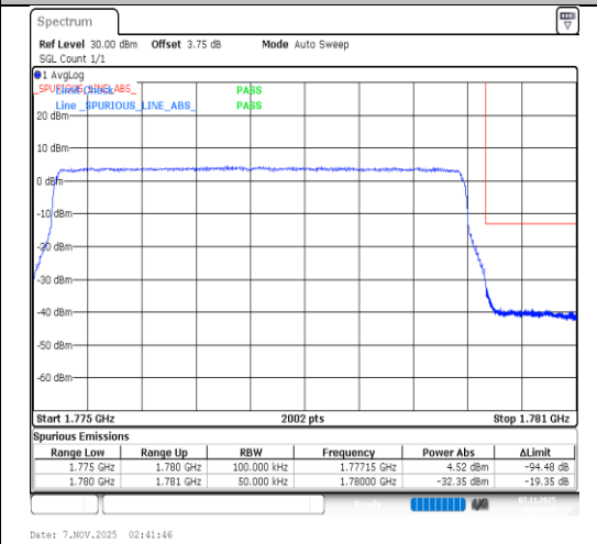
Band66-5MHz-16QAM-132647-25RB#0-PASS
