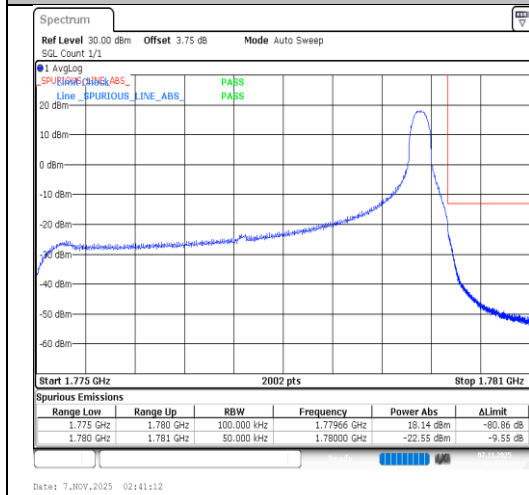
Band66-5MHz-16QAM-132647-1RB#24-PASS
