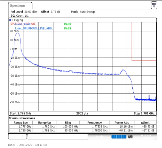
Band66-5MHz-16QAM-132647-1RB#0-PASS
