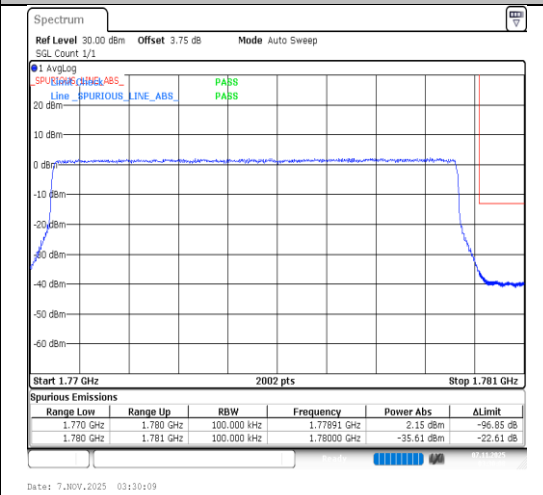
Band66-10MHz-QPSK-132622-50RB#0-PASS
