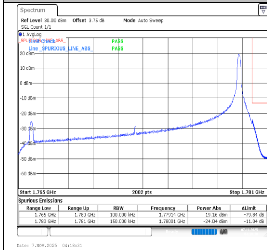
Band66-15MHz-QPSK-132597-1RB#74-PASS
