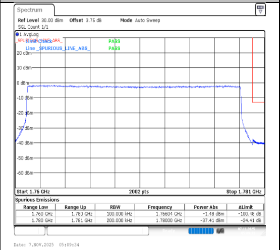
Band66-20MHz-16QAM-132572-100RB#0-PASS
