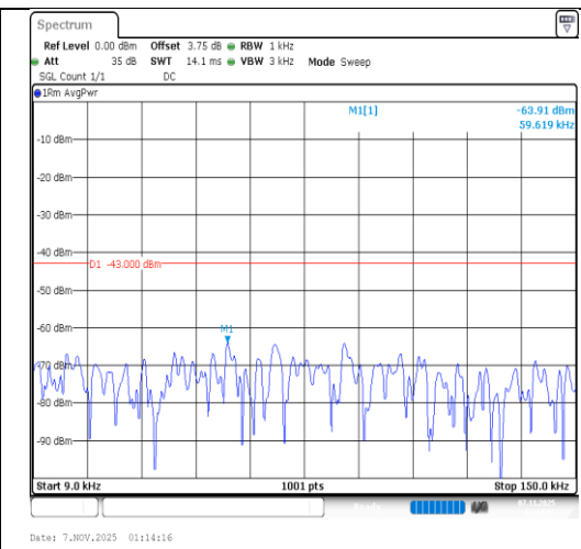
Band66-1.4MHz-64QAM-132322-1RB#5- 0.009~0.15-PASS
