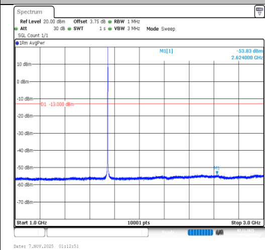
Band66-1.4MHz-64QAM-132322-1RB#0- 1000~3000-PASS
