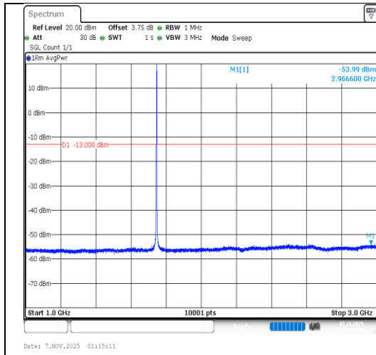
Band66-1.4MHz-QPSK-132322-6RB#0- 1000~3000-PASS
