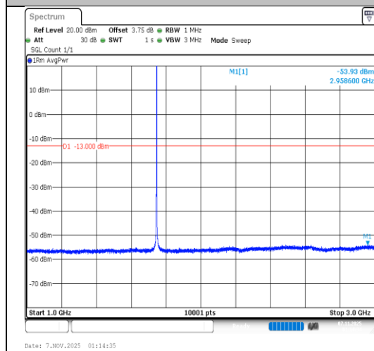
Band66-1.4MHz-64QAM-132322-1RB#5- 1000~3000-PASS
