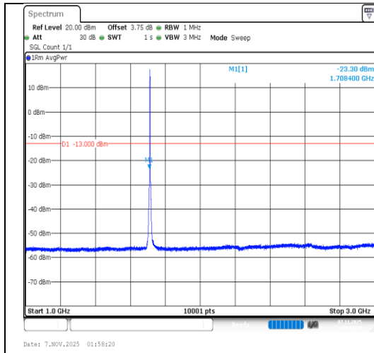
Band66-3MHz-QPSK-131987-15RB#0- 1000~3000-PASS
