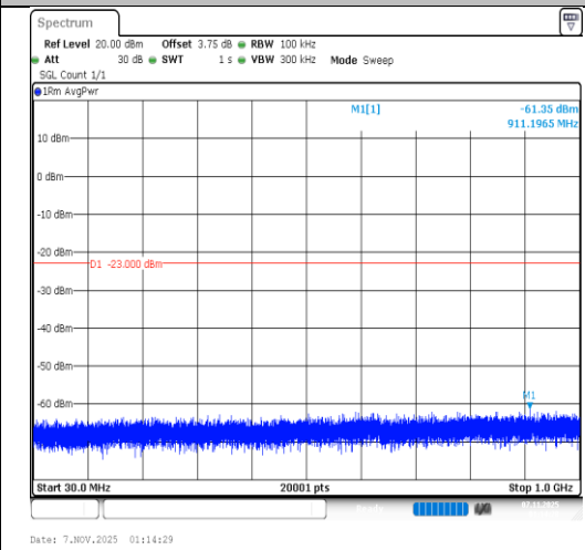
Band66-1.4MHz-64QAM-132322-1RB#5- 30~1000-PASS
