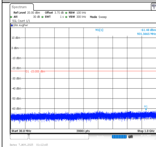
Band66-1.4MHz-64QAM-132322-1RB#0- 30~1000-PASS
