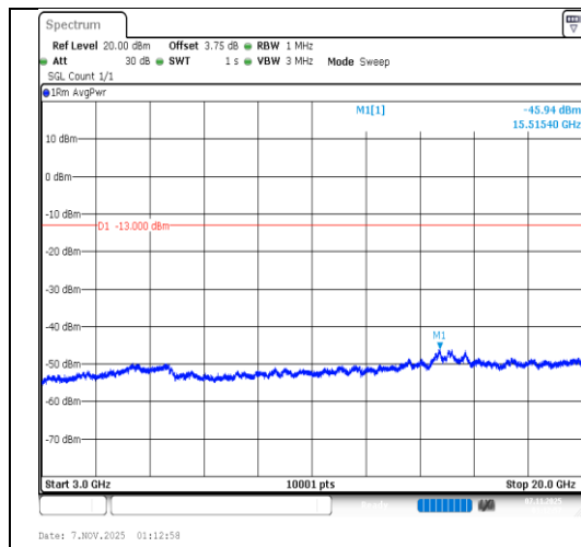
Band66-1.4MHz-64QAM-132322-1RB#0- 3000~20000-PASS
