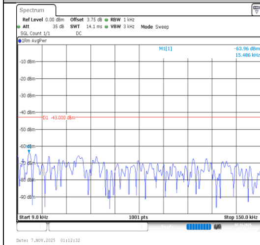
Band66-1.4MHz-64QAM-132322-1RB#0- 0.009~0.15-PASS
