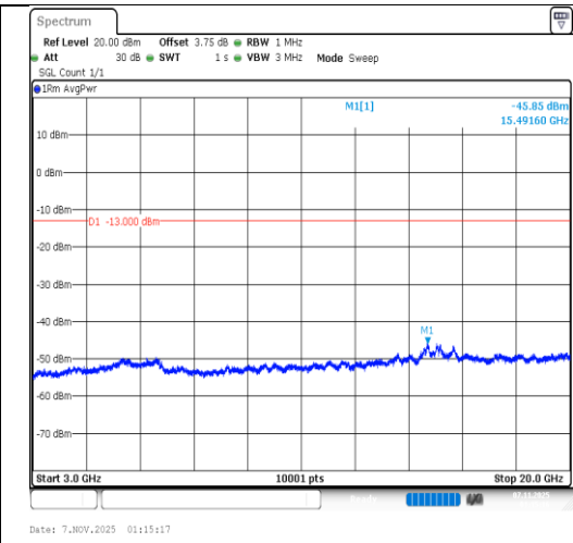
Band66-1.4MHz-QPSK-132322-6RB#0- 3000~20000-PASS
