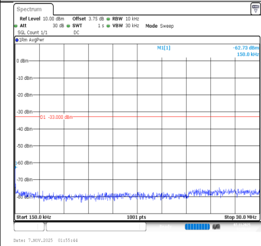
Band66-3MHz-64QAM-131987-1RB#0-0.15~30- PASS
