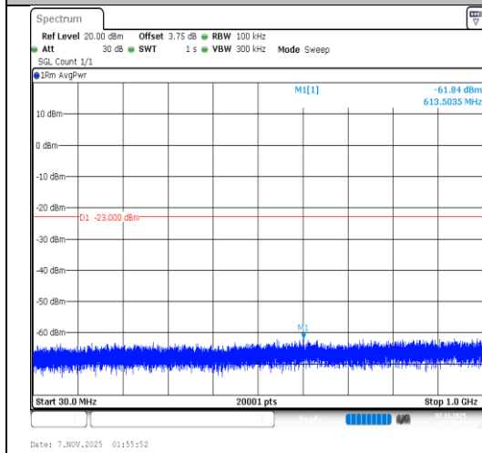
Band66-3MHz-64QAM-131987-1RB#0-30~1000- PASS
