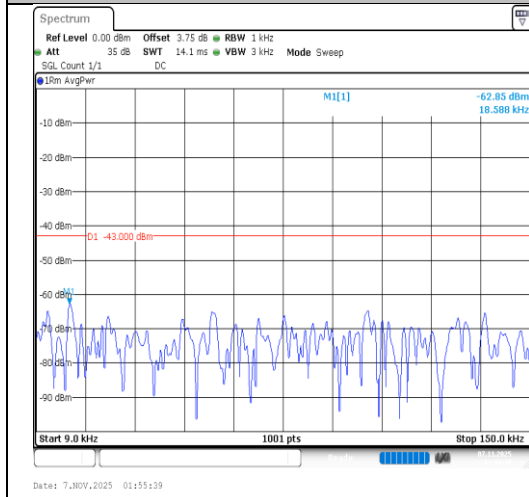
Band66-3MHz-64QAM-131987-1RB#0- 0.009~0.15-PASS
