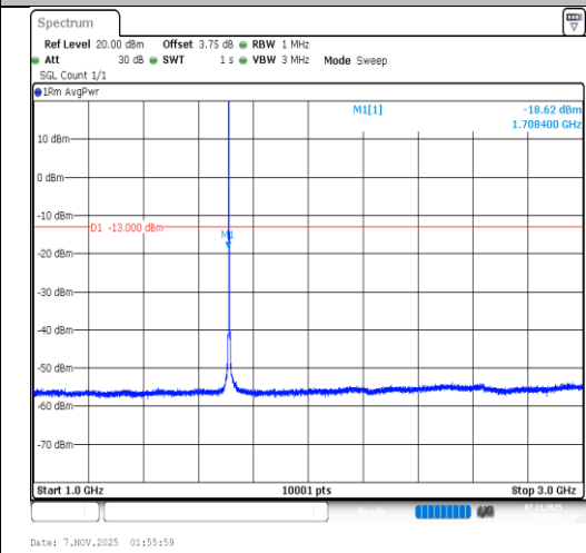
Band66-3MHz-64QAM-131987-1RB#0- 1000~3000-PASS
