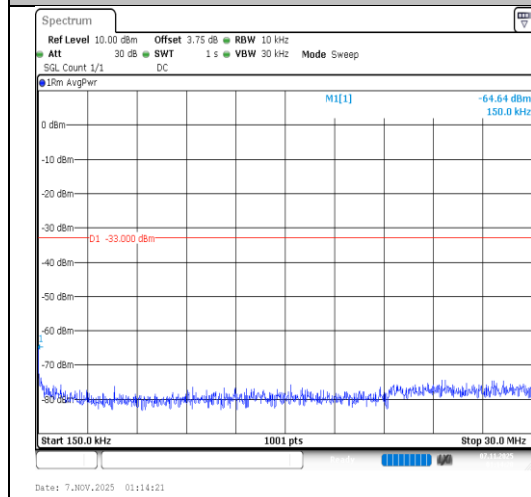
Band66-1.4MHz-64QAM-132322-1RB#5- 0.15~30-PASS
