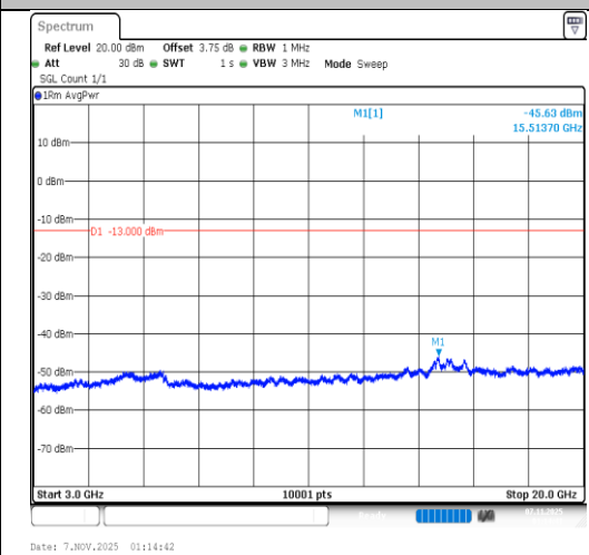
Band66-1.4MHz-64QAM-132322-1RB#5- 3000~20000-PASS
