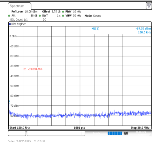
Band66-1.4MHz-64QAM-132322-1RB#0- 0.15~30-PASS
