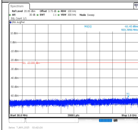
Band66-5MHz-QPSK-131997-1RB#0-30~1000- PASS
