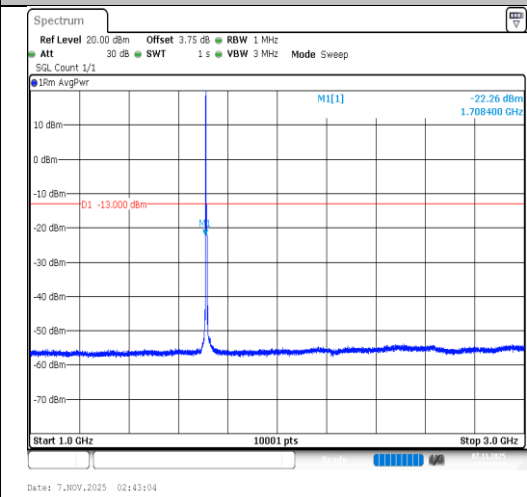
Band66-5MHz-16QAM-131997-1RB#0- 1000~3000-PASS
