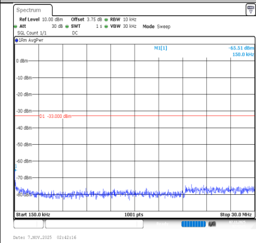
Band66-5MHz-QPSK-131997-1RB#0-0.15~30- PASS
