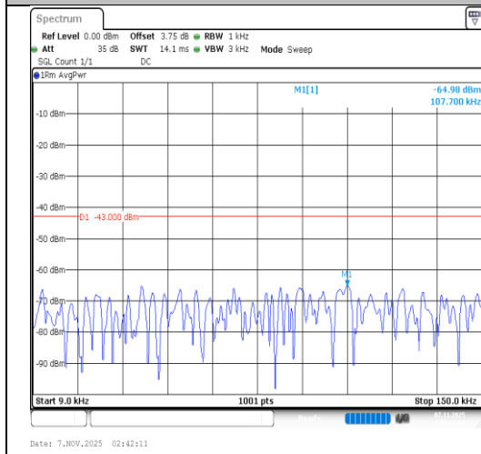
Band66-5MHz-QPSK-131997-1RB#0- 0.009~0.15-PASS
