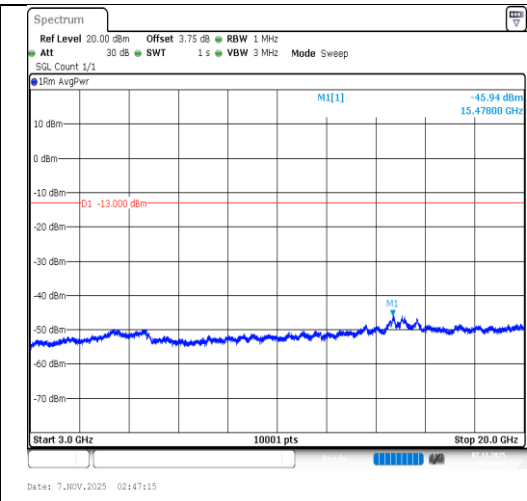
Band66-5MHz-64QAM-131997-25RB#0- 3000~20000-PASS
