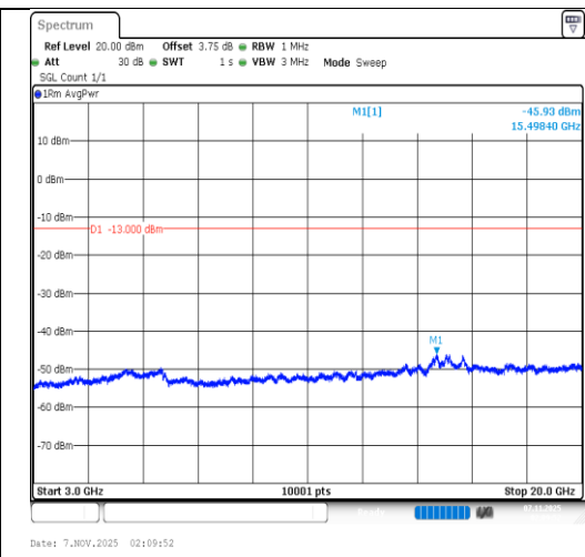
Band66-3MHz-16QAM-132657-15RB#0- 3000~20000-PASS
