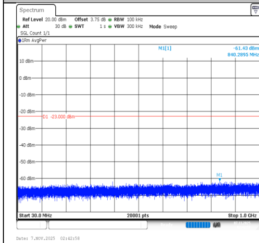
Band66-5MHz-16QAM-131997-1RB#0-30~1000- PASS
