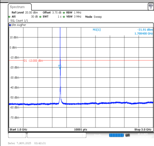
Band66-5MHz-QPSK-131997-1RB#0- 1000~3000-PASS
