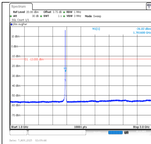
Band66-3MHz-16QAM-132657-15RB#0- 1000~3000-PASS
