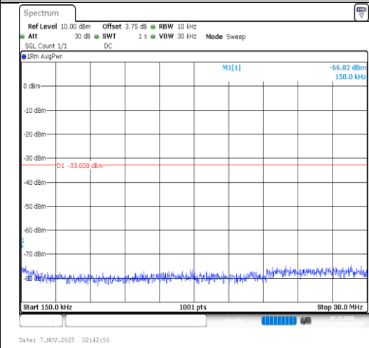
Band66-5MHz-16QAM-131997-1RB#0-0.15~30- PASS
