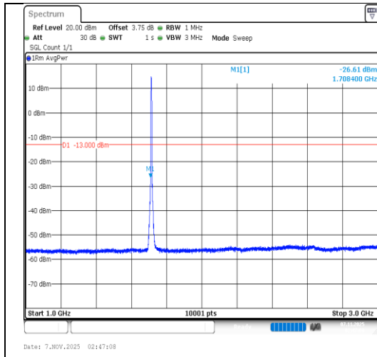
Band66-5MHz-64QAM-131997-25RB#0- 1000~3000-PASS
