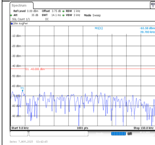
Band66-5MHz-16QAM-131997-1RB#0- 0.009~0.15-PASS
