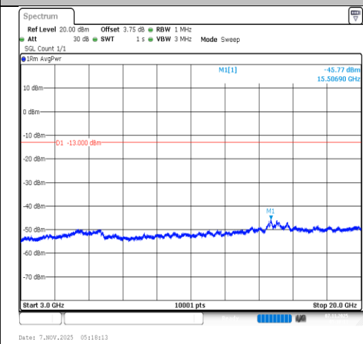
Band66-20MHz-16QAM-132322-1RB#99- 3000~20000-PASS
