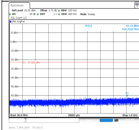
Band66-20MHz-16QAM-132322-1RB#0- 30~1000-PASS
