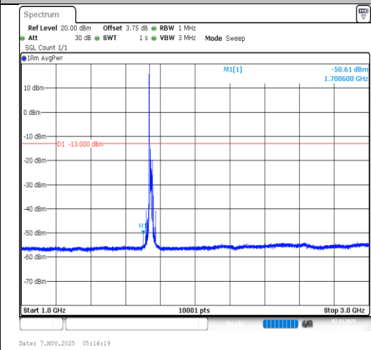
Band66-20MHz-16QAM-132322-1RB#0- 1000~3000-PASS
