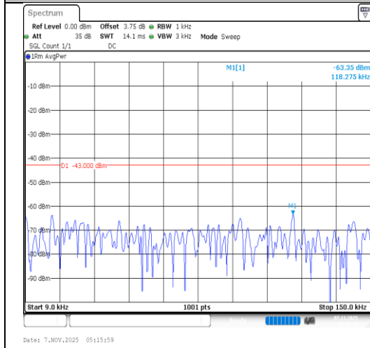
Band66-20MHz-16QAM-132322-1RB#0- 0.009~0.15-PASS
