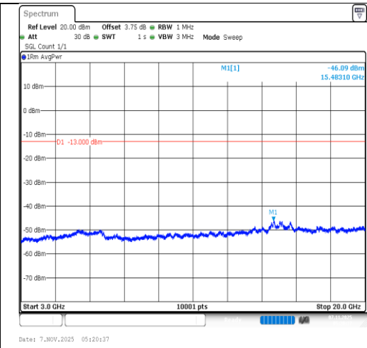
Band66-20MHz-64QAM-132322-100RB#0- 3000~20000-PASS
