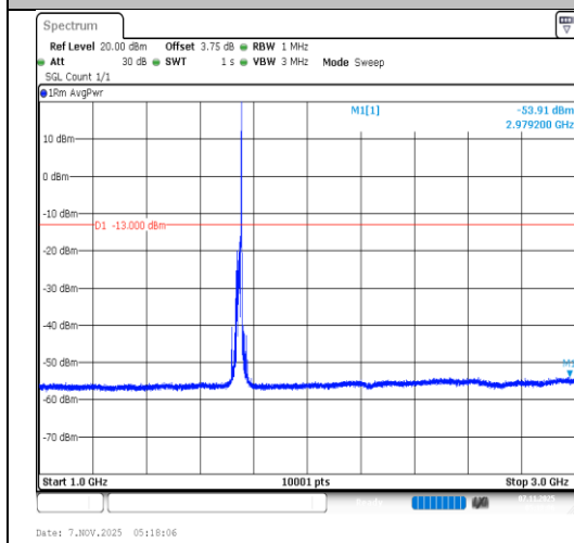
Band66-20MHz-16QAM-132322-1RB#99- 1000~3000-PASS
