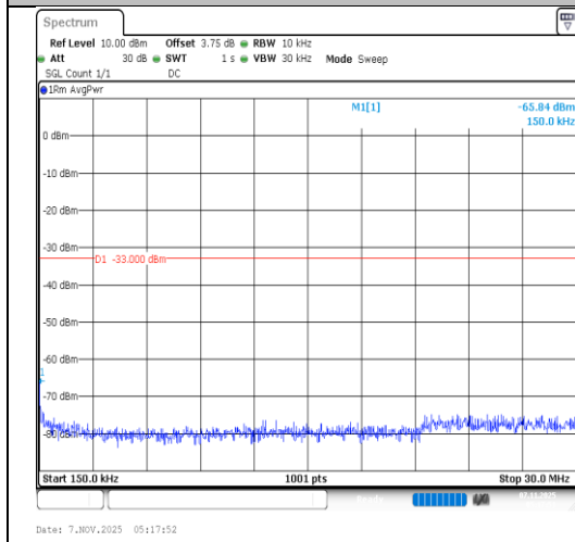
Band66-20MHz-16QAM-132322-1RB#99- 0.15~30-PASS
