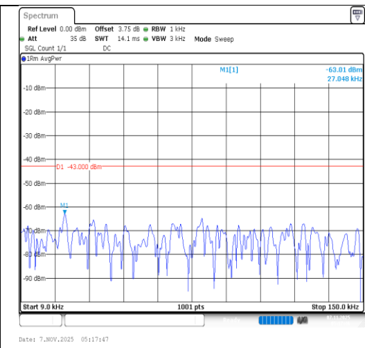
Band66-20MHz-16QAM-132322-1RB#99- 0.009~0.15-PASS
