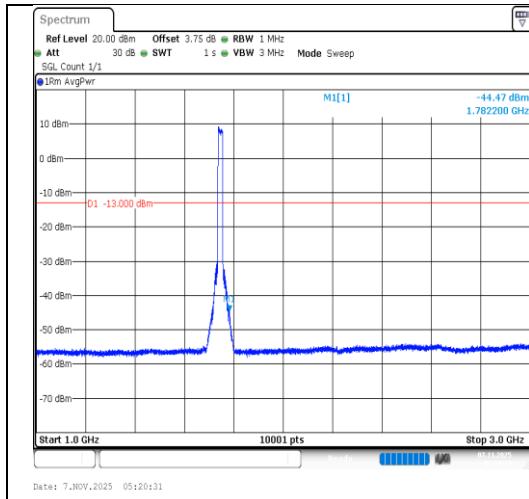
Band66-20MHz-64QAM-132322-100RB#0- 1000~3000-PASS
