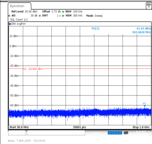
Band66-20MHz-16QAM-132322-1RB#99- 30~1000-PASS
