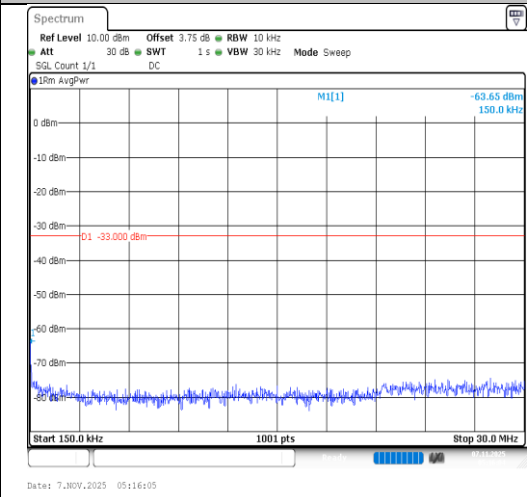
Band66-20MHz-16QAM-132322-1RB#0- 0.15~30-PASS
