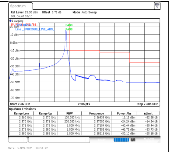
Band7-10MHz-64QAM-21400-1RB#49-PASS
