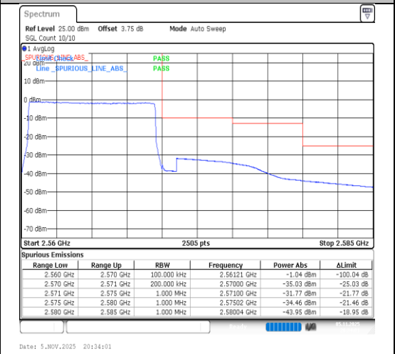
Band7-10MHz-16QAM-21400-50RB#0-PASS
