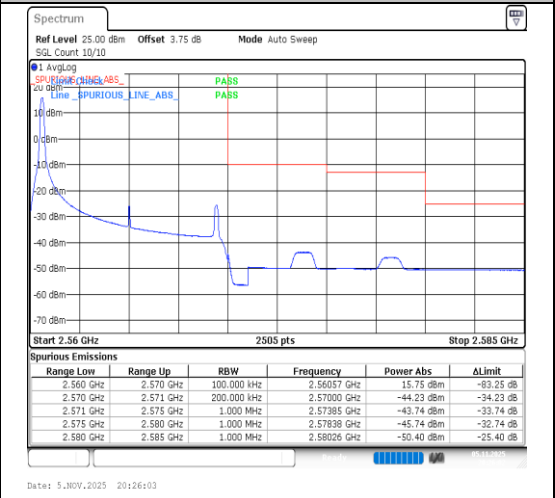
Band7-10MHz-16QAM-21400-1RB#0-PASS
