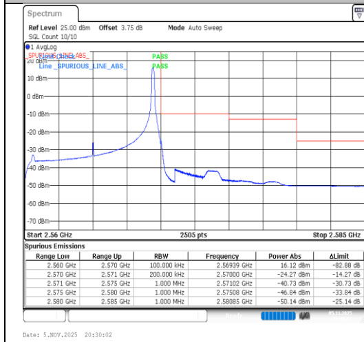
Band7-10MHz-16QAM-21400-1RB#49-PASS
