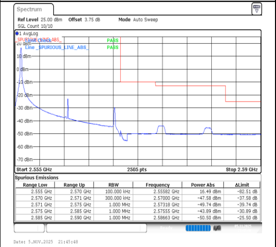
Band7-15MHz-16QAM-21375-1RB#0-PASS
