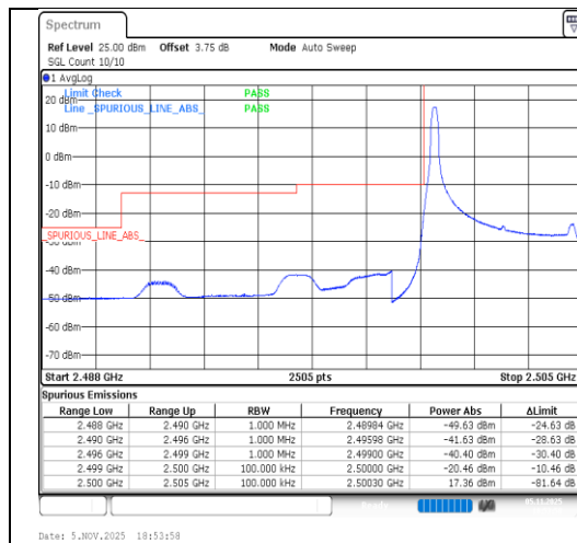
Band7-5MHz-QPSK-20775-1RB#0-PASS
