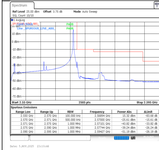
Band7-20MHz-16QAM-21350-1RB#99-PASS
