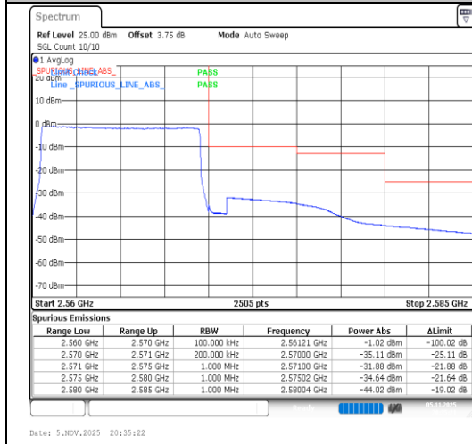
Band7-10MHz-64QAM-21400-50RB#0-PASS
