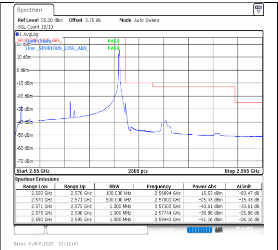
Band7-20MHz-64QAM-21350-1RB#99-PASS
