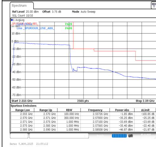
Band7-15MHz-64QAM-21375-75RB#0-PASS
