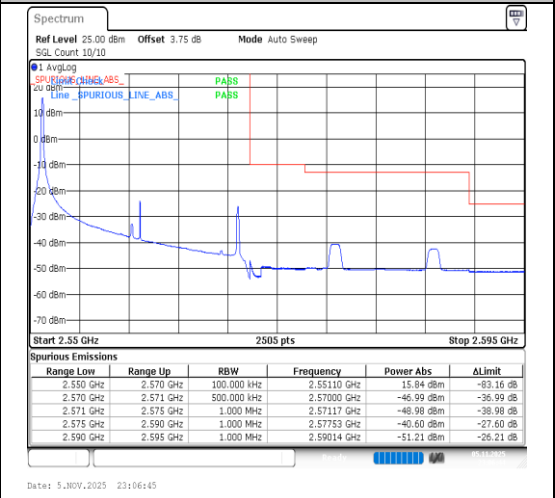
Band7-20MHz-16QAM-21350-1RB#0-PASS
