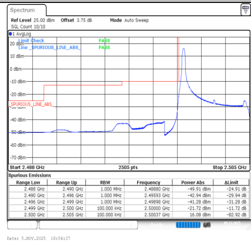
Band7-5MHz-64QAM-20775-1RB#0-PASS
