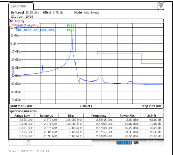
Band7-15MHz-64QAM-21375-1RB#74-PASS
