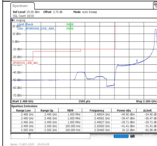
Band7-5MHz-64QAM-20775-1RB#24-PASS
