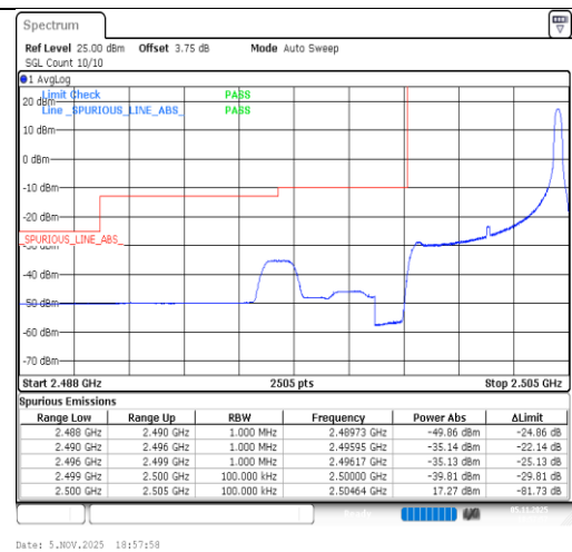
Band7-5MHz-QPSK-20775-1RB#24-PASS
