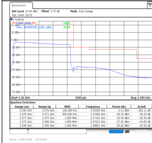
Band7-20MHz-64QAM-21350-100RB#0-PASS
