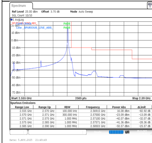
Band7-15MHz-16QAM-21375-1RB#74-PASS
