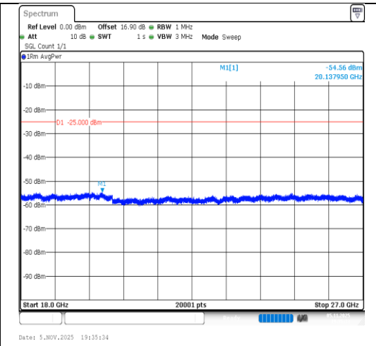
Band7-5MHz-QPSK-21425-1RB#0-18000~27000-PASS
