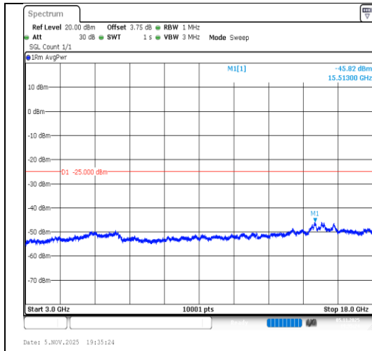
Band7-5MHz-QPSK-21425-1RB#0-3000~18000-PASS
