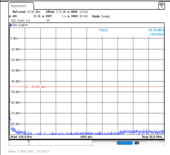
Band7-5MHz-QPSK-21425-1RB#24-0.15~30-PASS
