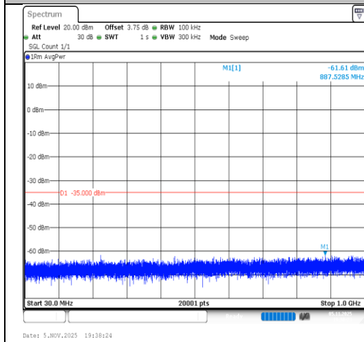
Band7-5MHz-QPSK-21425-1RB#24-30~1000-PASS
