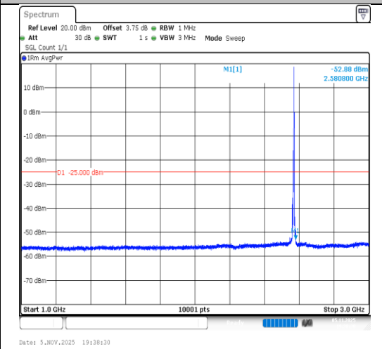
Band7-5MHz-QPSK-21425-1RB#24-1000~3000-PASS
