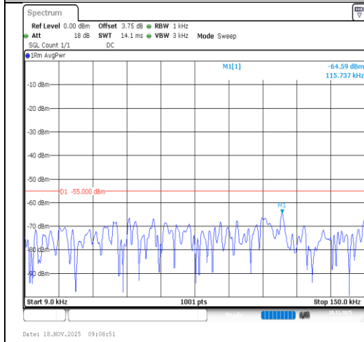
Band7-5MHz-QPSK-21425-1RB#24-0.009~0.15-PASS
