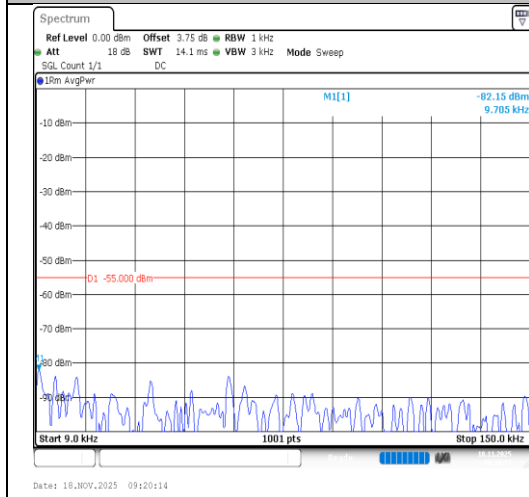
Band7-20MHz-QPSK-21100-100RB#0- 0.009~0.15-PASS
