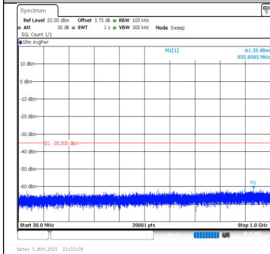
Band7-20MHz-QPSK-21100-100RB#0-30~1000- PASS
