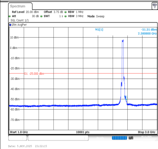
Band7-20MHz-QPSK-21100-100RB#0- 1000~3000-PASS
