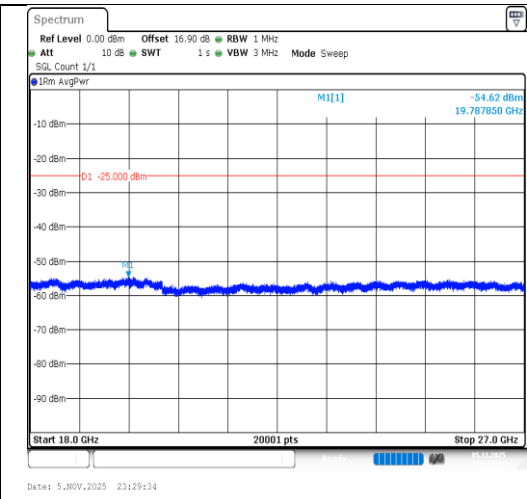
Band7-20MHz-QPSK-21100-1RB#99- 18000~27000-PASS
