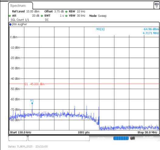
Band7-20MHz-QPSK-21100-100RB#0-0.15~30- PASS
