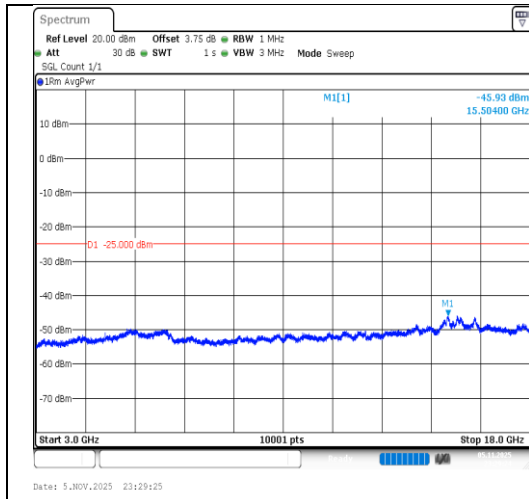
Band7-20MHz-QPSK-21100-1RB#99- 3000~18000-PASS
