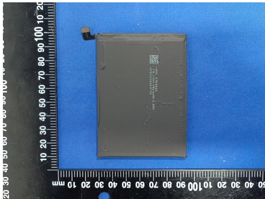
BATTERY 1 (REAR)
