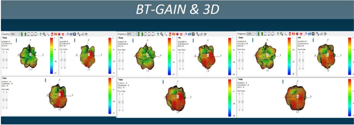
Radiation Pattern
