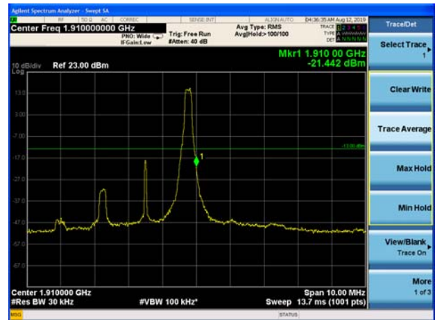
LTE Band 2 3MHz 64QAM 100%RB CH-High
