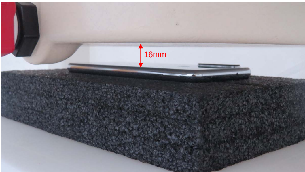
Picture 6: Back Side, the distance from handset to the bottom of the Phantom is 16mm
