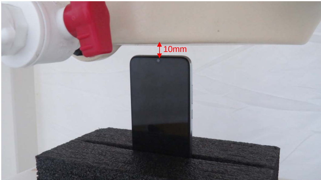
Picture 10: Top Side, the distance from handset to the bottom of the Phantom is 10mm
