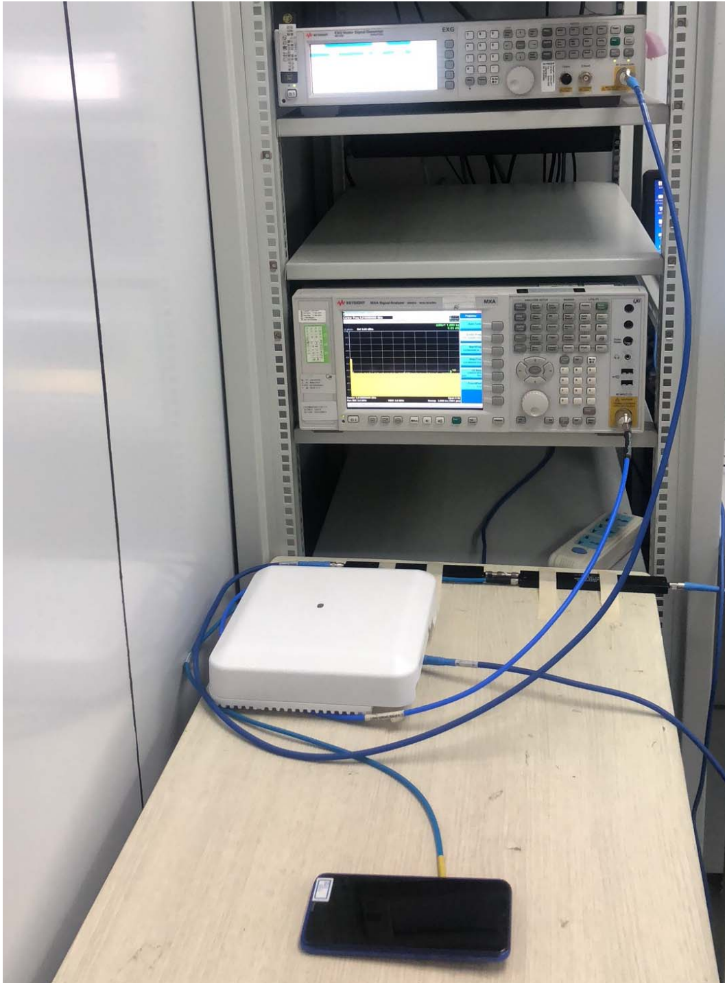
Picture 1 Test Setup
