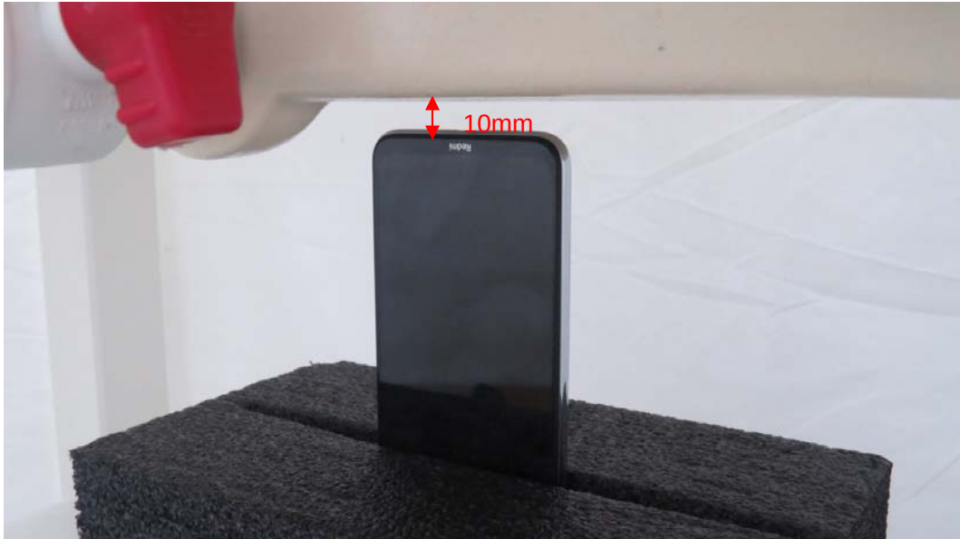
Picture 11: Bottom Side, the distance from handset to the bottom of the Phantom is 10mm
