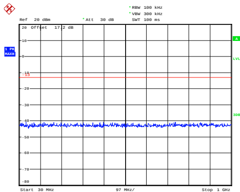
WCDMA Band IV CH-Low 30MHz~1GHz
