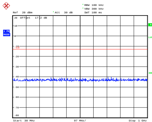
WCDMA Band IV CH-Middle 30MHz~1GHz
