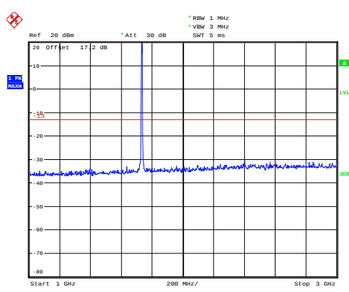
WCDMA Band IV CH-Middle 1GHz~3GHz
