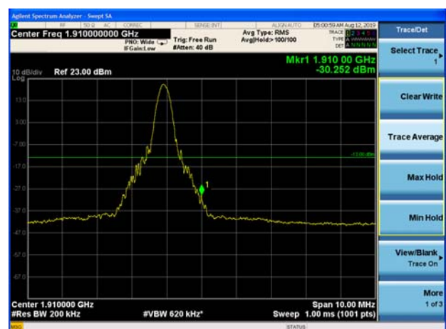
LTE Band 2 20MHz 64QAM 1RB CH-High
