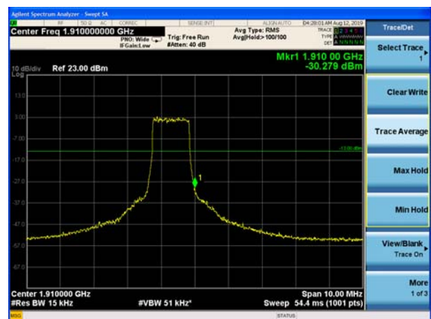
LTE Band 2 1.4MHz 64QAM 100%RB CH-High
