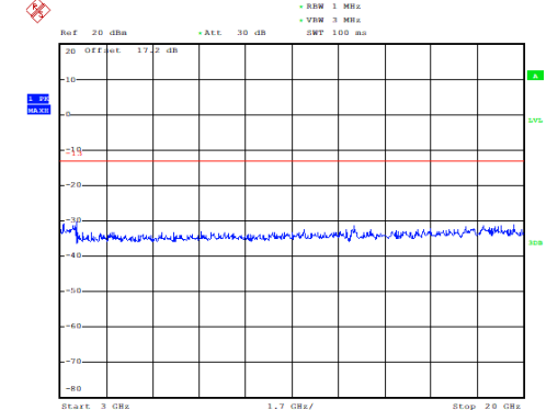
GSM 1900 CH-Low 3GHz~20GHz
