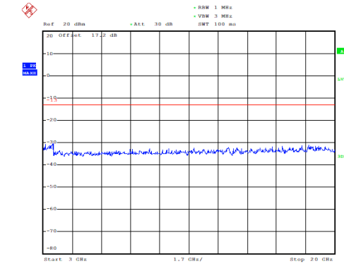
GSM 1900 CH-Middle 3GHz~20GHz
