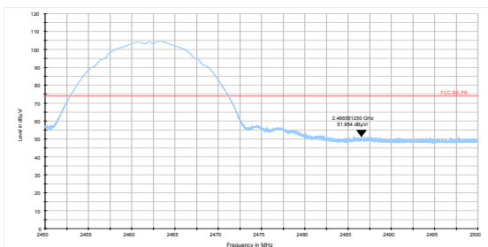
802.11b-Channel 11 Peak
