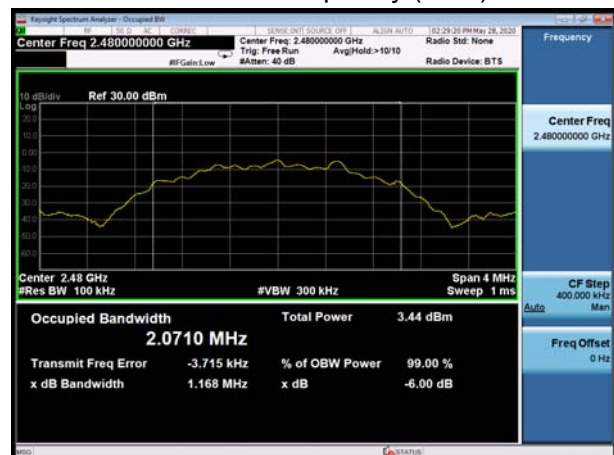
BLE V5.0 Carrier frequency (MHz): 2480
