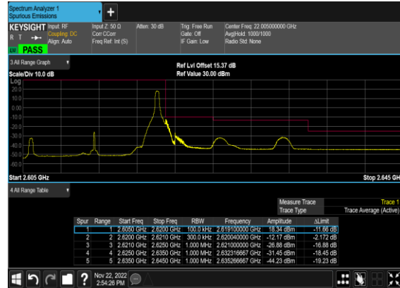
N38(15M)_DFT-s- OFDM_QPSK_Edge_1RB_Right_High_CH
