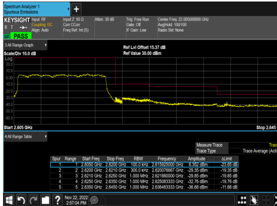
N38(15M)_DFT-s- OFDM_BPSK_Outer_Full_High_CH
