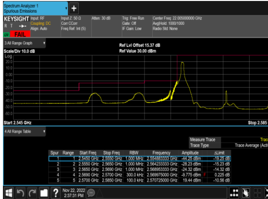
N38(15M)_DFT-s- OFDM_BPSK_Edge_1RB_Left_Low_CH
