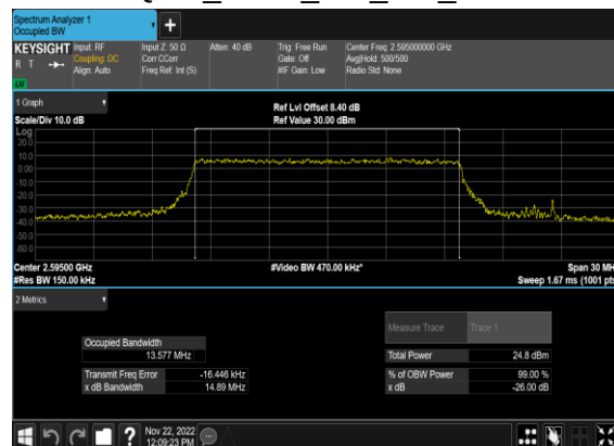
N38(15M)_CP-OFDM_256 QAM_Outer_Full_Mid_CH
