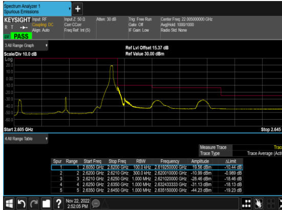
N38(15M)_DFT-s- OFDM_BPSK_Edge_1RB_Right_High_CH
