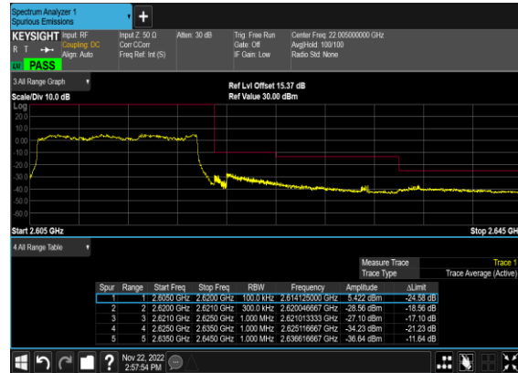
N38(15M)_DFT-s- OFDM_QPSK_Outer_Full_High_CH
