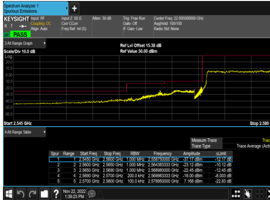
N38(10M)_DFT-s- OFDM_BPSK_Outer_Full_Low_CH
