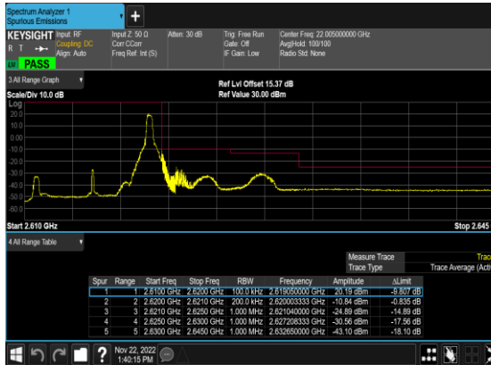
N38(10M)_DFT-s- OFDM_BPSK_Edge_1RB_Right_High_CH
