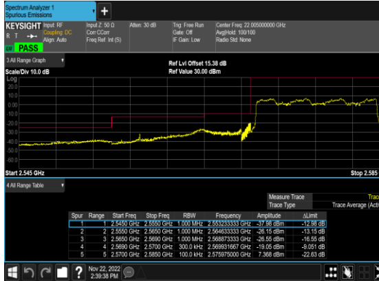
N38(15M)_DFT-s- OFDM_BPSK_Outer_Full_Low_CH
