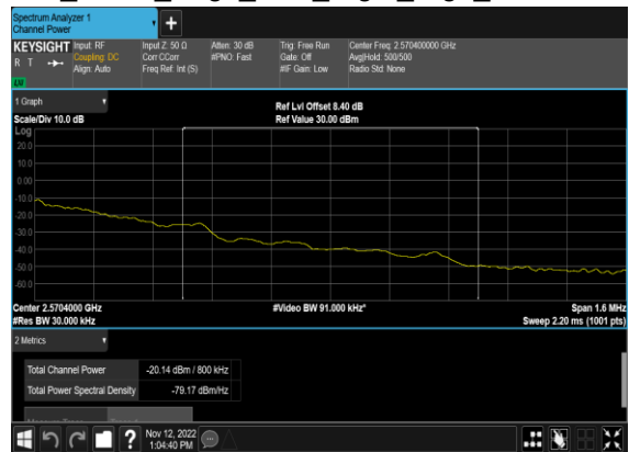
N7(40M)_DFT-s- OFDM_BPSK_Edge_1RB_Right_High_CH_CHP_PASS
