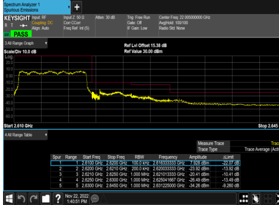
N38(10M)_DFT-s- OFDM_BPSK_Outer_Full_High_CH
