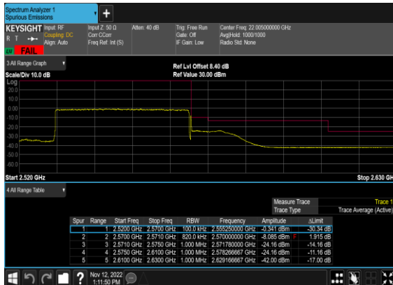
N7(40M)_DFT-s- OFDM_QPSK_Outer_Full_High_CH
