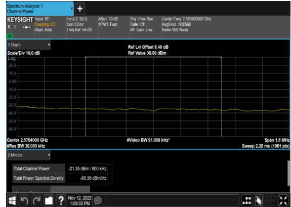
N7(40M)_DFT-s- OFDM_BPSK_Outer_Full_High_CH_CHP_PASS
