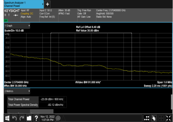
N7(40M)_DFT-s- OFDM_QPSK_Edge_1RB_Right_High_CH_CHP_PASS
