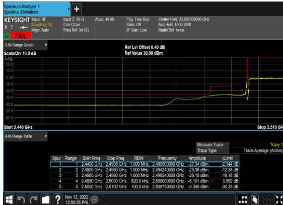
N7(40M)_DFT-s- OFDM_BPSK_Outer_Full_Low_CH
