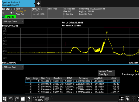
N38(10M)_DFT-s- OFDM_BPSK_Edge_1RB_Left_Low_CH
