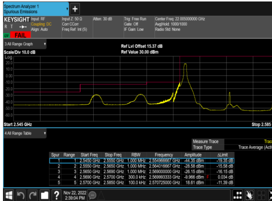
N38(15M)_DFT-s- OFDM_QPSK_Edge_1RB_Left_Low_CH
