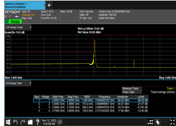
N78(50M)_DFT-s- OFDM_QPSK_Edge_1RB_Left_Low_CH
