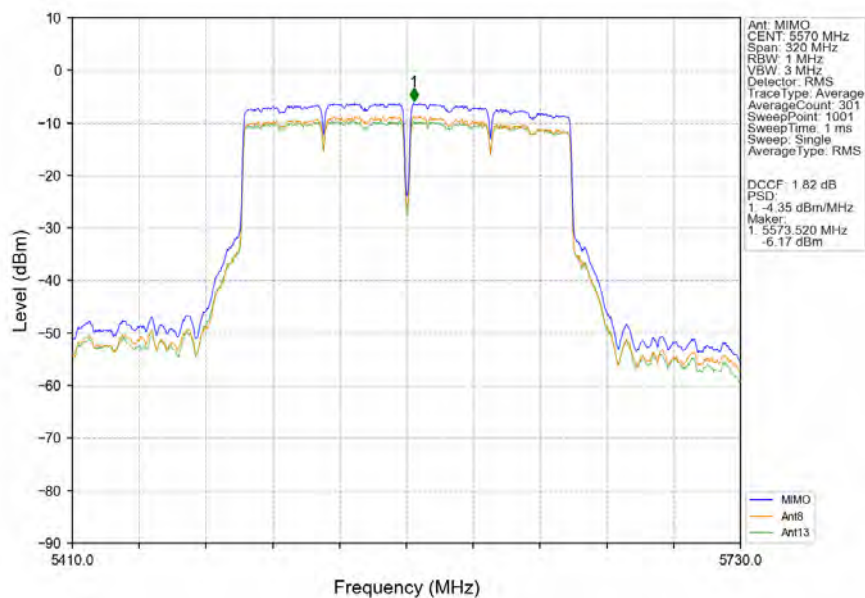
802.11ac(VHT160)_MCH_5570MHz_MIMO_NTNV
