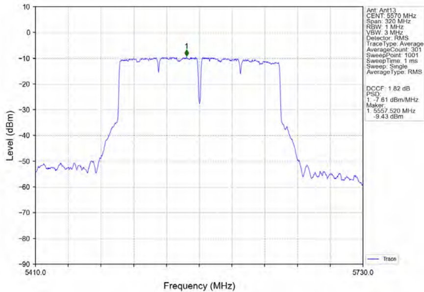
802.11ac(VHT160)_MCH_5570MHz_MIMO_NTNV
