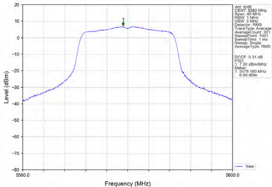
802.11ac(VHT20)_MCH_5580MHz_Ant8_NTNV
