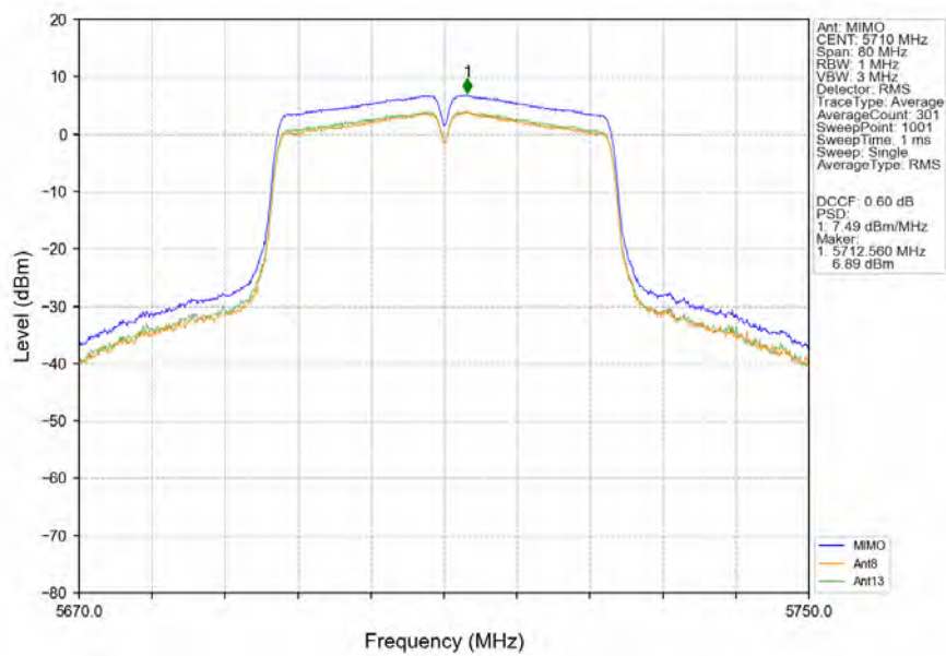
802.11n(HT40)_HCH_5710MHz_MIMO_NTNV
