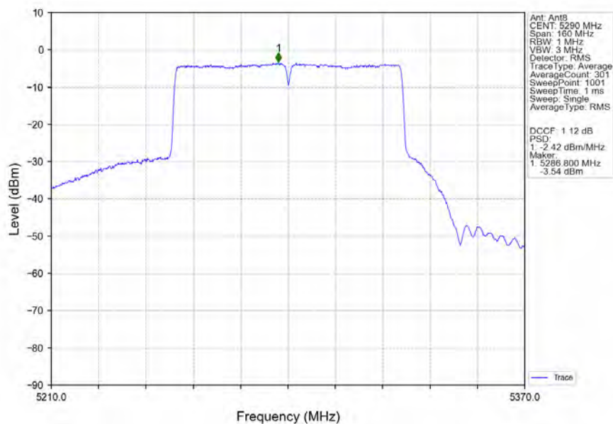
802.11ac(VHT80)_MCH_5290MHz_Ant8_NTNV
