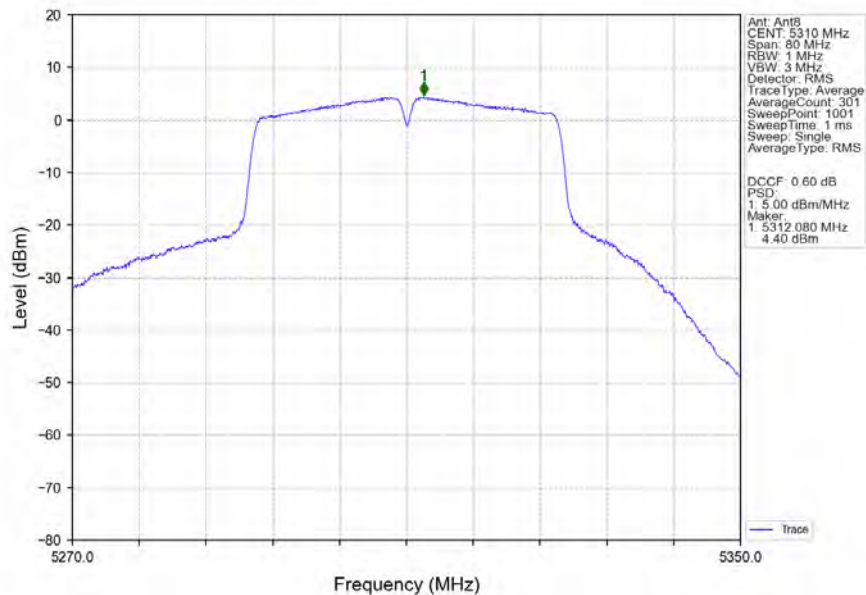
802.11ac(VHT40)_HCH_5310MHz_Ant8_NTNV
