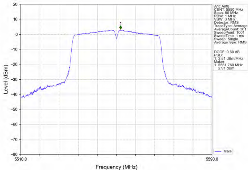
802.11n(HT40)_MCH_5550MHz_Ant8_NTNV
