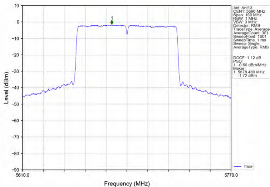
802.11ac(VHT80)_HCH_5690MHz_Ant13_NTNV
