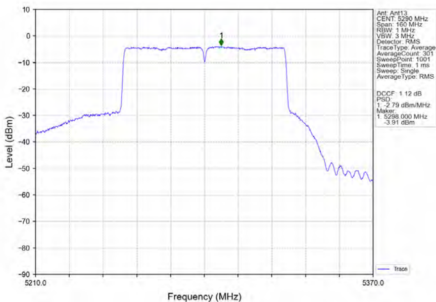
802.11ac(VHT80)_MCH_5290MHz_MIMO_NTNV
