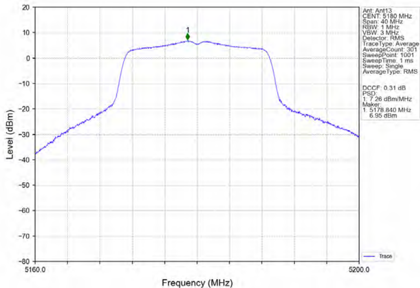
802.11ac(VHT20)_LCH_5180MHz_Ant13_NTNV
