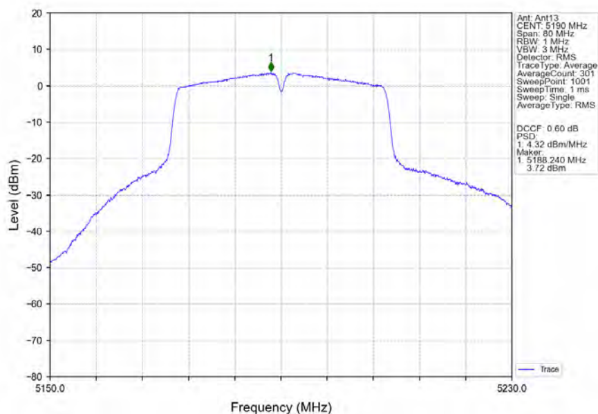
802.11ac(VHT40)_LCH_5190MHz_Ant13_NTNV
