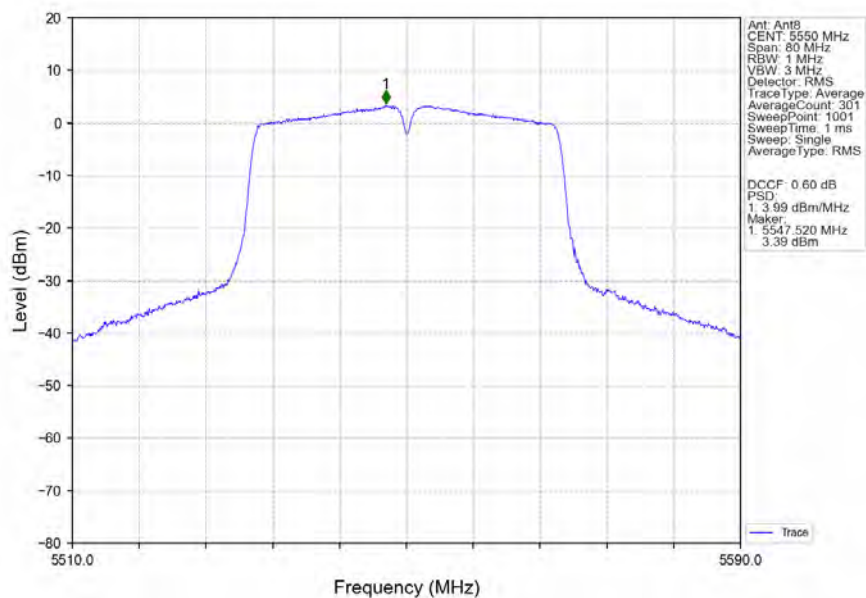
802.11ac(VHT40)_MCH_5550MHz_Ant8_NTNV
