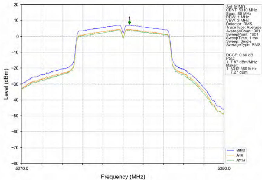
802.11n(HT40)_HCH_5310MHz_MIMO_NTNV
