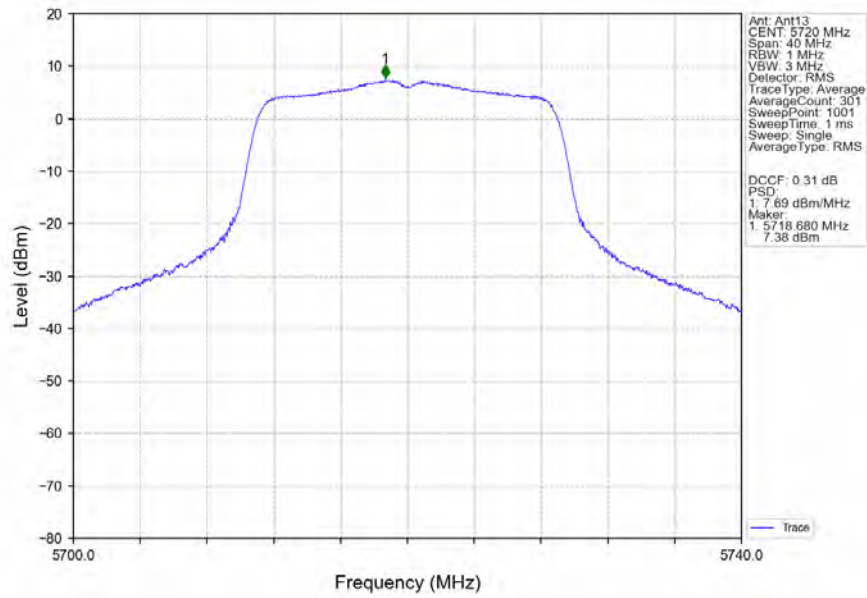
802.11ac(VHT20)_HCH_5720MHz_MIMO_NTNV
