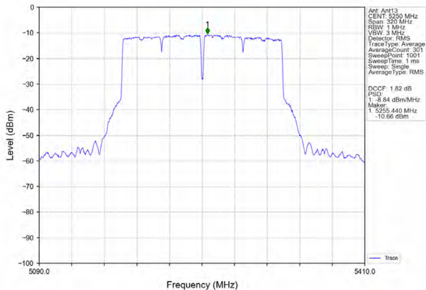
802.11ac(VHT160)_MCH_5250MHz_Ant13_NTNV
