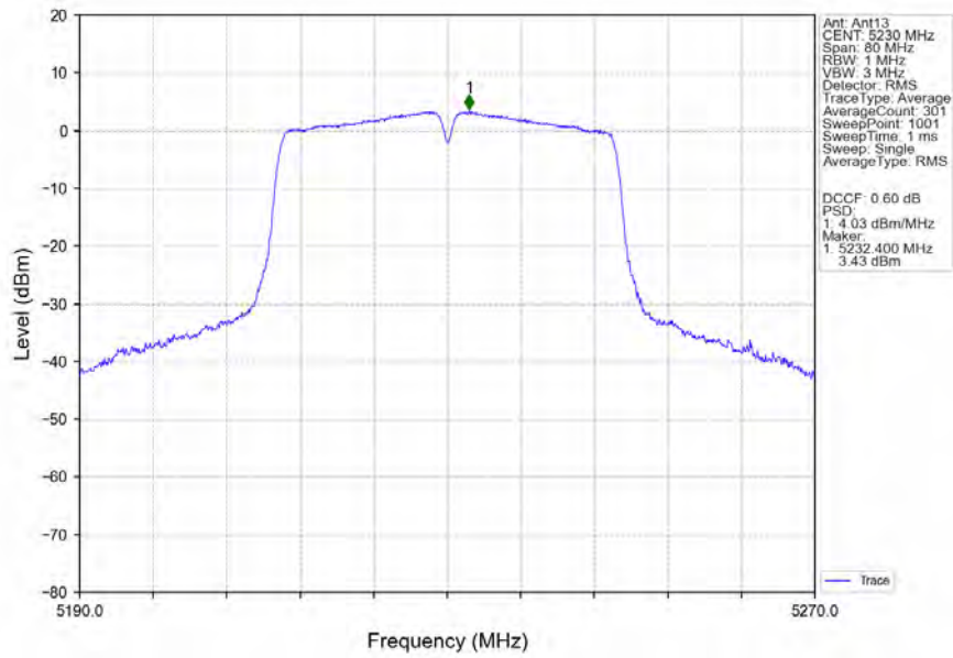
802.11n(HT40)_HCH_5230MHz_MIMO_NTNV
