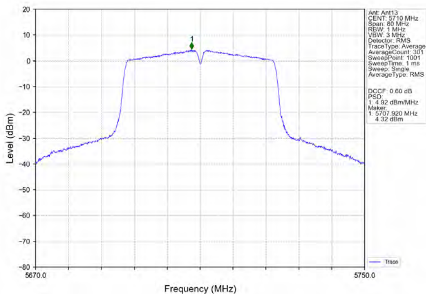
802.11ac(VHT40)_HCH_5710MHz_MIMO_NTNV
