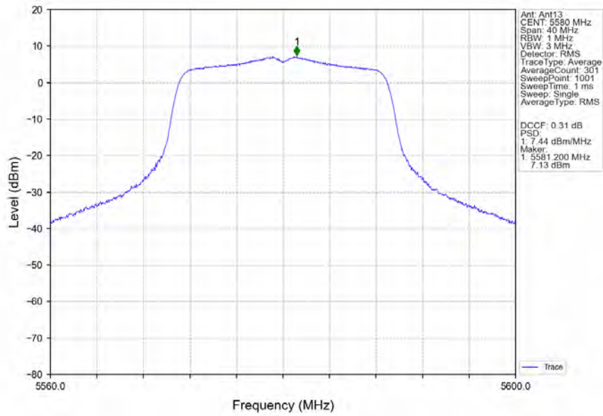
802.11ac(VHT20)_MCH_5580MHz_MIMO_NTNV
