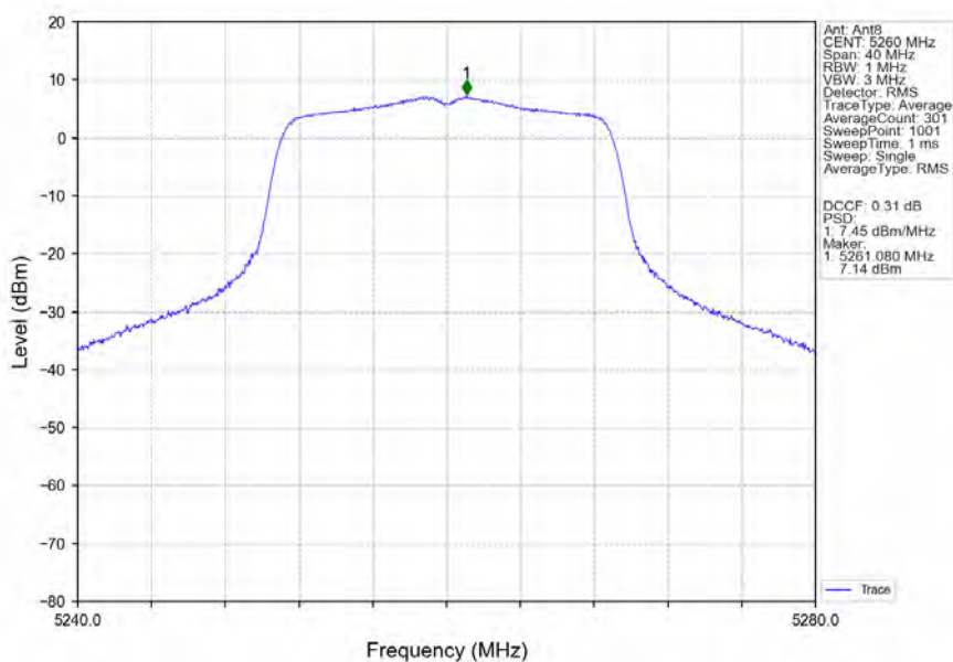
802.11ac(VHT20)_LCH_5260MHz_Ant8_NTNV
