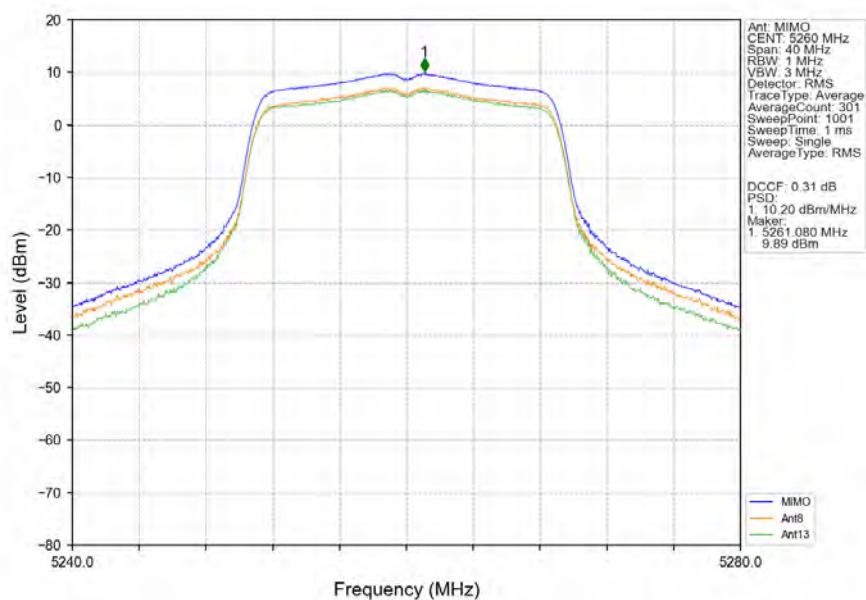
802.11ac(VHT20)_LCH_5260MHz_MIMO_NTNV
