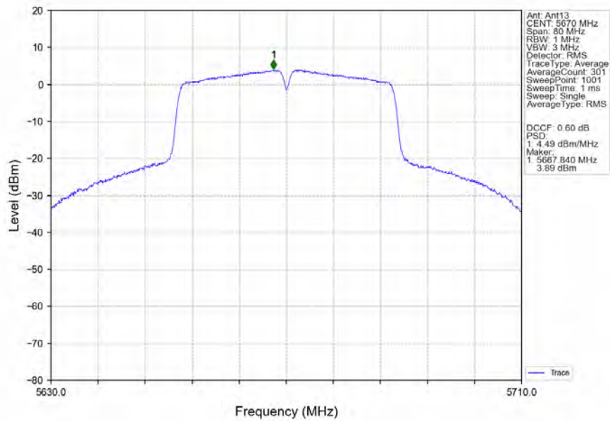
802.11ac(VHT40)_HCH_5670MHz_Ant13_NTNV
