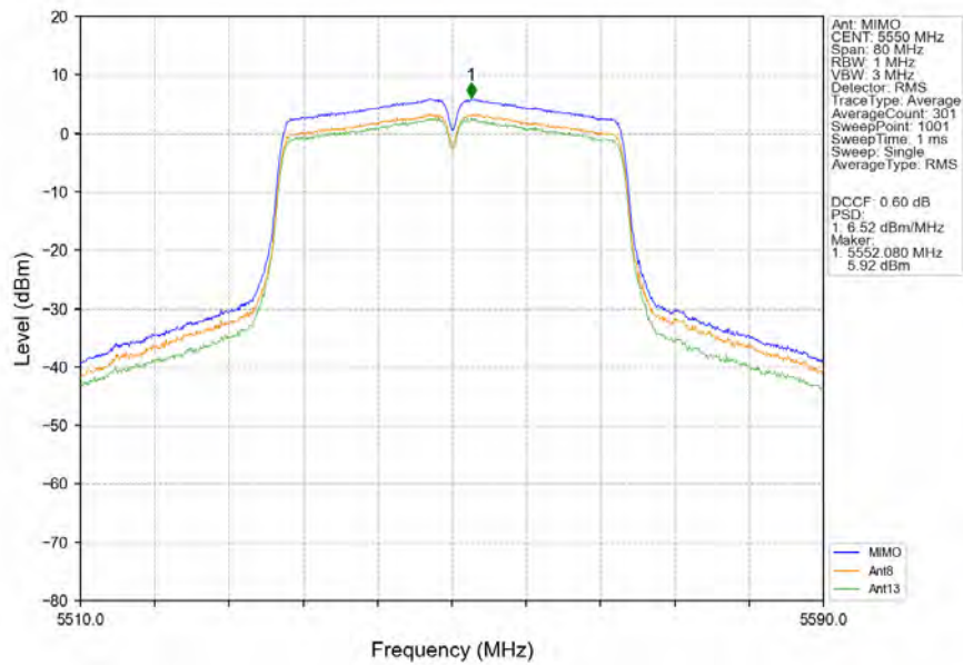
802.11ac(VHT40)_MCH_5550MHz_MIMO_NTNV
