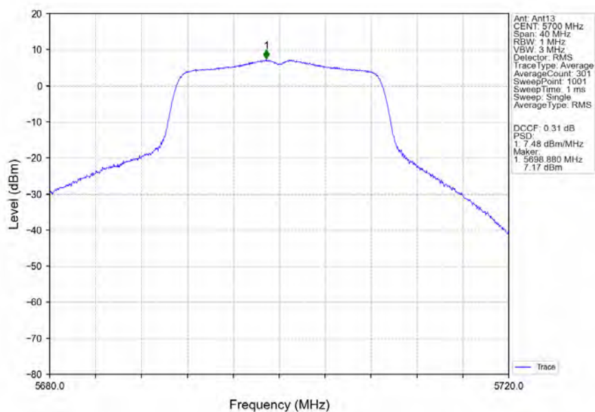
802.11ac(VHT20)_HCH_5700MHz_Ant13_NTNV
