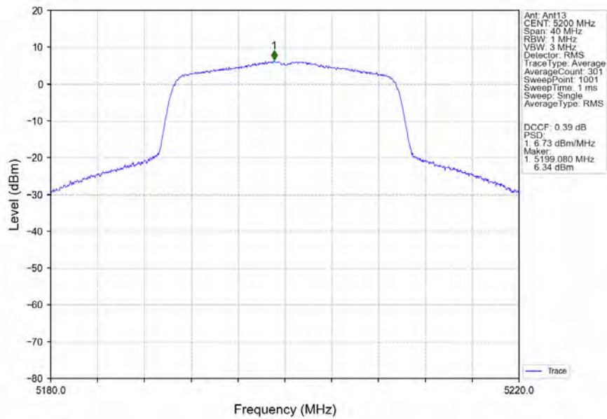
802.11ax(HEW20)_MCH_5200MHz_RU242_Left_Ant13_NTNV
