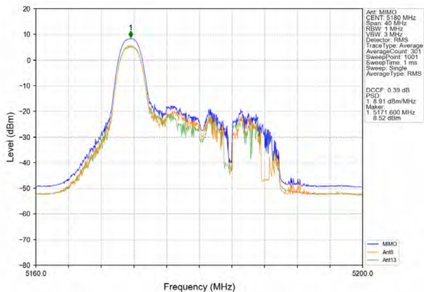
802.11ax(HEW20)_LCH_5180MHz_RU26_Left_MIMO_NTNV
