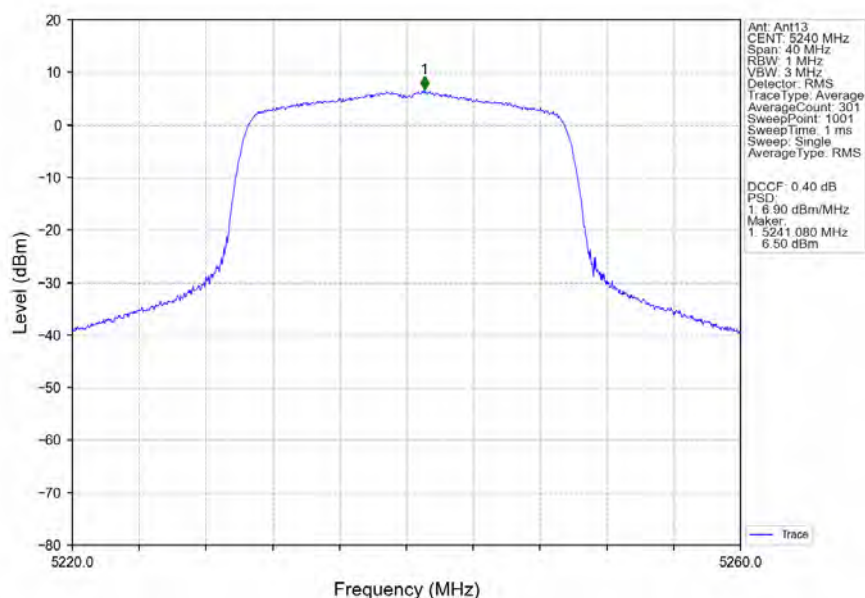
802.11ax(HEW20)_HCH_5240MHz_RU242_Left_Ant13_NTNV
