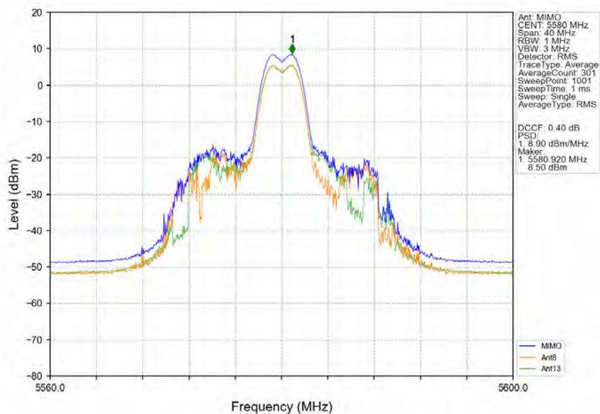
802.11ax(HEW20)_MCH_5580MHz_RU26_Mid_MIMO_NTNV
