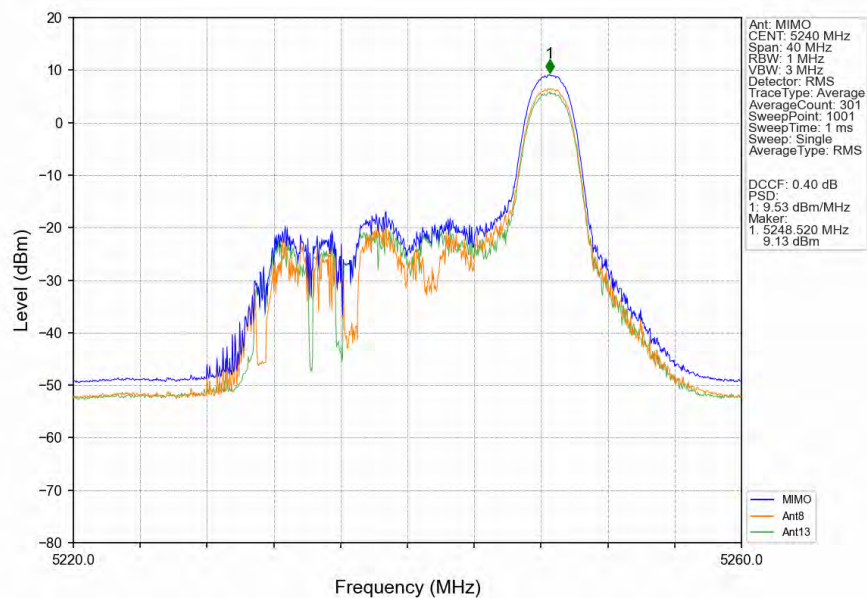
802.11ax(HEW20)_HCH_5240MHz_RU26_Right_MIMO_NTNV
