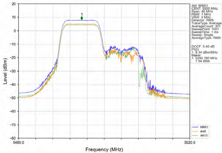
802.11ax(HEW20)_LCH_5500MHz_RU106_Left_MIMO_NTNV
