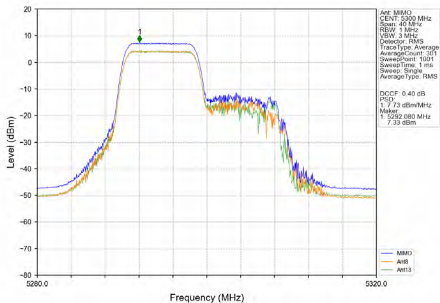
802.11ax(HEW20)_MCH_5300MHz_RU106_Left_MIMO_NTNV
