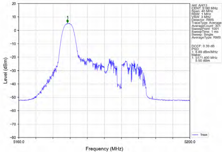
802.11ax(HEW20)_LCH_5180MHz_RU26_Left_MIMO_NTNV
