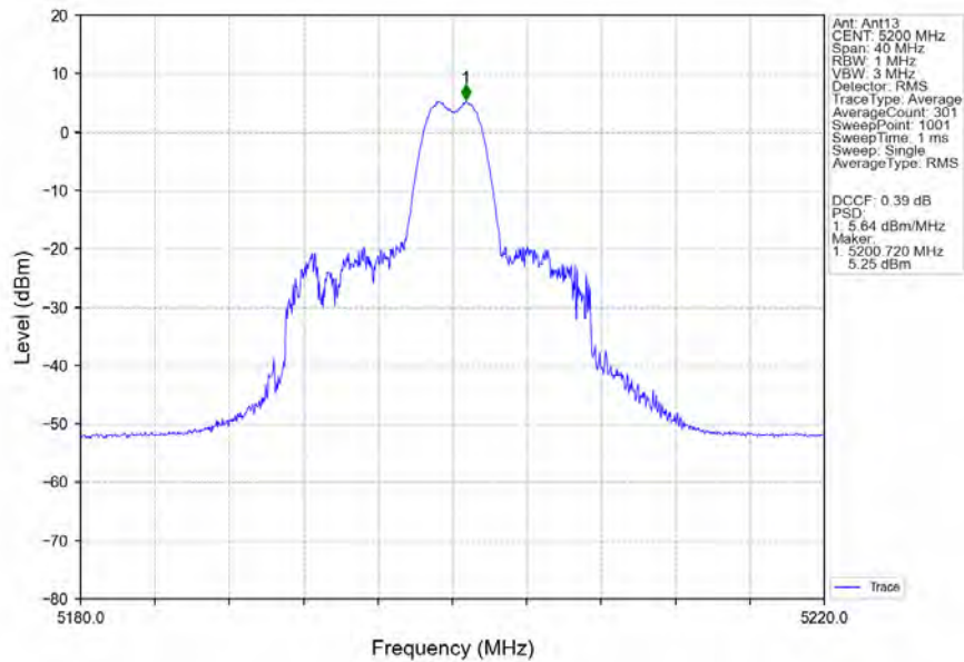
802.11ax(HEW20)_MCH_5200MHz_RU26_Mid_MIMO_NTNV
