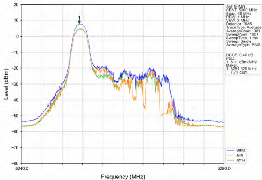
802.11ax(HEW20)_LCH_5260MHz_RU26_Left_MIMO_NTNV
