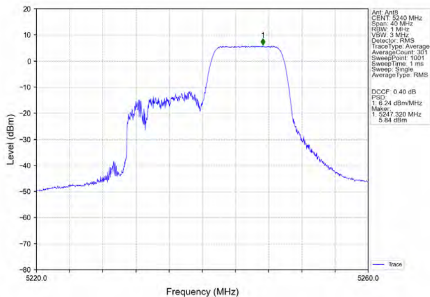
802.11ax(HEW20)_HCH_5240MHz_RU106_Right_Ant8_NTNV
