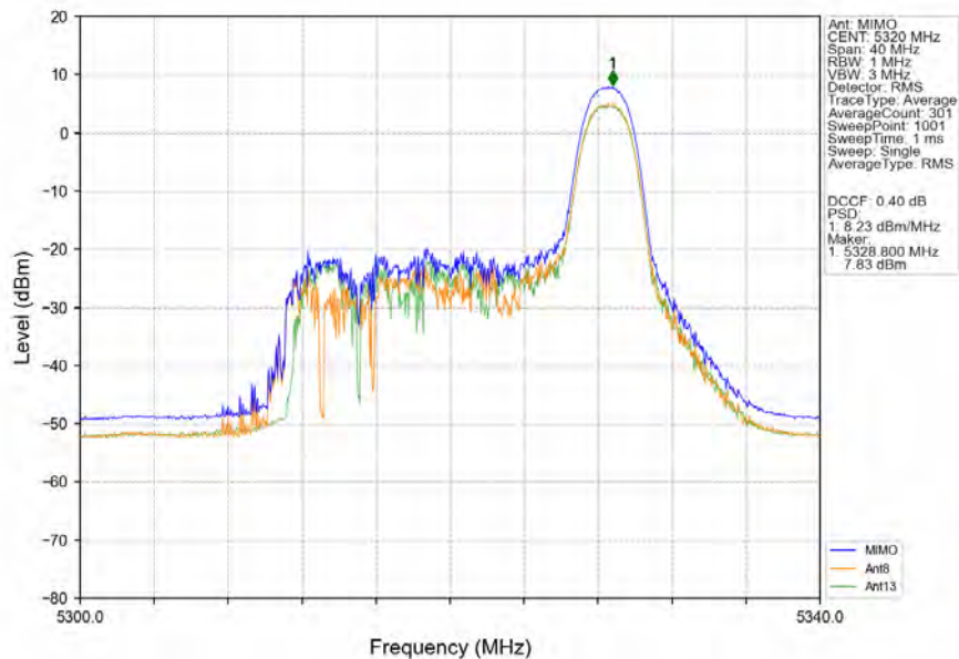
802.11ax(HEW20)_HCH_5320MHz_RU26_Right_MIMO_NTNV
