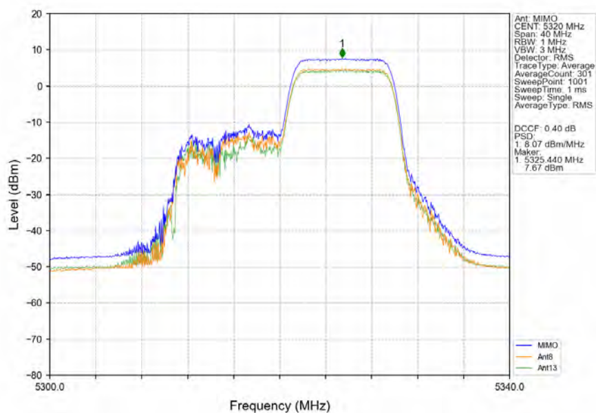
802.11ax(HEW20)_HCH_5320MHz_RU106_Right_MIMO_NTNV
