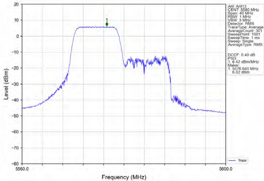
802.11ax(HEW20)_MCH_5580MHz_RU106_Left_MIMO_NTNV
