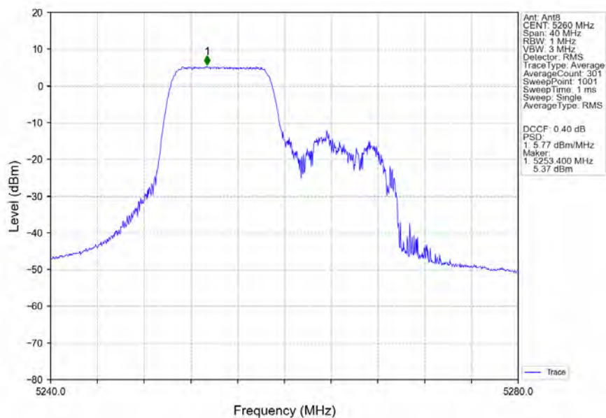
802.11ax(HEW20)_LCH_5260MHz_RU106_Left_Ant8_NTNV
