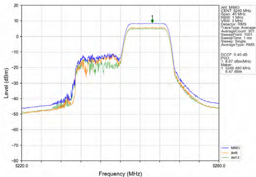
802.11ax(HEW20)_HCH_5240MHz_RU106_Right_MIMO_NTNV
