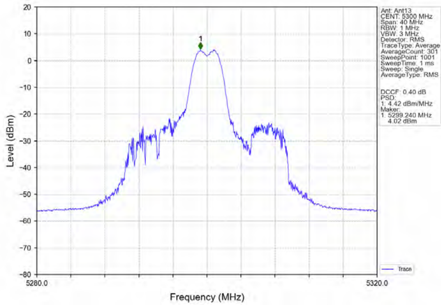
802.11ax(HEW20)_MCH_5300MHz_RU26_Mid_MIMO_NTNV
