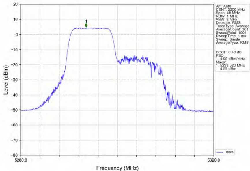
802.11ax(HEW20)_MCH_5300MHz_RU106_Left_Ant8_NTNV
