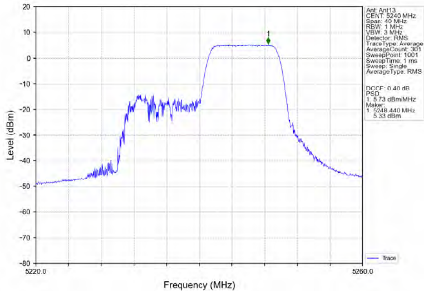
802.11ax(HEW20)_HCH_5240MHz_RU106_Right_MIMO_NTNV
