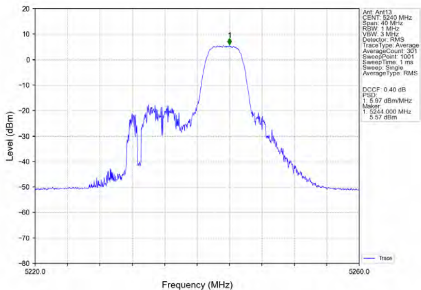
802.11ax(HEW20)_HCH_5240MHz_RU52_Right_Ant13_NTNV
