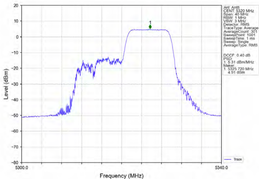
802.11ax(HEW20)_HCH_5320MHz_RU106_Right_Ant8_NTNV
