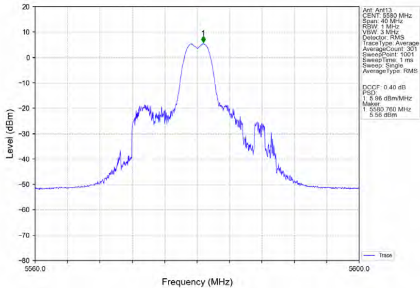
802.11ax(HEW20)_MCH_5580MHz_RU26_Mid_MIMO_NTNV
