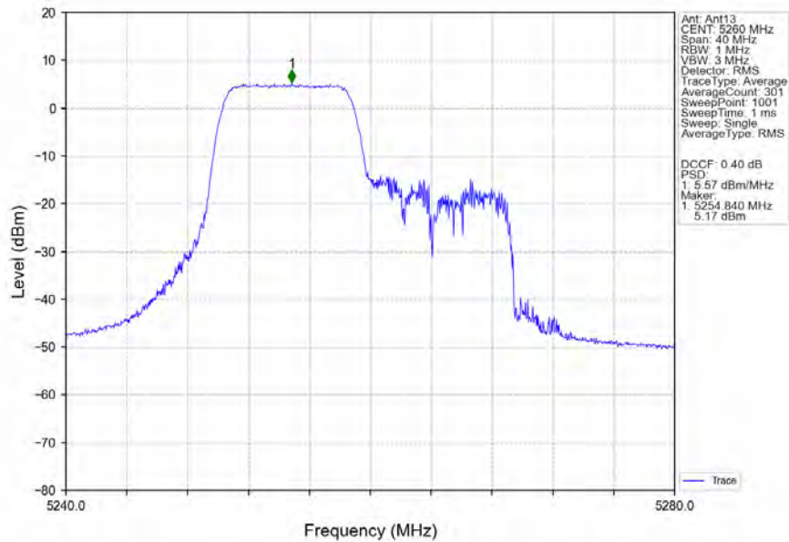
802.11ax(HEW20)_LCH_5260MHz_RU106_Left_MIMO_NTNV
