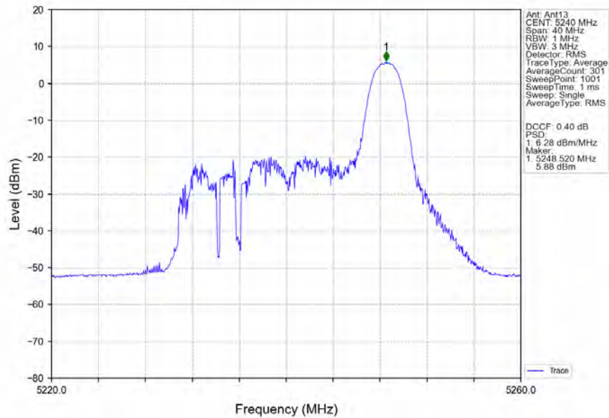
802.11ax(HEW20)_HCH_5240MHz_RU26_Right_MIMO_NTNV
