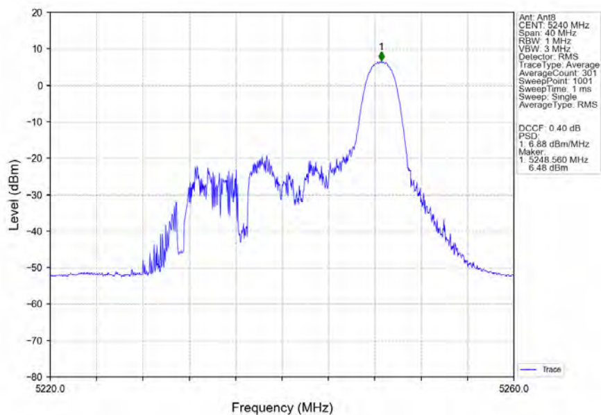
802.11ax(HEW20)_HCH_5240MHz_RU26_Right_Ant8_NTNV
