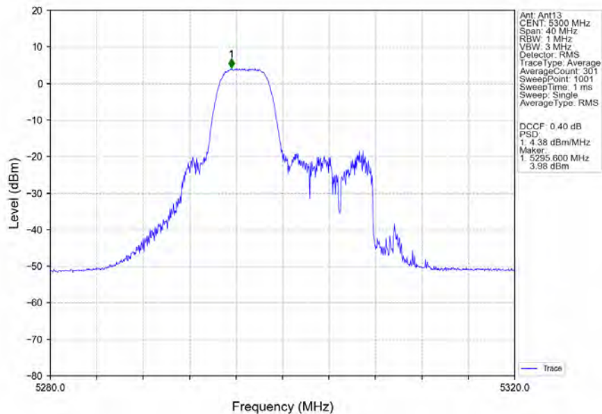
802.11ax(HEW20)_MCH_5300MHz_RU52_Mid_Ant13_NTNV
