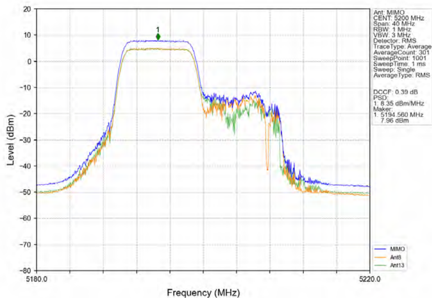
802.11ax(HEW20)_MCH_5200MHz_RU106_Left_MIMO_NTNV
