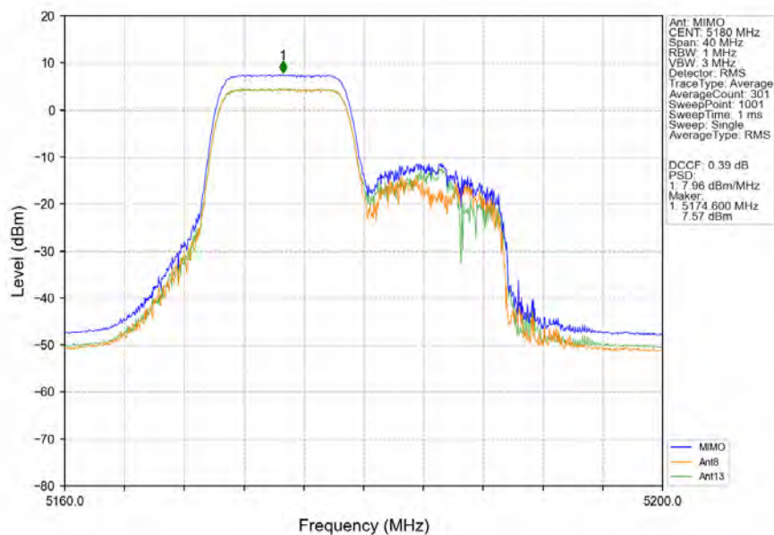
802.11ax(HEW20)_LCH_5180MHz_RU106_Left_MIMO_NTNV
