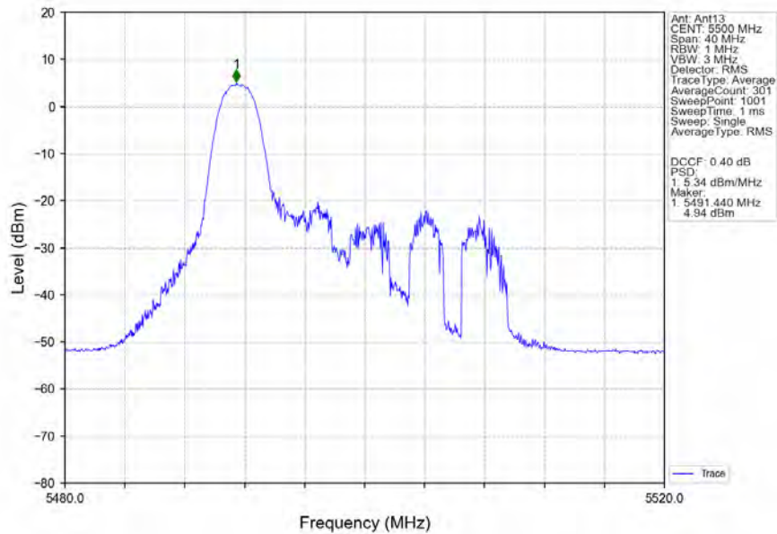
802.11ax(HEW20)_LCH_5500MHz_RU26_Left_MIMO_NTNV
