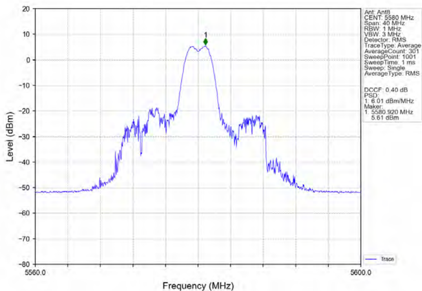
802.11ax(HEW20)_MCH_5580MHz_RU26_Mid_Ant8_NTNV
