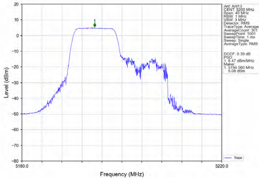
802.11ax(HEW20)_MCH_5200MHz_RU106_Left_MIMO_NTNV
