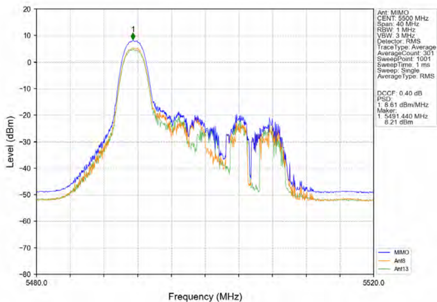
802.11ax(HEW20)_LCH_5500MHz_RU26_Left_MIMO_NTNV
