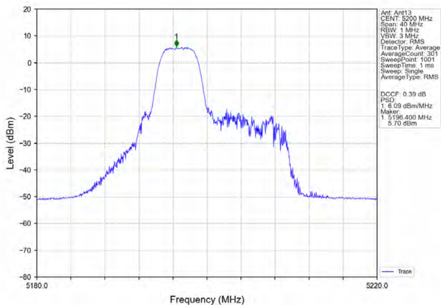
802.11ax(HEW20)_MCH_5200MHz_RU52_Mid_Ant13_NTNV
