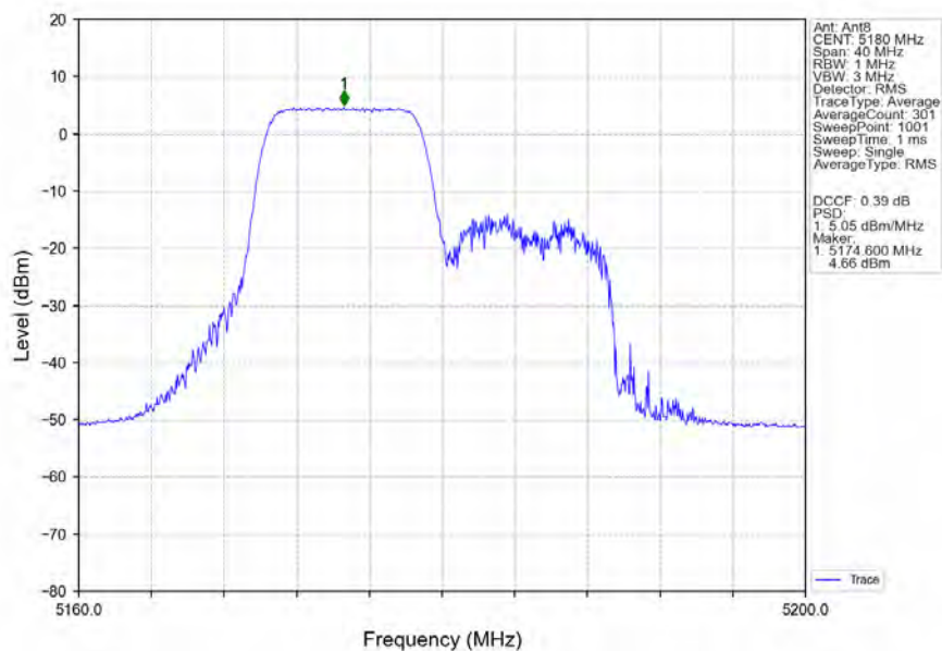
802.11ax(HEW20)_LCH_5180MHz_RU106_Left_Ant8_NTNV
