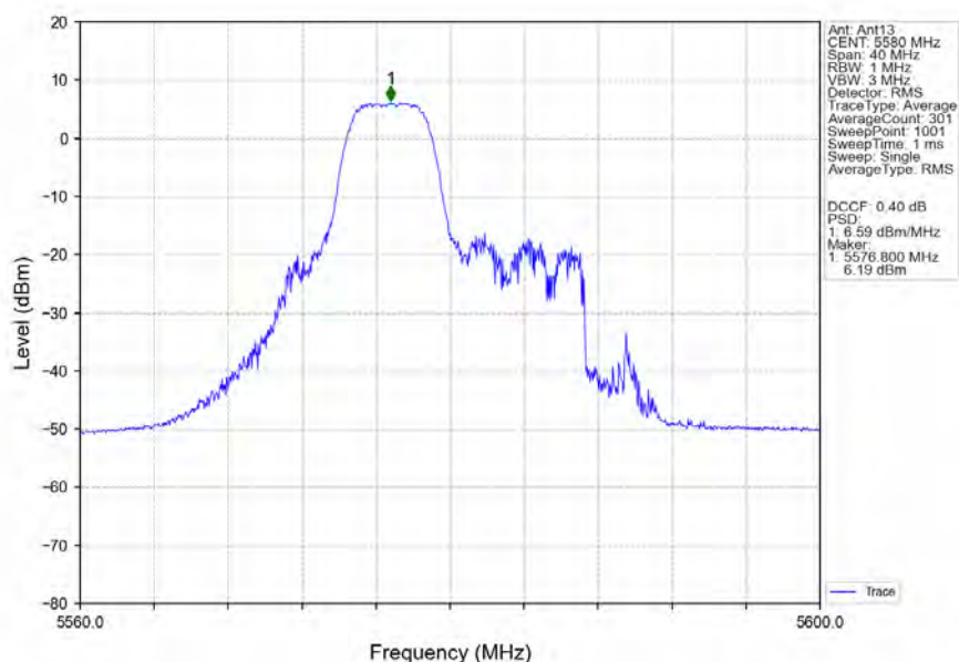
802.11ax(HEW20)_MCH_5580MHz_RU52_Mid_Ant13_NTNV
