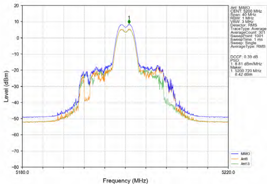
802.11ax(HEW20)_MCH_5200MHz_RU26_Mid_MIMO_NTNV
