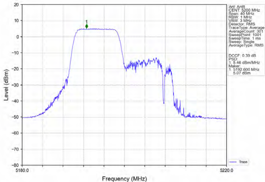
802.11ax(HEW20)_MCH_5200MHz_RU106_Left_Ant8_NTNV
