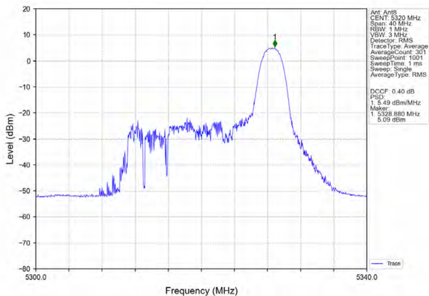
802.11ax(HEW20)_HCH_5320MHz_RU26_Right_Ant8_NTNV
