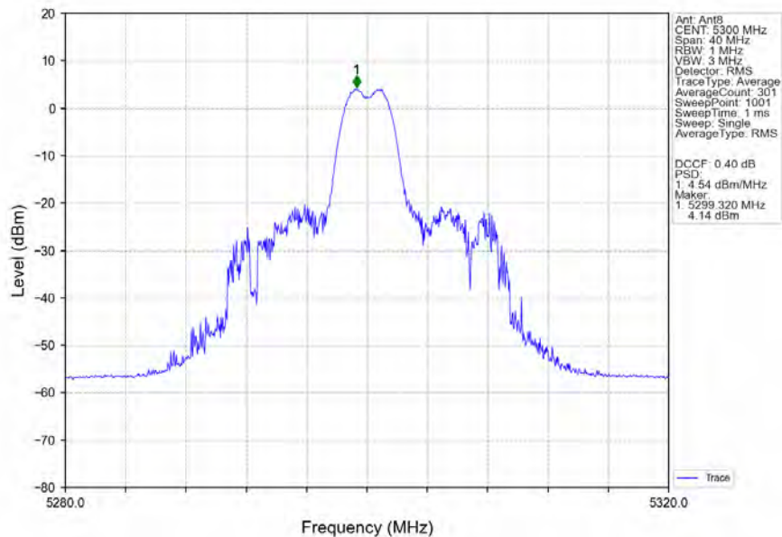
802.11ax(HEW20)_MCH_5300MHz_RU26_Mid_Ant8_NTNV
