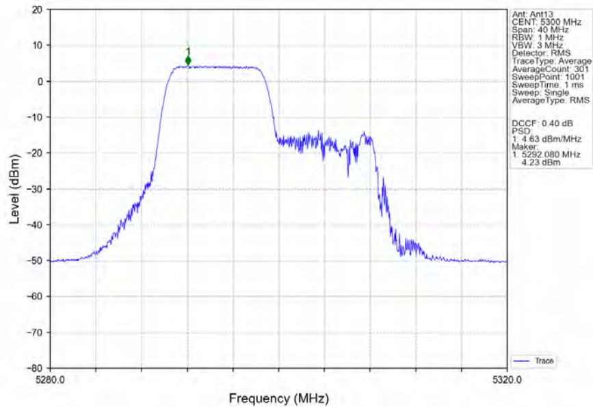
802.11ax(HEW20)_MCH_5300MHz_RU106_Left_MIMO_NTNV
