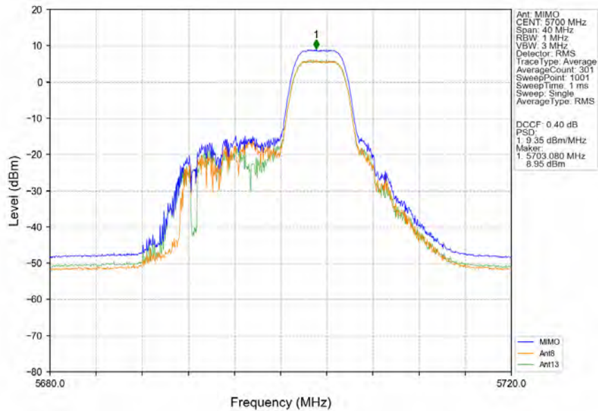
802.11ax(HEW20)_HCH_5700MHz_RU106_Right_Ant8_NTNV
