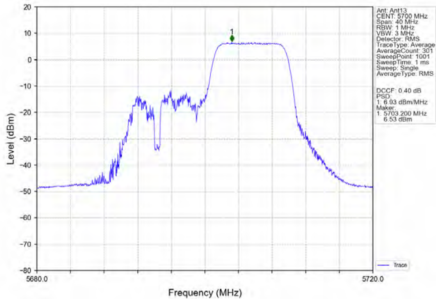
802.11ax(HEW20)_HCH_5700MHz_RU106_Right_MIMO_NTNV
