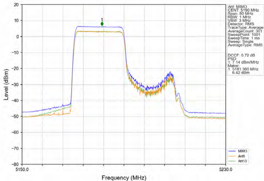
802.11ax(HEW40)_LCH_5190MHz_RU242_Left_MIMO_NTNV
