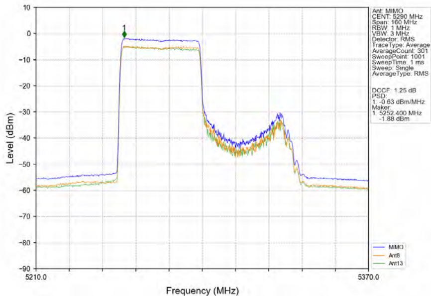
802.11ax(HEW80)_MCH_5290MHz_RU484_Left_MIMO_NTNV
