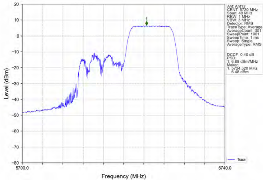
802.11ax(HEW20)_HCH_5720MHz_RU106_Right_MIMO_NTNV
