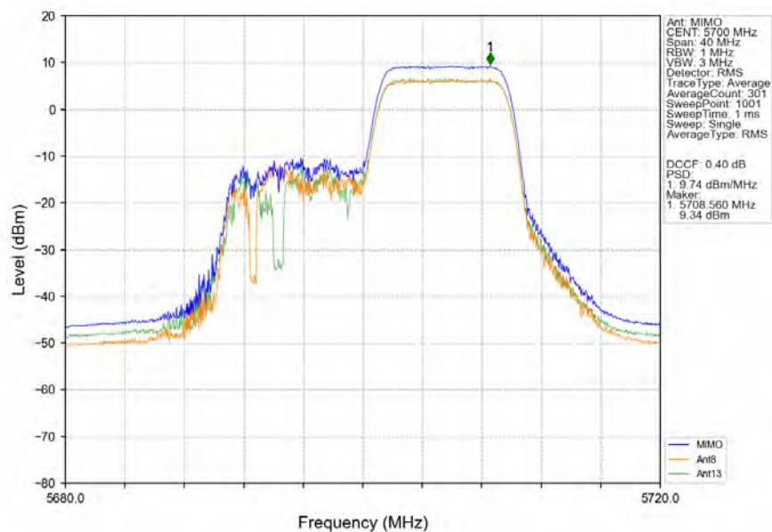
802.11ax(HEW20)_HCH_5700MHz_RU106_Right_MIMO_NTNV
