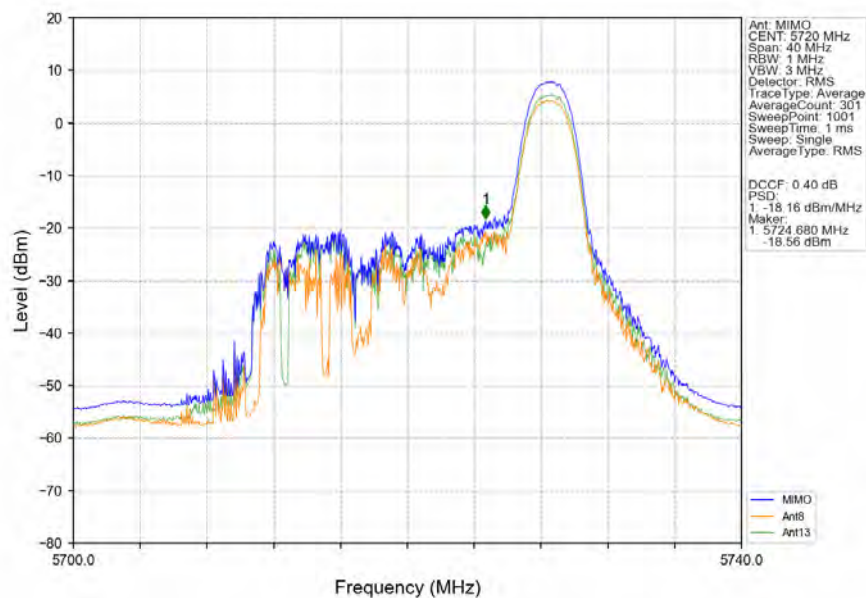
802.11ax(HEW20)_HCH_5720MHz_RU26_Right_MIMO_NTNV
