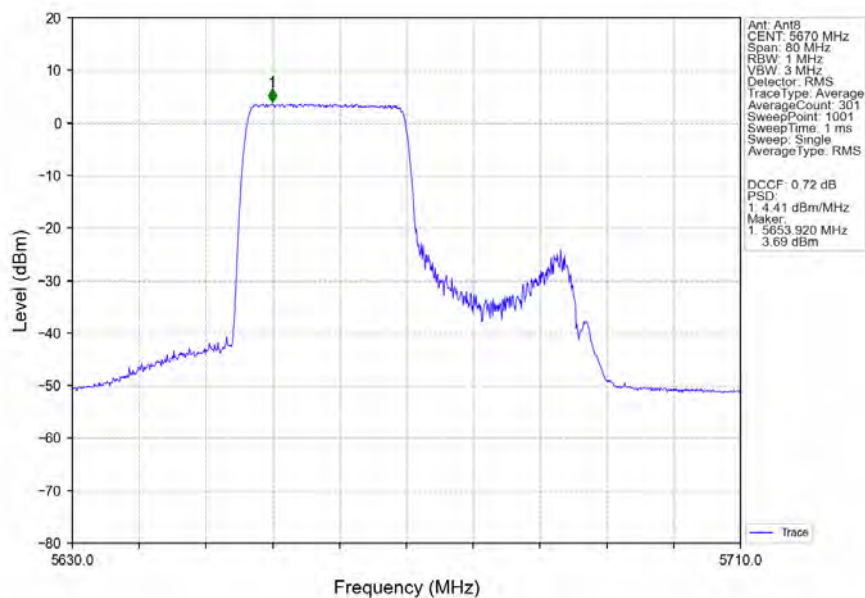
802.11ax(HEW40)_HCH_5670MHz_RU242_Right_Ant8_NTNV
