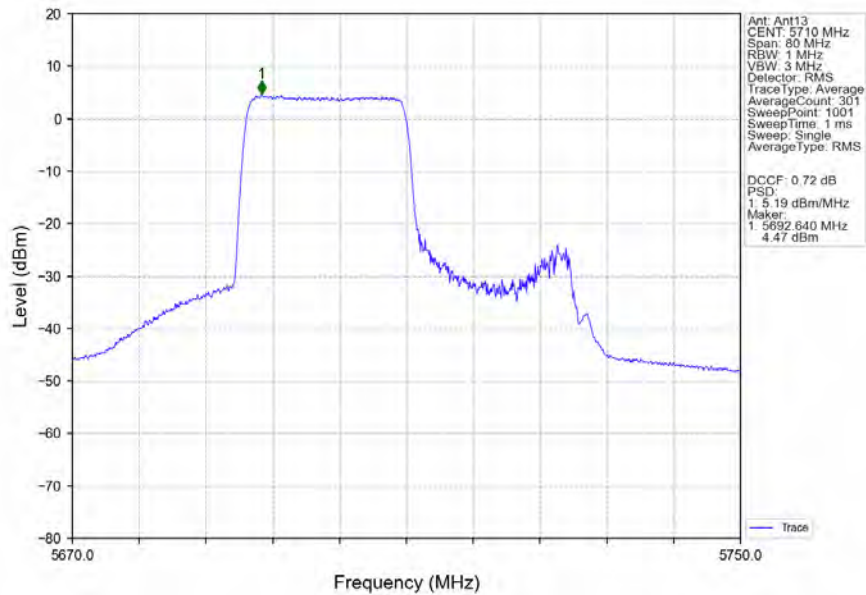
802.11ax(HEW40)_HCH_5710MHz_RU242_Right_MIMO_NTNV
