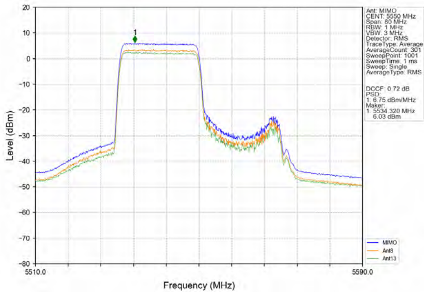
802.11ax(HEW40)_MCH_5550MHz_RU242_Left_MIMO_NTNV
