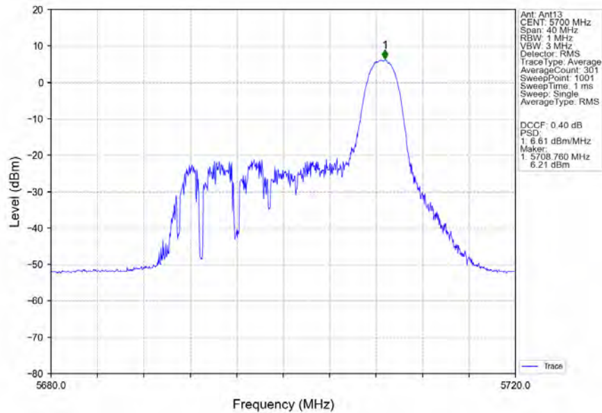
802.11ax(HEW20)_HCH_5700MHz_RU26_Right_MIMO_NTNV
