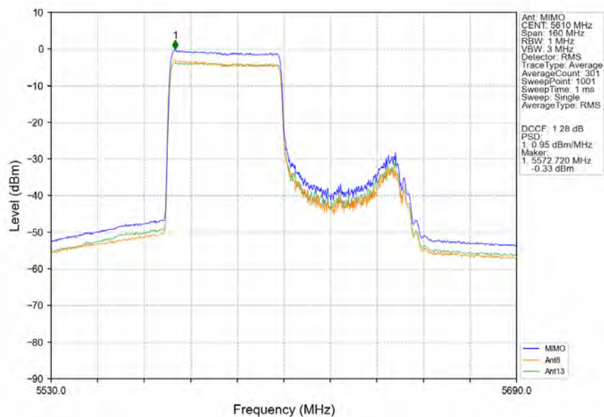
802.11ax(HEW80)_HCH_5610MHz_RU484_Right_MIMO_NTNV
