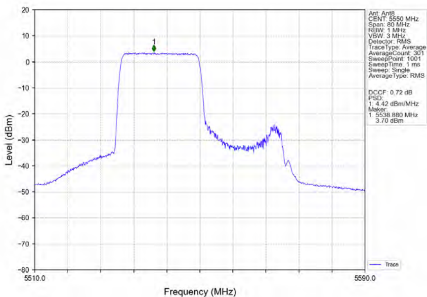
802.11ax(HEW40)_MCH_5550MHz_RU242_Left_Ant8_NTNV
