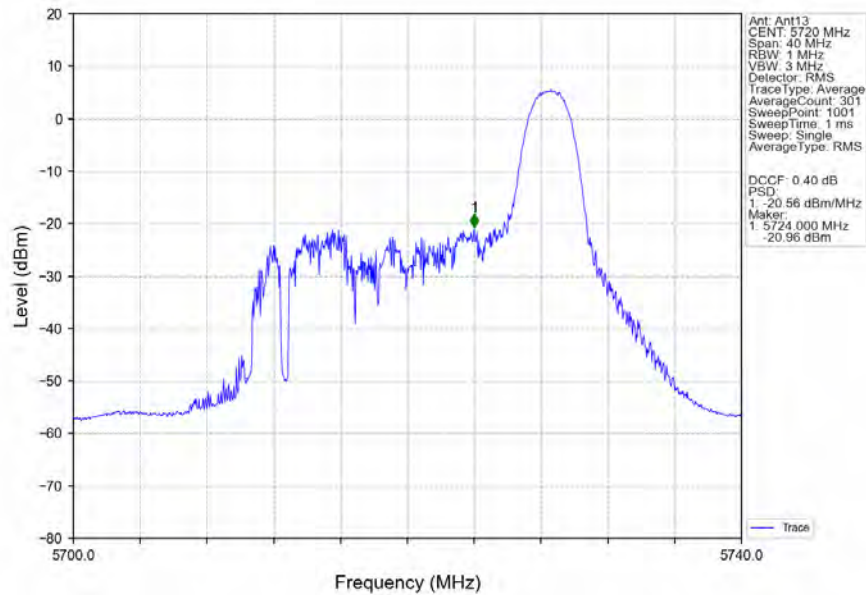
802.11ax(HEW20)_HCH_5720MHz_RU26_Right_MIMO_NTNV
