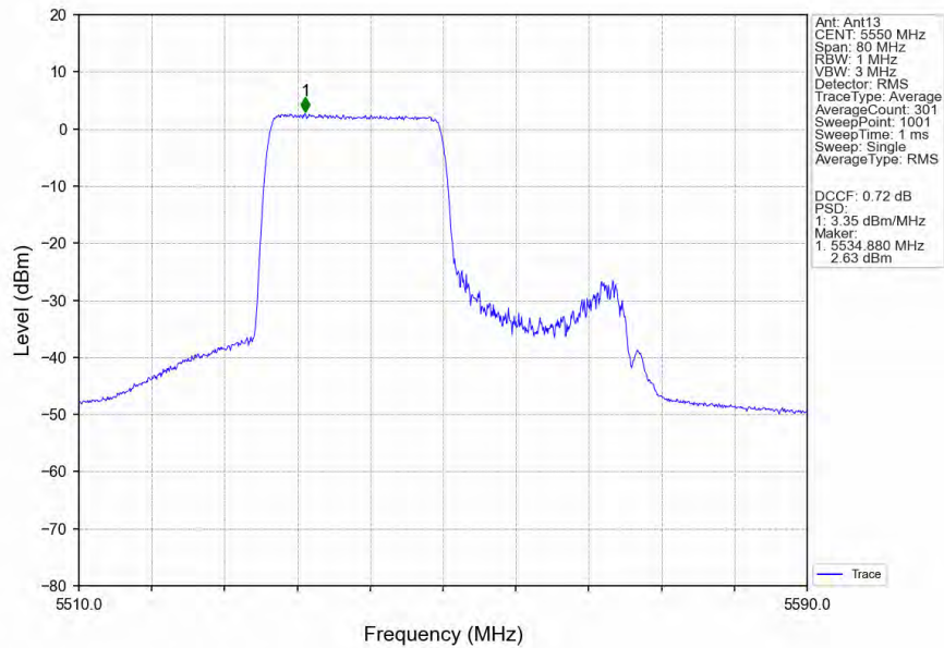
802.11ax(HEW40)_MCH_5550MHz_RU242_Left_MIMO_NTNV
