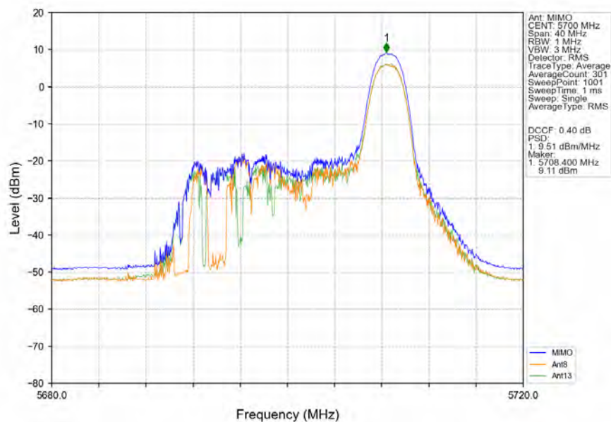
802.11ax(HEW20)_HCH_5700MHz_RU26_Right_MIMO_NTNV
