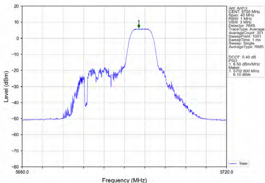
802.11ax(HEW20)_HCH_5700MHz_RU52_Right_Ant13_NTNV
