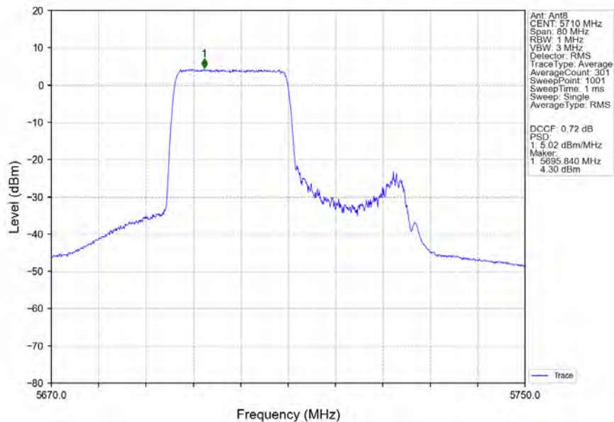
802.11ax(HEW40) HCH 5710MHz RU242 Right Ant8 NTN
