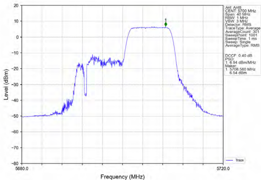
802.11ax(HEW20)_HCH_5700MHz_RU106_Right_Ant8_NTNV
