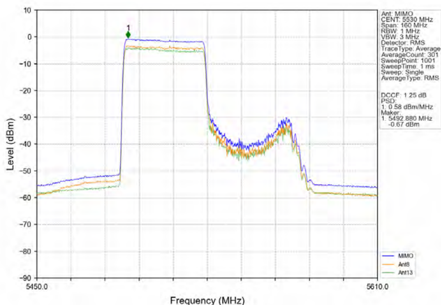
802.11ax(HEW80)_LCH_5530MHz_RU484_Left_MIMO_NTNV
