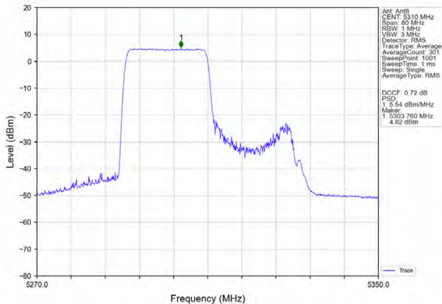
802.11ax(HEW40) HCH 5310MHz RU242 Right Ant8 NTN
