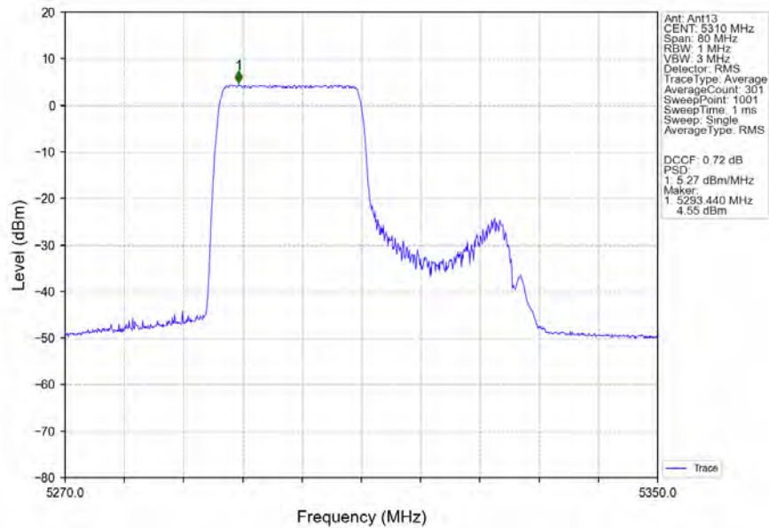
802.11ax(HEW40)_HCH_5310MHz_RU242_Right_MIMO_NTNV
