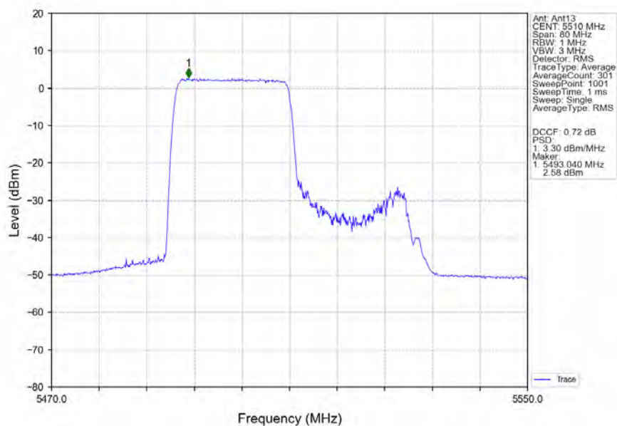
802.11ax(HEW40)_LCH_5510MHz_RU242_Left_MIMO_NTNV
