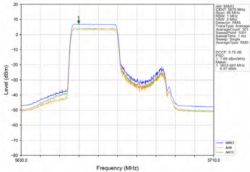
802.11ax(HEW40)_HCH_5670MHz_RU242_Right_MIMO_NTNV
