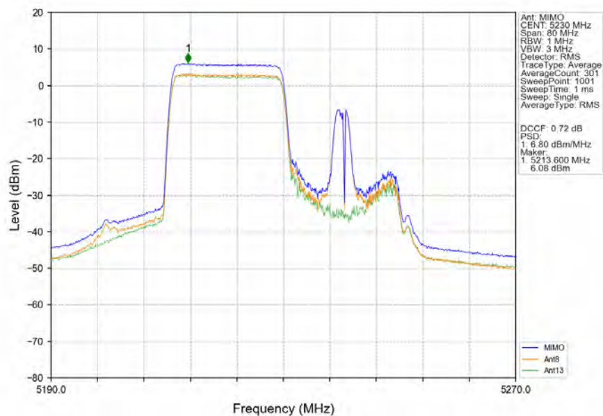
802.11ax(HEW40)_HCH_5230MHz_RU242_Right_MIMO_NTNV
