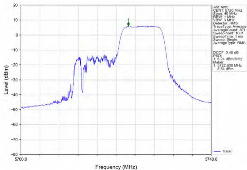
802.11ax(HEW20)_HCH_5720MHz_RU106_Right_Ant8_NTNV
