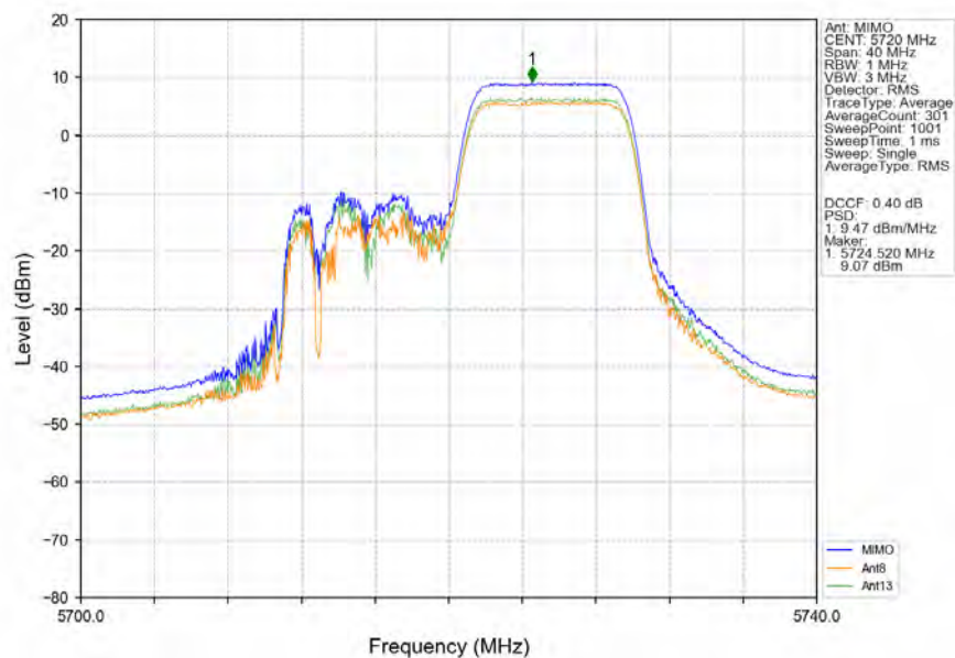
802.11ax(HEW20)_HCH_5720MHz_RU106_Right_MIMO_NTNV
