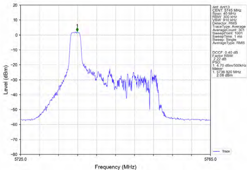
802.11ax(HEW20)_LCH_5745MHz_RU26_Left_Ant13_NTNV
