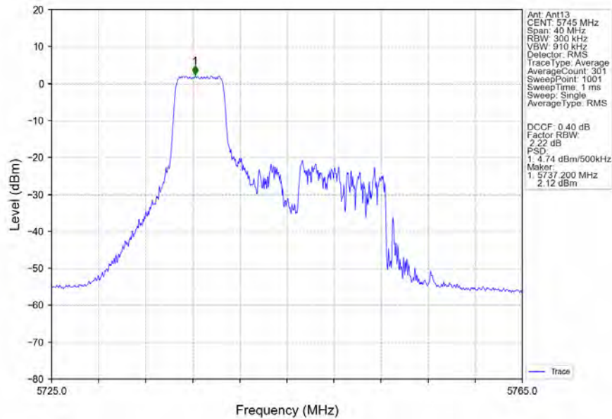
802.11ax(HEW20)_LCH_5745MHz_RU52_Left_MIMO_NTNV
