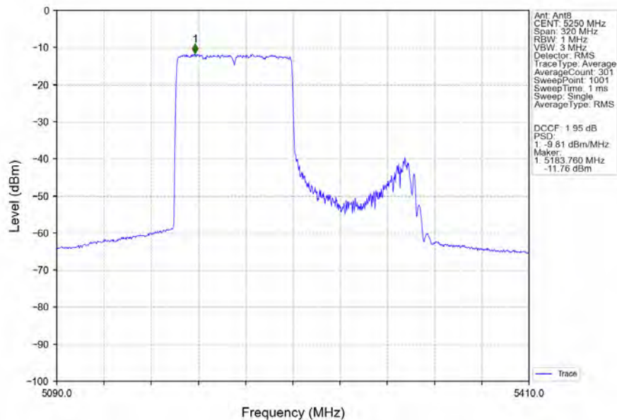
802.11ax(HEW160)_MCH_5250MHz_RU996_Left_Ant8_NTNV
