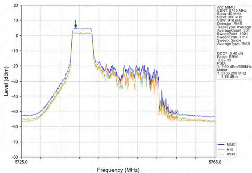
802.11ax(HEW20)_LCH_5745MHz_RU52_Left_MIMO_NTNV
