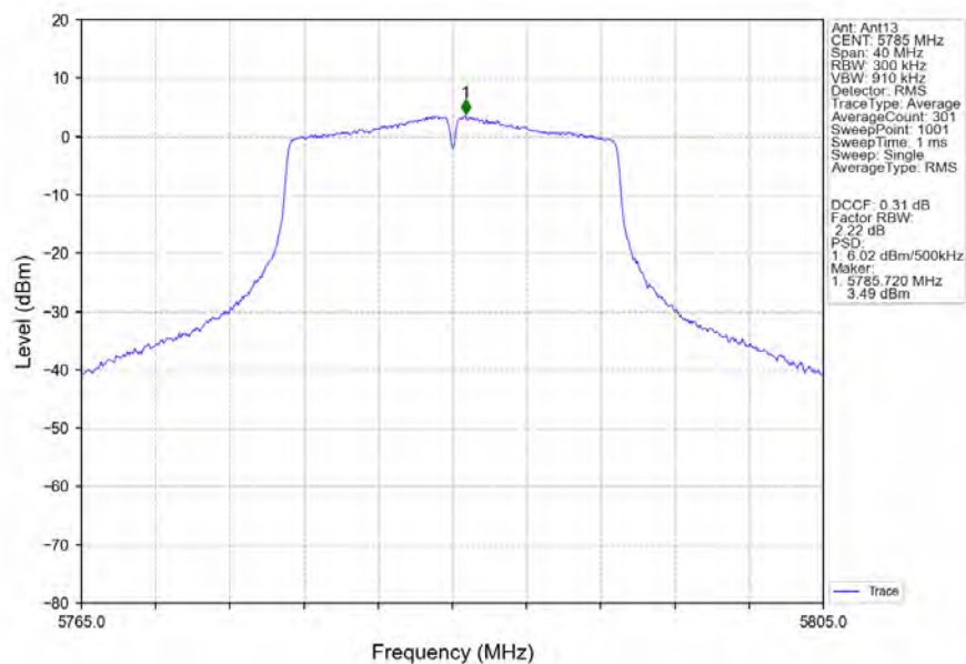
802.11ac(VHT20)_MCH_5785MHz_Ant13_NTNV
