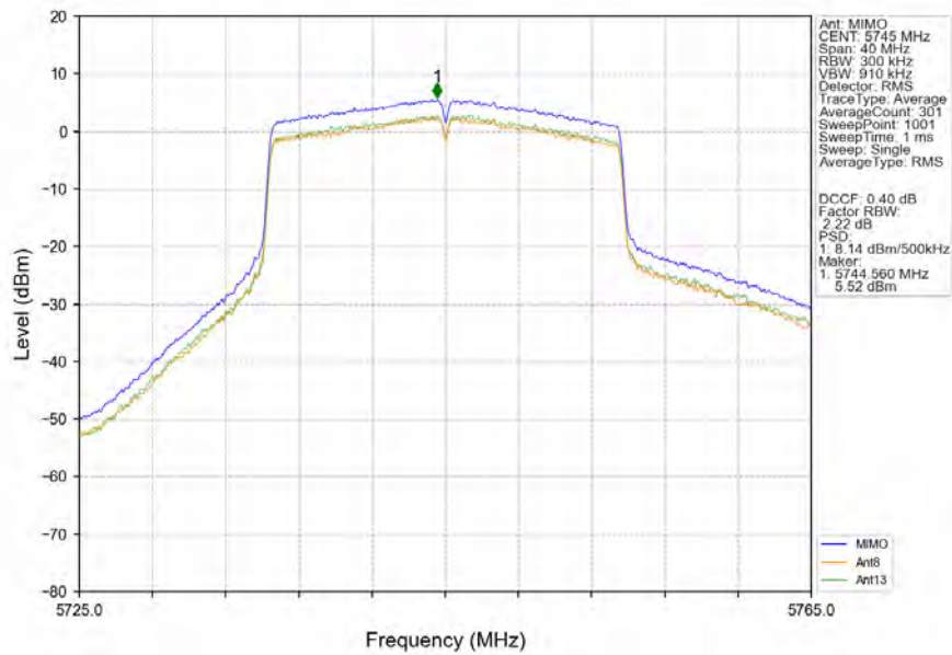
802.11ax(HEW20)_LCH_5745MHz_RU242_Left_MIMO_NTNV
