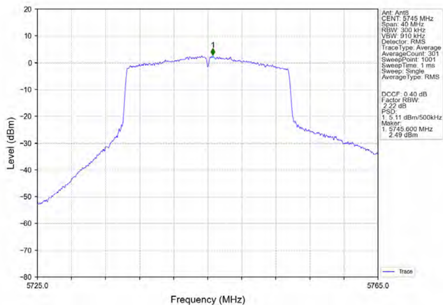
802.11ax(HEW20)_LCH_5745MHz_RU242_Left_Ant8_NTNV
