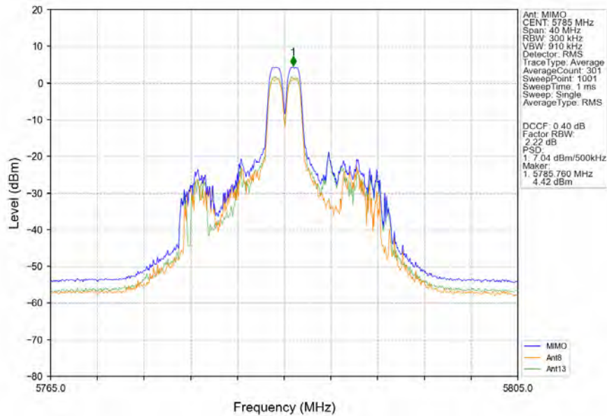
802.11ax(HEW20)_MCH_5785MHz_RU52_Mid_Ant8_NTNV
