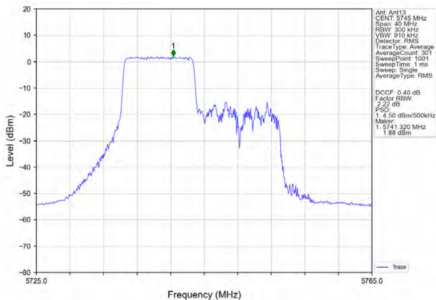
802.11ax(HEW20)_LCH_5745MHz_RU106_Left_Ant13_NTNV
