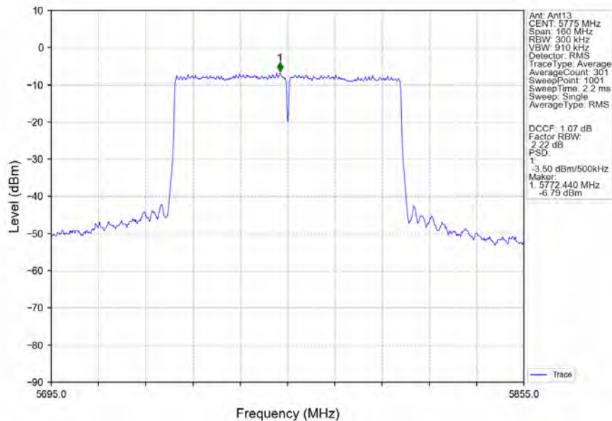
802.11ac(VHT80)_MCH_5775MHz_Ant13_NTNV
