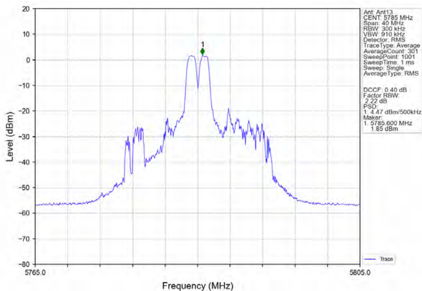
802.11ax(HEW20)_MCH_5785MHz_RU26_Mid_Ant13_NTNV
