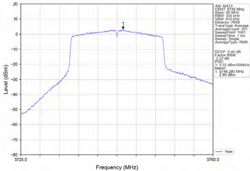
802.11ax(HEW20)_LCH_5745MHz_RU242_Left_MIMO_NTNV
