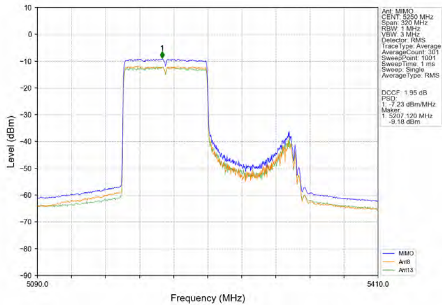
802.11ax(HEW160)_MCH_5250MHz_RU996_Left_MIMO_NTNV
