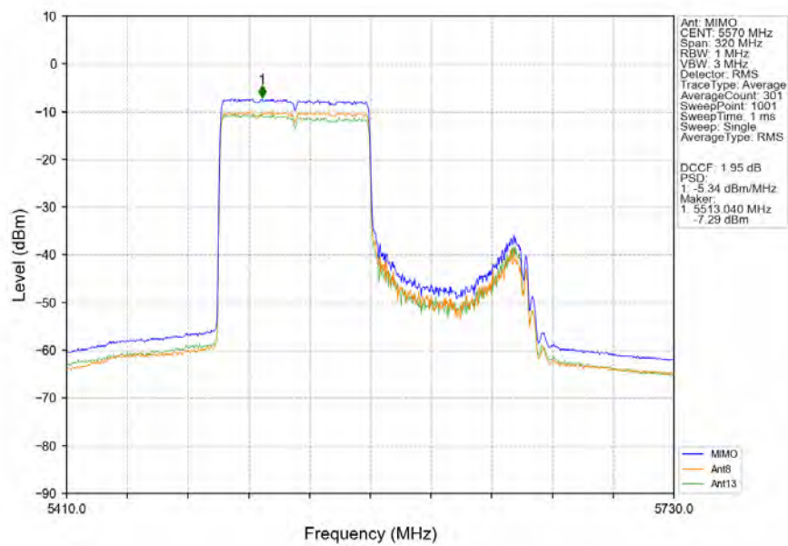
802.11ax(HEW160)_MCH_5570MHz_RU996_Left_MIMO_NTNV
