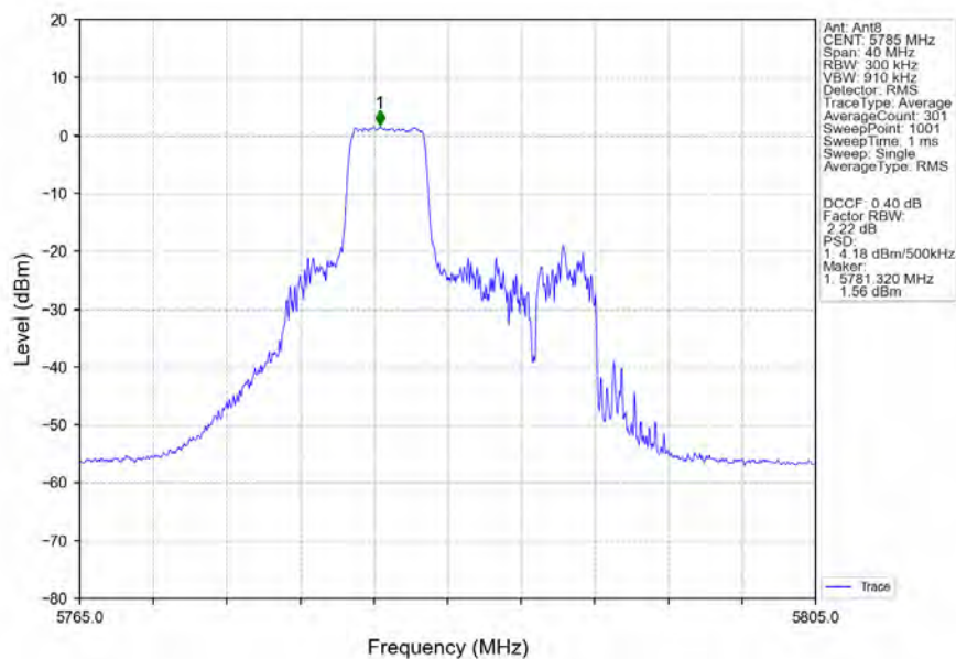
802.11ax(HEW20)_MCH_5785MHz_RU52_Mid_Ant8_NTNV
