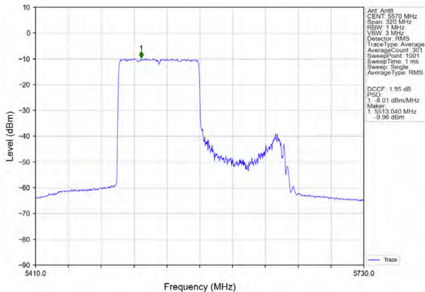
802.11ax(HEW160)_MCH_5570MHz_RU996_Left_Ant8_NTNV
