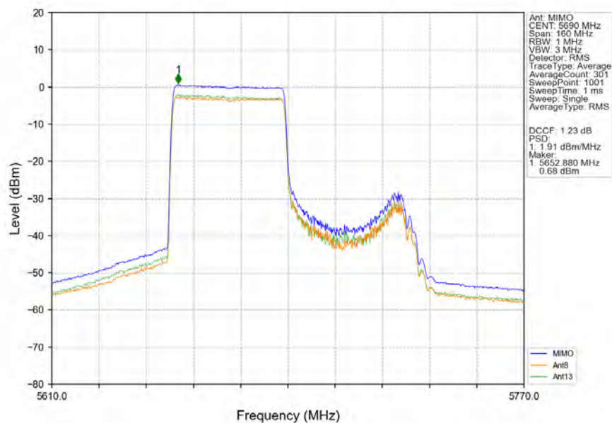
802.11ax(HEW80)_HCH_5690MHz_RU484_Right_MIMO_NTNV
