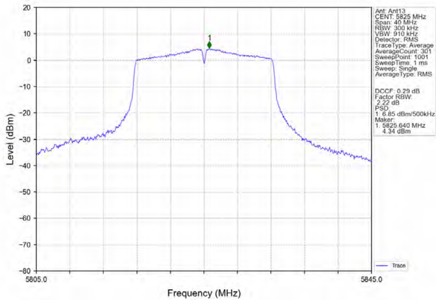
802.11a_HCH_5825MHz_Ant13_NTNV
