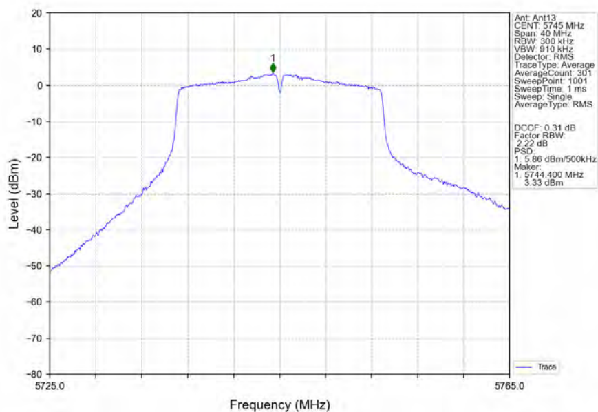
802.11ac(VHT20)_LCH_5745MHz_MIMO_NTNV
