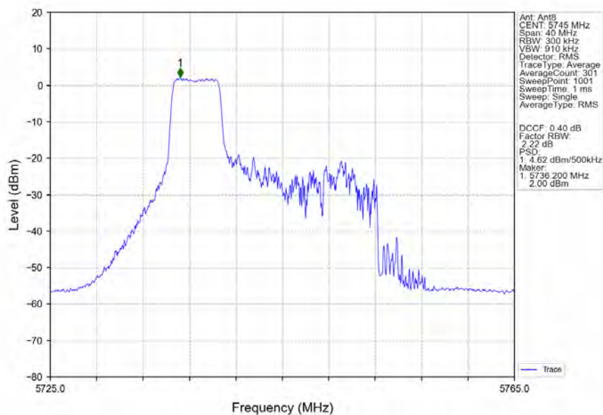
802.11ax(HEW20)_LCH_5745MHz_RU52_Left_Ant8_NTNV
