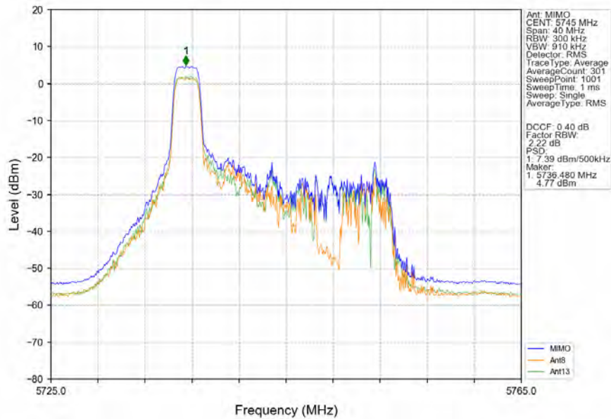
802.11ax(HEW20)_LCH_5745MHz_RU52_Left_Ant8_NTNV
