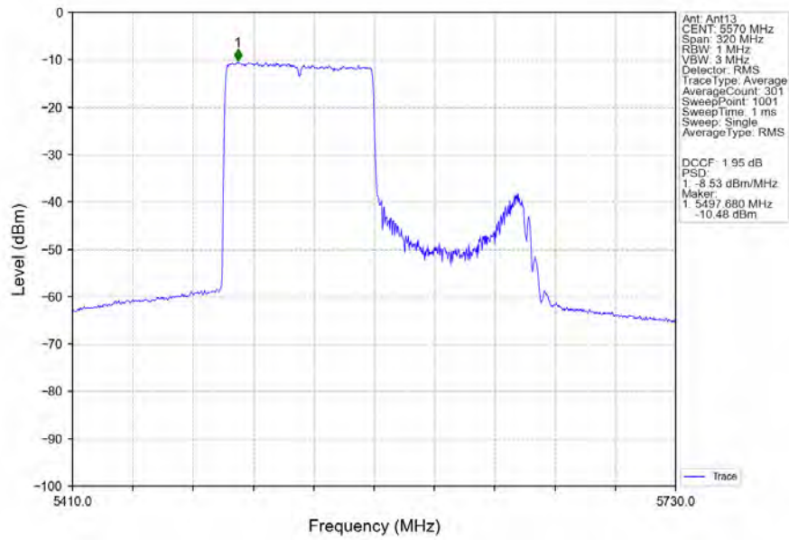
802.11ax(HEW160)_MCH_5570MHz_RU996_Left_MIMO_NTNV
