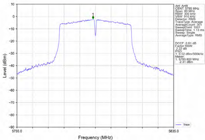
802.11n(HT40)_HCH_5795MHz_Ant8_NTNV
