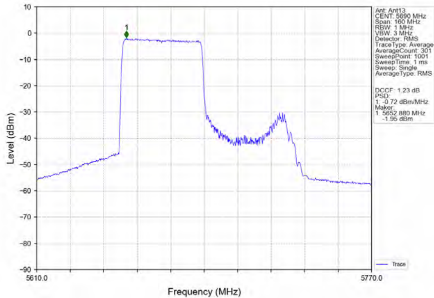
802.11ax(HEW80)_HCH_5690MHz_RU484_Right_MIMO_NTNV
