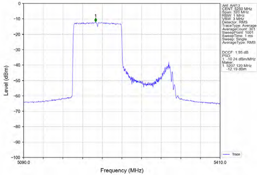
802.11ax(HEW160)_MCH_5250MHz_RU996_Left_MIMO_NTNV
