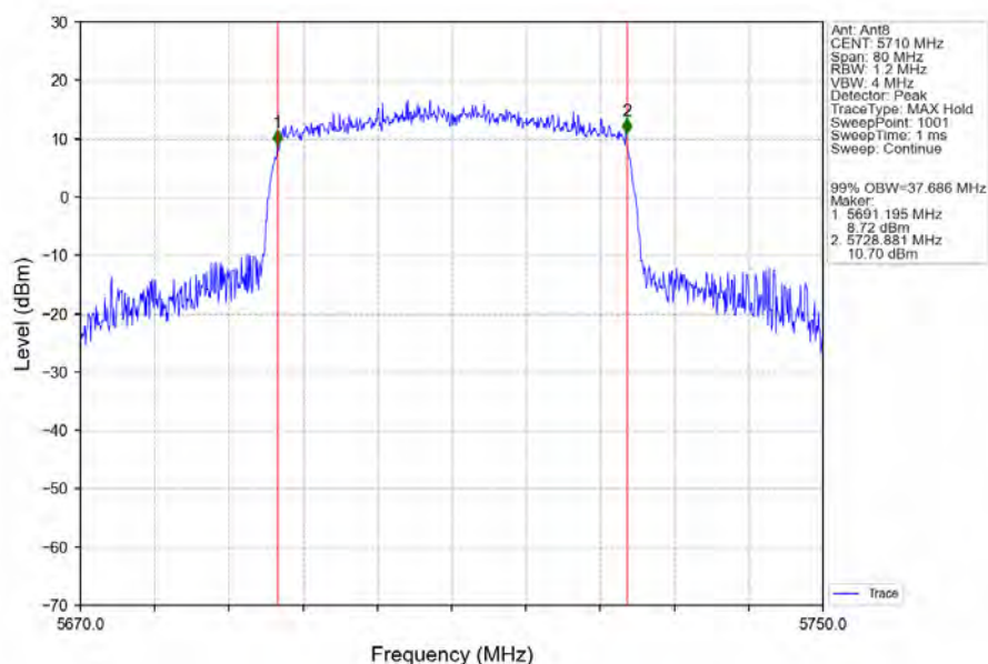
802.11ax(HEW40)_HCH_5710MHz_RU484_Left_Ant8_NTNV
