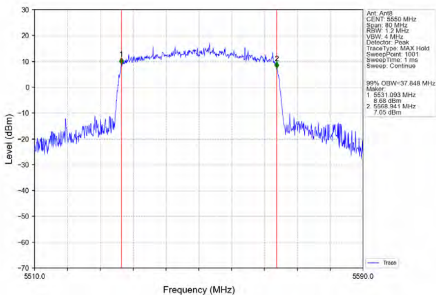
802.11ax(HEW40)_MCH_5550MHz_RU484_Left_Ant8_NTNV
