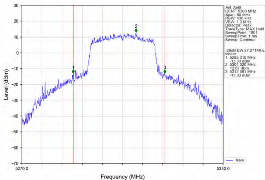
802.11ax(HEW20)_MCH_5300MHz_RU242_Left_Ant8_NTNV
