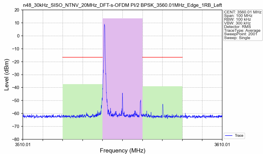
n48_30kHz_SISO_NTNV_20MHz_DFT-s-OFDM_PI/2_BPSK_3560.01MHz_Edge_1RB_Left_Ant8
