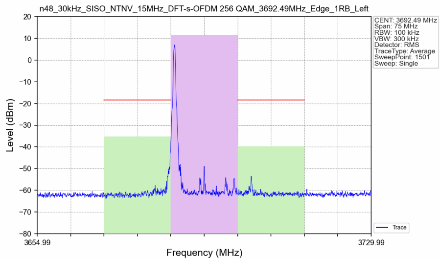
n48_30kHz_SISO_NTNV_15MHz_DFT-s-OFDM 256 QAM_3692.49MHz_Edge_1RB_Left_Ant8
