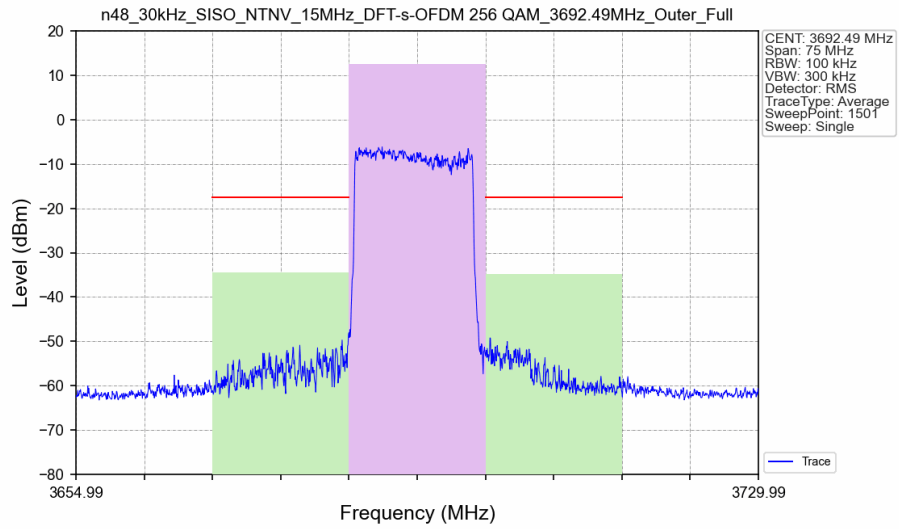
n48_30kHz_SISO_NTNV_15MHz_DFT-s-OFDM 256 QAM_3692.49MHz_Outer_Full_Ant8
