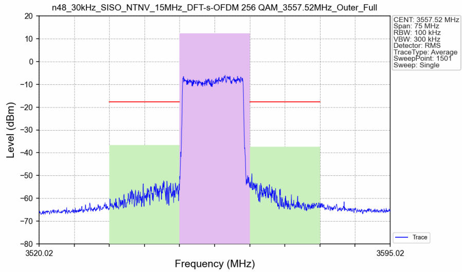
n48_30kHz_SISO_NTNV_15MHz_DFT-s-OFDM 256 QAM_3557.52MHz_Outer_Full_Ant8
