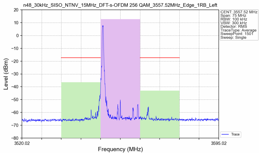
n48_30kHz_SISO_NTNV_15MHz_DFT-s-OFDM 256 QAM_3557.52MHz_Edge_1RB_Left_Ant8
