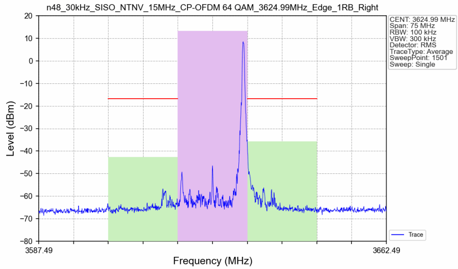
n48_30kHz_SISO_NTNV_15MHz_CP-OFDM 64 QAM_3624.99MHz_Edge_1RB_Right_Ant8
