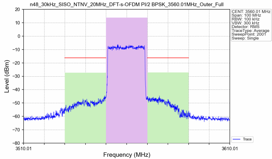
n48_30kHz_SISO_NTNV_20MHz_DFT-s-OFDM_PI/2_BPSK_3560.01MHz_Outer_Full_Ant8
