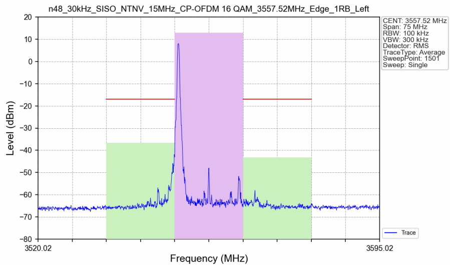
n48_30kHz_SISO_NTNV_15MHz_CP-OFDM_16_QAM_3557.52MHz_Edge_1RB_Left_Ant8
