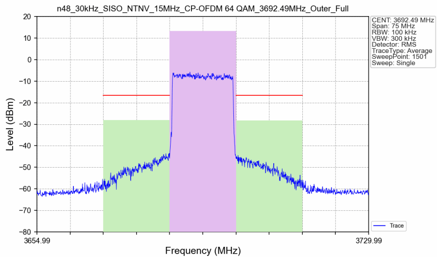
n48_30kHz_SISO_NTNV_15MHz_CP-OFDM 64 QAM_3692.49MHz_Outer_Full_Ant8
