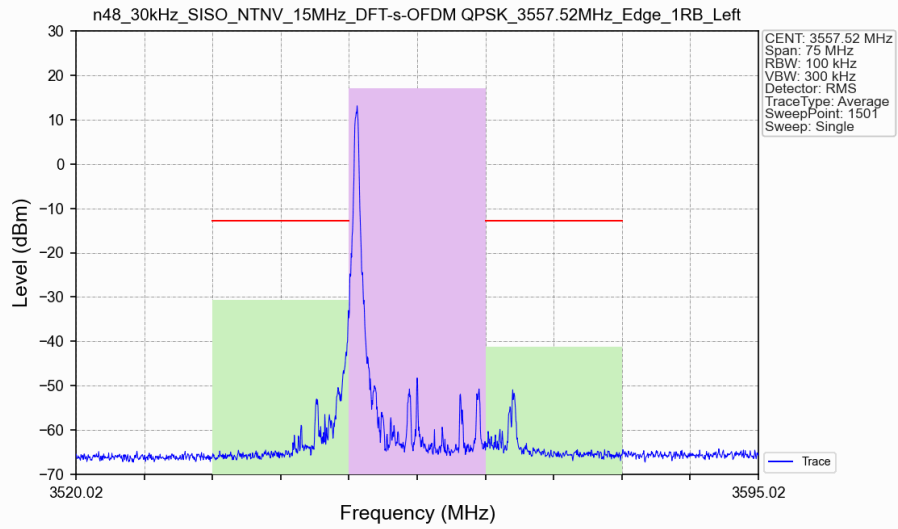
n48_30kHz_SISO_NTNV_15MHz_DFT-s-OFDM QPSK_3557.52MHz_Edge_1RB_Left_Ant8
