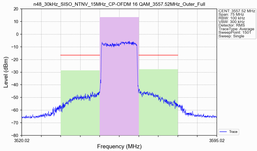
n48_30kHz_SISO_NTNV_15MHz_CP-OFDM_16_QAM_3557.52MHz_Outer_Full_Ant8
