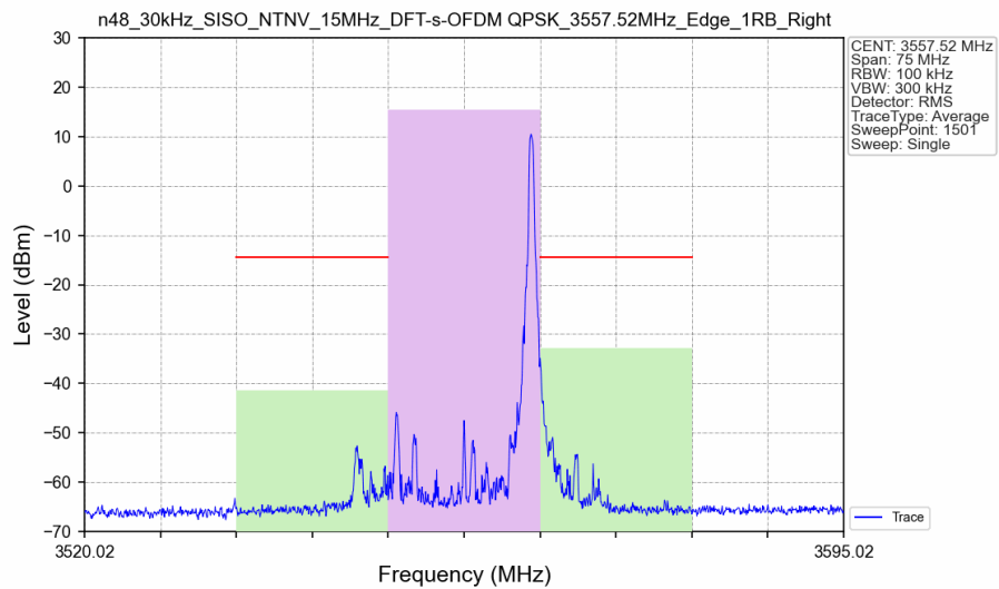
n48_30kHz_SISO_NTNV_15MHz_DFT-s-OFDM QPSK_3557.52MHz_Edge_1RB_Right_Ant8
