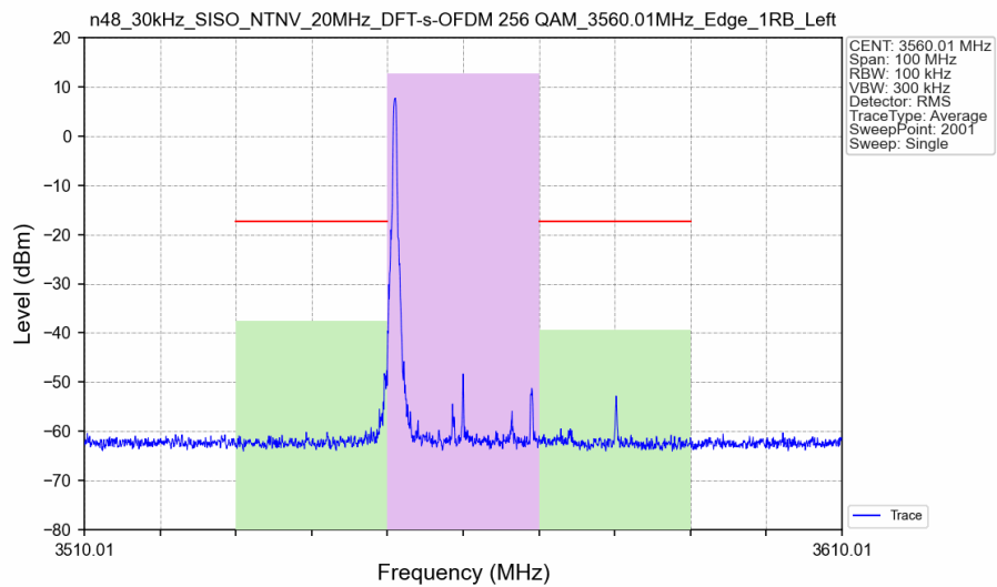
n48_30kHz_SISO_NTNV_20MHz_DFT-s-OFDM 256 QAM_3560.01MHz_Edge_1RB_Left_Ant8
