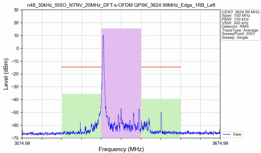
n48_30kHz_SISO_NTNV_20MHz_DFT-s-OFDM QPSK_3624.99MHz_Edge_1RB_Left_Ant8
