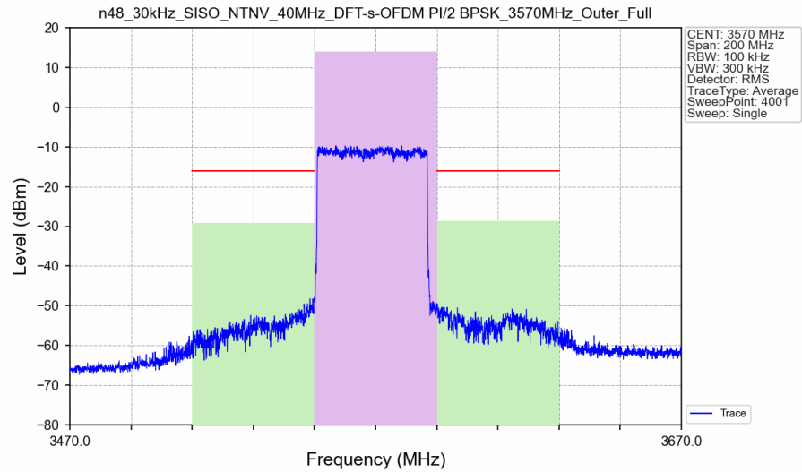
n48_30kHz_SISO_NTNV_40MHz_DFT-s-OFDM PI/2 BPSK_3570MHz_Outer_Full_Ant8
