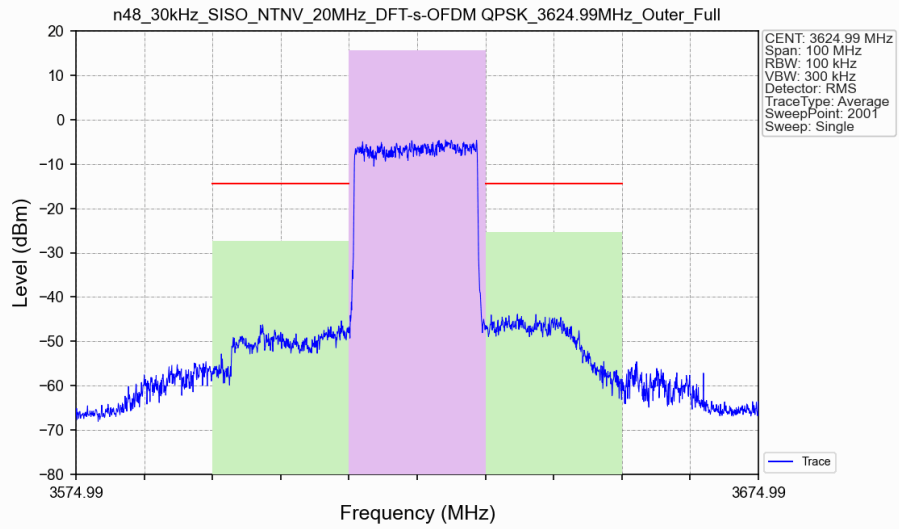
n48_30kHz_SISO_NTNV_20MHz_DFT-s-OFDM QPSK_3624.99MHz_Outer_Full_Ant8
