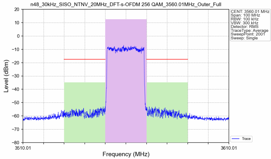
n48_30kHz_SISO_NTNV_20MHz_DFT-s-OFDM 256 QAM_3560.01MHz_Outer_Full_Ant8
