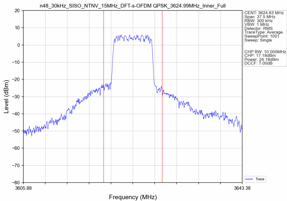
n48_30kHz_SISO_NTNV_15MHz_DFT-s-OFDM QPSK_3624.99MHz_Inner_Full_Ant8
