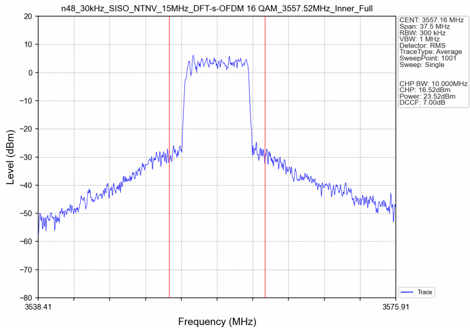
n48_30kHz_SISO_NTNV_15MHz_DFT-s-OFDM_16_QAM_3557.52MHz_Inner_Full_Ant8
