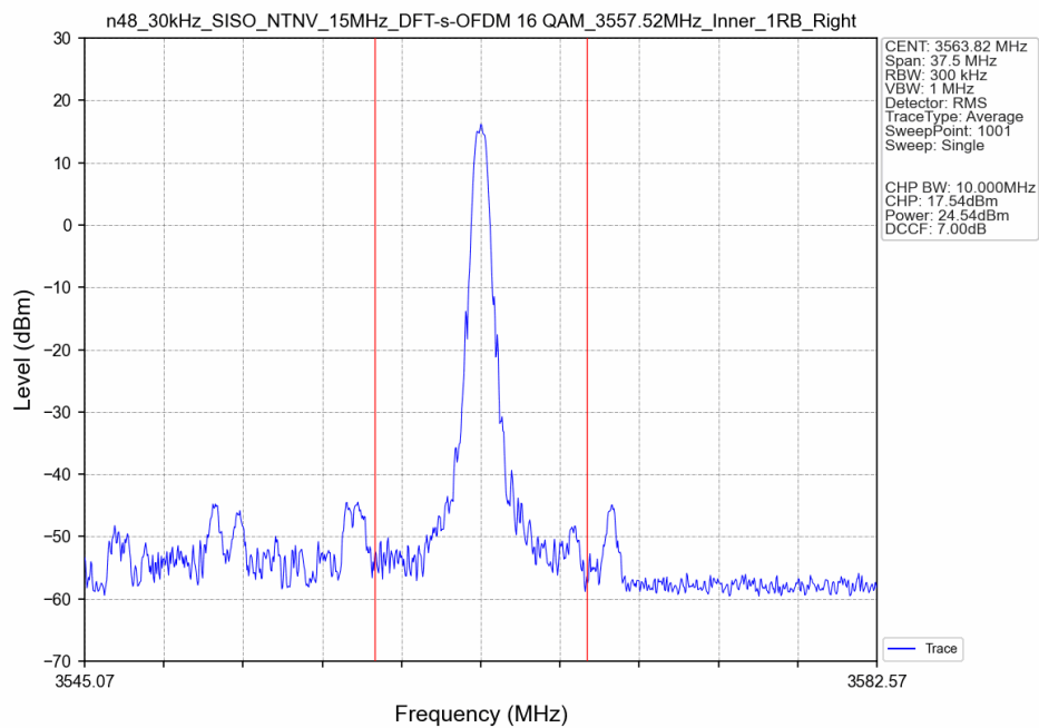
n48_30kHz_SISO_NTNV_15MHz_DFT-s-OFDM_16_QAM_3557.52MHz_Inner_1RB_Right_Ant8
