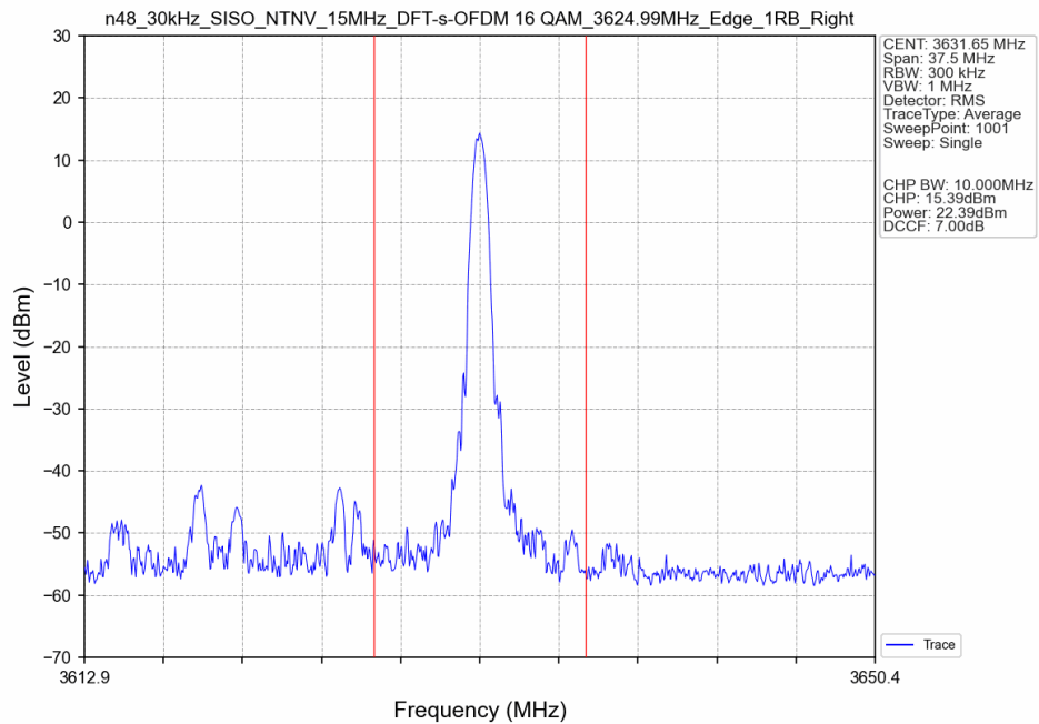
n48_30kHz_SISO_NTNV_15MHz_DFT-s-OFDM 16 QAM_3624.99MHz_Edge_1RB_Right_Ant8
