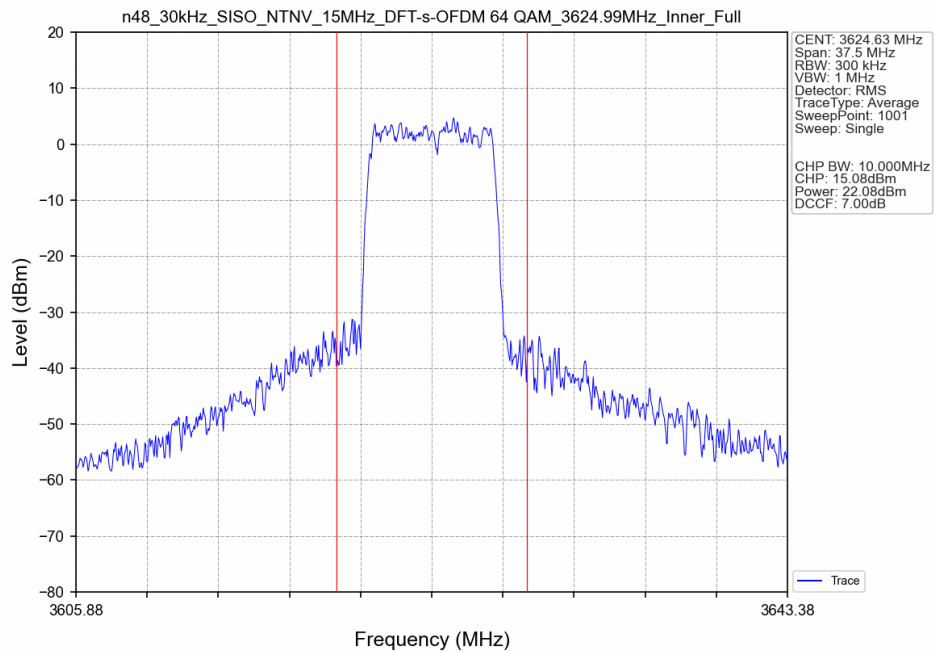
n48_30kHz_SISO_NTNV_15MHz_DFT-s-OFDM 64 QAM_3624.99MHz_Inner_Full_Ant8
