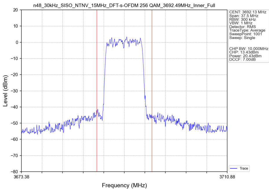
n48_30kHz_SISO_NTNV_15MHz_DFT-s-OFDM 256 QAM_3692.49MHz_Inner_Full_Ant8
