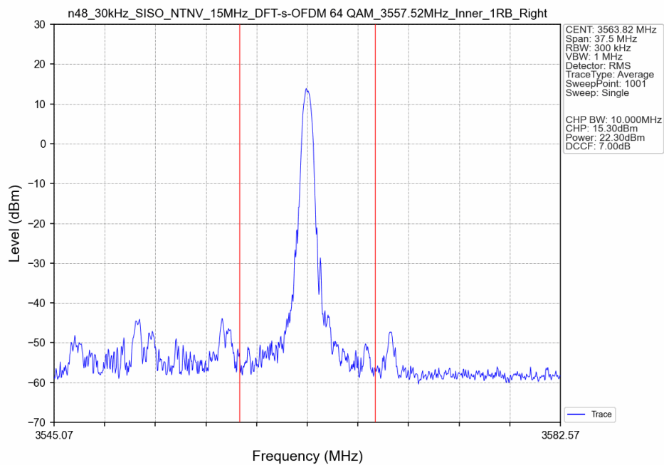
n48_30kHz_SISO_NTNV_15MHz_DFT-s-OFDM 64 QAM_3557.52MHz_Inner_1RB_Right_Ant8
