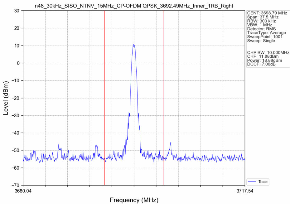
n48_30kHz_SISO_NTNV_15MHz_CP-OFDM QPSK_3692.49MHz_Inner_1RB_Right_Ant8
