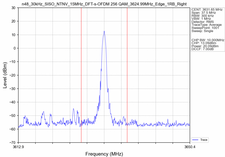
n48_30kHz_SISO_NTNV_15MHz_DFT-s-OFDM 256 QAM_3624.99MHz_Edge_1RB_Right_Ant8
