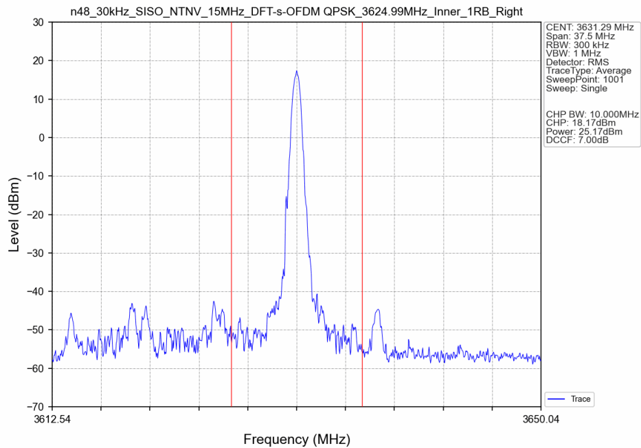
n48_30kHz_SISO_NTNV_15MHz_DFT-s-OFDM QPSK_3624.99MHz_Inner_1RB_Right_Ant8
