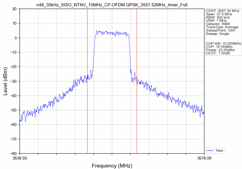
n48_30kHz_SISO_NTNV_15MHz_CP-OFDM QPSK_3557.52MHz_Inner_Full_Ant8
