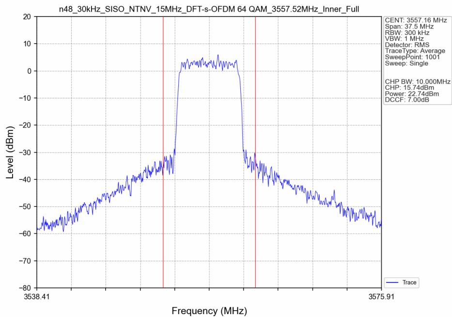
n48_30kHz_SISO_NTNV_15MHz_DFT-s-OFDM 64 QAM_3557.52MHz_Inner_Full_Ant8
