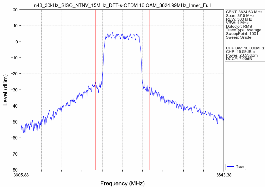
n48_30kHz_SISO_NTNV_15MHz_DFT-s-OFDM_16_QAM_3624.99MHz_Inner_Full_Ant8
