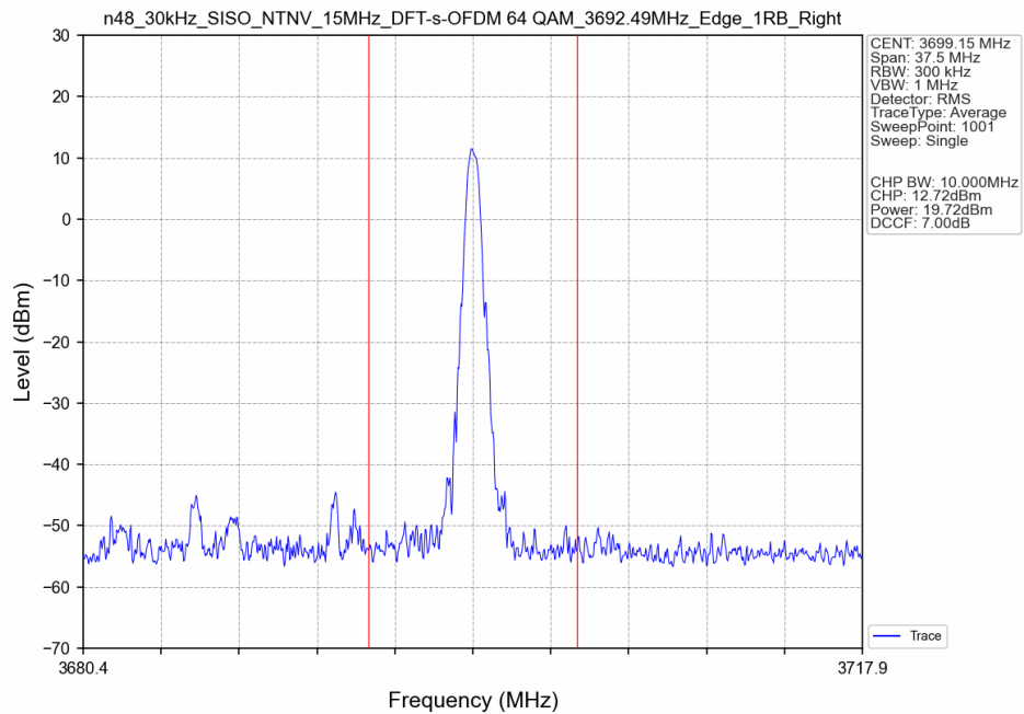
n48_30kHz_SISO_NTNV_15MHz_DFT-s-OFDM 64 QAM_3692.49MHz_Edge_1RB_Right_Ant8
