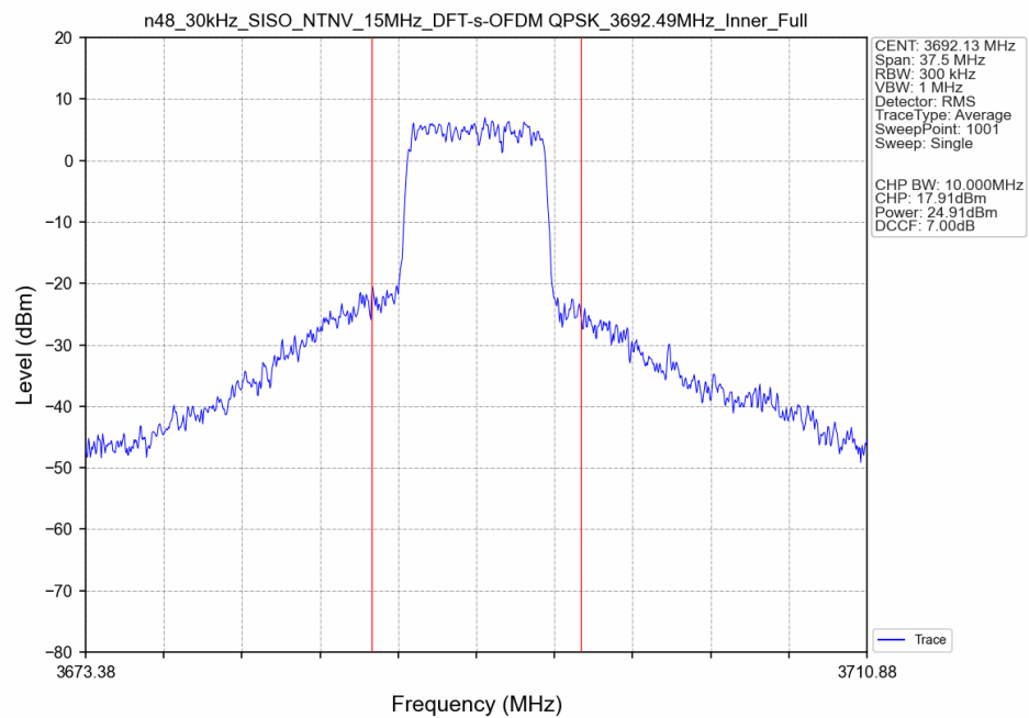
n48_30kHz_SISO_NTNV_15MHz_DFT-s-OFDM QPSK_3692.49MHz_Inner_Full_Ant8
