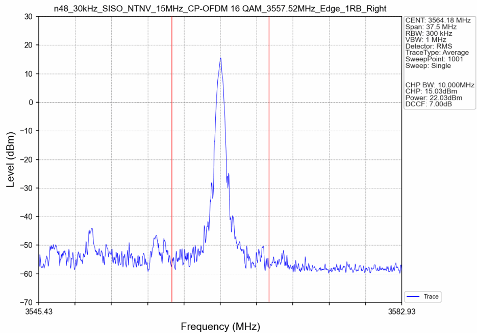
n48_30kHz_SISO_NTNV_15MHz_CP-OFDM 16 QAM 3557.52MHz_Edge_1RB_Right_Ant8
