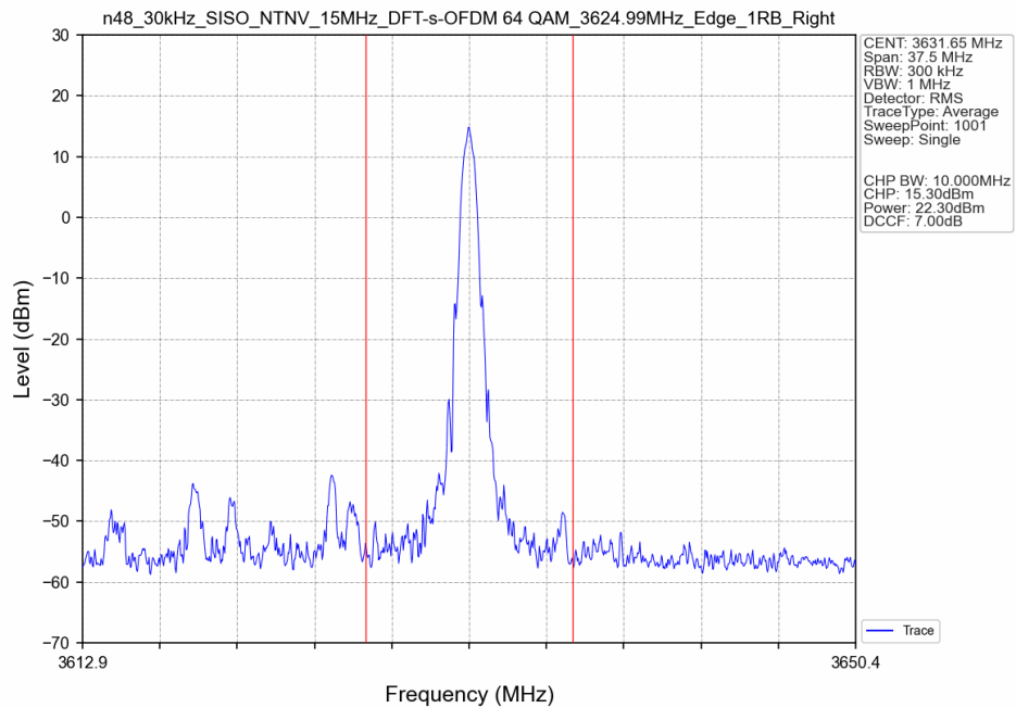
n48_30kHz_SISO_NTNV_15MHz_DFT-s-OFDM 64 QAM_3624.99MHz_Edge_1RB_Right_Ant8
