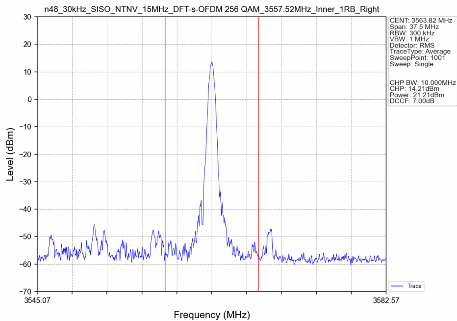
n48_30kHz_SISO_NTNV_15MHz_DFT-s-OFDM 256 QAM_3557.52MHz_Inner_1RB_Right_Ant8
