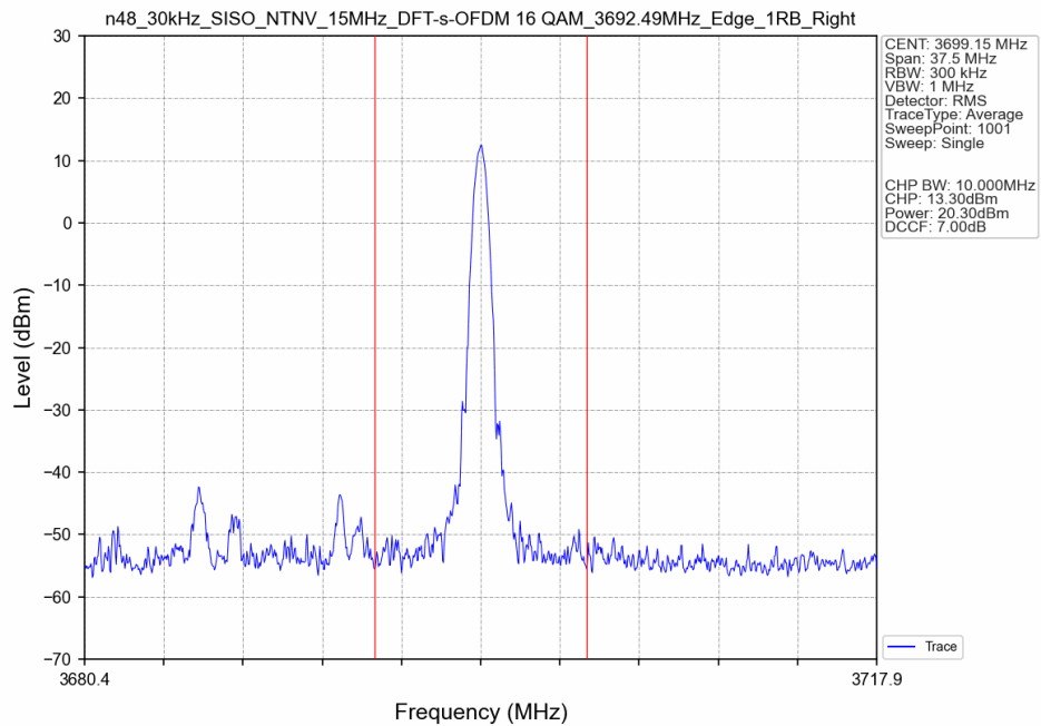
n48_30kHz_SISO_NTNV_15MHz_DFT-s-OFDM_16_QAM_3692.49MHz_Edge_1RB_Right_Ant8
