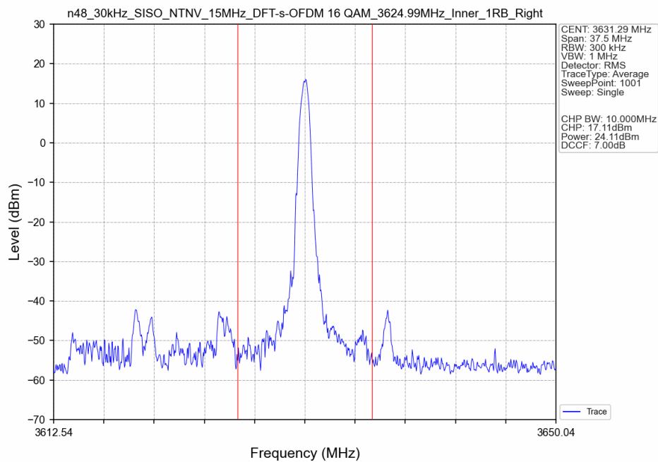
n48_30kHz_SISO_NTNV_15MHz_DFT-s-OFDM_16_QAM_3624.99MHz_Inner_1RB_Right_Ant8
