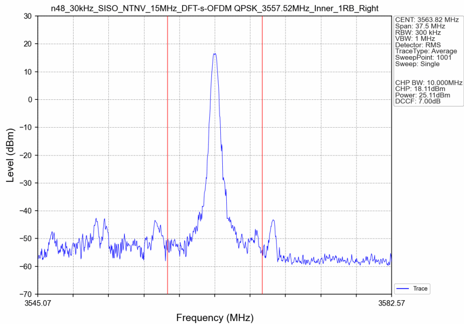
n48_30kHz_SISO_NTNV_15MHz_DFT-s-OFDM_QPSK_3557.52MHz_Inner_1RB_Right_Ant8
