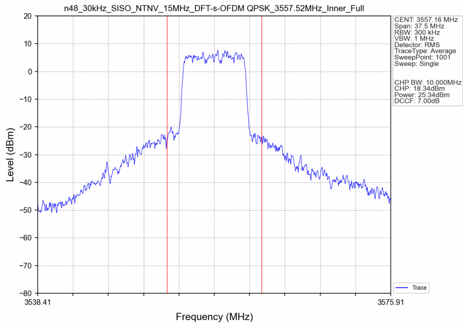
n48_30kHz_SISO_NTNV_15MHz_DFT-s-OFDM QPSK_3557.52MHz_Inner_Full_Ant8
