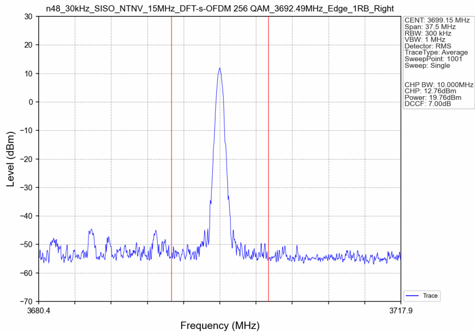
n48_30kHz_SISO_NTNV_15MHz_DFT-s-OFDM 256 QAM_3692.49MHz_Edge_1RB_Right_Ant8
