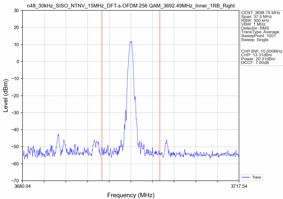
n48_30kHz_SISO_NTNV_15MHz_DFT-s-OFDM 256 QAM_3692.49MHz_Inner_1RB_Right_Ant8
