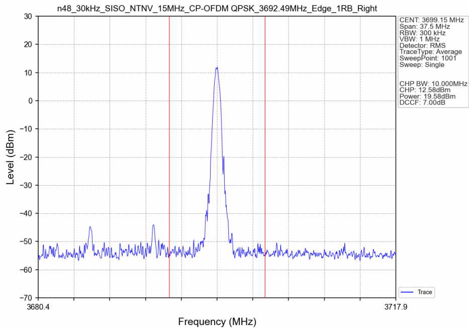
n48_30kHz_SISO_NTNV_15MHz_CP-OFDM QPSK_3692.49MHz_Edge_1RB_Right_Ant8
