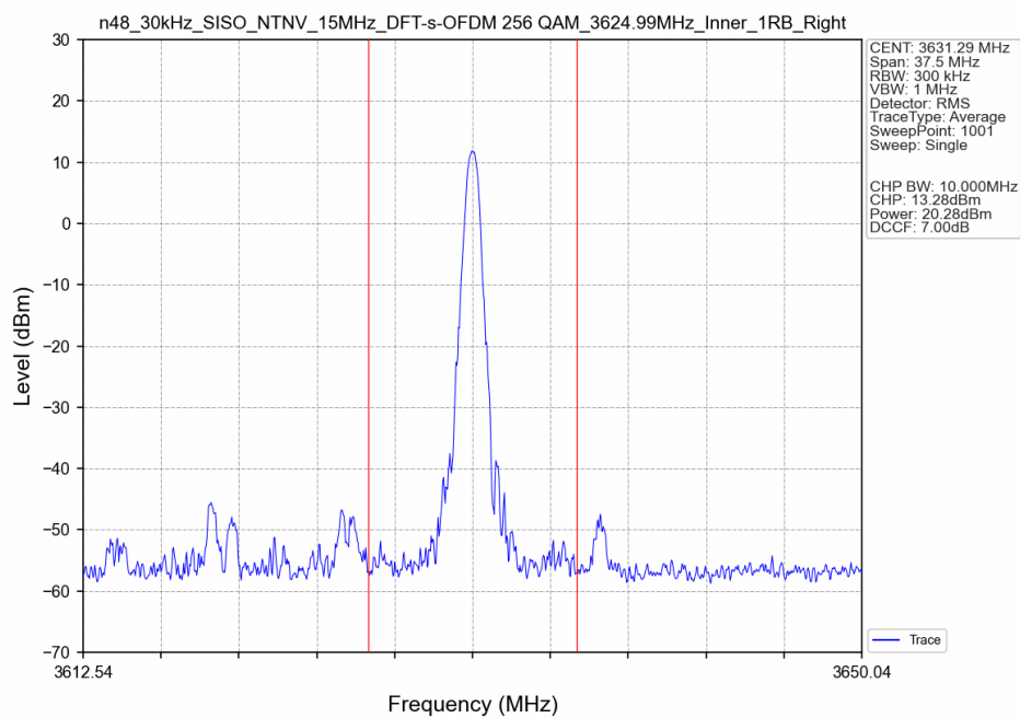
n48_30kHz_SISO_NTNV_15MHz_DFT-s-OFDM 256 QAM_3624.99MHz_Inner_1RB_Right_Ant8
