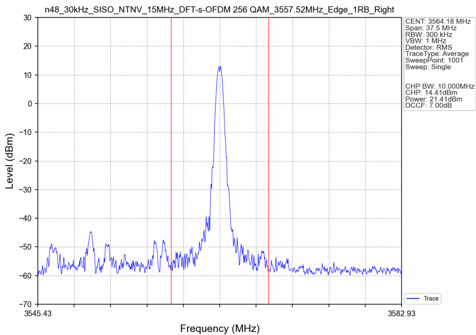
n48_30kHz_SISO_NTNV_15MHz_DFT-s-OFDM 256 QAM_3557.52MHz_Edge_1RB_Right_Ant8
