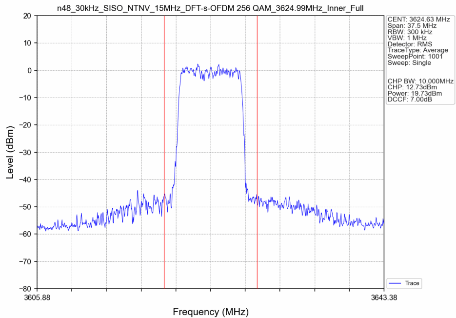
n48_30kHz_SISO_NTNV_15MHz_DFT-s-OFDM 256 QAM_3624.99MHz_Inner_Full_Ant8
