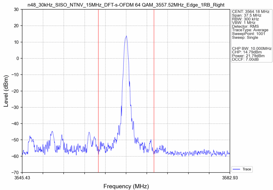
n48_30kHz_SISO_NTNV_15MHz_DFT-s-OFDM 64 QAM_3557.52MHz_Edge_1RB_Right_Ant8
