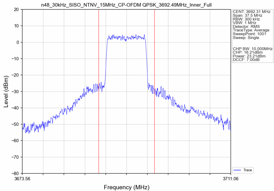
n48_30kHz_SISO_NTNV_15MHz_CP-OFDM QPSK_3692.49MHz_Inner_Full_Ant8
