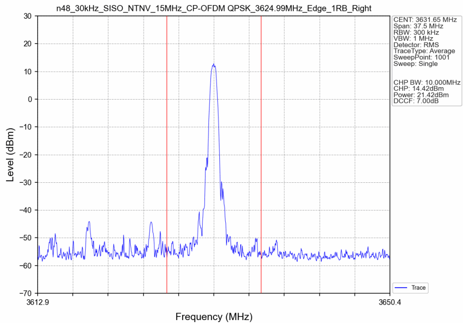
n48_30kHz_SISO_NTNV_15MHz_CP-OFDM QPSK_3624.99MHz_Edge_1RB_Right_Ant8
