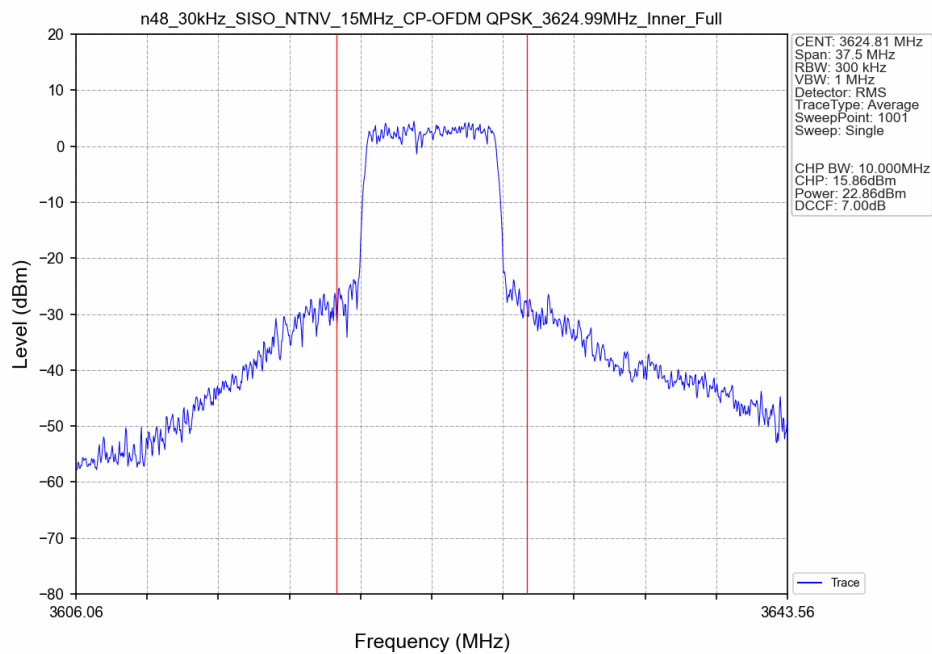
n48_30kHz_SISO_NTNV_15MHz_CP-OFDM QPSK_3624.99MHz_Inner_Full_Ant8
