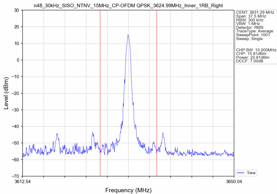
n48_30kHz_SISO_NTNV_15MHz_CP-OFDM QPSK_3624.99MHz_Inner_1RB_Right_Ant8
