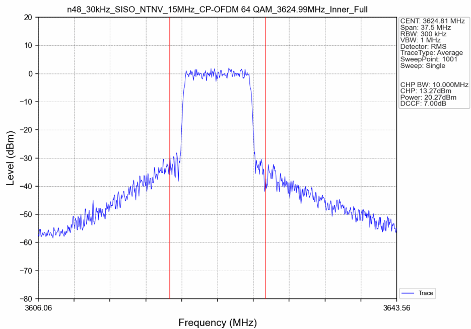
n48_30kHz_SISO_NTNV_15MHz_CP-OFDM 64 QAM_3624.99MHz_Inner_Full_Ant8
