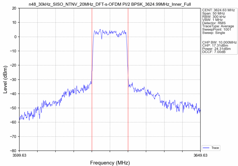
n48_30kHz_SISO_NTNV_20MHz_DFT-s-OFDM PI/2 BPSK_3624.99MHz_Inner_Full_Ant8
