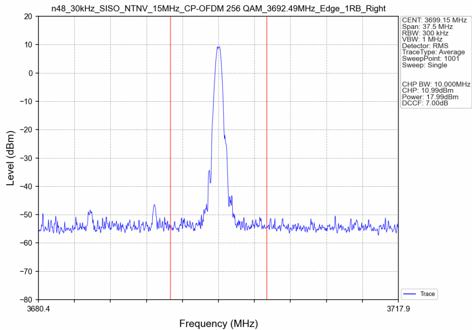
n48_30kHz_SISO_NTNV_15MHz_CP-OFDM 256 QAM 3692.49MHz_Edge_1RB_Right_Ant8
