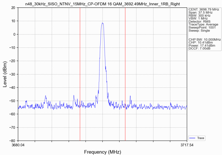
n48_30kHz_SISO_NTNV_15MHz_CP-OFDM 16 QAM 3692.49MHz_Inner_1RB_Right_Ant8
