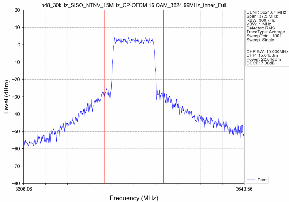
n48_30kHz_SISO_NTNV_15MHz_CP-OFDM 16 QAM_3624.99MHz_Inner_Full_Ant8
