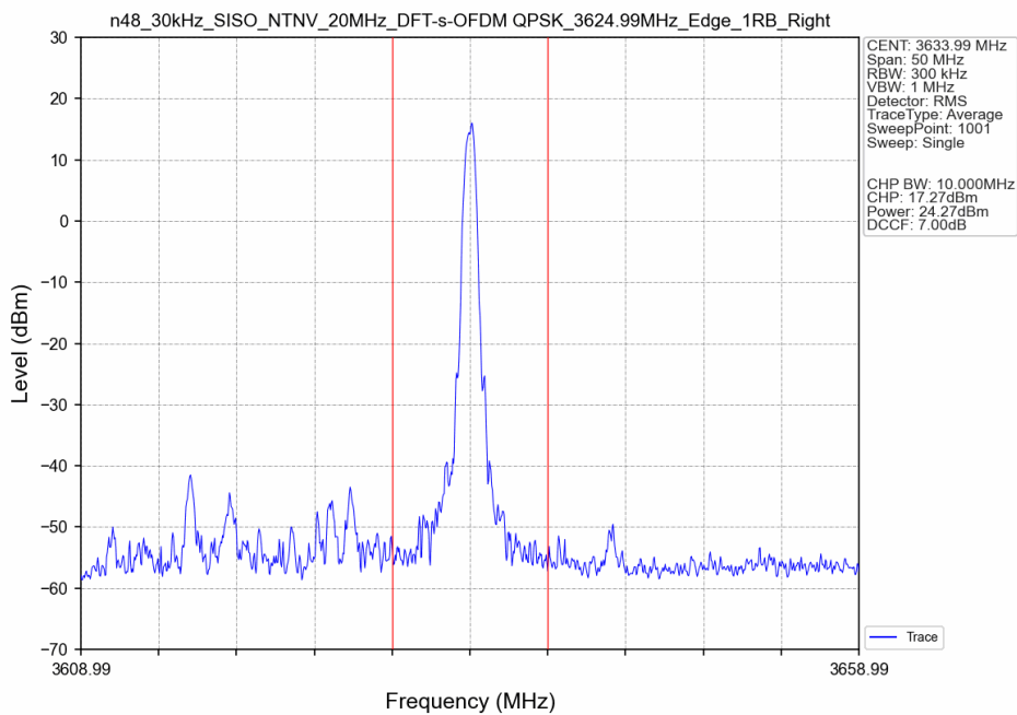
n48_30kHz_SISO_NTNV_20MHz_DFT-s-OFDM QPSK_3624.99MHz_Edge_1RB_Right_Ant8
