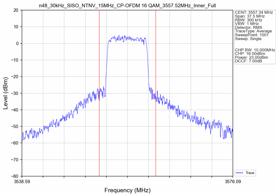
n48_30kHz_SISO_NTNV_15MHz_CP-OFDM 16 QAM 3557.52MHz_Inner_Full_Ant8
