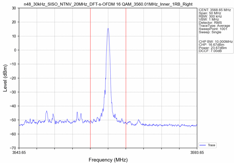
n48_30kHz_SISO_NTNV_20MHz_DFT-s-OFDM 16 QAM_3560.01MHz_Inner_1RB_Right_Ant8
