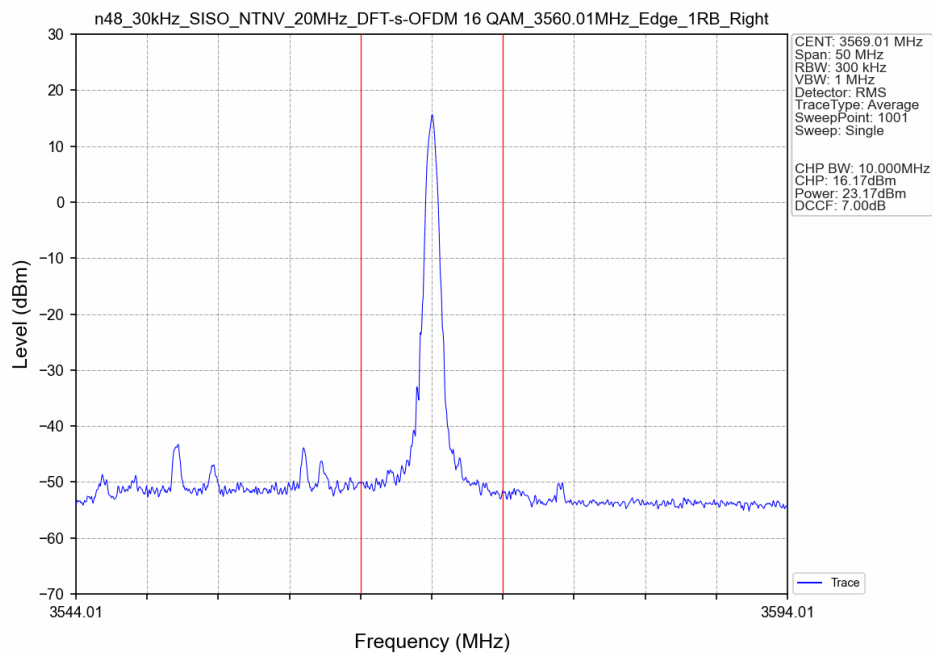
n48_30kHz_SISO_NTNV_20MHz_DFT-s-OFDM 16 QAM_3560.01MHz_Edge_1RB_Right_Ant8
