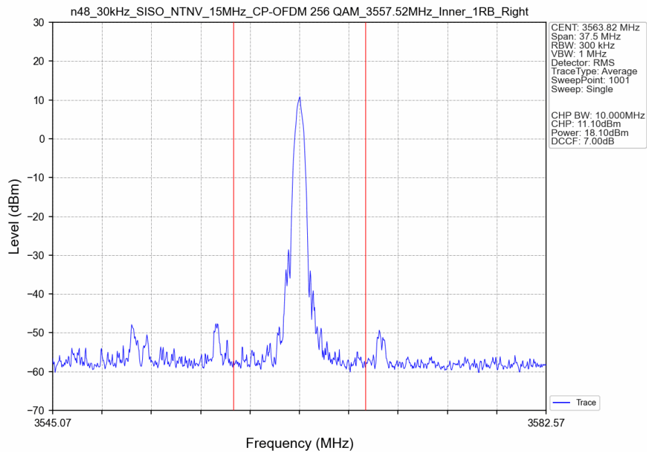
n48_30kHz_SISO_NTNV_15MHz_CP-OFDM 256 QAM 3557.52MHz_Inner_1RB_Right_Ant8
