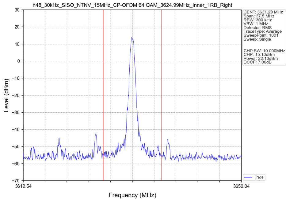
n48_30kHz_SISO_NTNV_15MHz_CP-OFDM 64 QAM_3624.99MHz_Inner_1RB_Right_Ant8
