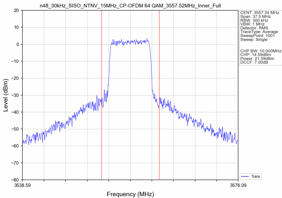
n48_30kHz_SISO_NTNV_15MHz_CP-OFDM 64 QAM_3557.52MHz_Inner_Full_Ant8
