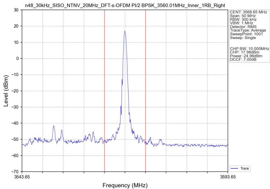
n48_30kHz_SISO_NTNV_20MHz_DFT-s-OFDM PI/2 BPSK_3560.01MHz_Inner_1RB_Right_Ant8
