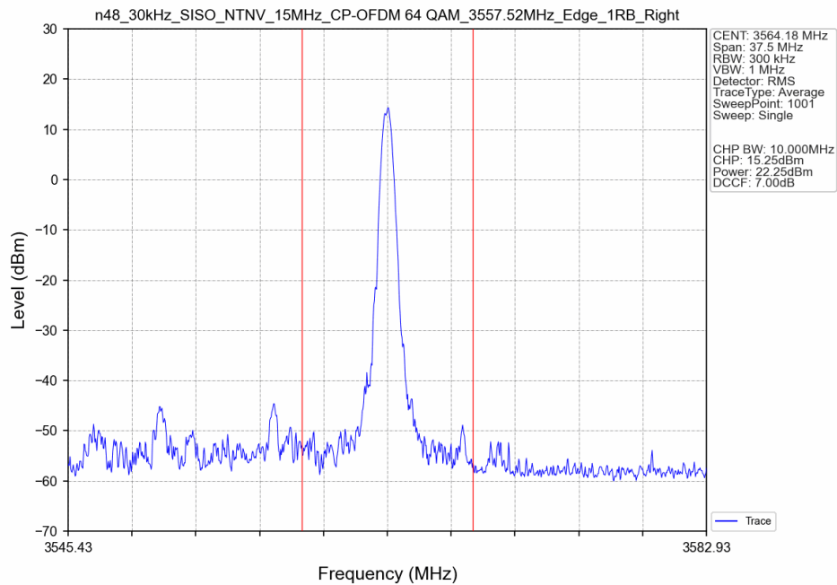
n48_30kHz_SISO_NTNV_15MHz_CP-OFDM 64 QAM_3557.52MHz_Edge_1RB_Right_Ant8
