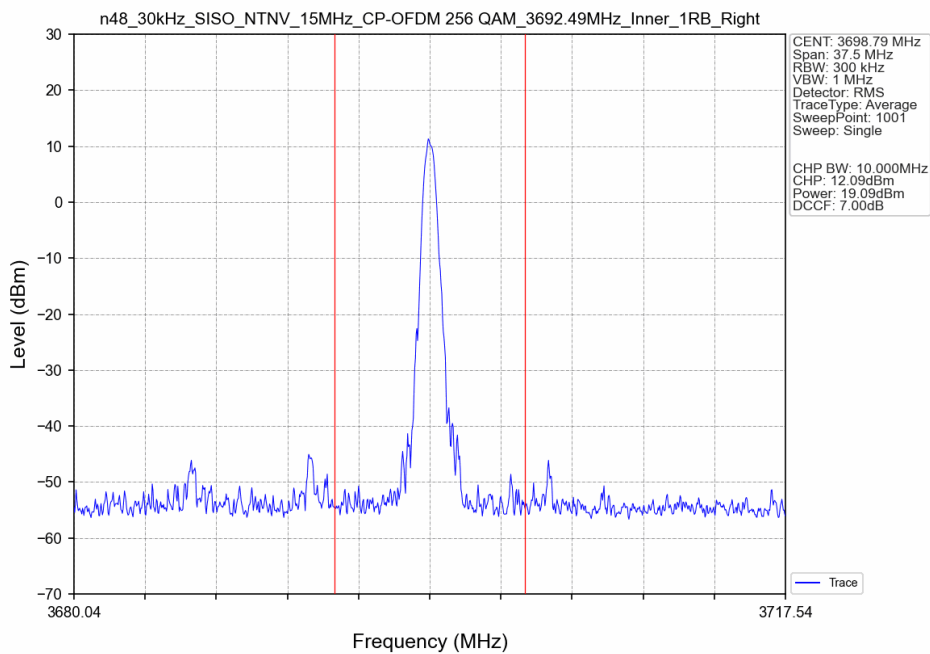
n48_30kHz_SISO_NTNV_15MHz_CP-OFDM 256 QAM_3692.49MHz_Inner_1RB_Right_Ant8
