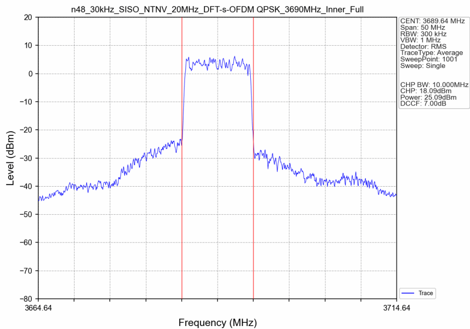
n48_30kHz_SISO_NTNV_20MHz_DFT-s-OFDM QPSK_3690MHz_Inner_Full_Ant8
