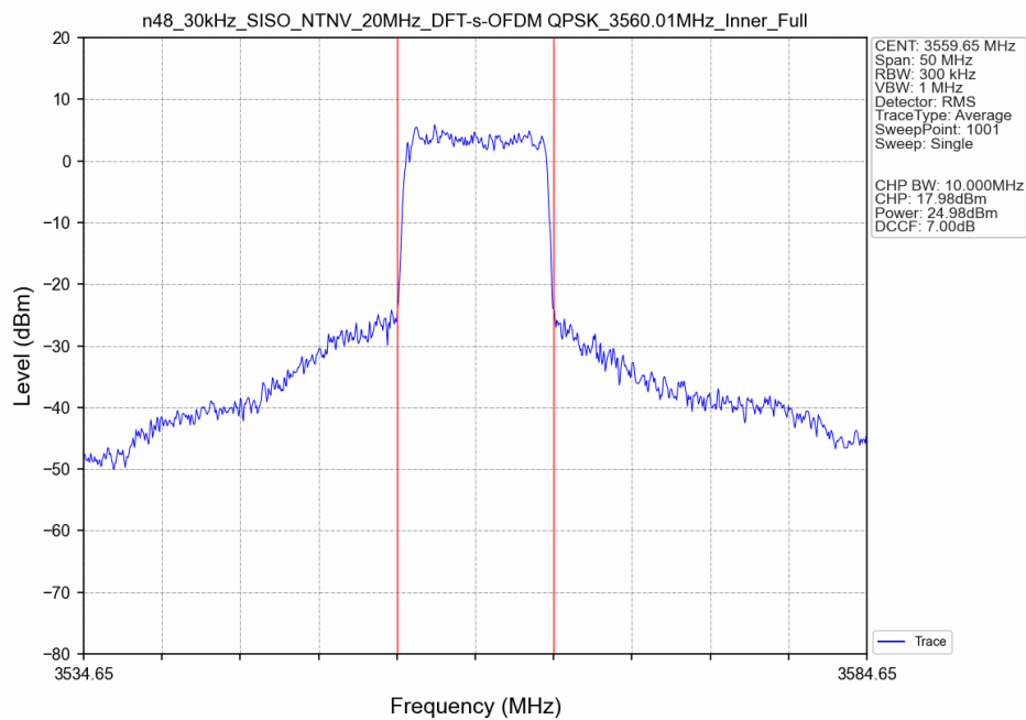
n48_30kHz_SISO_NTNV_20MHz_DFT-s-OFDM QPSK_3560.01MHz_Inner_Full_Ant8
