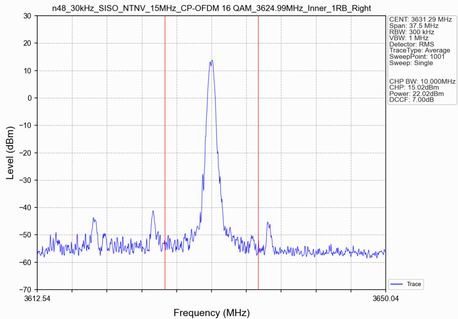
n48_30kHz_SISO_NTNV_15MHz_CP-OFDM 16 QAM 3624.99MHz_Inner_1RB_Right_Ant8
