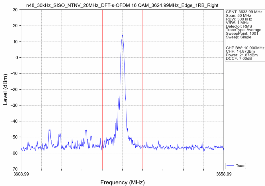
n48_30kHz_SISO_NTNV_20MHz_DFT-s-OFDM 16 QAM_3624.99MHz_Edge_1RB_Right_Ant8
