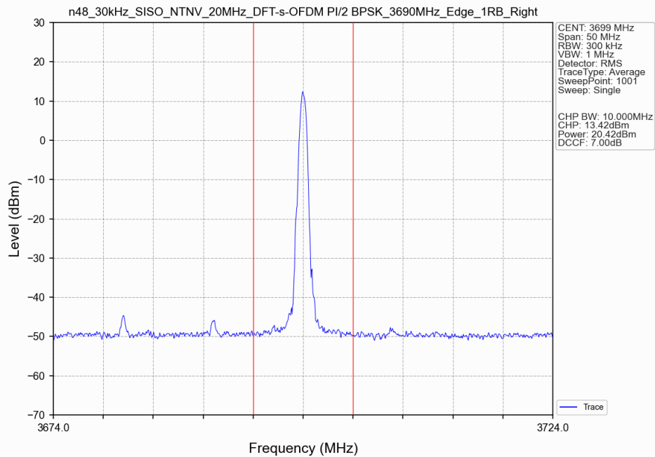
n48_30kHz_SISO_NTNV_20MHz_DFT-s-OFDM PI/2 BPSK_3690MHz_Edge_1RB_Right_Ant8
