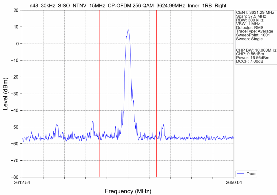
n48_30kHz_SISO_NTNV_15MHz_CP-OFDM 256 QAM 3624.99MHz_Inner_1RB_Right_Ant8
