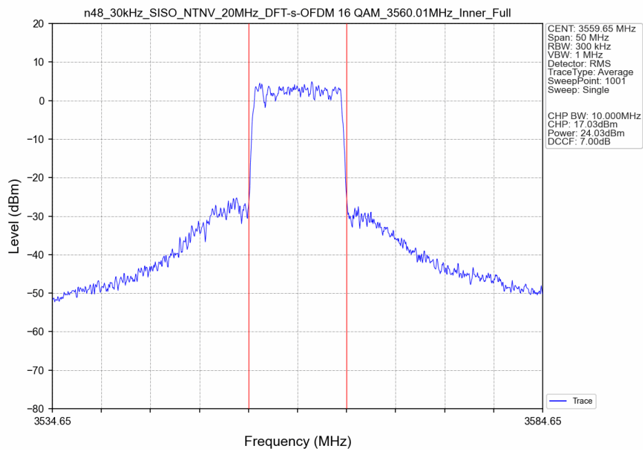
n48_30kHz_SISO_NTNV_20MHz_DFT-s-OFDM 16 QAM_3560.01MHz_Inner_Full_Ant8
