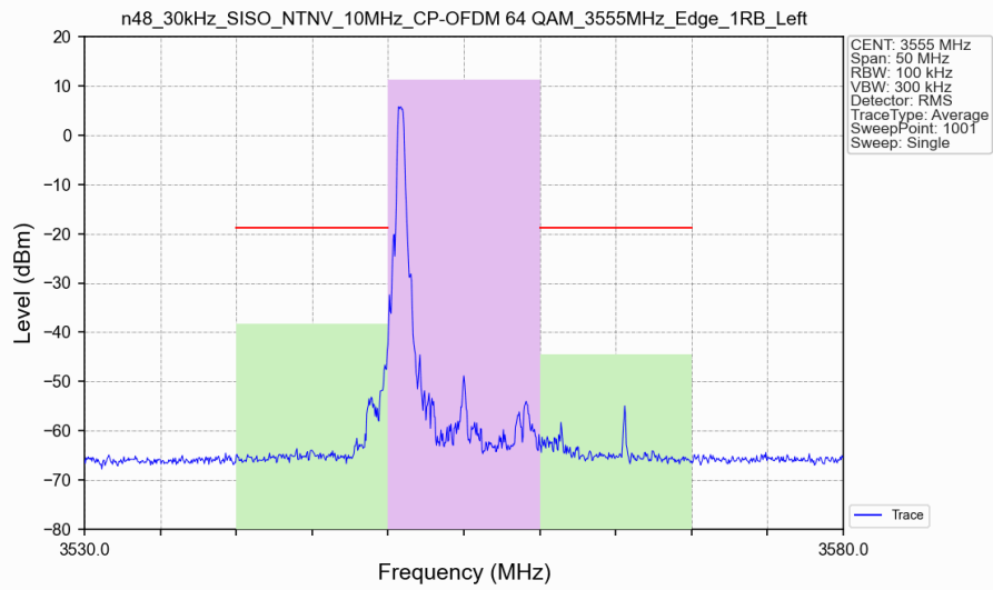
n48_30kHz_SISO_NTNV_10MHz_CP-OFDM 64 QAM_3555MHz_Edge_1RB_Left_Ant8
