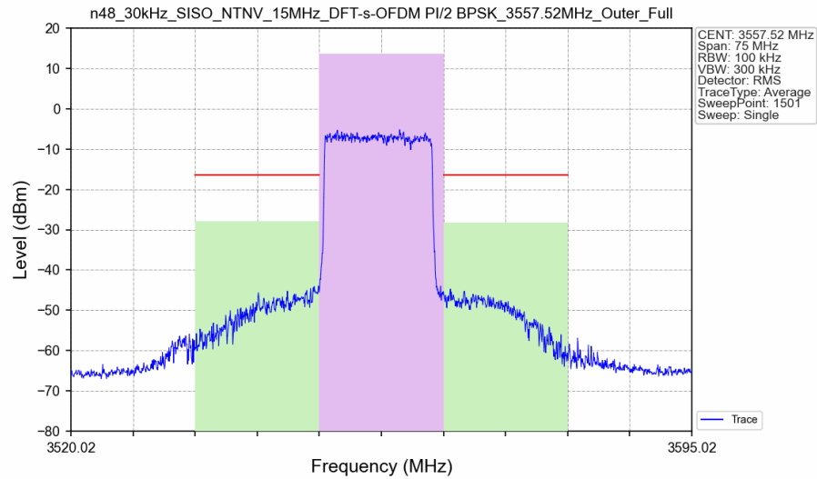
n48_30kHz_SISO_NTNV_15MHz_DFT-s-OFDM_PI/2_BPSK_3557.52MHz_Outer_Full_Ant8
