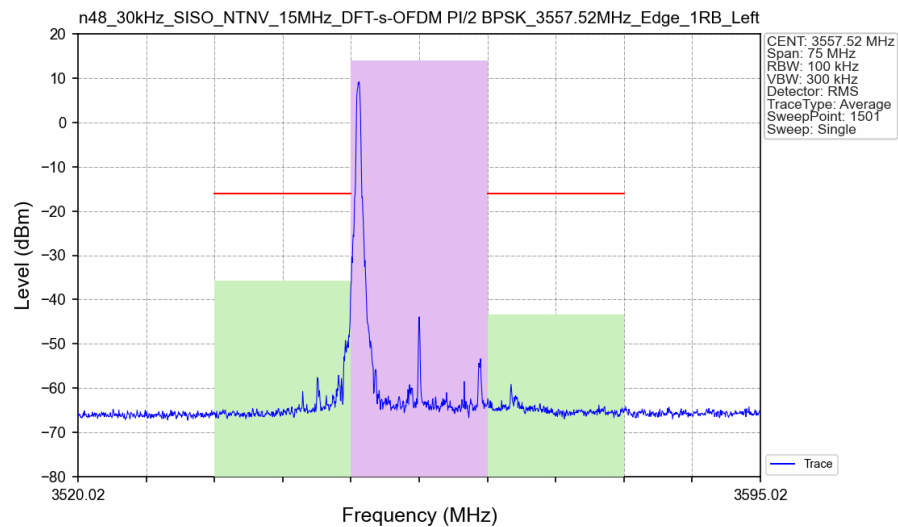
n48_30kHz_SISO_NTNV_15MHz_DFT-s-OFDM_PI/2_BPSK_3557.52MHz_Edge_1RB_Left_Ant8
