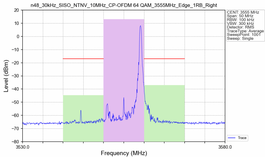
n48_30kHz_SISO_NTNV_10MHz_CP-OFDM 64 QAM_3555MHz_Edge_1RB_Right_Ant8
