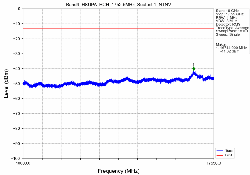
Band4_HSUPA_HCH_1752.6MHz_Subtest 1_NTNV
