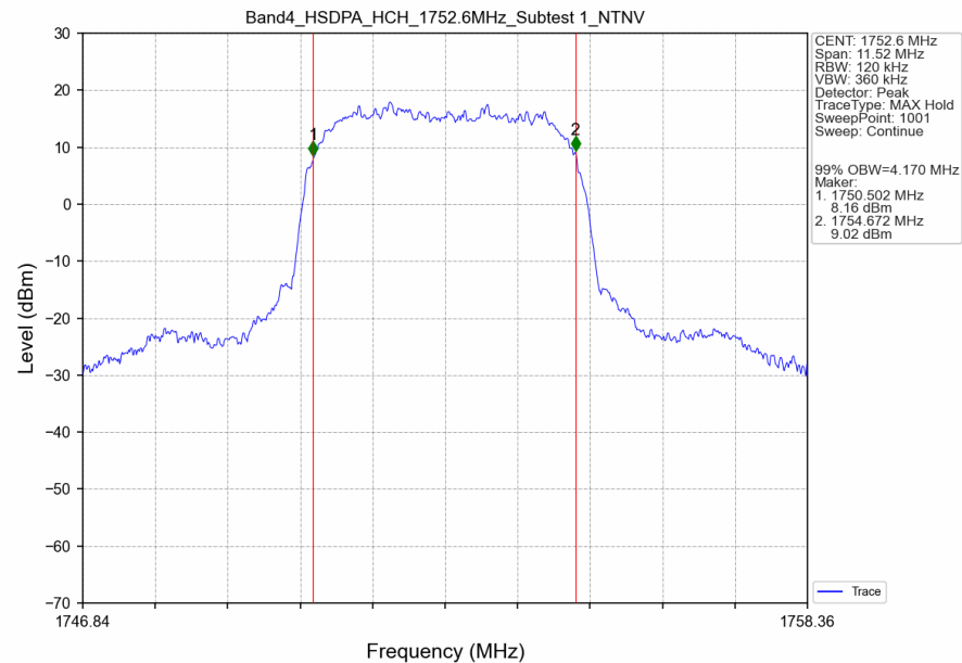
Band4_HSDPA_HCH_1752.6MHz_Subtest 1_NTNV
