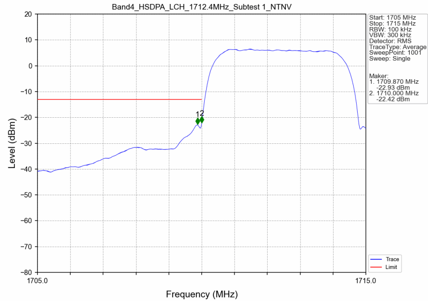
Band4_HSDPA_LCH_1712.4MHz_Subtest 1_NTNV
