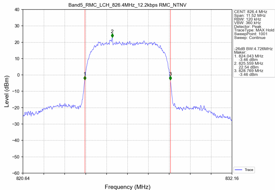
Band5_RMC_LCH_826.4MHz_12.2kbps RMC_NTNV
