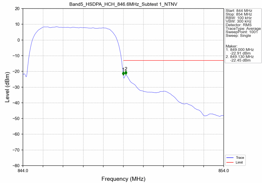
Band5_HSDPA_HCH_846.6MHz_Subtest 1_NTNV
