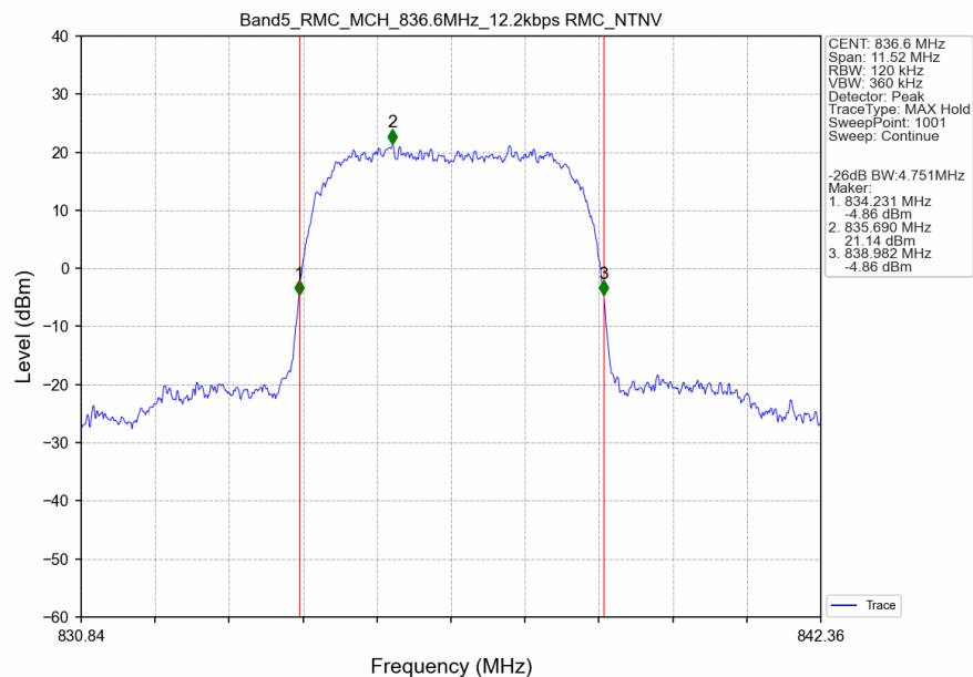
Band5_RMC_MCH_836.6MHz_12.2kbps RMC_NTNV
