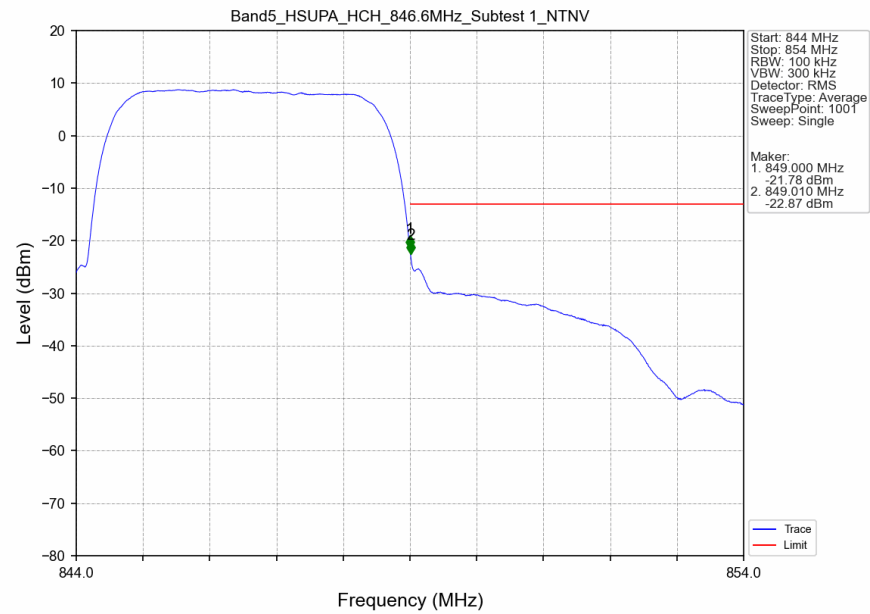
Band5_HSUPA_HCH_846.6MHz_Subtest 1_NTNV
