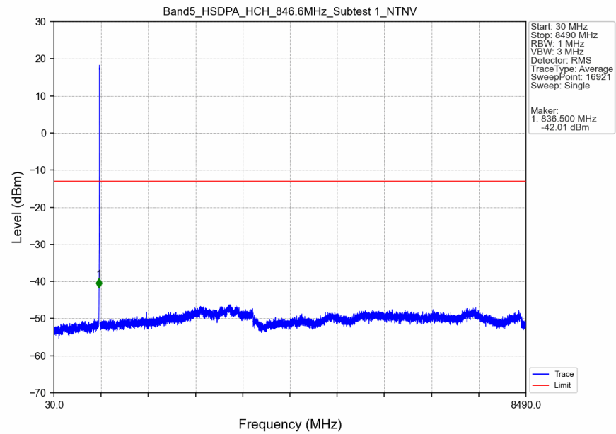
Band5_HSDPA_HCH_846.6MHz_Subtest 1_NTNV
