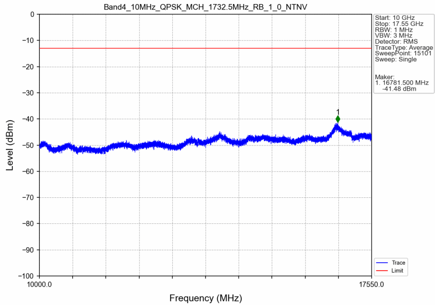
Band4_10MHz_QPSK_MCH_1732.5MHz_RB_1_0_NTNV
