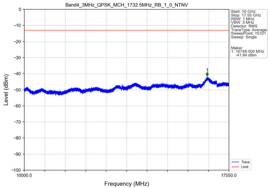
Band4_3MHz_QPSK_MCH_1732.5MHz_RB_1_0_NTNV
