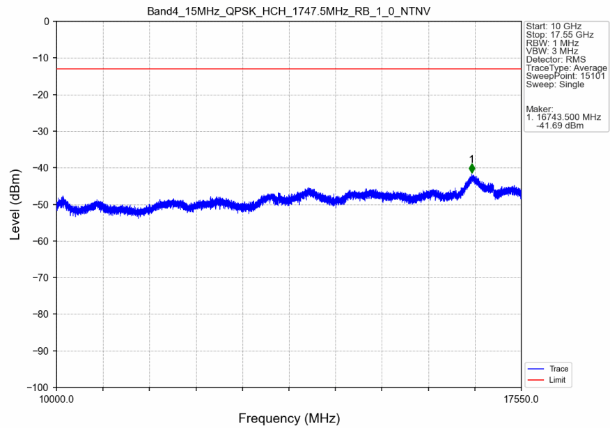
Band4_15MHz_QPSK_HCH_1747.5MHz_RB_1_0_NTNV
