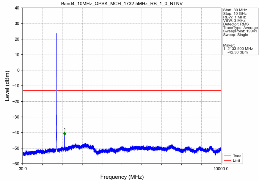
Band4_10MHz_QPSK_MCH_1732.5MHz_RB_1_0_NTNV
