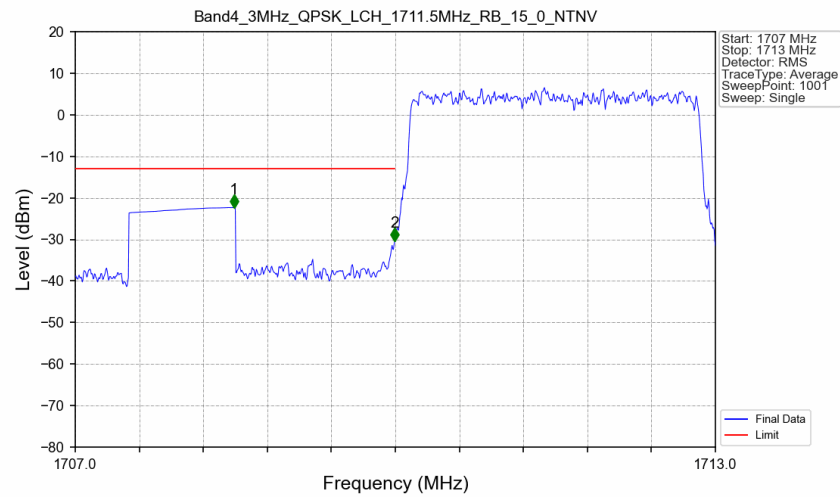
Band4 3MHz QPSK LCH 1711.5MHz RB 15 0 NTN
