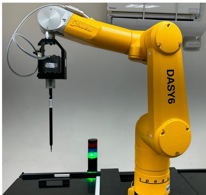
Fig.1 Photograph of the SAR measurement system
