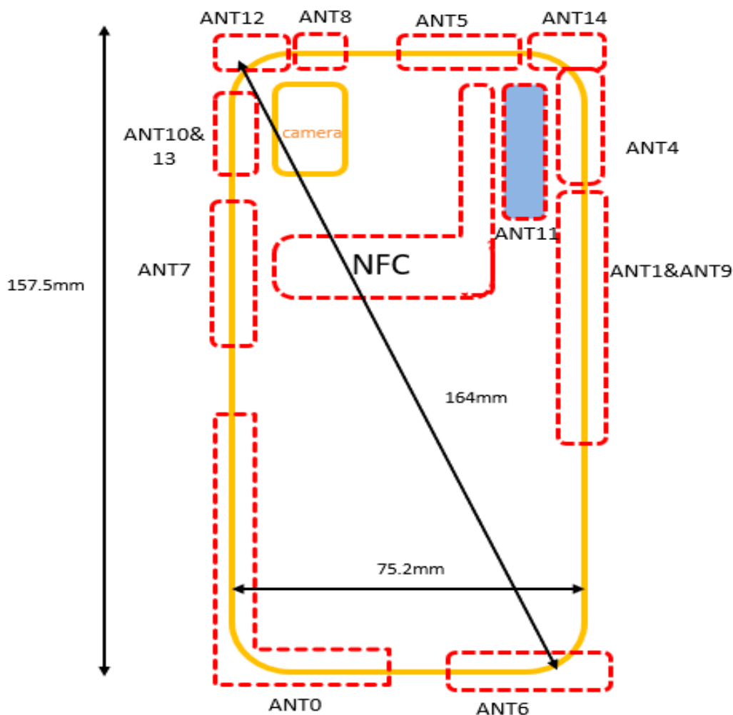
Photograph 5. Antenna position of EUT
