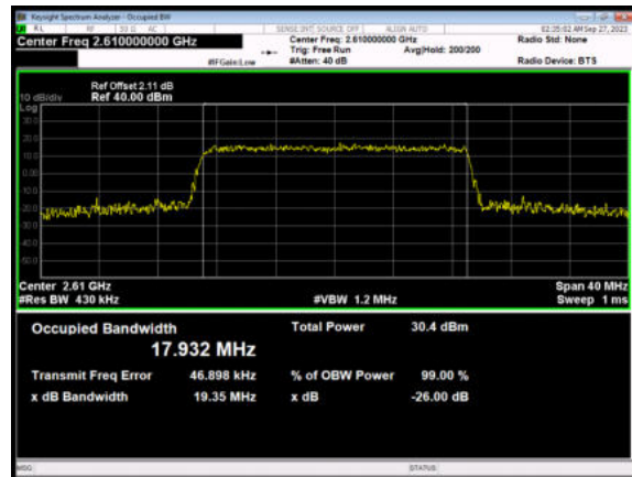
LTE Band 38 16QAM 20MHz CH-High
