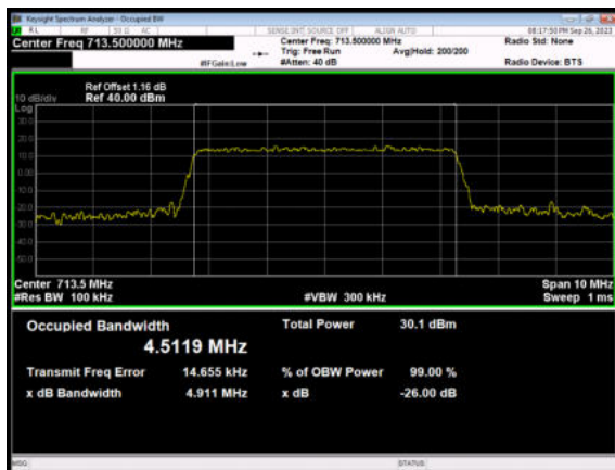
LTE Band 12 64QAM 5MHz CH-High
