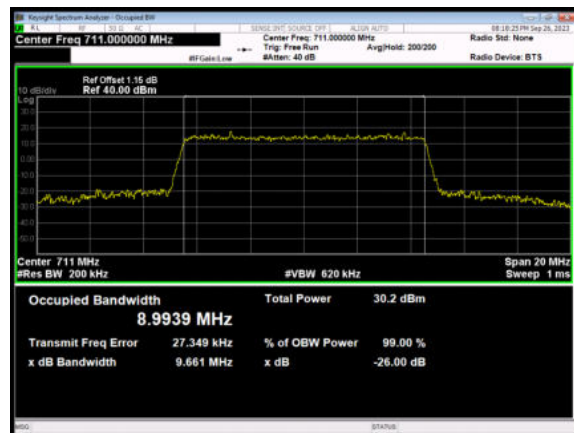
LTE Band 12 64QAM 10MHz CH-High
