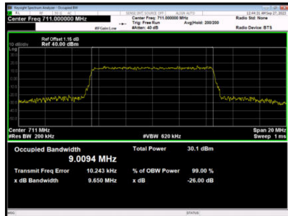
LTE Band 17 16QAM 10MHz CH-High
