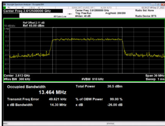
LTE Band 38 16QAM 15MHz CH-High
