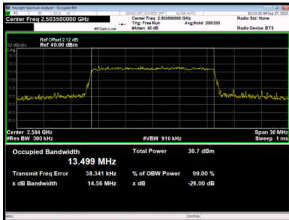
LTE Band 41 64QAM 15MHz CH-Middle
