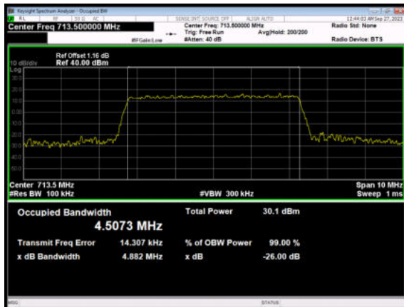
LTE Band 17 16QAM 5MHz CH-High
