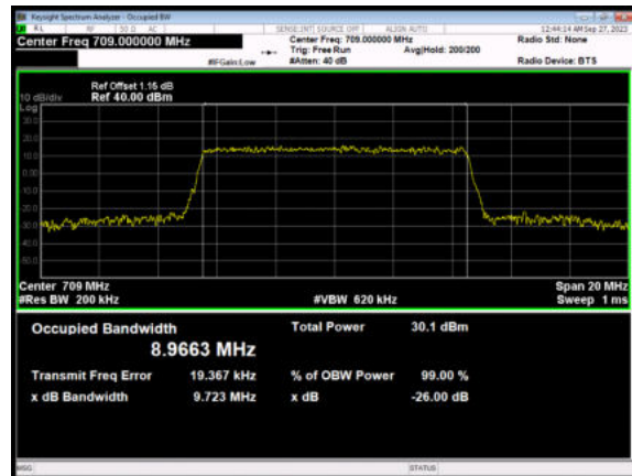
LTE Band 17 16QAM 10MHz CH-Middle
