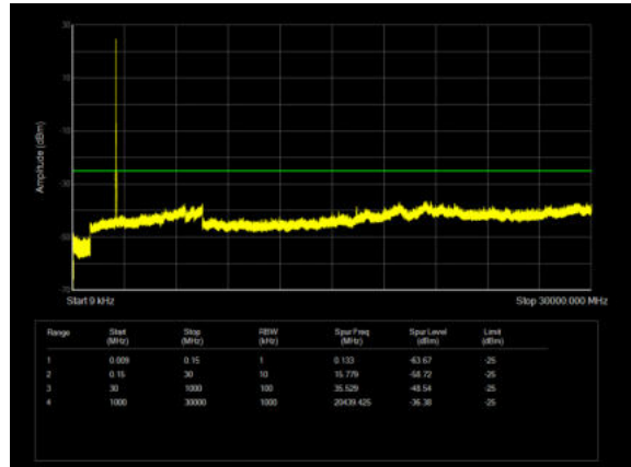
LTE Band 41 20MHz CH- Middle 9kHz~30GHz
