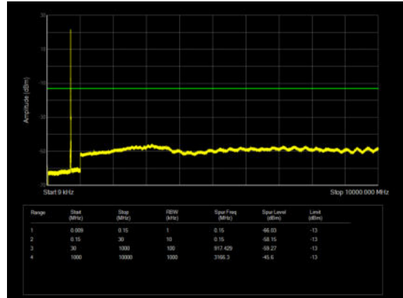
LTE Band 17 10MHz CH-High 9kHz ~10GHz
