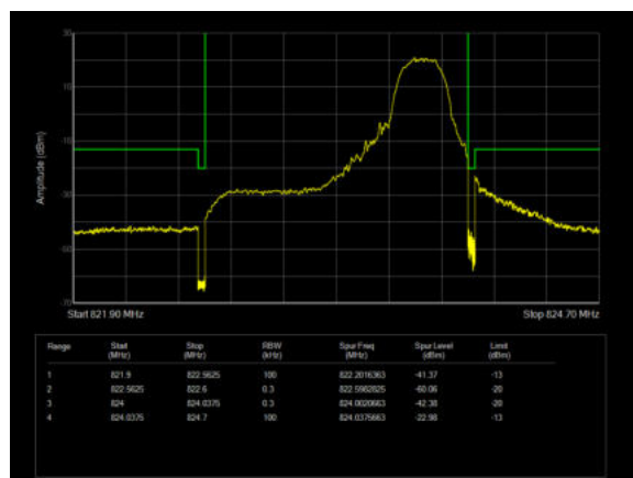
LTE Band 26 64QAM 1.4MHz CH-High 100%RB
