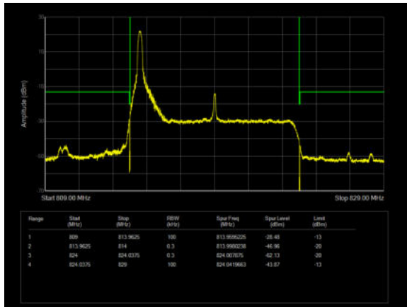
LTE Band 26 QPSK 10MHz CH-Low 100%RB
