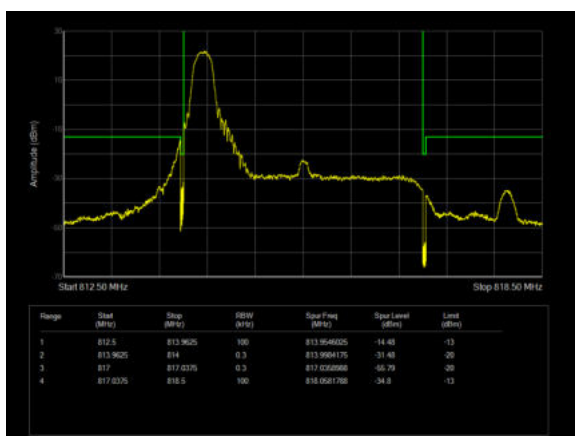
LTE Band 26 QPSK 3MHz CH-Low 1RB
