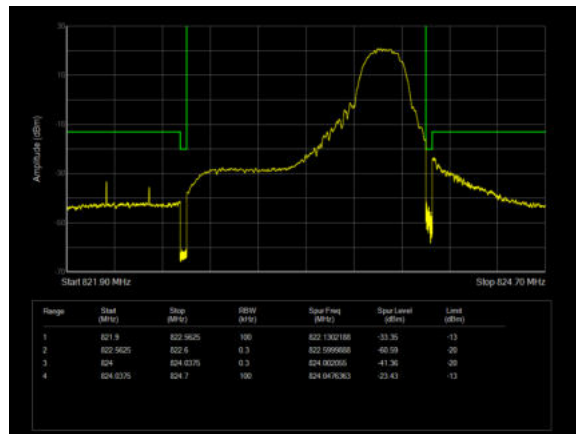
LTE Band 26 16QAM 1.4MHz CH-High 1RB
