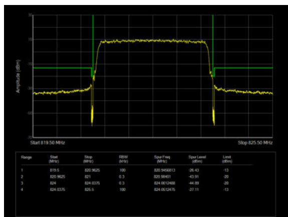
LTE Band 26 QPSK 5MHz CH-High 1RB
