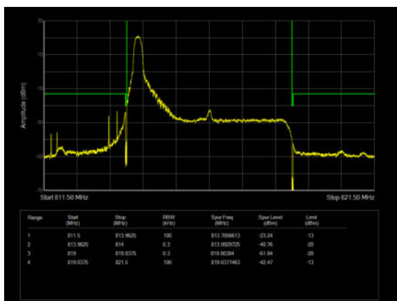
LTE Band 26 64QAM 5MHz CH-Low 1RB
