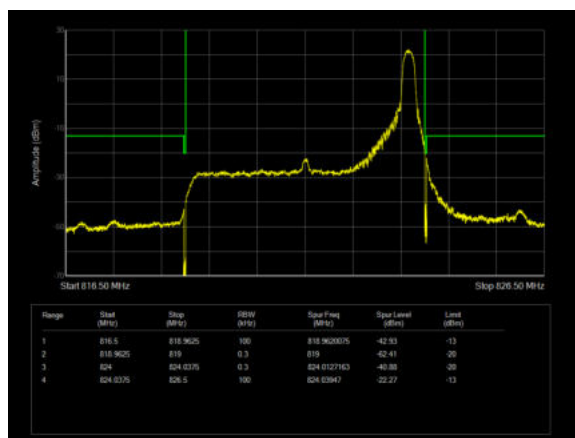
LTE Band 26 QPSK 5MHz CH-High 100%RB
