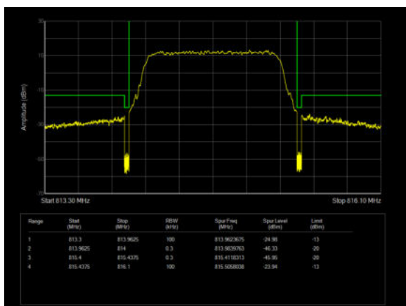
LTE Band 26 64QAM 1.4MHz CH-Low 100%RB
