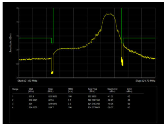
LTE Band 26 QPSK 1.4MHz CH-High 100%RB
