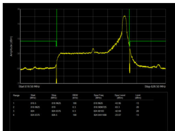
LTE Band 26 16QAM 5MHz CH-High 100%RB
