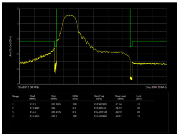
LTE Band 26 QPSK 1.4MHz CH-Low 100%RB
