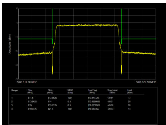
LTE Band 26 QPSK 5MHz CH-Low 100%RB
