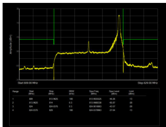
LTE Band 26 64QAM 10MHz CH-High 100%RB
