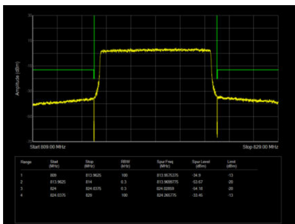
LTE Band 26 64QAM 10MHz CH-Low 100%RB
