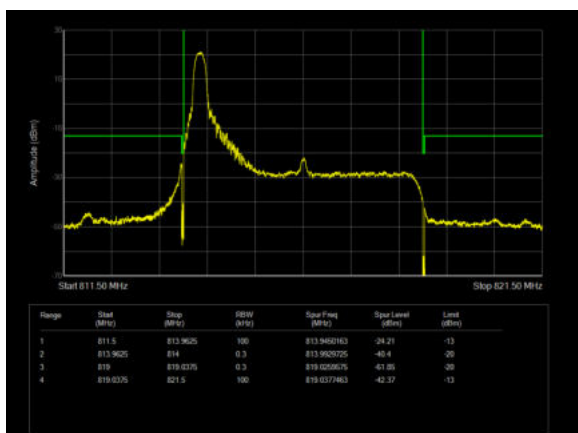
LTE Band 26 16QAM 5MHz CH-Low 100%RB
