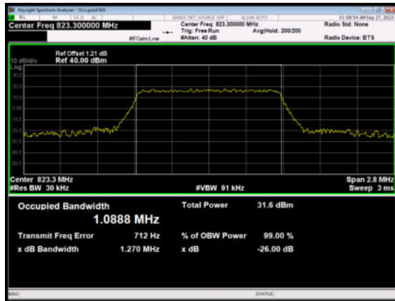
LTE Band 26 QPSK 1.4MHz CH High
