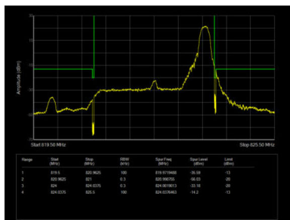
LTE Band 26 QPSK 3MHz CH-High 1RB
