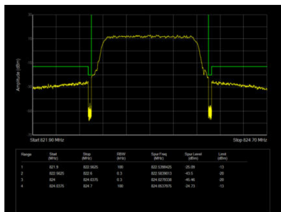
LTE Band 26 16QAM 3MHz CH-High 1RB
