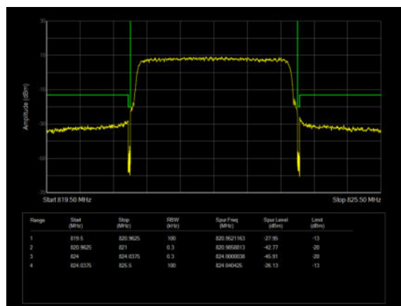
LTE Band 26 64QAM 5MHz CH-High 1RB
