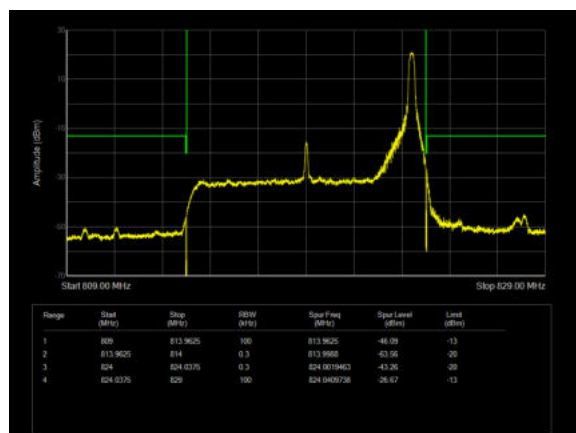
LTE Band 26 16QAM 10MHz CH-High 1RB
