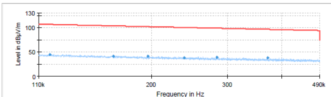
Radiates Emission from 110kHz to 490kHz
