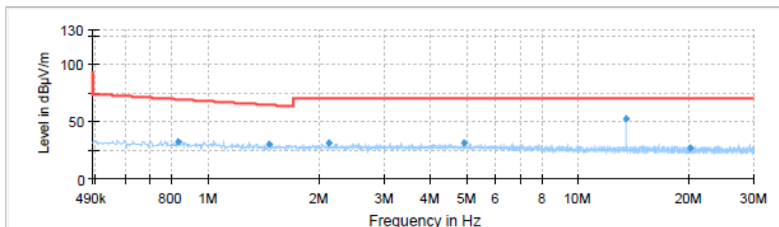
Radiates Emission from 490kHz to 30MHz
